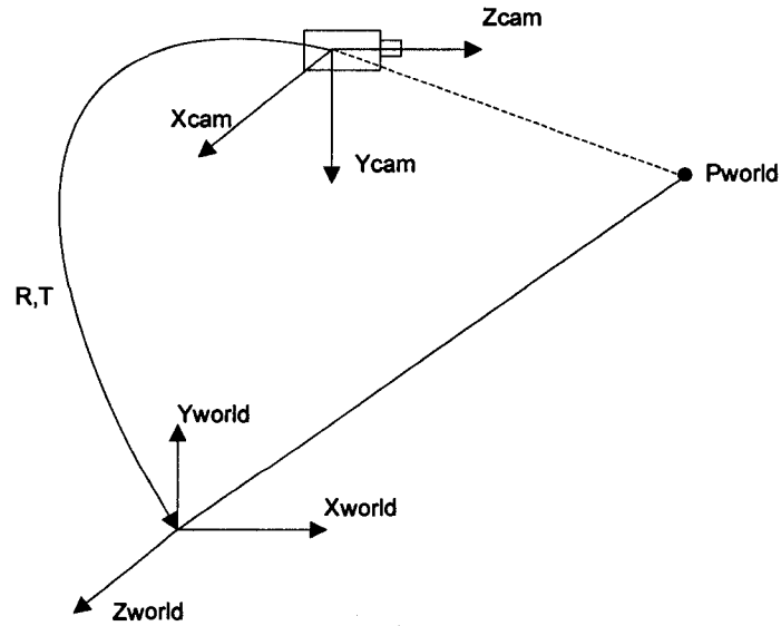
Figure 2.2. Extrinsic camera transformation graph
