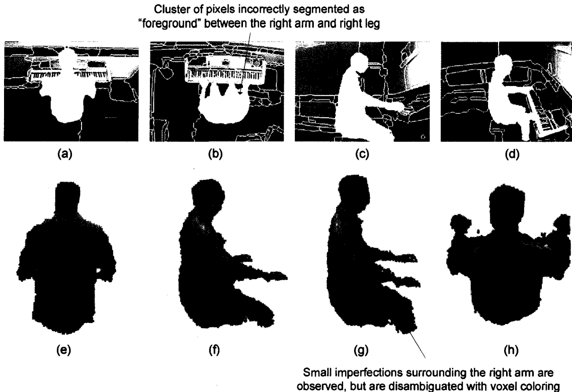
Figure 5.22. Shape-from-silhouette reconstruction using silhouette data obtained from a region-based segmentation method [9, 10]
