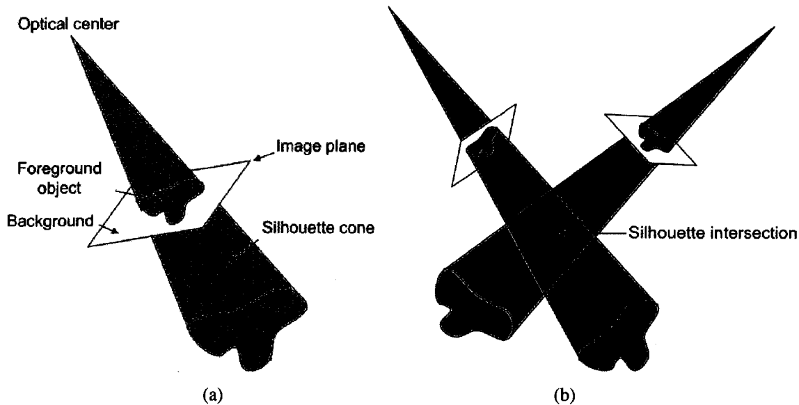
Figure 2.6. Basics of shape-from-silhouette volumetric reconstruction.
