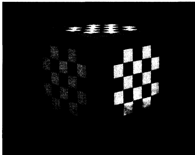
Figure 2.4. The design of a (20 cm) 3 calibration cube
