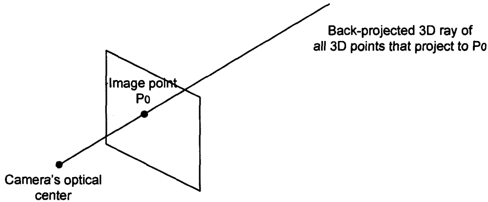
Figure B.1. Back-projection of an image point in 3D space
