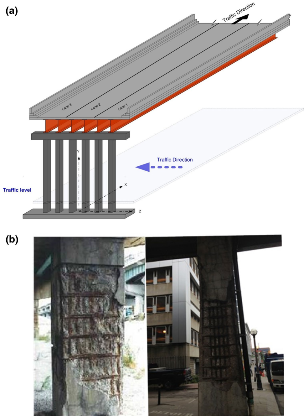
Fig. 11 a Case study V: bridge column of slab-on-girder bridge subjected to local corrosion. b (i) Case study V: sample of slab-on-girder bridge columns with partial corrosion damage (Gardiner Parkway-Expressway, Toronto, Canada). (ii) Case study V:(a) most affected corrosion zone on a slab-on-girder bridge column; (b) column reinforcement and location of mid-height section; (c) column cross-section details. c Case study V: possible damage of RC beam-column subjected to combined external loads and corrosion: (a) flexural and corrosion cracks; (b) initial spalling; (c) one stirrup failure; (d) spalling on all sides; (e) two stirrups failure; (f) loss of confinement and possible buckling. d Case study V: FE discretization of the column and lateral displacement of un-corroded (UC) and corroded (CO) column, both with e = 5H , for (a) below yield load ( M = 3000 \text{ kN}\cdot\text{m} ); (b) after yield and below ultimate ( M = 6000 \text{ kN}\cdot\text{m} ); and, (c) at ultimate load ( M_{UC} = 8200 \text{ kN}\cdot\text{m} and M_{CO} = 6750 \text{ kN}\cdot\text{m} ). e Case study V: M - \Delta_{\text{lateral}} at the mid-height section of the column where the corrosion load is applied, for e = 5H and for different corrosion cases
