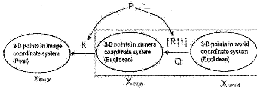
Figure 2.4: The relationship among P , K and Q .
