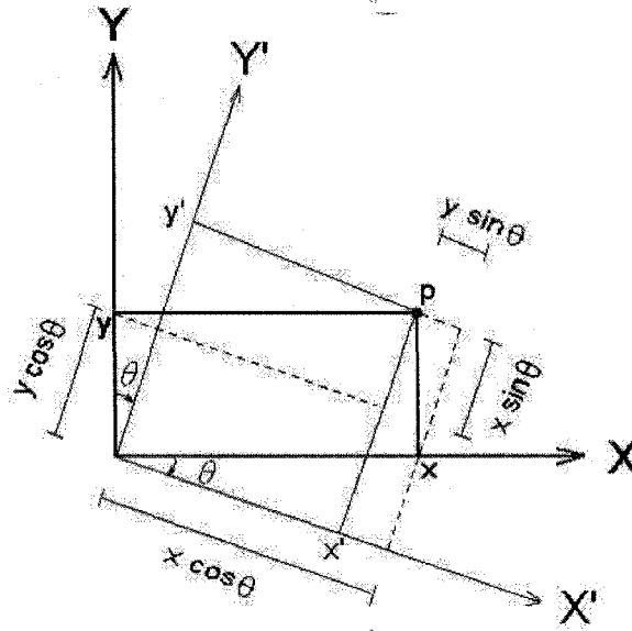
Figure 2.6: Rotation of a coordinate system.
