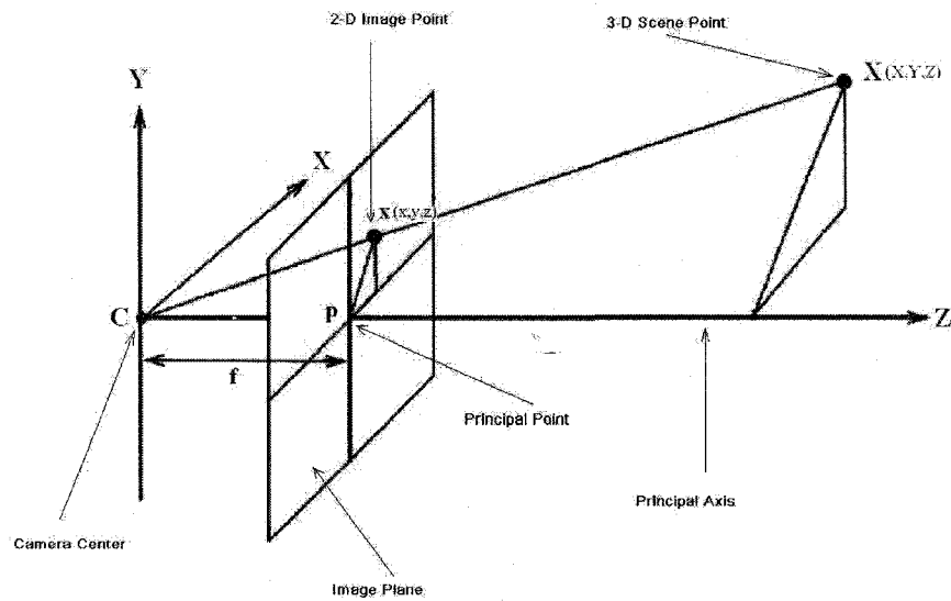
Figure 2.1: Pinhole camera model.
