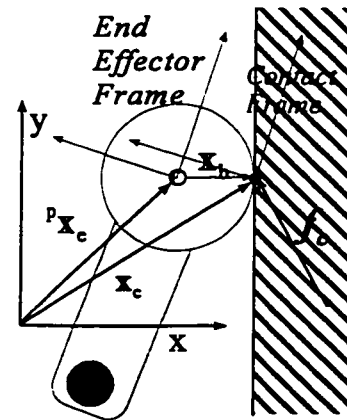
Figure 2.9 - Contact Frame
