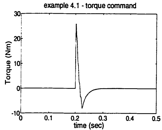
Figure 4.4 - Control Torque
