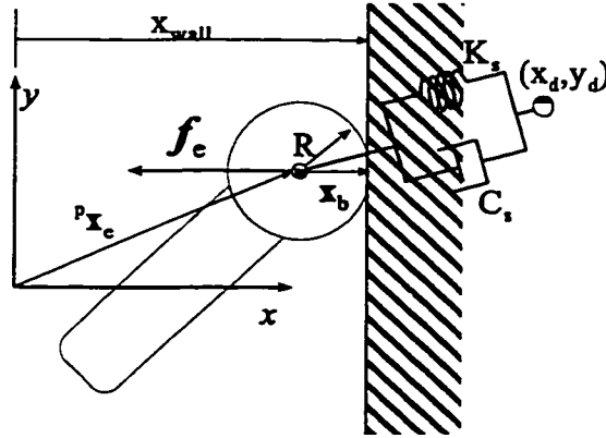
Figure 3.4 Stiffness Control
