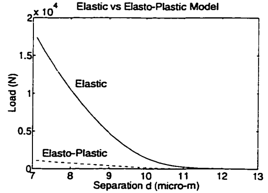
Figure 2.4 - Contact Load
