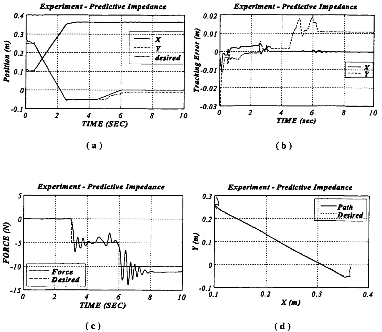
Figure 6.11 - Experimental results - Extended Model Predictive Impedance
