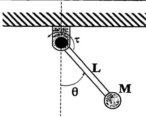
Figure 4.5 - Pendulum
