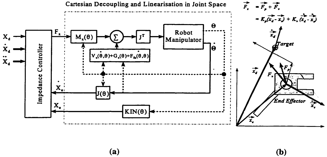
Figure 5.3 - Impedance Control
