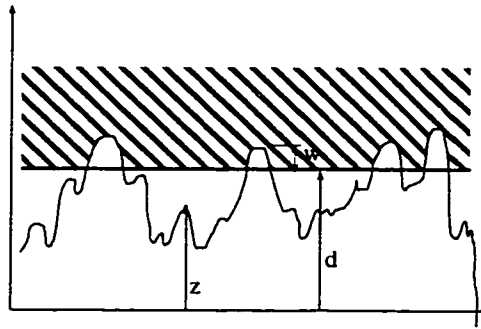
Figure 2.2 - GW Contact profile
