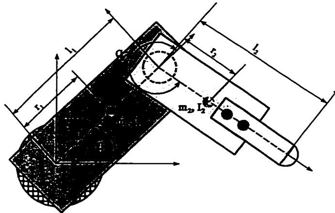
Figure 6.2 - Robot Geometry
