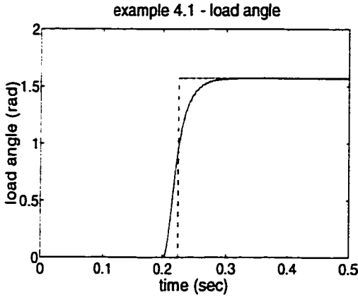
Figure 4.3 - Load Angle
