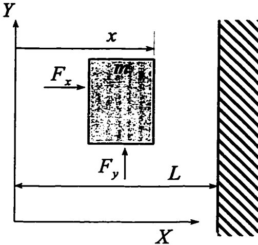
Fig. 3.3 - Unilateral Constraints
