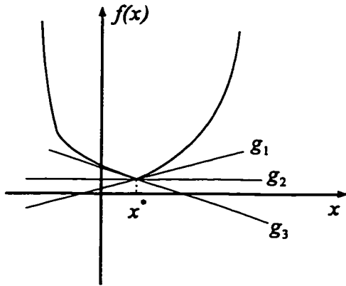
Figure 5.7 - Subdifferential
