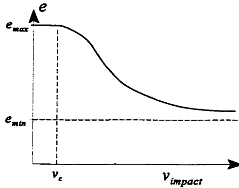
Figure 2.5 - Coefficient of Restitution vs impact speed
