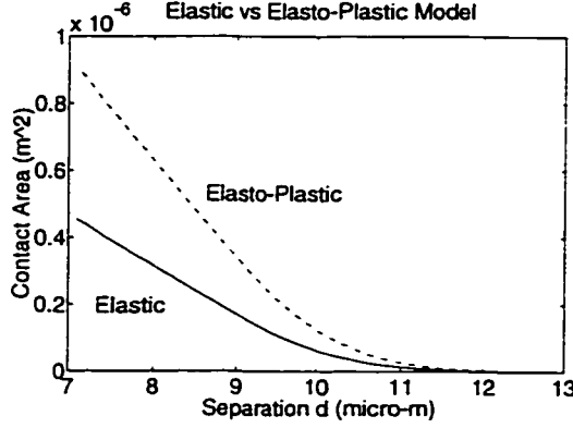
Figure 2.3 - True Contact Area
