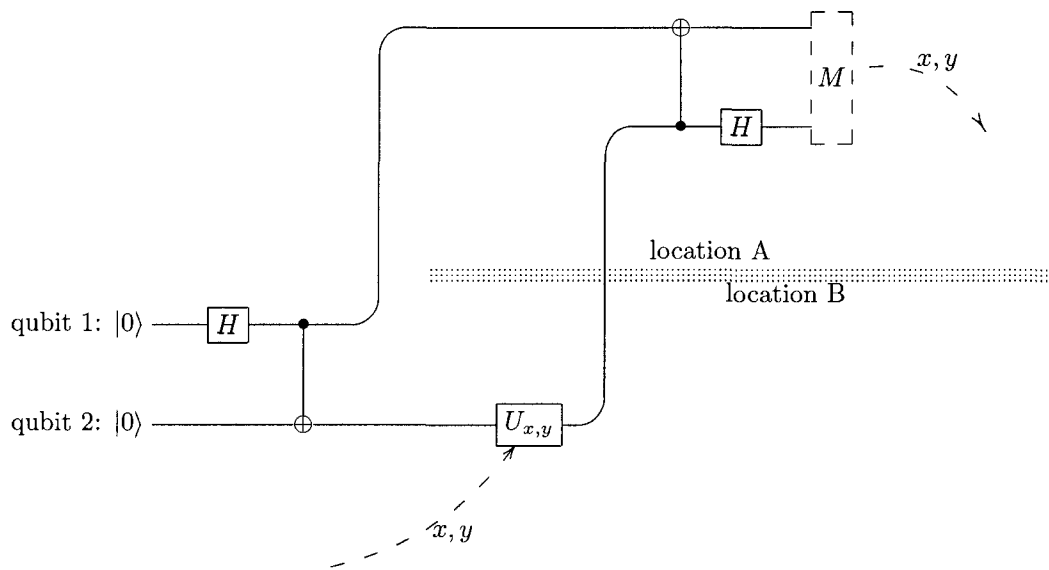
Figure 3.3: Dense coding protocol.
