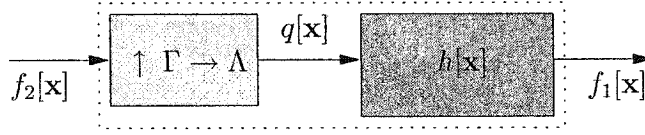
Fig. 2.1 Image up-sampling.
