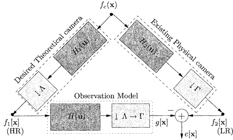
Fig. 4.1 Scenario for image up-sampling.
