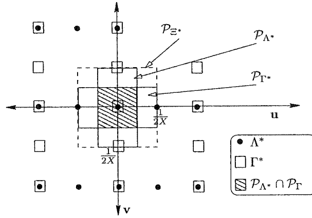
Fig. 2.4 Sample passband of H(\mathbf{u}) .
