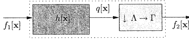
Fig. 2.2 Image down-sampling.
