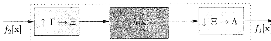
Fig. 2.3 Image arbitrary rate conversion.
