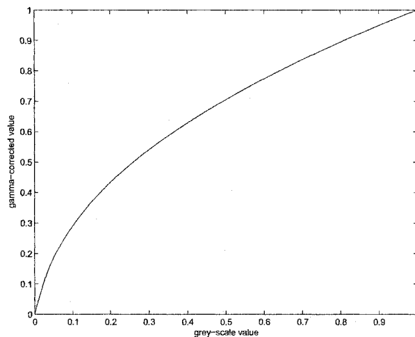
Fig. 5.1 ITU R Rec. 709 for gamma correction.
