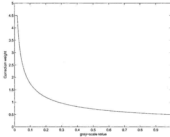
Fig. 5.2 Correction weights \frac{\partial f^{(\gamma)}}{\partial f} .
