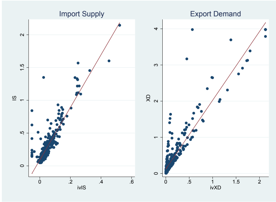
Figure 6: Raw measures vs instrumental variables measures
