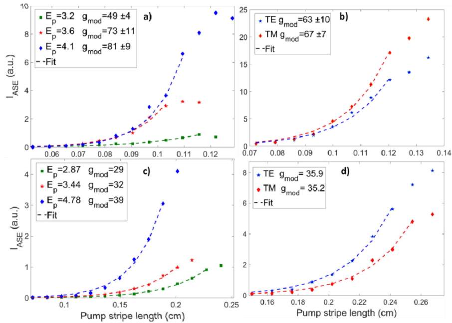
Fig. 5. (a) and (c): Emission intensities as a function of the stripe length for the sample with 0.9% IR-140 and a thickness of t_{PMMA} = 4 \mu m (a), and 0.8% IR-140 and a thickness of t_{PMMA} = 1 \mu m (c). (b) and (d): Emission intensities in the TM and TE orientations as a function of the stripe length for the sample with 0.9% IR-140 and a thickness of t_{PMMA} = 4 \mu m (b), and 0.8% IR-140 and a thickness of t_{PMMA} = 1 \mu m (d). The modal gain g_{mod} (in cm^{-1} ) is obtained by fitting Eq. (6) to the measurements. Pump energy densities E_d are in mJ/cm^2 .
