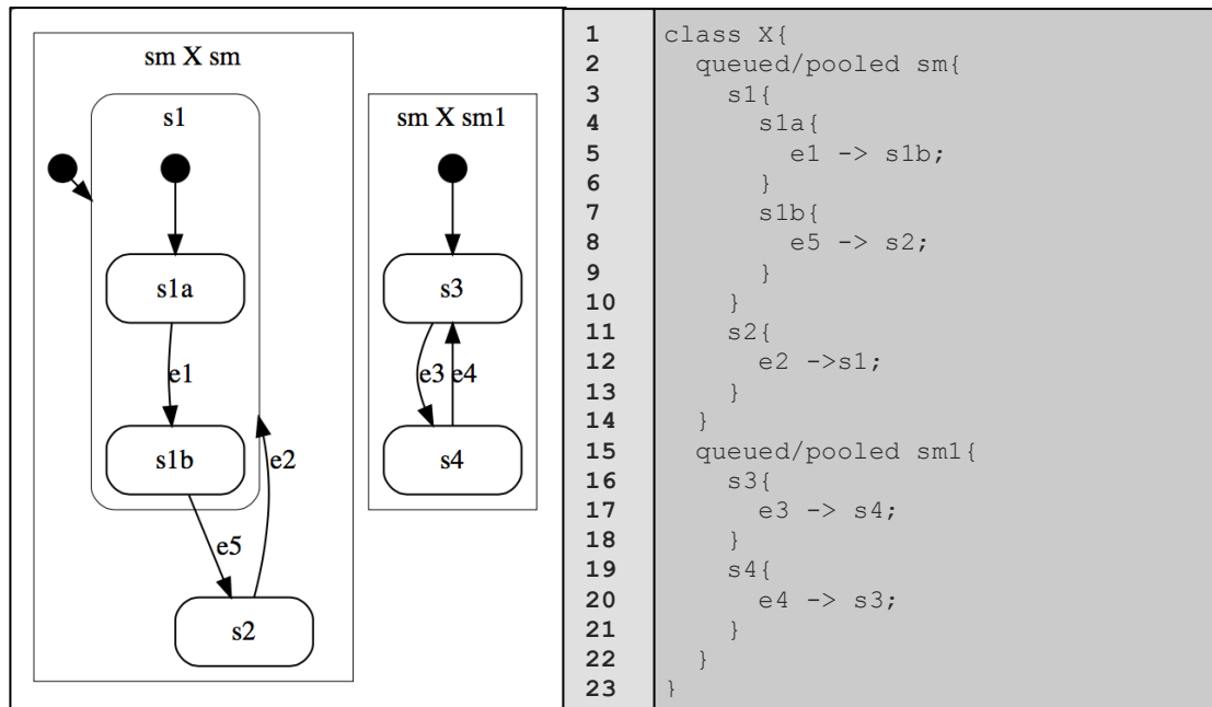
Figure 5.7: A state diagram for multiple queued state machines in one class as shown in UmlpeOnline
