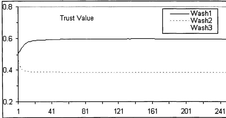
Figure 34: Trust value in Scenario 4 (bootstrap)
