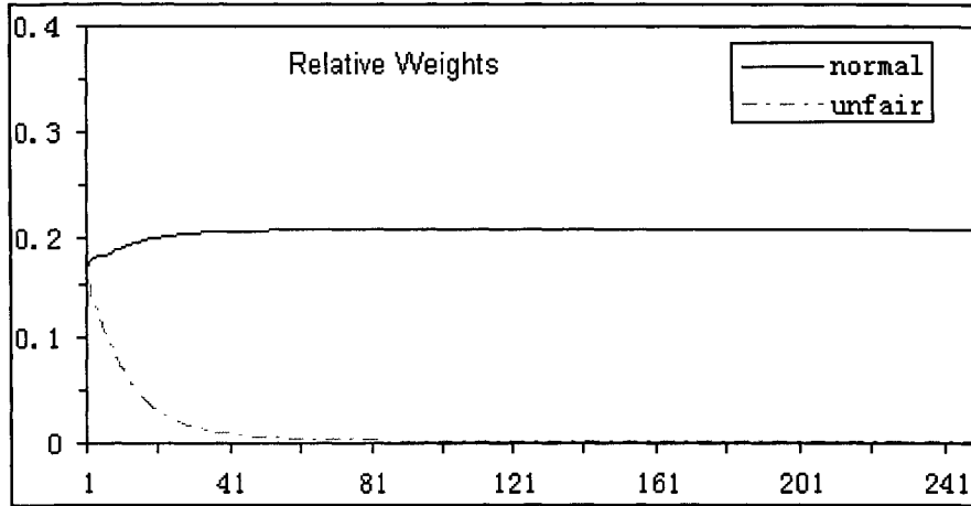
Figure 10: Relative weights in Scenario 4 (single)
