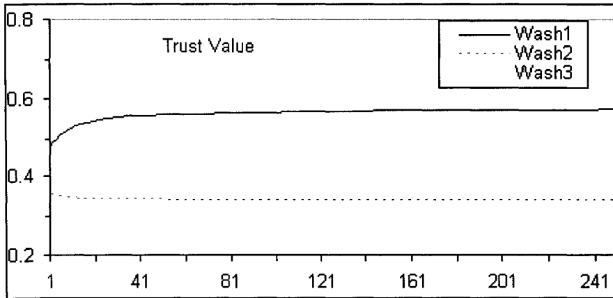
Figure 14: Trust value in Scenario 2(multiple)
