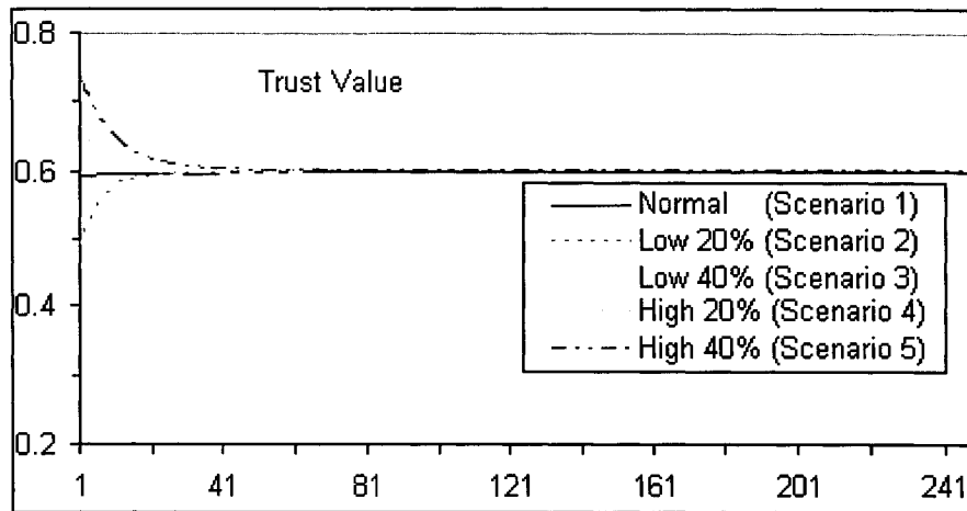
Figure 7: Trust value in Scenarios 1 through 5 (single)
