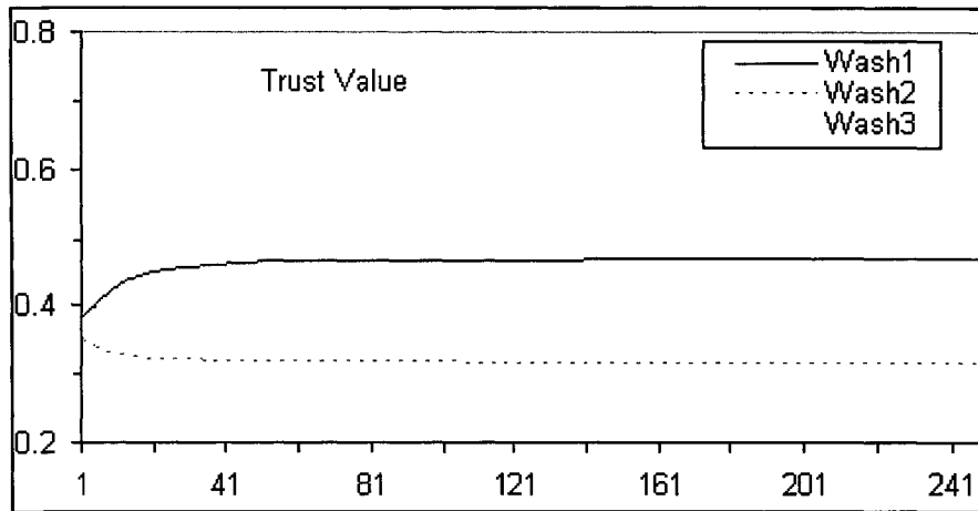
Figure 17: Trust value in Scenario 3 (multiple)
