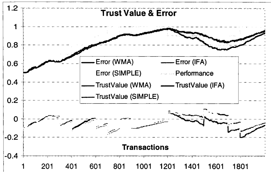
Figure 40: Trust value, performance and error with 0% unfair recommenders
