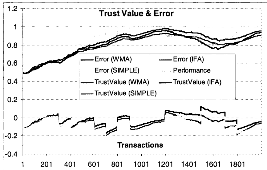
Figure 41: Trust value, performance and error with 20% unfair recommenders
