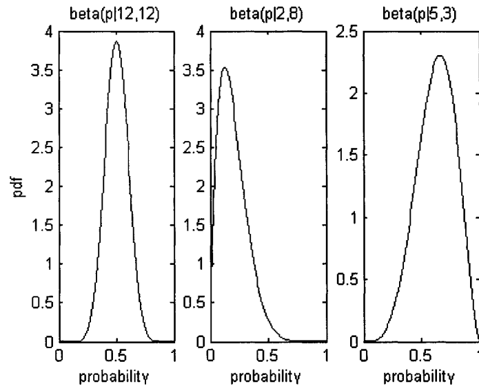
Figure 1: Beta distributions
