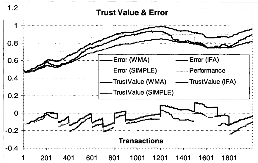
Figure 42: Trust value, performance and error with 40% unfair recommenders
