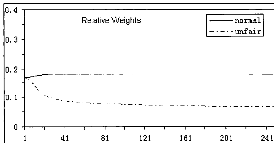
Figure 31: Trust value in Scenario 3 (bootstrap)
