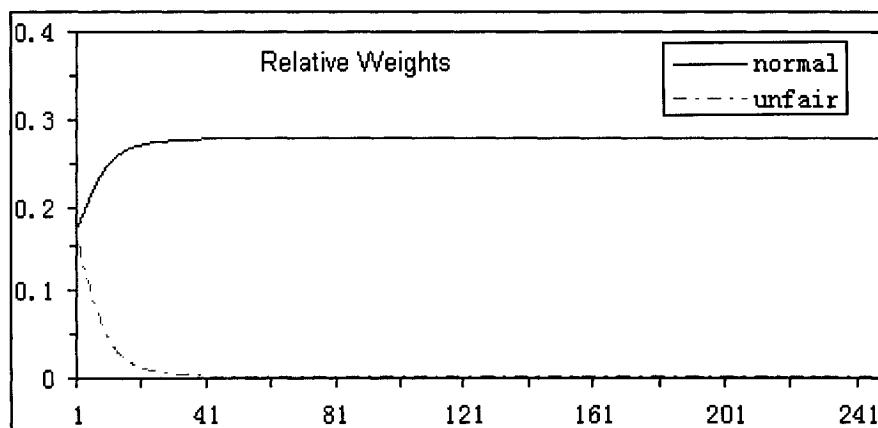
Figure 9: Relative weights in Scenario 3 (single)
