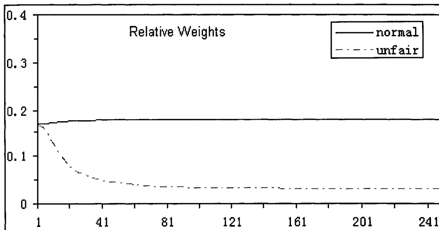
Figure 28: Trust value in Scenario 2 (bootstrap)
