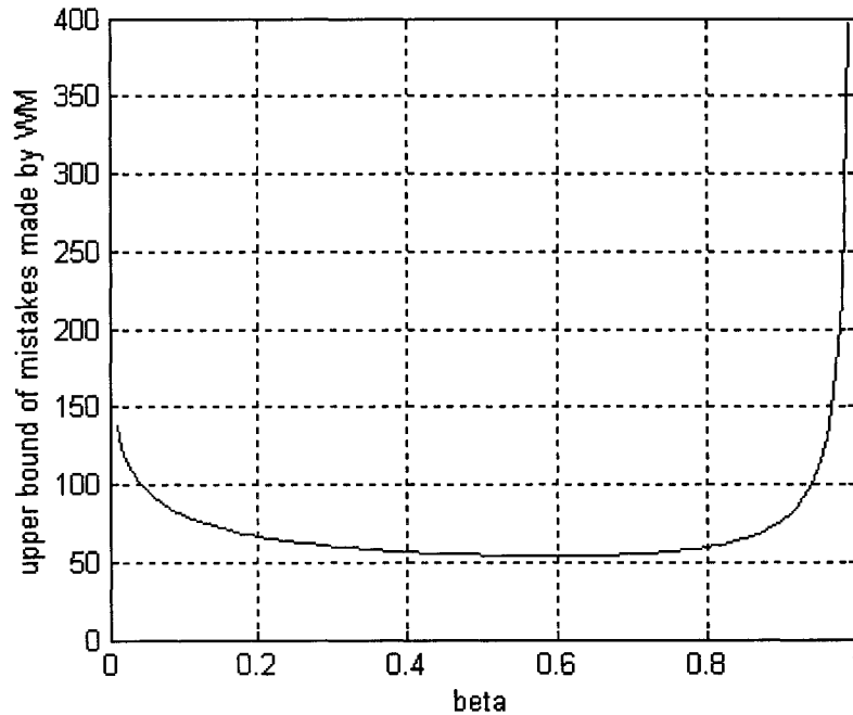
Figure 3: The upper bound of mistakes
