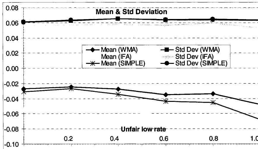
Figure 46: Mean and standard deviation of average error ( \alpha=0.99, Punfair=1 )
