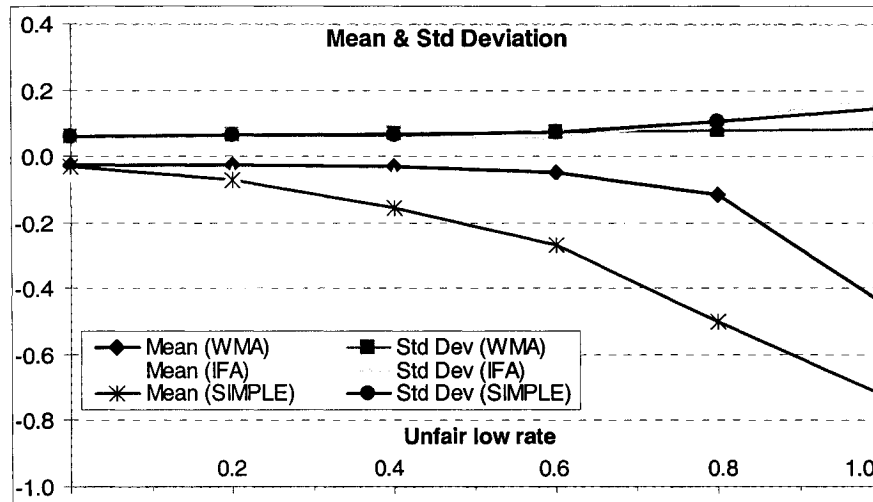
Figure 45: Mean and standard deviation of average error ( \alpha=0.2, Punfair=0.25 )
