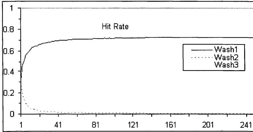
Figure 33: Hit rate in Scenario 3 (bootstrap)
