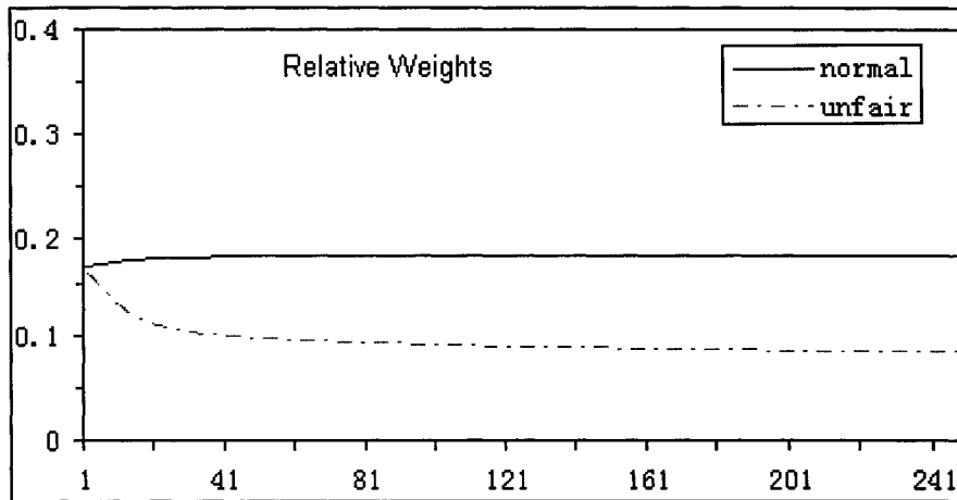
Figure 18: Relative weights in Scenario 3 (multiple)
