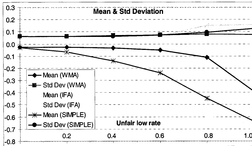
Figure 43: Mean and standard deviation of average estimation error
