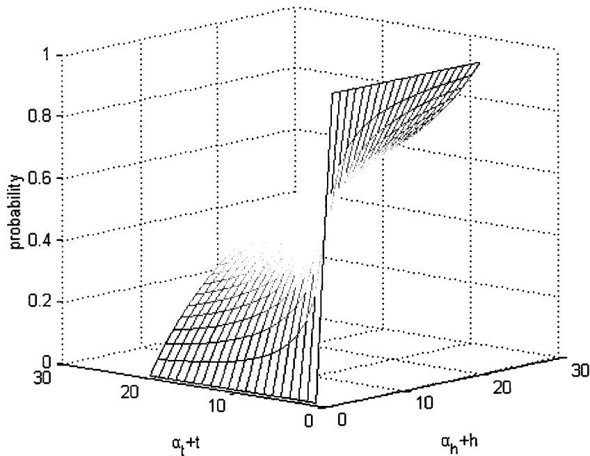
Figure 2: Bayesian estimation
