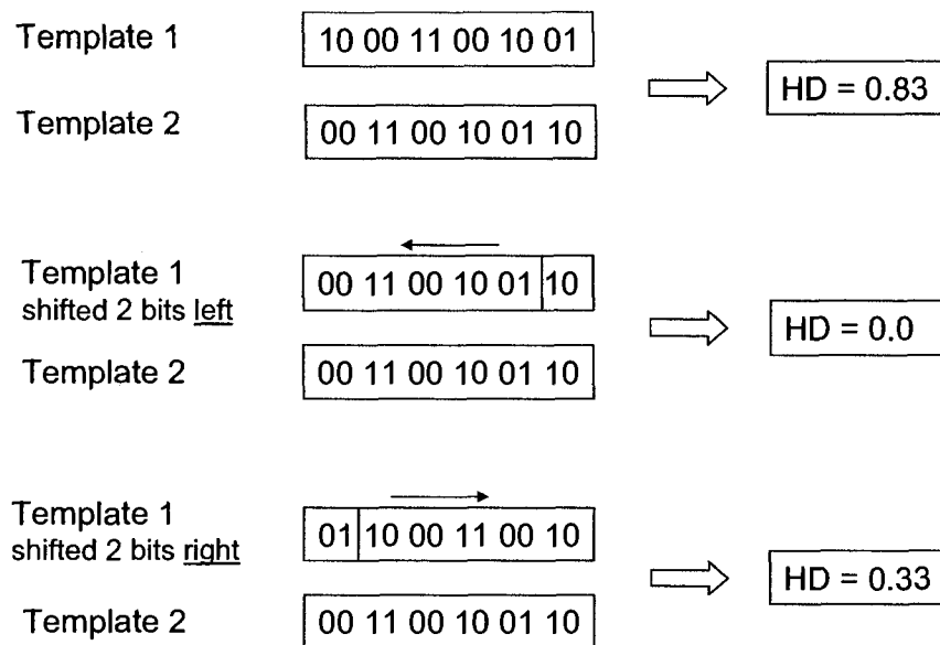
Figure 4.3: An example of template shifting adapted from (Masek, 2003). The reference template (Template 1) is shifted 2 bits right once and shifted 2 bits left once in search of the best match. Shifting left gave the perfect match with HD=0 .
