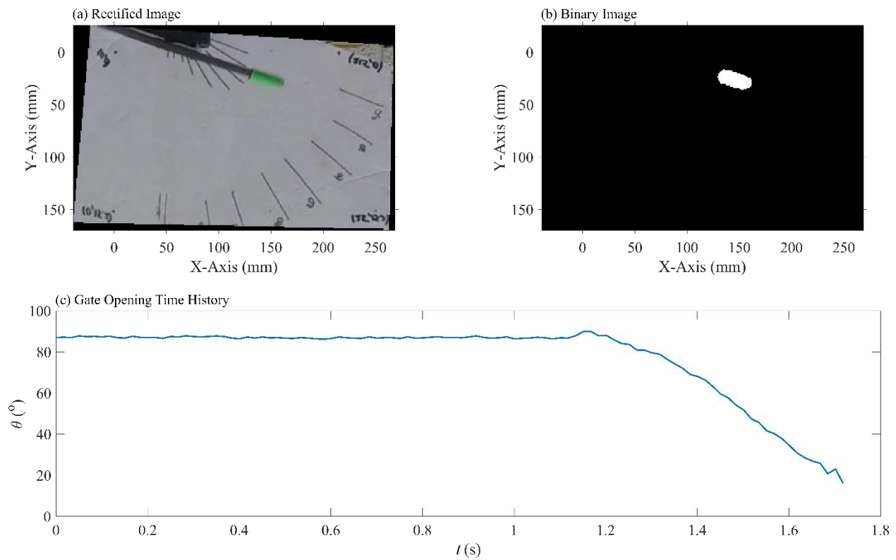
Fig. A - 3. Gate opening tracking algorithm used to determine the gate opening time. (a) GoPro image rectified within the plane of the angular scale, (b) binary image developed using color thresholding; and (c) time history of the gate opening.
