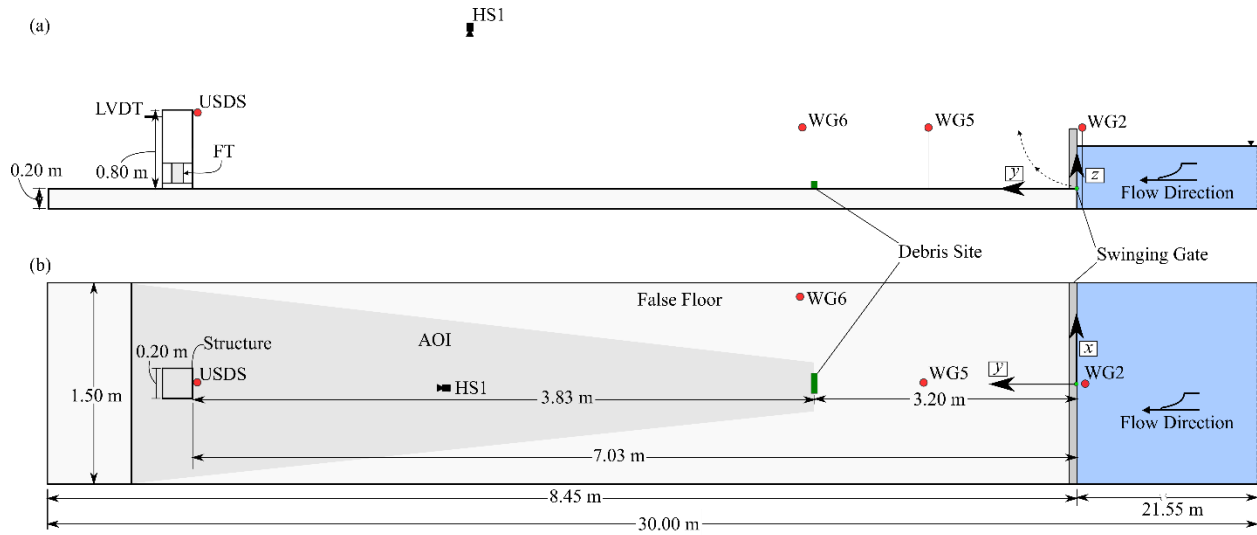
Fig. 5-24. Dam-break Flume (DBF) at the University of Ottawa, Canada: (a) side view and (b) top view. The initial debris site is indicated with a green rectangle. The wave gauge (WG) positions are indicated using red circles.
