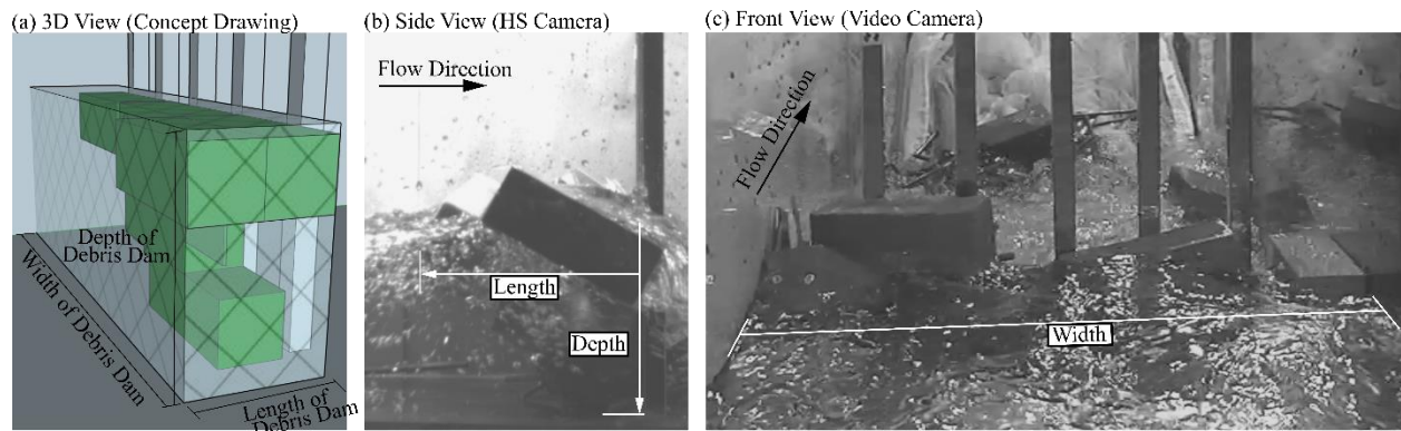
Fig. 4-22. Measurements of the debris dam properties. (a) conceptual image; (b) view from the HS; (c) view from the VC.
