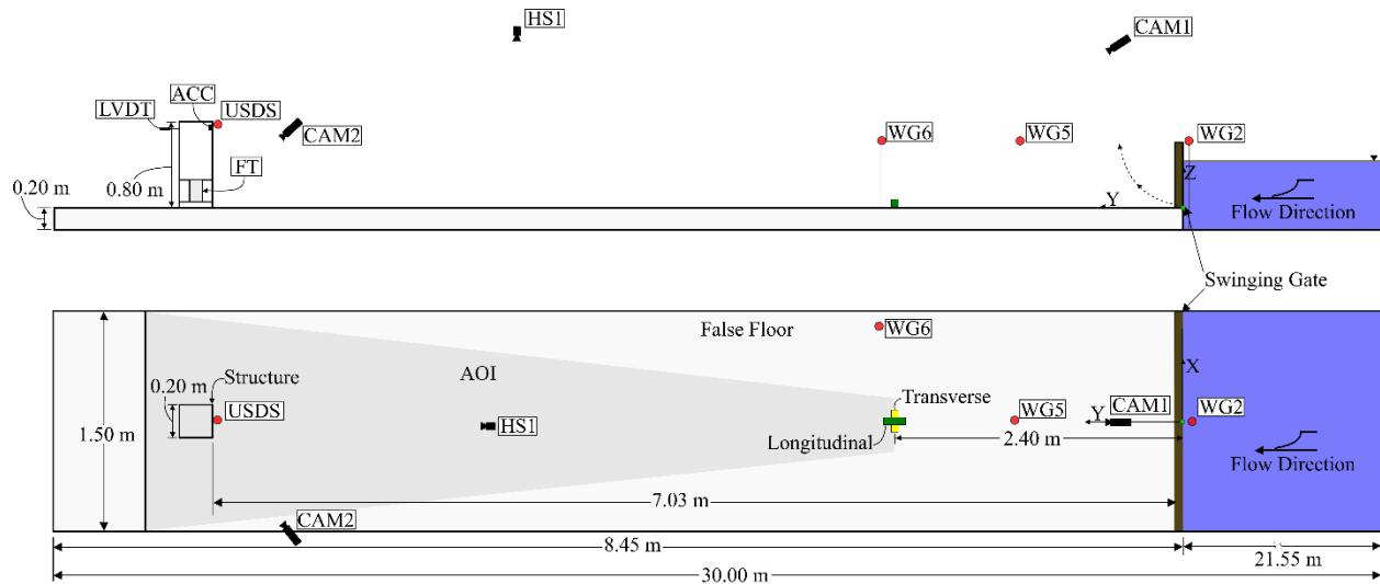
Fig. 5-1. University of Ottawa Dam-break Wave Flume. ACC = accelerometer, USDS = ultrasonic distance sensor, LVDT = linear variable differential transform, CAM = camera, FT = load cell, HS = High Speed Camera, WG = wave gauge.
