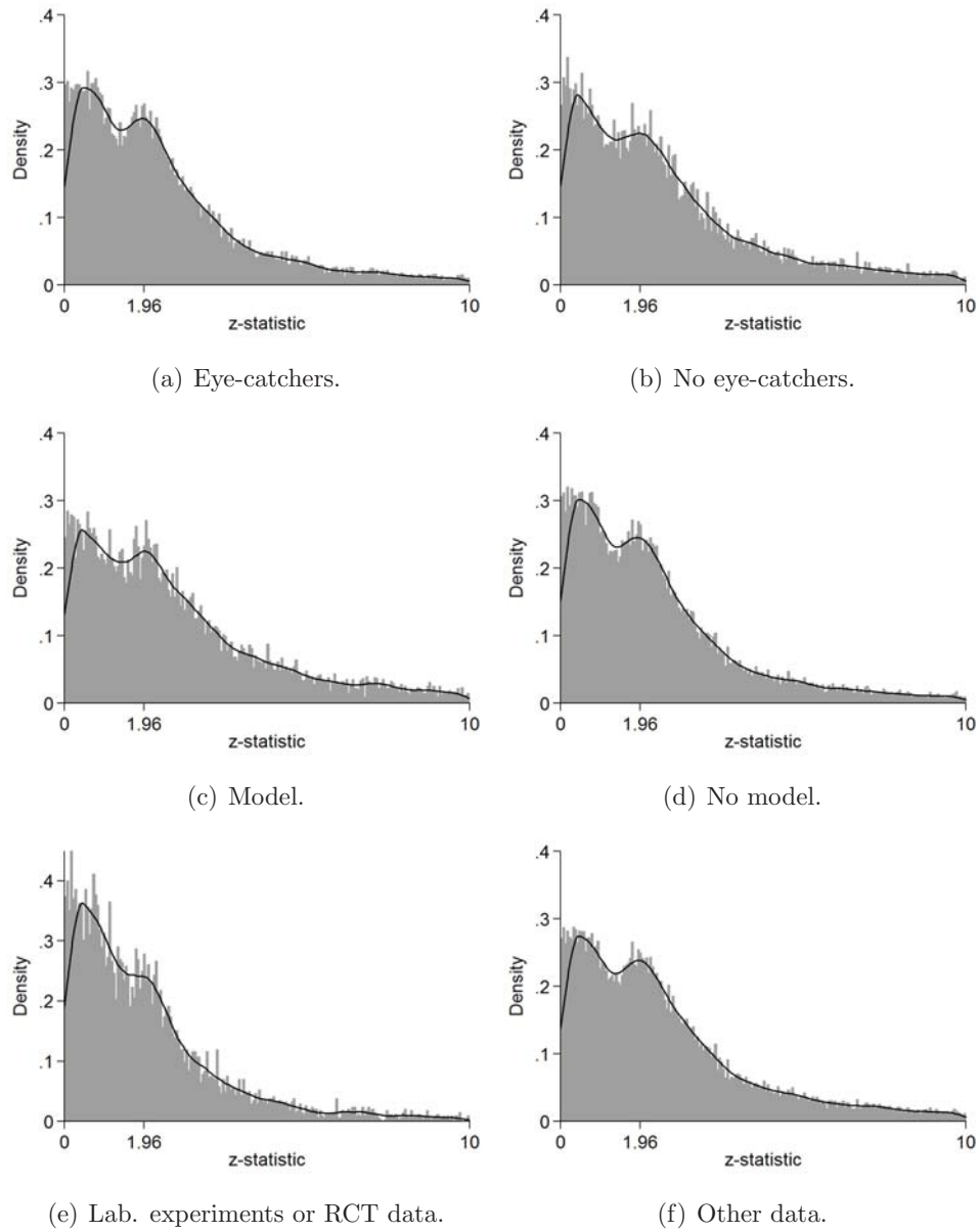
Figure 6: Distributions of z-statistics for different sub-samples: use of eye-catchers, presence of a theoretical contribution, and type of data used.
