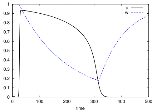
Figure 4.10: Test case 2: plot in time of the solution at the point (50, 50) .
