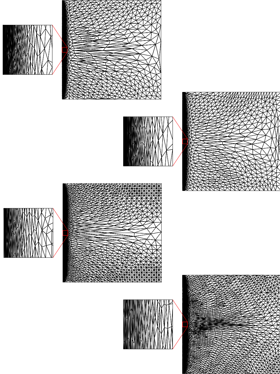
Figure 2.8: Adapted meshes for u_1 with approximately 2500 vertices, with zoom near the boundary at x = 0 . From top to bottom: residual (element), residual (metric), Hessian, hierarchical.
