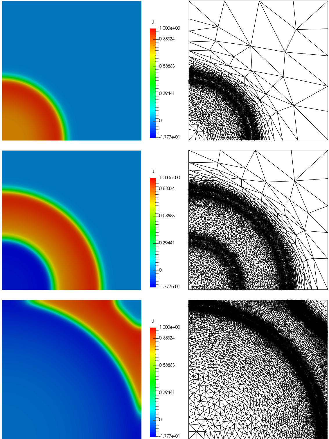
Figure 4.2: Test case 1: transmembrane potential u (left) and corresponding adapted mesh (right) when applying the adaptive method with TOL_S^U = 0.125 , TOL_S^W = 0.0125 and \tau = 0.5 at t = 87.5 (top), t = 175 (centre) and t = 350 (bottom).
