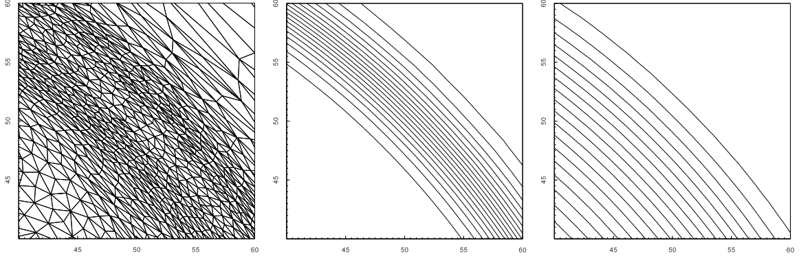
Figure 4.3: Test case 1: zoom of the mesh at wave-front at time t = 175 (left), and contours of u (centre) and w (right).
