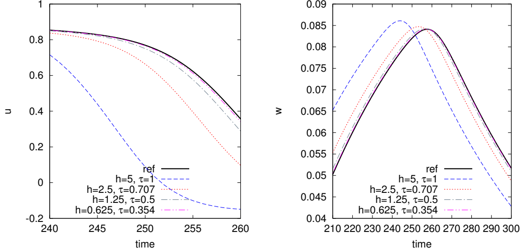
Figure 4.4: Test case 1: comparison of reference solution with solutions on uniform meshes, plotted at point (x, y) = (0.5, 0.5) of u (left) and w (right).
