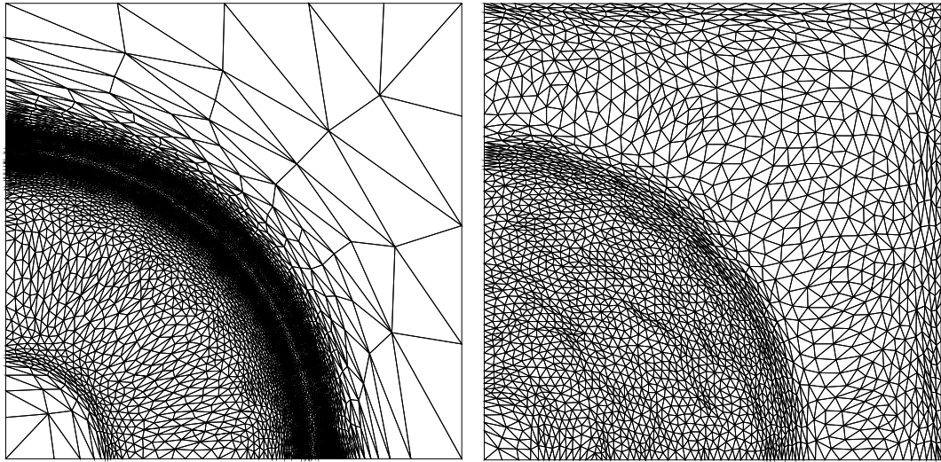
Figure 4.15: Test case 2: adapted mesh at t = 30 (left) during the depolarization phase and at t = 316 (right) during the repolarization phase.
