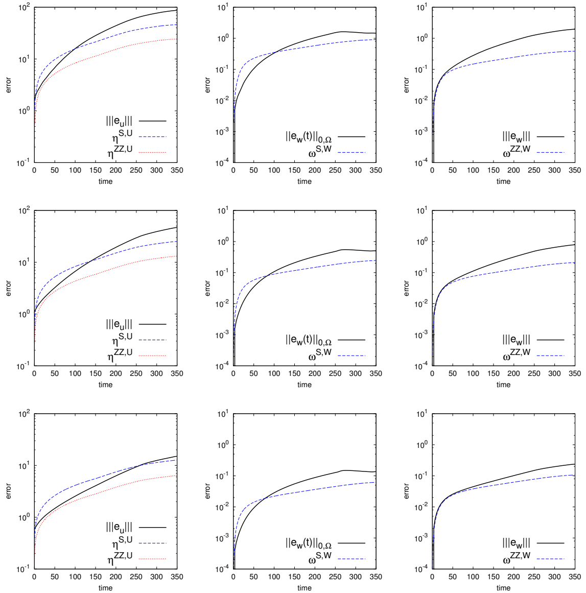
Figure 4.7: Test case 1: estimators and exact error solving with uniform meshes with h = 5, \tau = 1 (top), h = 2.5, \tau = 0.5 (centre), h = 1.25, \tau = 0.25 (bottom).
