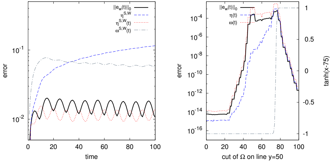
Figure 4.1: Left: plot of the total error over time. Right: plot of the error (left y -axis) and source term (right y -axis) over the line y = 50 at time t = 100 .
