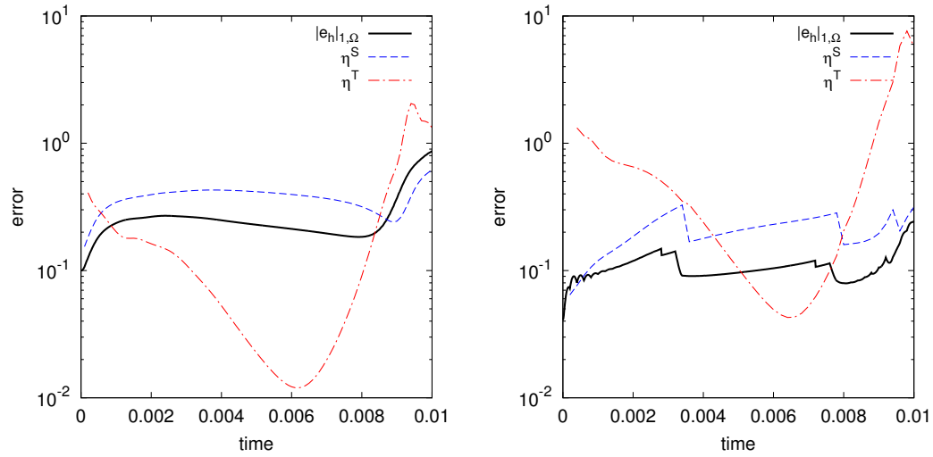
Figure 3.6: Plot of error for Test case 2. Plot of error in time on a uniform mesh with h = 0.025, \tau = 2 \times 10^{-4} (left) and using space-only adaptation with TOL_S = 0.25, \tau = 2 \times 10^{-4} (right).
