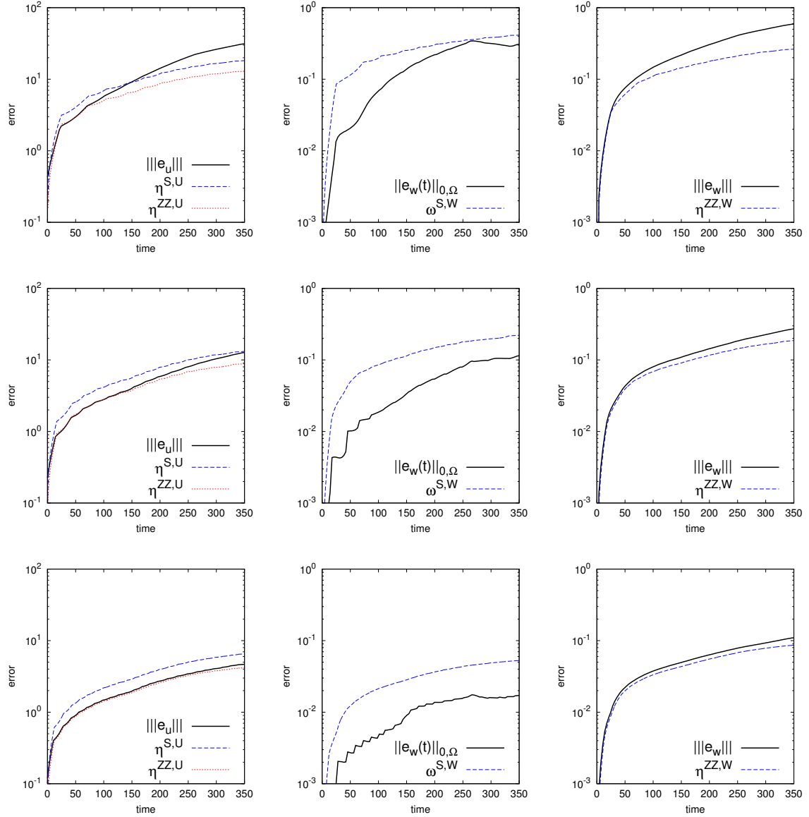
Figure 4.8: Test case 1: estimators and exact error when applying mesh adaptation with TOL_{S,U} = 0.5, TOL_{S,W} = 0.2, \tau = 1 (top), TOL_{S,U} = 0.25, TOL_{S,W} = 0.2, \tau = 0.5 (centre), TOL_{S,U} = 0.125, TOL_{S,W} = 0.05, \tau = 0.25 (bottom).
