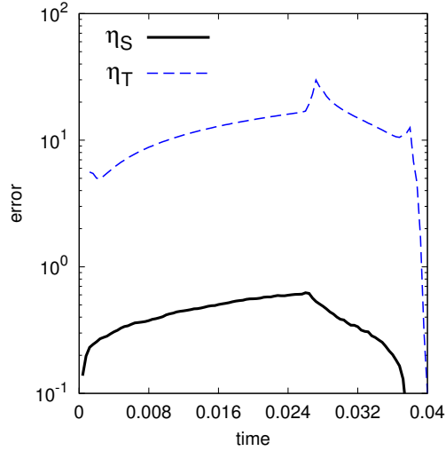
Figure 3.1: Test case 1: plot of the error estimators in time for the solution on a uniform mesh.
