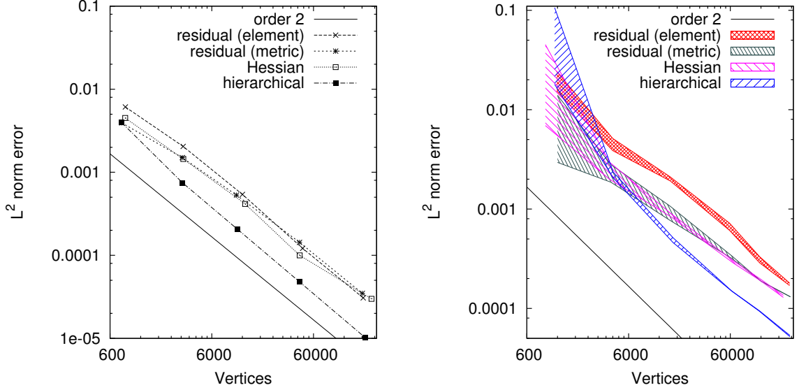
Figure 2.13: L^2 norm error calculations for u_2 with \alpha = 100 (left) and \alpha = 1000 (right). The plot on the right depicts the envelope of the oscillating error.
