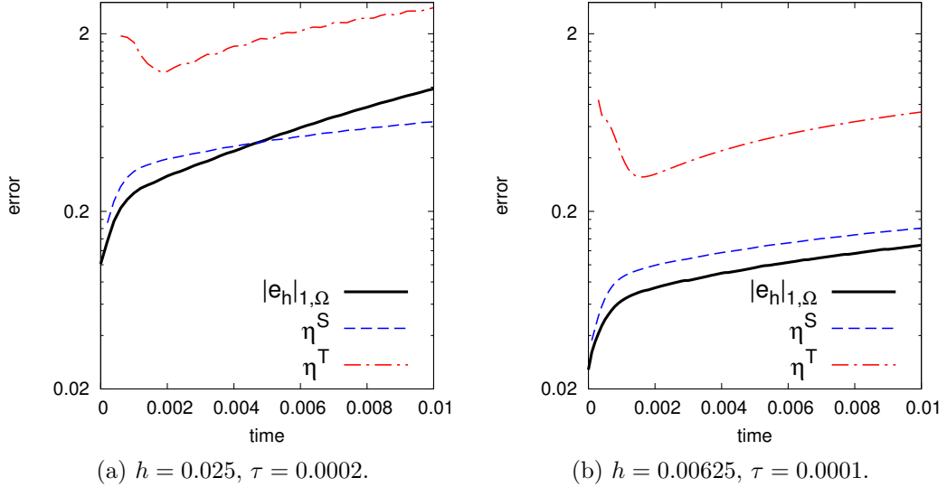
Figure 3.2: Plot of the exact and estimated error in time for uniform mesh and constant time step.
