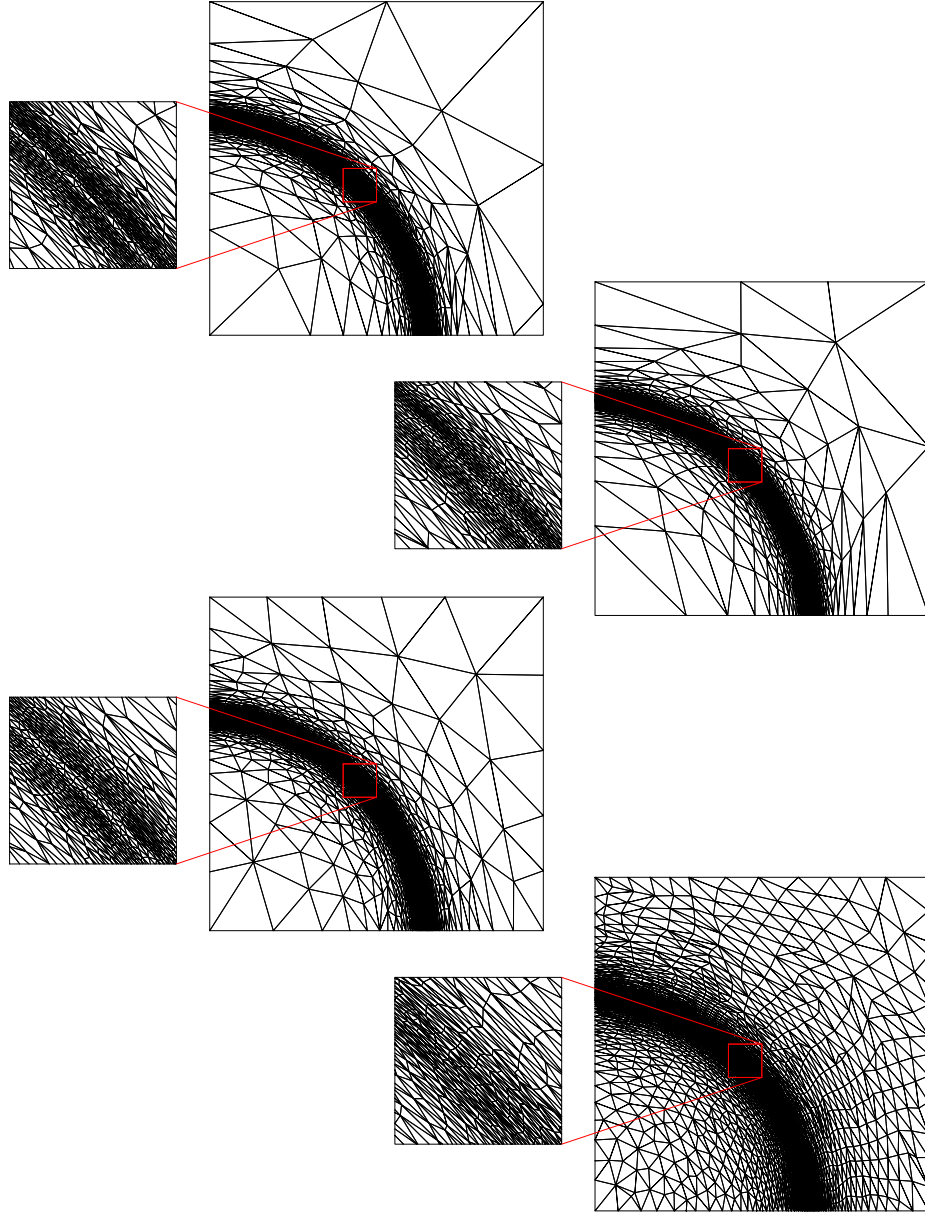
Figure 2.11: Adapted meshes for u_2 , \alpha = 100 with approximately 3000 vertices, with zoom to wave front. From top to bottom: residual (element), residual (metric), Hessian, hierarchical.
