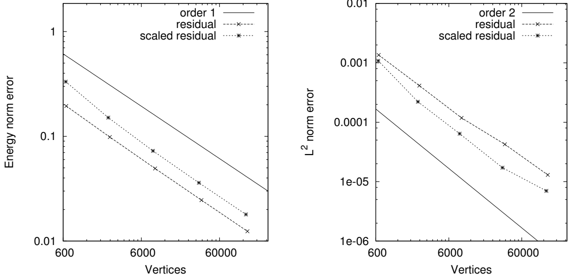
Figure 2.6: Energy norm (left) and L^2 norm (right) error calculations for u_1 for residual estimators.
