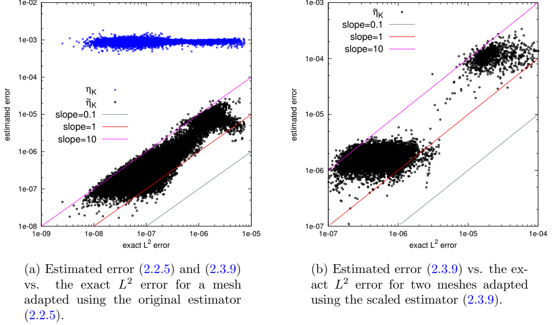
Figure 2.5: Estimated error vs. exact L^2 error over elements.
