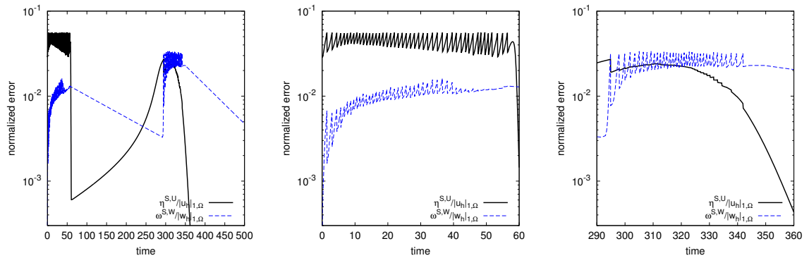
Figure 4.14: Test case 2: evolution of the space error for space-time adapted solution.
