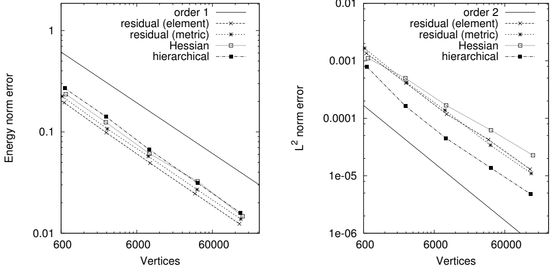
Figure 2.9: Energy norm (left) and L^2 norm (right) error calculations for u_1 .
