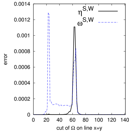
Figure 4.11: Test case 2: plot of the estimators for w on the line x = y at time t = 20 . Solution computed on a uniform mesh with 6400 elements and a constant time step 0.25.
