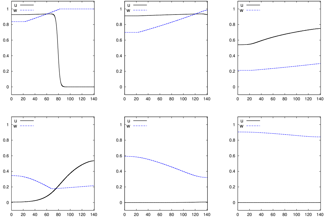
Figure 4.9: Test case 2: plot of u, w over the line x = y as a function of arc-length at different points in time. During the depolarization at t = 30 (top left), start of the plateau at t = 60 (top centre), start of the repolarization at t = 254 (top right), part way through the repolarization at t = 316 (bottom left), beginning of the recovery phase at t = 360 (bottom centre), and end of the simulation at t = 500 (bottom right).
