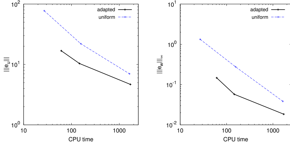
Figure 4.5: Test case 1: error vs. CPU time for uniform and adapted mesh computations.
