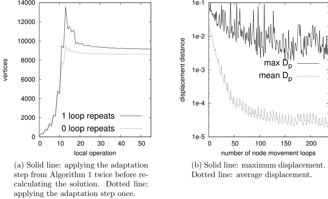
Figure 2.3: Left: Number of vertices after refinement/derefinement. Right: Maximum and average displacement of nodes for cumulative node movement loops.
