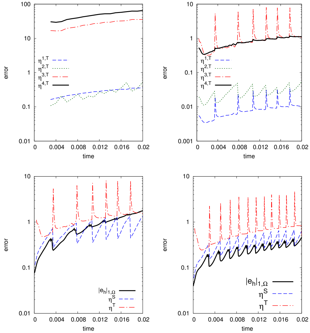
Figure 3.3: Test case 1. Top: evolution of time estimator applying mesh adaptation with TOL_S = 0.5 with constant time step \tau = 0.001 (left) and \tau = 0.000125 (right). Bottom: evolution of the estimators and exact error for TOL_S = 0.5 , \tau = 0.000125 (left) and TOL_S = 0.52 , \tau = 8.85625 \times 10^{-5} (right).
