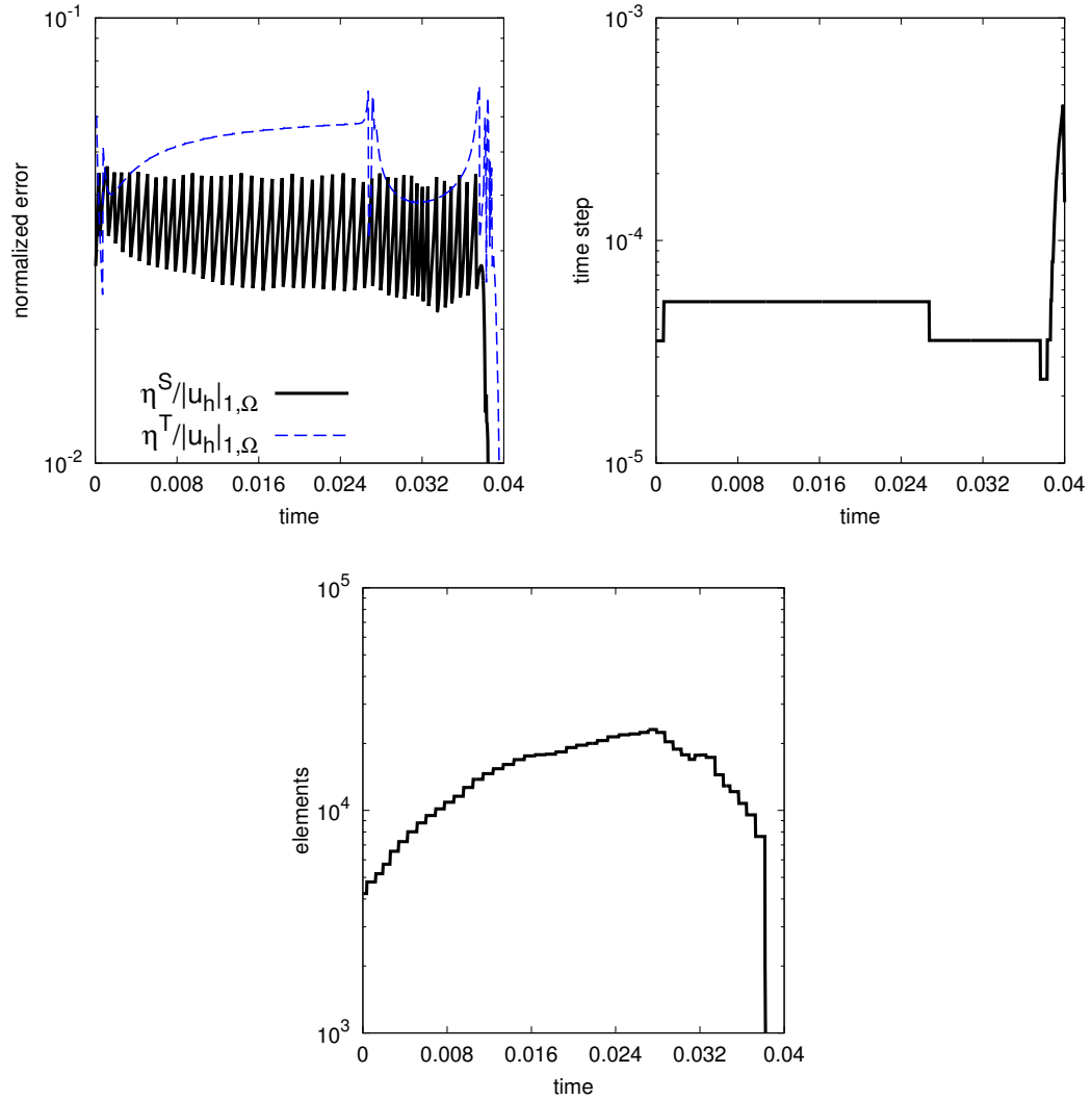
Figure 3.5: Test case 1: space-time adaptive algorithm with TOL_S = 0.125 , TOL_T = 0.09375 : the relative space and time error estimators (top left), the evolution of the time step (top right), and number of elements (bottom).
