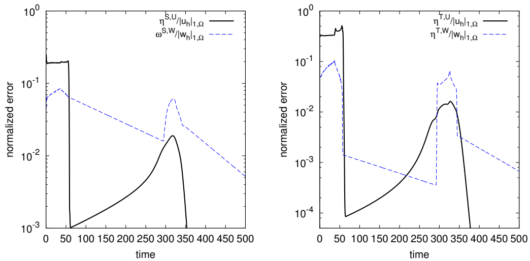
Figure 4.12: Test case 2: evolution of the normalized space error (left) and time error (right) computed on a uniform mesh with h = 2.5 and step \tau = 0.5 .
