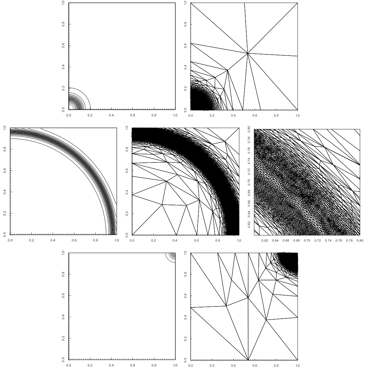
Figure 3.4: Examples of contours and adapted meshes with TOL_S = 0.125 , TOL_T = 0.09375 at t = 0.00141933 (top), t = 0.0265008 (center) with zoom to the wave-front (center right), and at t = 0.0382107 (bottom).
