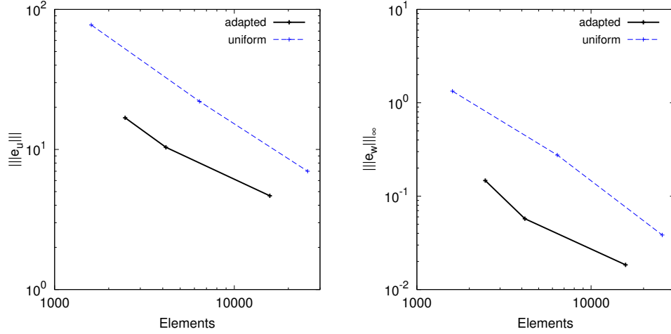
Figure 4.6: Test case 1: error vs. number of elements for uniform and adapted mesh computations.
