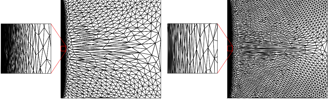
Figure 2.7: Adapted meshes with 2500 vertices using the H^1 estimator (left) and scaled estimator (right).
