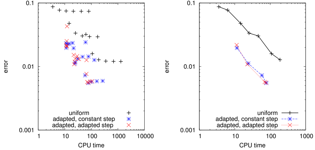
Figure 3.8: Test case 2: CPU time vs. error for all computations (left) and best points (right).
