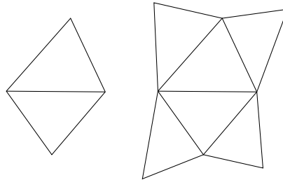
Figure 2.1: Extension of the edge patch for edge swapping.
