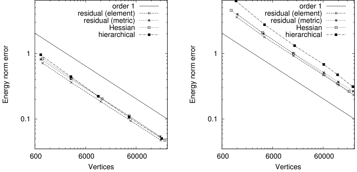
Figure 2.12: Energy norm error calculations for u_2 with \alpha = 100 (left) and \alpha = 1000 (right).
