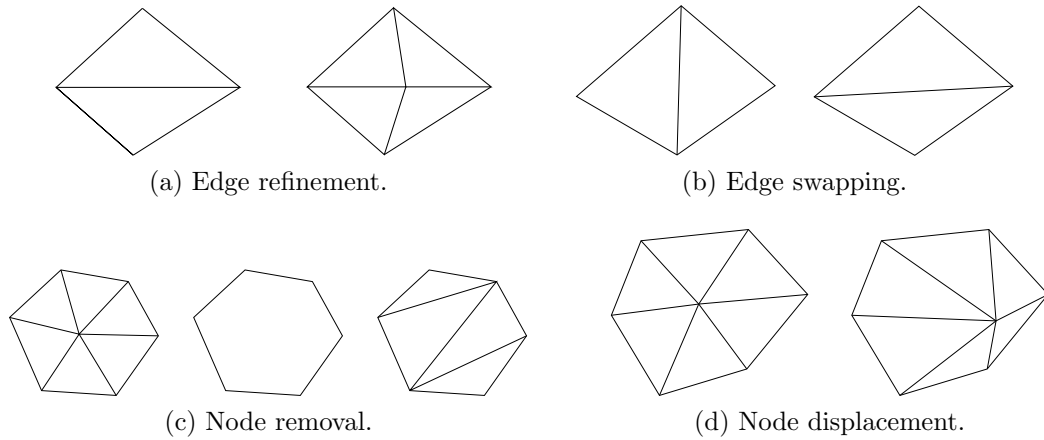
Figure 1.1: Local mesh operations.
