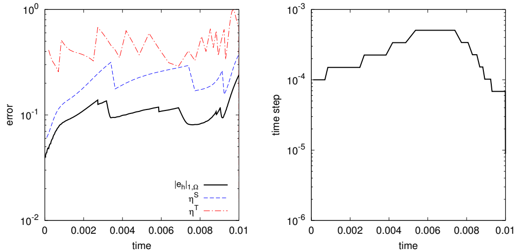
Figure 3.7: Test case 2: plot of the error (left) and time step (right) using space-time adaptation with TOL_S = 0.25 and TOL_T = 0.375 .
