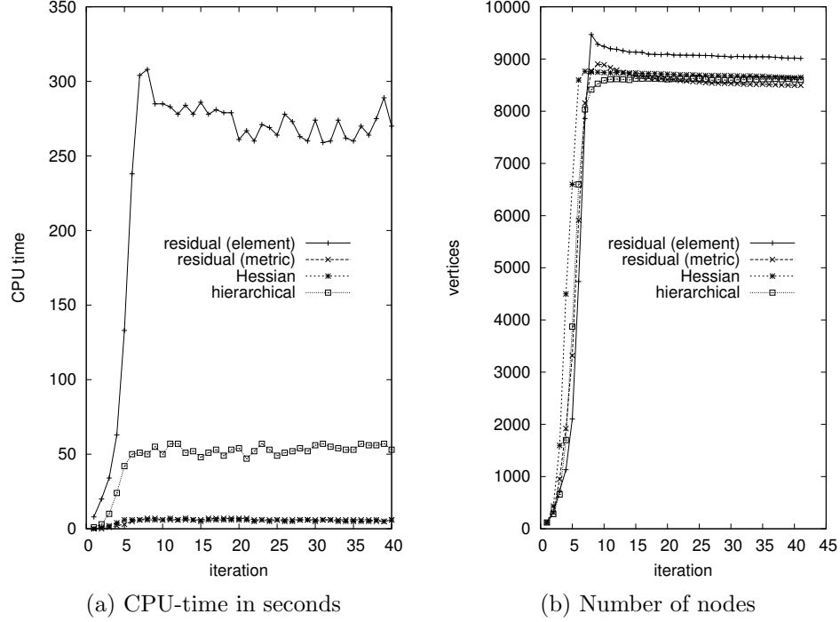
Figure 2.10: Left: CPU time for each iteration. Right: number of nodes at each iteration.
