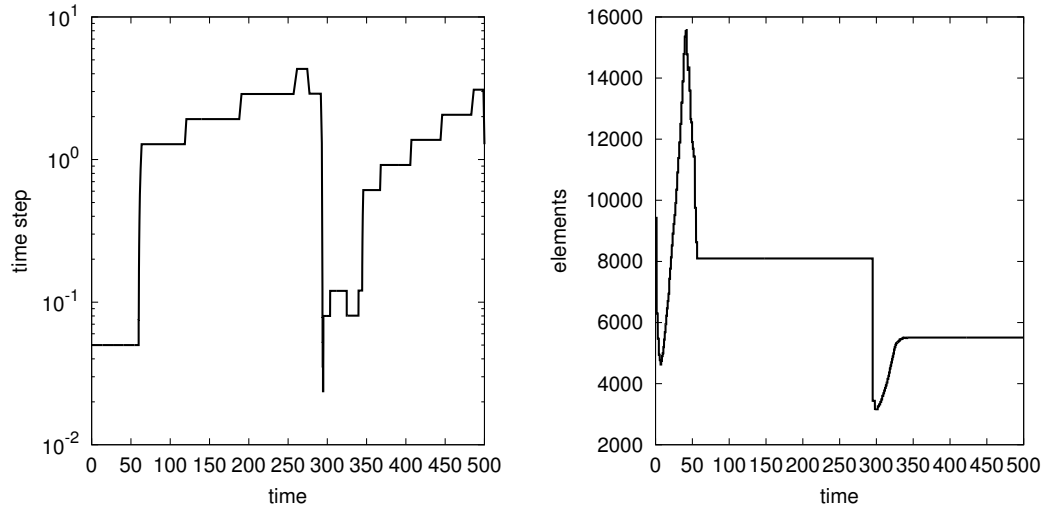
Figure 4.13: Test case 2: evolution of the time step (left) and the number of elements (right).
