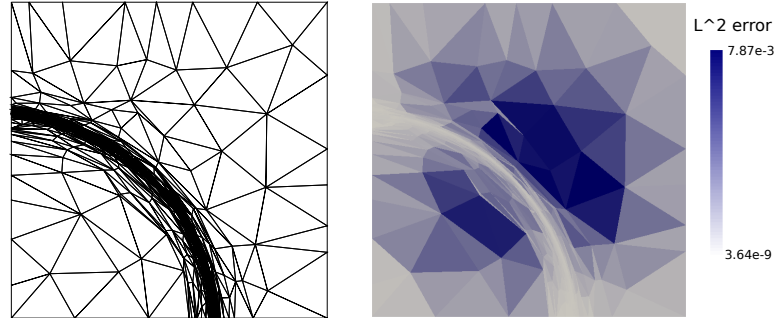
Figure 2.14: Mesh with about 1100 vertices adapted with the hierarchical method (left) and the distribution of the exact L^2 error (right).
