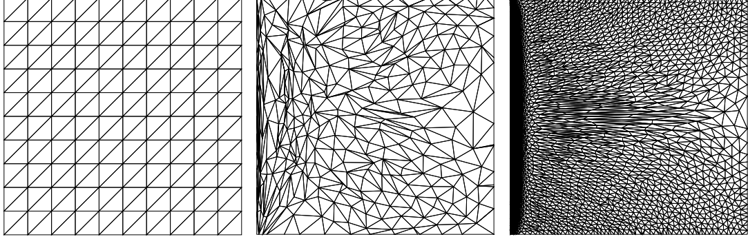
Figure 2.2: Left: initial uniform mesh with 121 vertices. Middle: first adapted mesh with 324 vertices. Right: final mesh with 8559 vertices.
