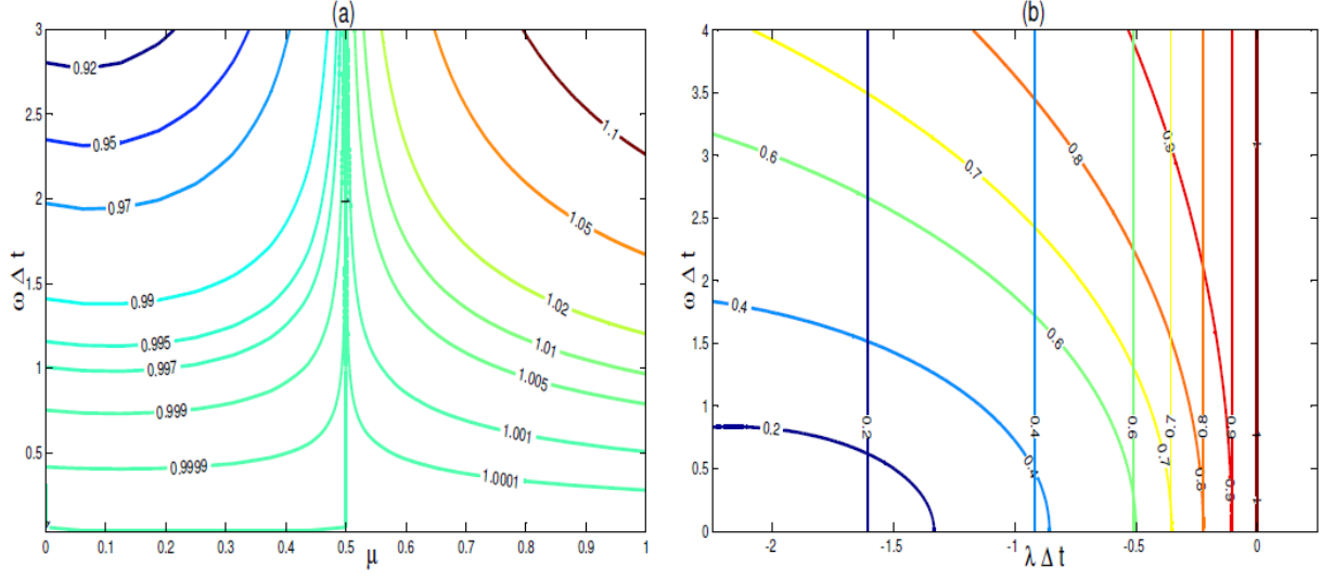
Figure 3.5 Treatment of the linear term. (a): Module of the amplification factor, for oscillation equation (3.9) using \theta = 0.5 , plotted as function of \mu and \omega\Delta t . (b): Module of the amplification factor for Equation (3.5) using \mu = 0.5 and \theta = 0.5 plotted on the \lambda\Delta t - \omega\Delta t plane.
