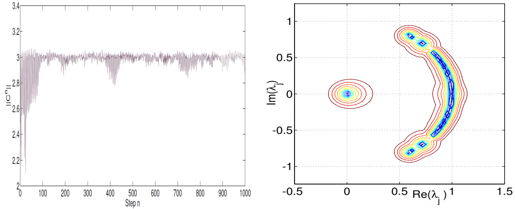
Figure 5.2 Left: Evolution of the parameter \|\mathbf{C}^n\| using method 1-CN (test a) with periodic boundary conditions in the x - and y -directions. Right: Eigenvalue spectrum and pseudospectra of the same method with the same boundary conditions
