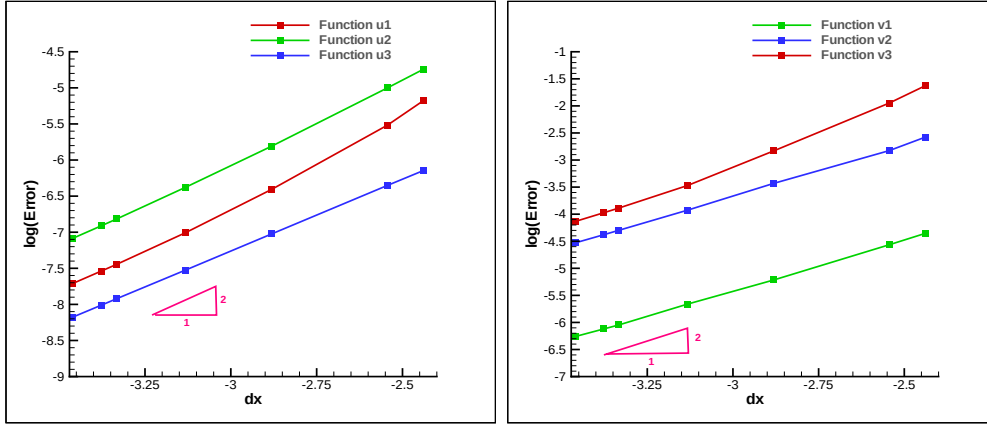
Figure 6.2 Evolution of L^1 -error in log-log scale until time T = 5 ( dx = \log(\Delta\lambda) ) for the nonlinear foliated flux defined on the basis of the scalar potential h(x, u) = (x \cdot \mathbf{a})f(u) . Left: For the nonlinear foliated flux defined by using \mathbf{a} = \mathbf{i}_1 . Right: For the nonlinear foliated flux defined by using \mathbf{a} = \mathbf{i}_1 + \mathbf{i}_2 + \mathbf{i}_3 .
