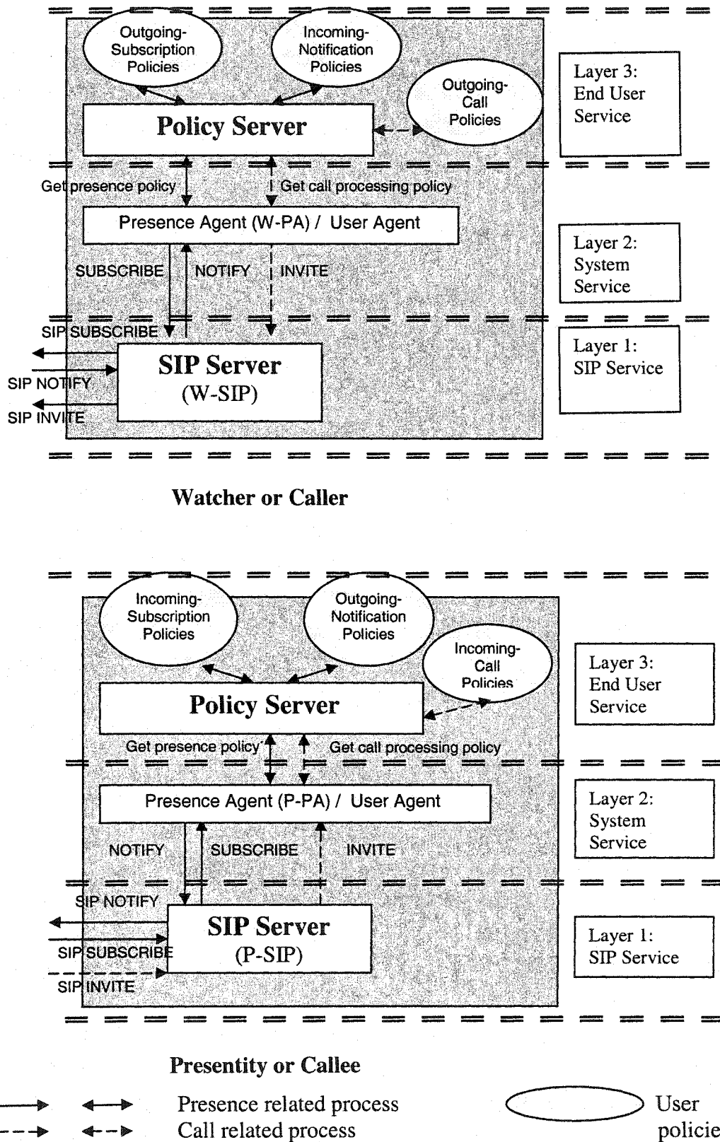
Figure 4.34 End User Policies in a three-layer Architecture
