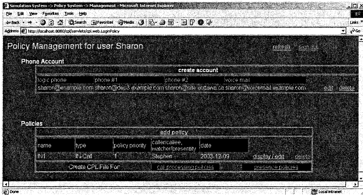
Figure 5.21 Policy Management Display
