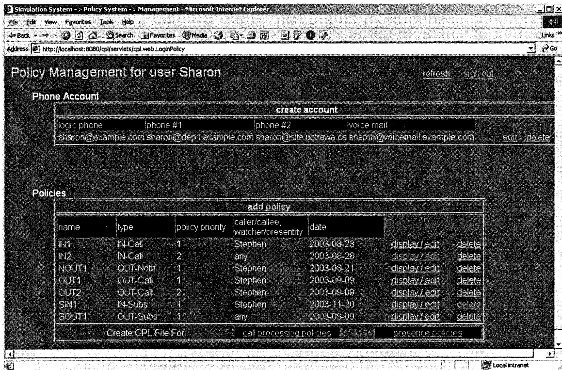
Figure 5.26 Policy Management Display (Sharon has created seven policies)
