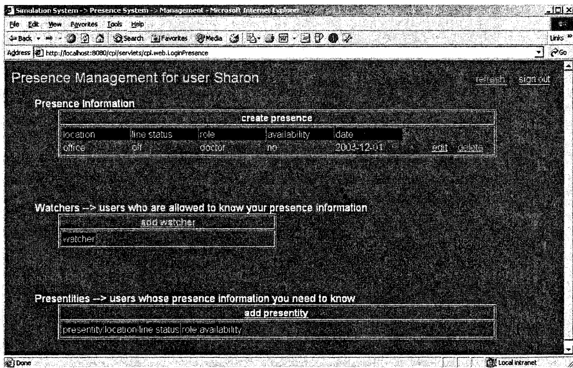
Figure 5.8 Presence Management Display
