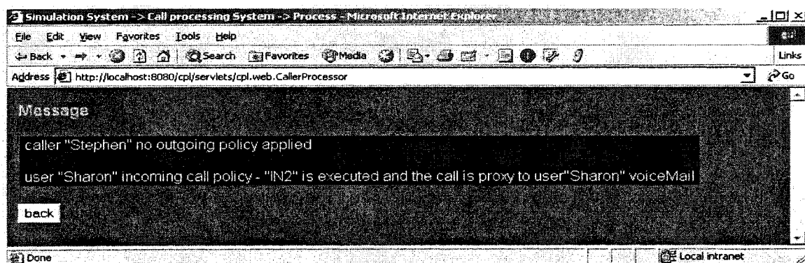
Figure 5.36 Message for “IN2” Test Result (Stephen’s call is forwarded to Sharon’s voice mail according to Sharon’s policy “IN2”)
