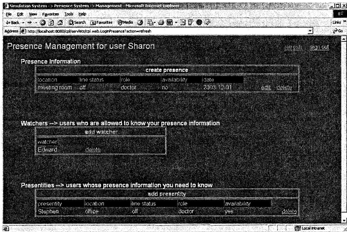
Figure 5.14 Presence Management Update
