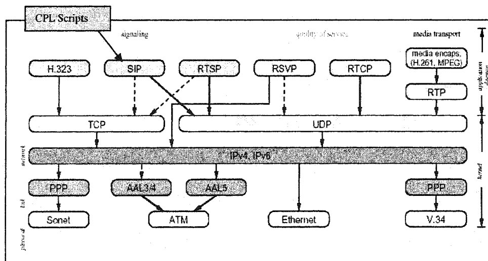
Figure 2.1 Internet Telephony Protocols
