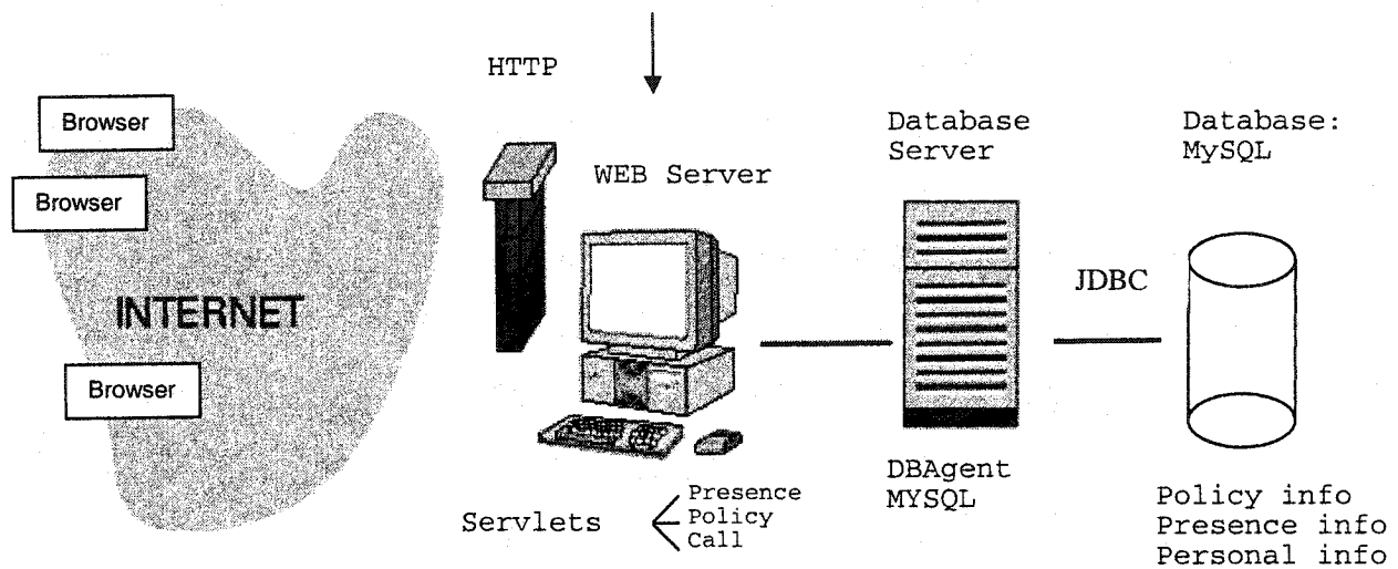
Figure 5.2 Architecture of Simulation System
