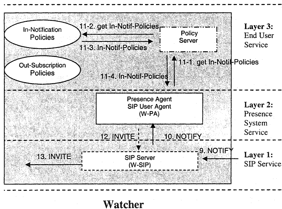
Figure 3.4 A Process on an Incoming-NOTIFY
