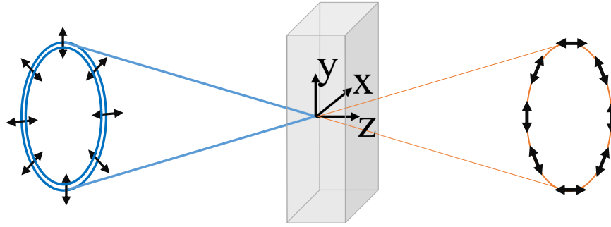
Fig. 8. Expected output for Type-I collinear downconversion with a conical pump beam centered on the optic axis (z). The signal and idler photons are produced in a single supercone centered on the optic axis.
