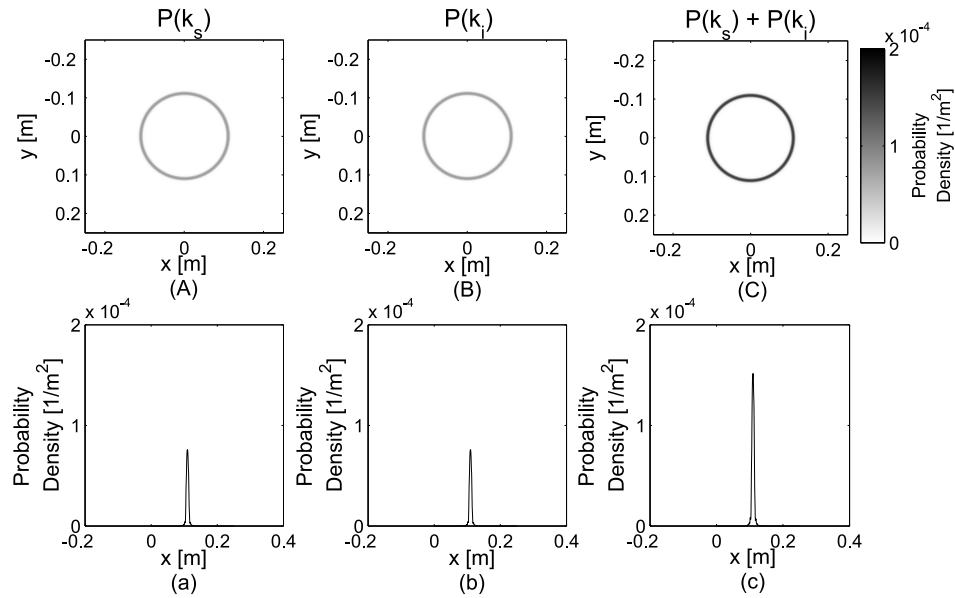
Fig. 7. Probability densities for Type-I degenerate downconversion in a 500\ \mu\text{m} -thick BBO crystal for a pump beam wavelength of 405 nm, and signal and idler wavelength of 810 nm. Since for degenerate phasematching |\mathbf{k}_{s(i)}| is fixed, \theta_{s(i)} and \phi_{s(i)} completely determine the signal and idler wavevectors. In turn, the position of the photons after the crystal determines these angles, so these plots are given in the crystal frame (x,y) at z=20\text{cm} after the crystal exit face. Plots (A), (B), and (C) give (A) the probability density for the signal photon, P(\mathbf{k}_s) ; (B) the probability density for the idler photon, P(\mathbf{k}_i) ; and (C) P(\mathbf{k}_s) + P(\mathbf{k}_i) , which is proportional to the photon flux. Plots (a), (b), and (c) are produced from plots (A), (B), (C), respectively, by plotting along y = 0 .
