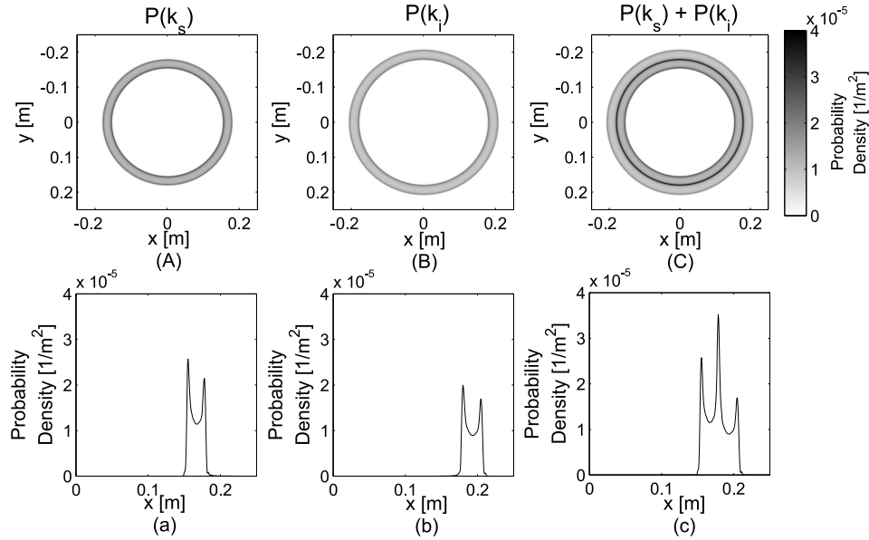
Fig. 2. Marginal probability density ( P(\mathbf{k}_s) , P(\mathbf{k}_i) ) for Type-II degenerate down-conversion. The pump cone half-angle is 41.8^\circ in a 500 \mu\text{m} -thick BBO crystal. The pump beam wavelength is 405 nm and the signal and idler wavelengths are 810 nm. Since for degenerate phasematching |\mathbf{k}_{s(i)}| is fixed, \theta_{s(i)} and \phi_{s(i)} completely determine the signal and idler wavevectors. In turn, the position of the photons after the crystal determines these angles, so these plots are given in the crystal frame ( x, y ) at z=20\text{cm} after the crystal exit face. Plots (A), (B), and (C) give (A) the probability density of generating a signal photon at \mathbf{k}_s , (B) the probability density of generating an idler photon at \mathbf{k}_i , and (C) P(\mathbf{k}_s) + P(\mathbf{k}_i) , which is proportional to the photon flux. Plots (a), (b), and (c) are produced from plots (A), (B), and (C), respectively, by plotting along y = 0 .
