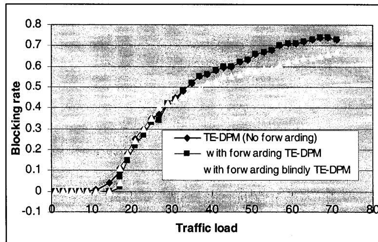
Figure 37: Blocking rate (simple network one).
