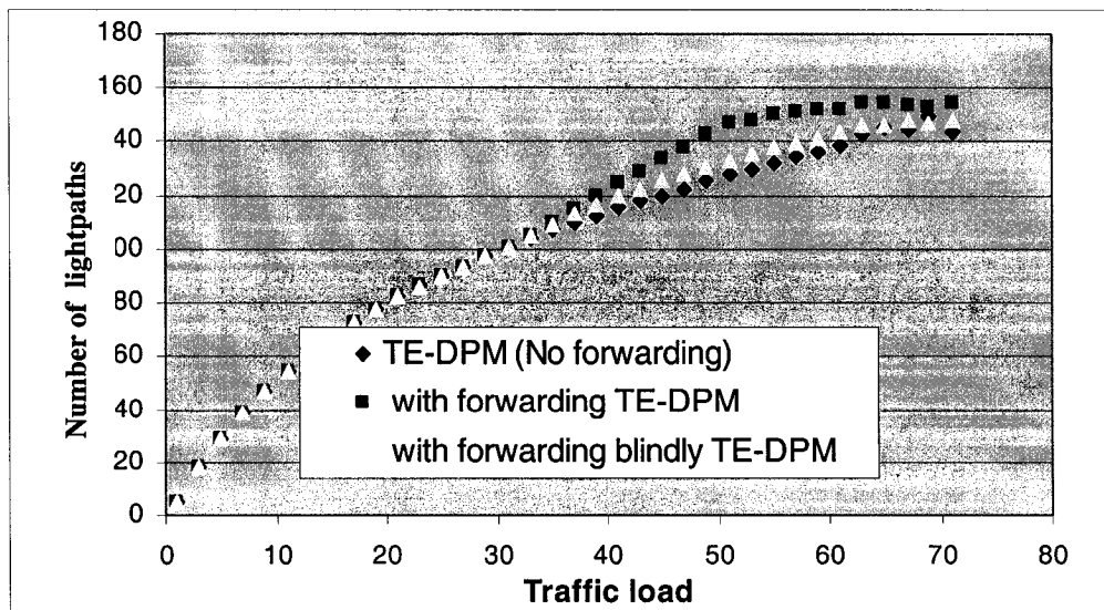
Figure 27: Average number of lightpaths established (NSFNET network).
