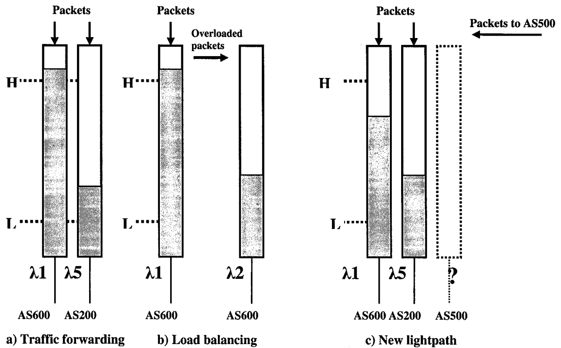
Figure 20: Buffers for AS100.
