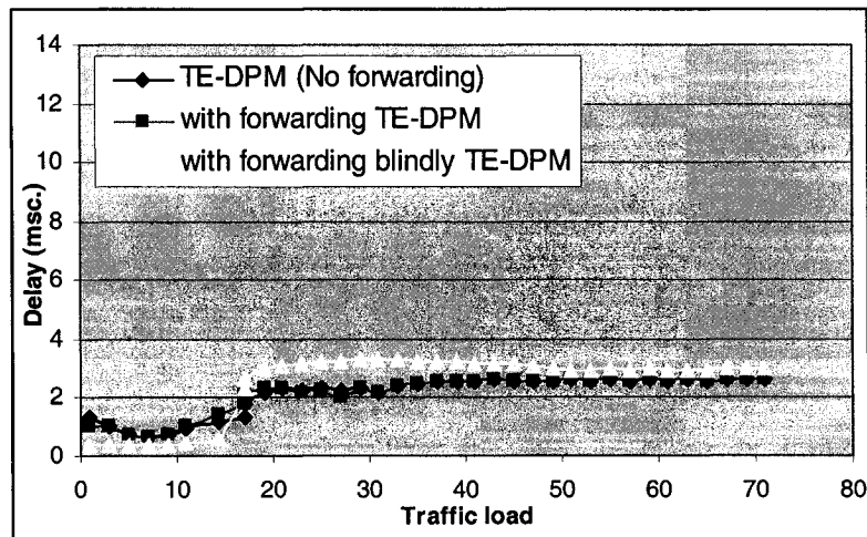
Figure 40: Average delay (simple network one).
