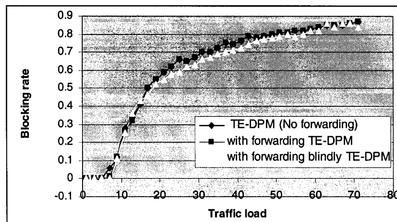
Figure 38: Blocking rate (simple network two).
