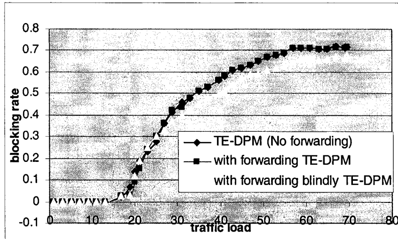
Figure 39: Blocking rate (star network).
