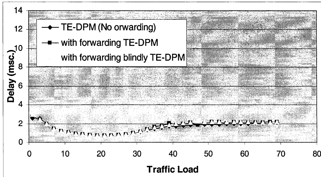
Figure 29: Average delay (NSFNET network).
