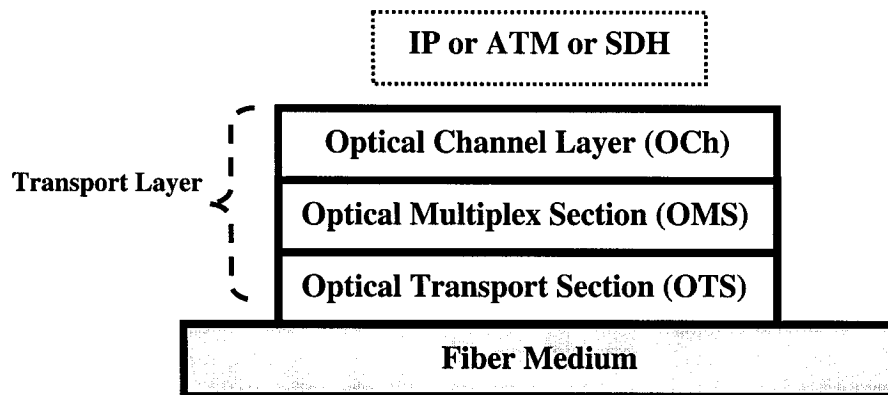
Figure 1: Optical network layered architecture.
