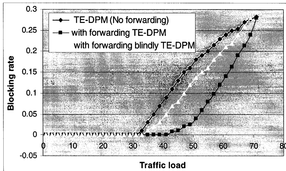
Figure 28: Blocking rate (NSFNET network).
