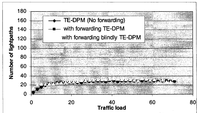
Figure 35: Average number of lightpaths established (simple network two).
