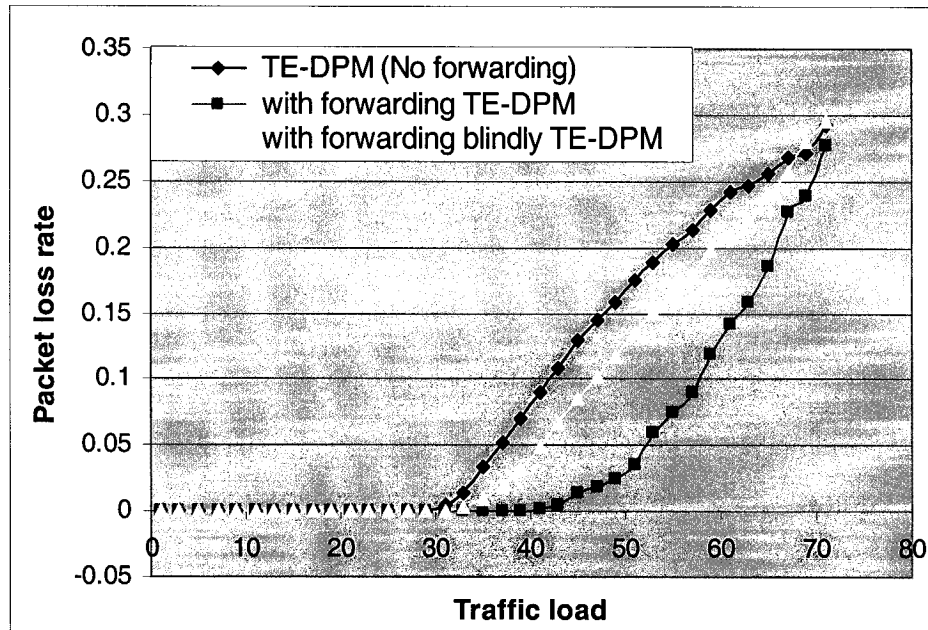
Figure 26: Packet loss rate (NSFNET network).
