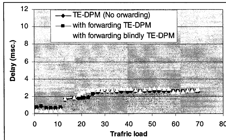
Figure 42: Average delay (Star network).
