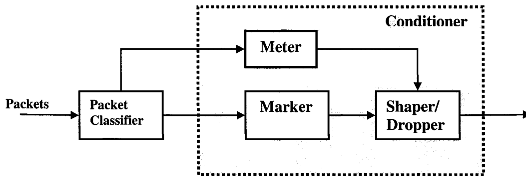
Figure 9: Packet classifier and traffic conditioner.
