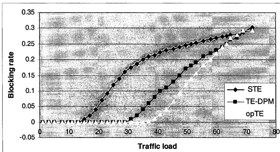
Figure 24: Blocking rate with different TE techniques and not traffic forwarding (NSFNET network).
