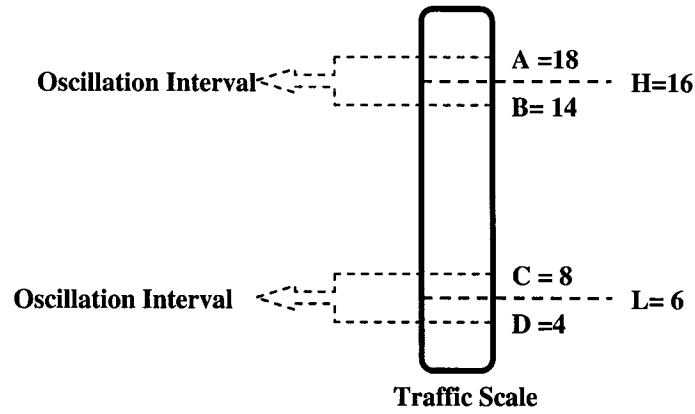
Figure 43: Oscillation interval example.
