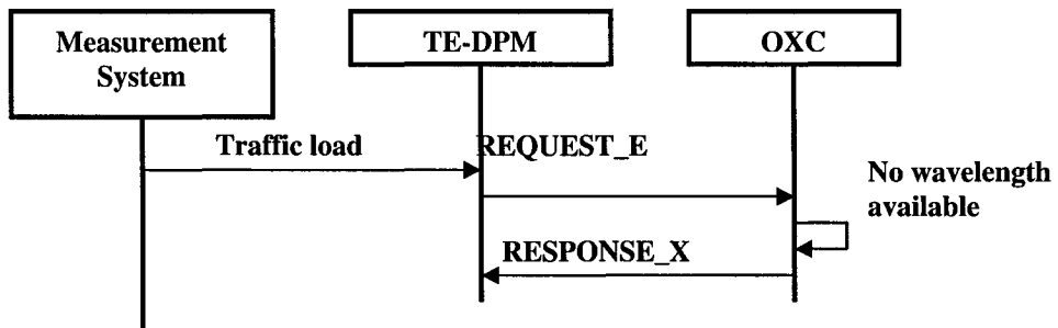
b) TE-DPM and OXC interaction.
