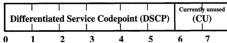
Figure 8: DiffServ field in the 8-bit ToS.
