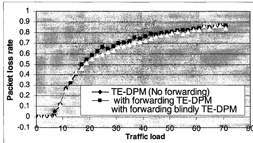
Figure 31: Packet loss rate (simple network one).
