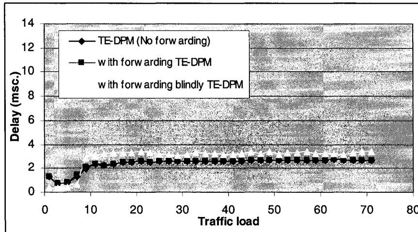
Figure 41: Average delay (Simple network two).
