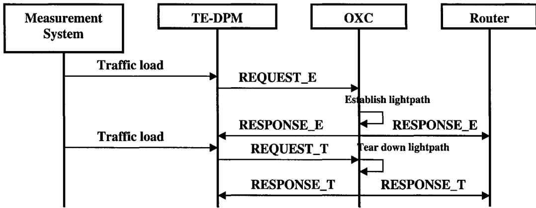
a) TE-DPM and OXC Interaction.
