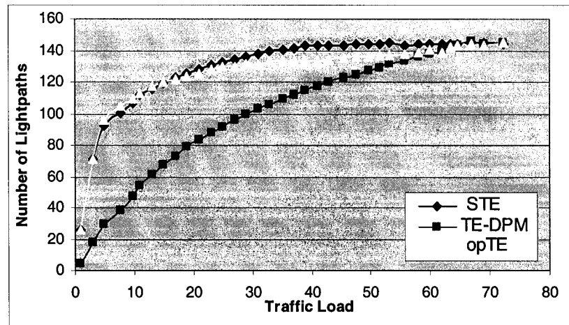
Figure 23: Average lightpaths established with different TE techniques and no traffic forwarding (NSFNET network).
