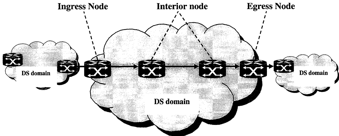
Figure 7: Differentiated service domain.
