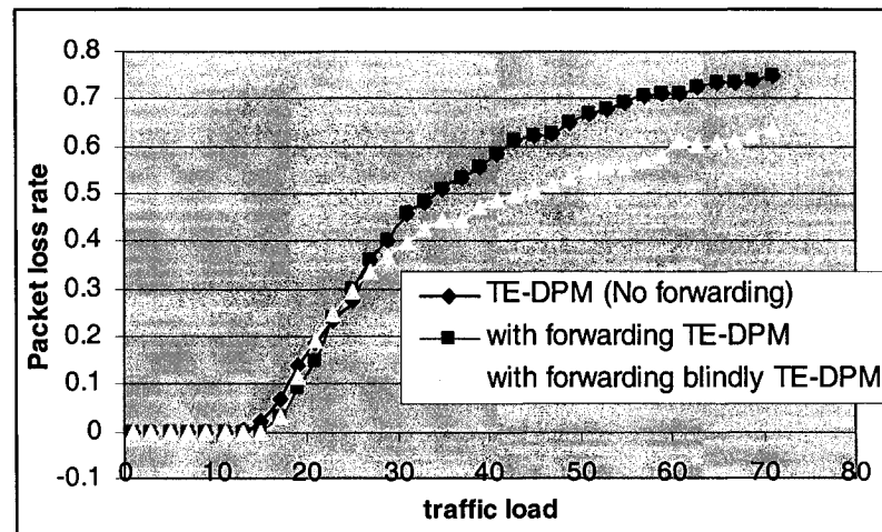
Figure 32: Packet loss rate (simple network two).
