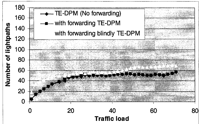
Figure 34: Average number of lightpaths established (simple network one).
