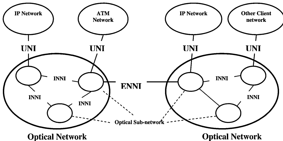
Figure 2: Optical network logical control structure.
