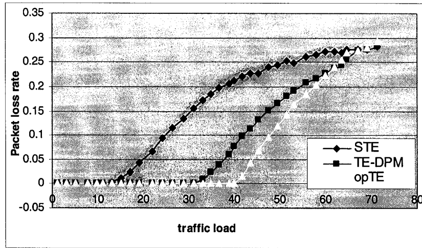
Figure 22: Fraction of packets lost with different TE techniques and no traffic forwarding (NSFNET network).
