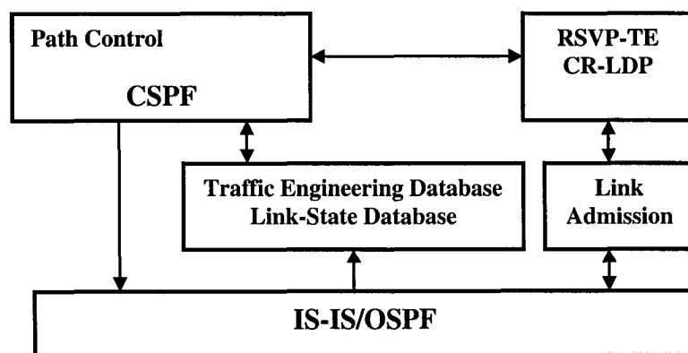
Figure 11: MPLS-TE functional components.
