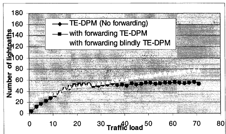
Figure 36: Average number of lightpaths established (star network).
