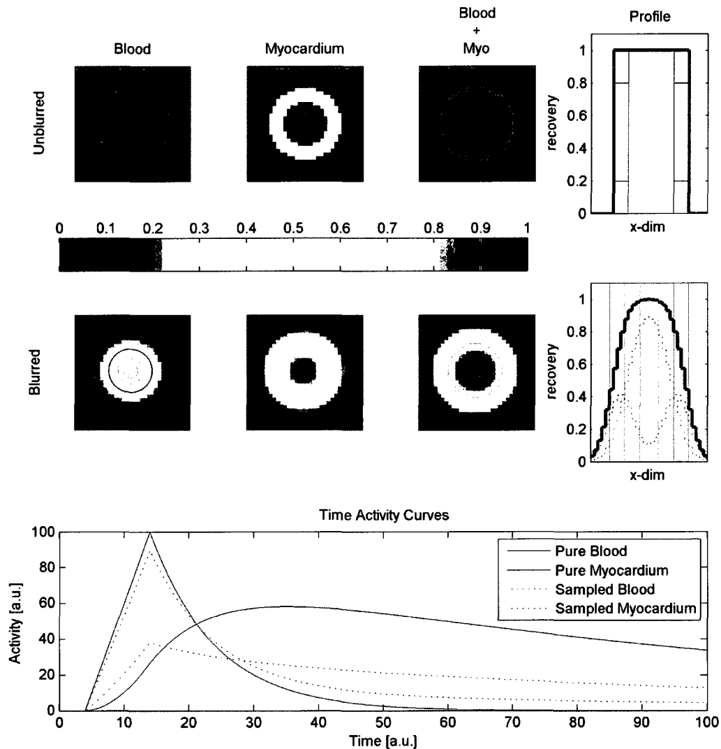
Figure 2-11 – Blurring effects on signal mixing and recovery losses. Pure blood and myocardium contributions are shown in the top row along with their sum and a profile along a line in the center of the image. After blurring the recovery in the myocardium is much reduced, as well as a slight reduction in the blood recovery. Pure TACs and sampled TACs (ROIs shown in blurred blood image) are compared in the bottom figure.
