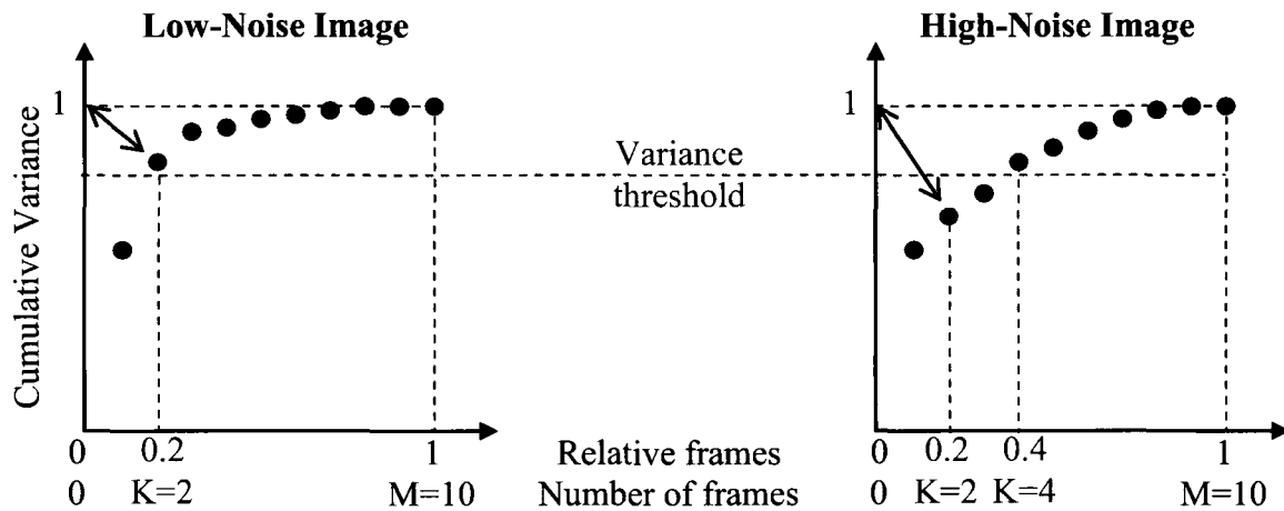
Figure 4-1 – Demonstration of two alternative methods for resolving number of factors, K , base on the cumulative variance in the image.
