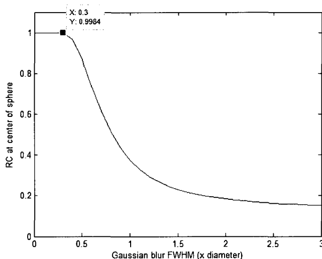
Figure 6-14 – Recovery coefficient at the center of a sphere with uniform activity with varying isotropic Gaussian blur. When the blur \text{FWHM} < \text{diameter}/3 nearly perfect RC is present at the center of the sphere.
