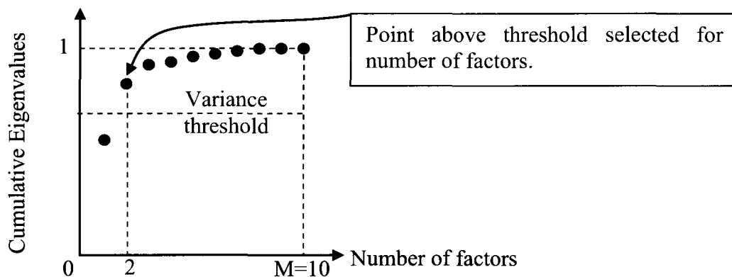
Figure 2-13 – Demonstration of a method for resolving number of factors, K , based on the cumulative Eigenvalues of the image covariance matrix, which corresponds to the image variance.
