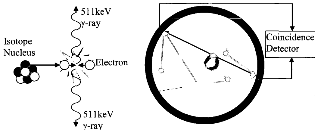
Figure 2-2 – Positron emission tomography. The positron discharge followed by annihilation with an electron producing two collinear photons ( \gamma -rays) on the left. The projected line of response based on a detection of coincident events by the scanner is shown on the right. The image is a cross-section of the chest with red depicting tracer uptake in the heart muscle. A transmission image is fused in gray, showing the lungs and arms for anatomical reference.
