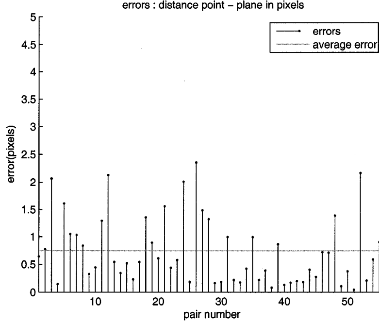
Figure 3.8: Distance point to plane for all matches
