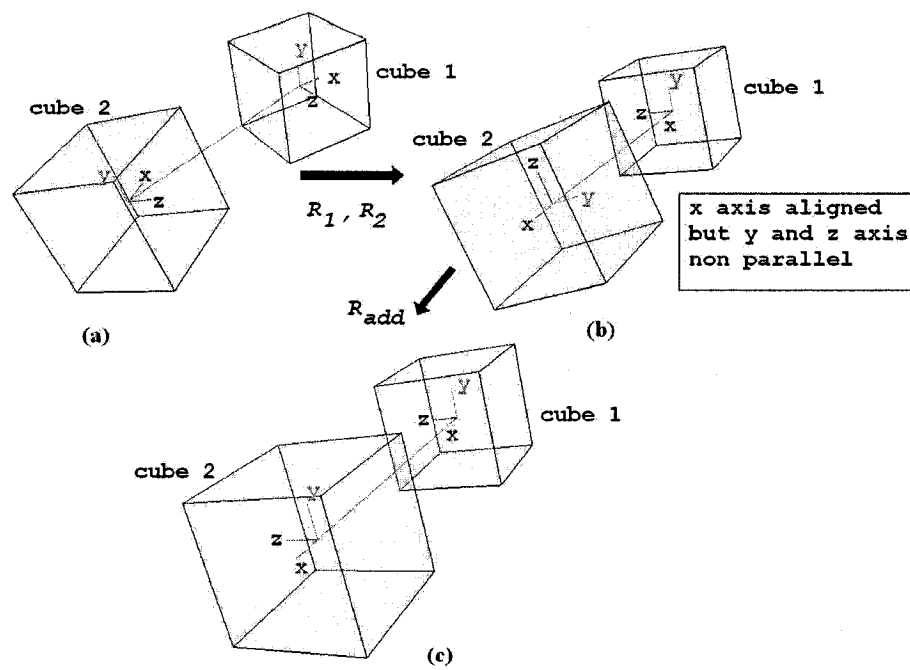
Figure 3.10: Rectification process with compensating rotation
