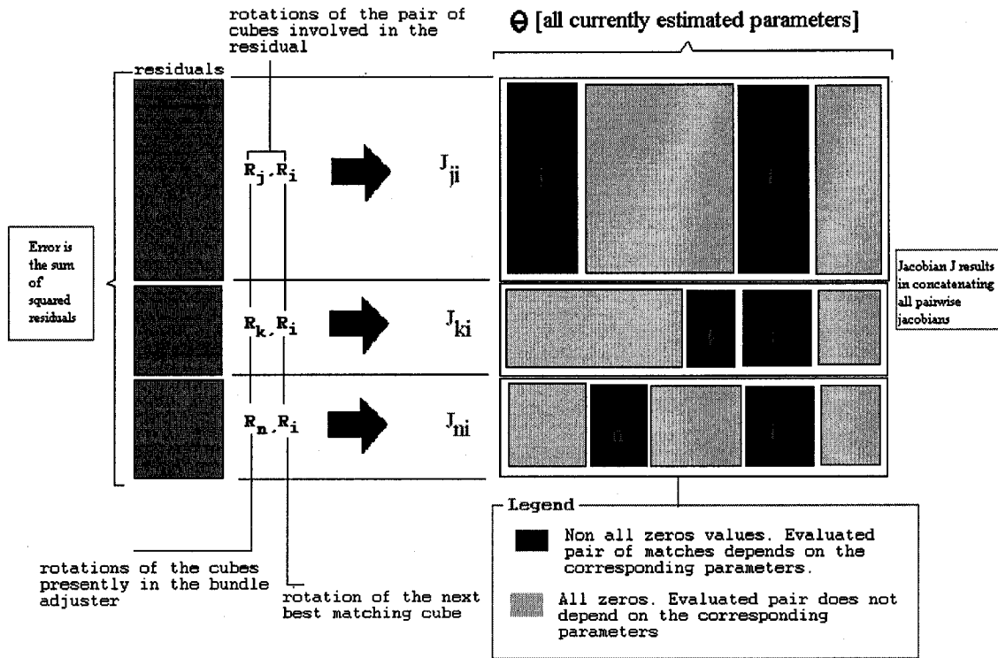
Figure 4.5: Concatenation principle in the residuals and Jacobians evaluation. Example with the bundle adjustment algorithm with four cubes, the fourth cube of index i being added to the adjuster that already contains cubes j , k and n .
