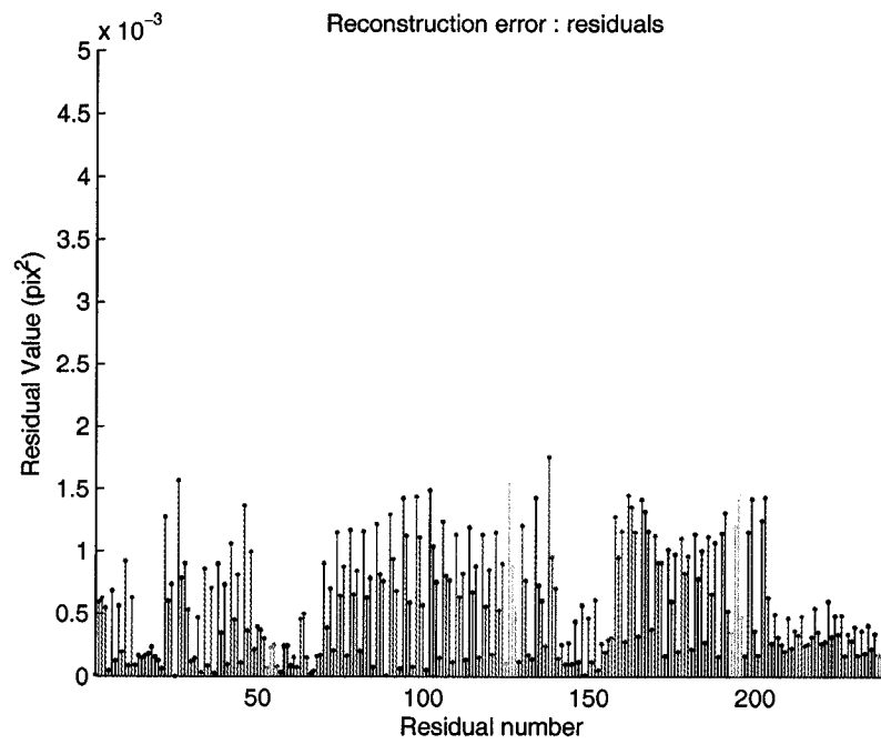
Figure 4.17: Residuals at the last iteration of the second stage for the indoor set: residuals r_{ij} , i \in \{1, \dots, \approx 25\} for the matches and j \in \{1, \dots, 4\} for the panoramas.
