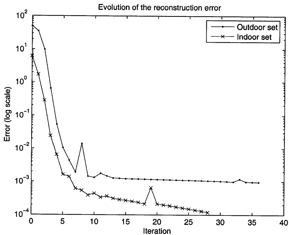
Figure 4.21: Evolution of the reconstruction error for both sequences during the bundle adjustment of stage 2.
