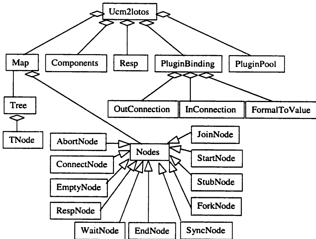
Figure 38 Class Diagram for Ucm2LotosSpec and Ucm2LotosScenarios
