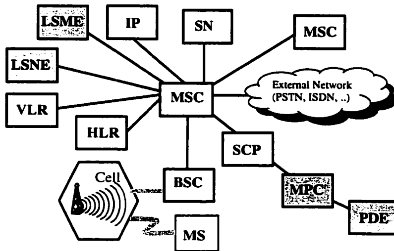
Figure 1 WIN Network Reference Model
