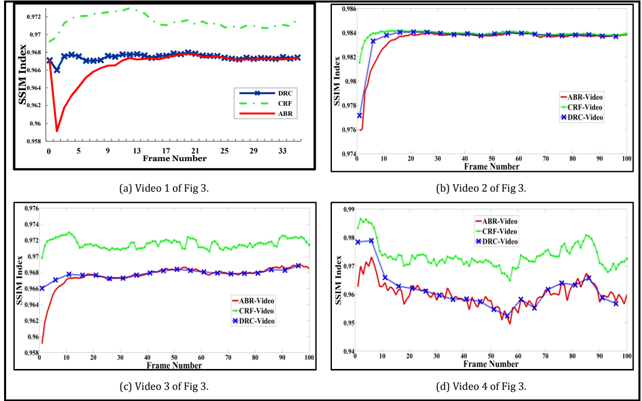
Figure 16: SSIM values (without I-frame).
