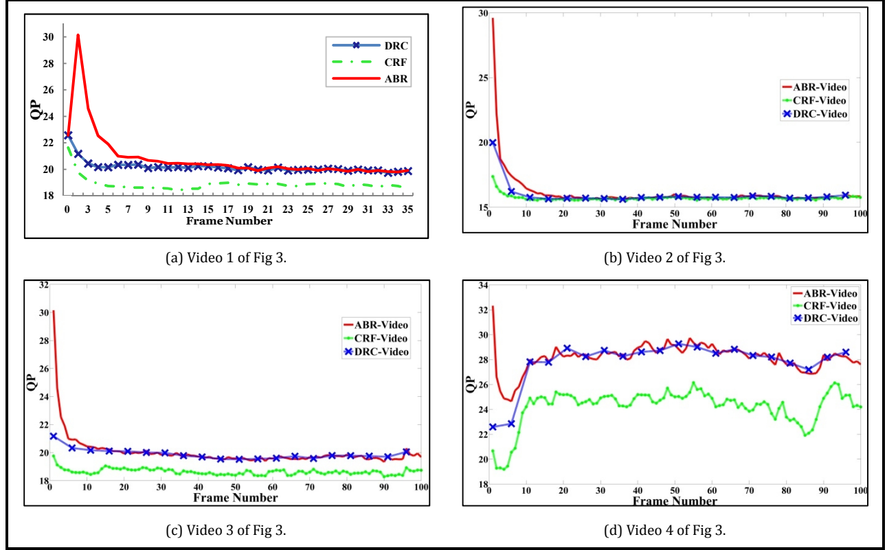
Figure 13: QP values.
