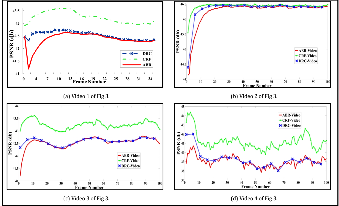
Figure 15: PSNR values (without I-frame).
