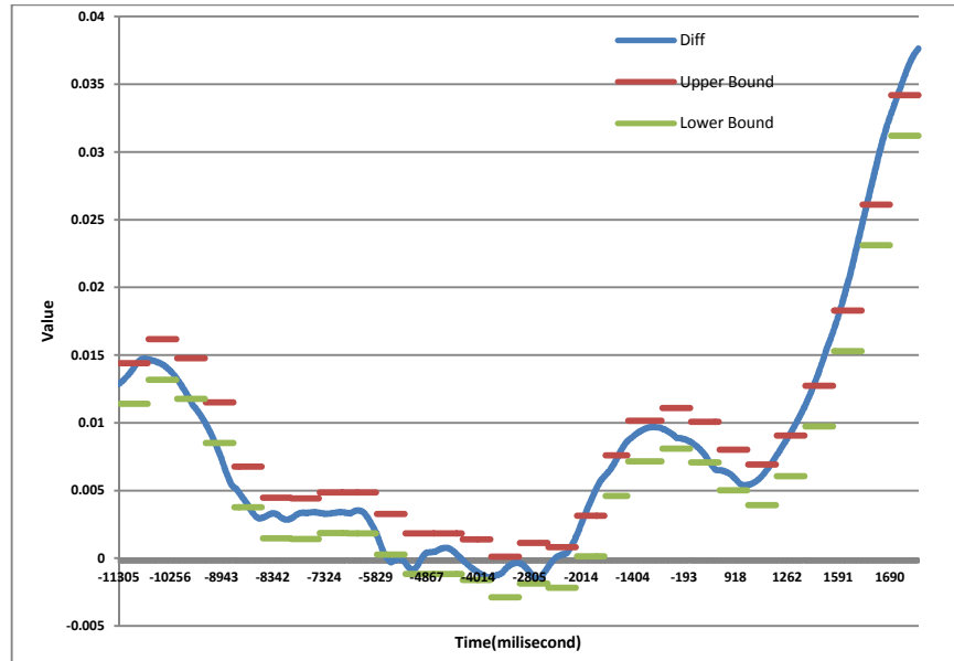
Figure 35: The performance of the proposed method when the bandwidth changes from 1500 Kbps to 2000 Kbps.
