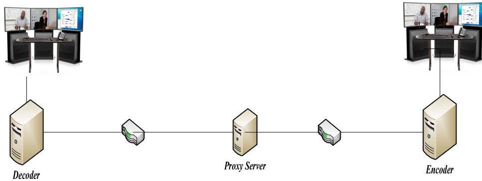
Figure 12: Simulation architecture.
