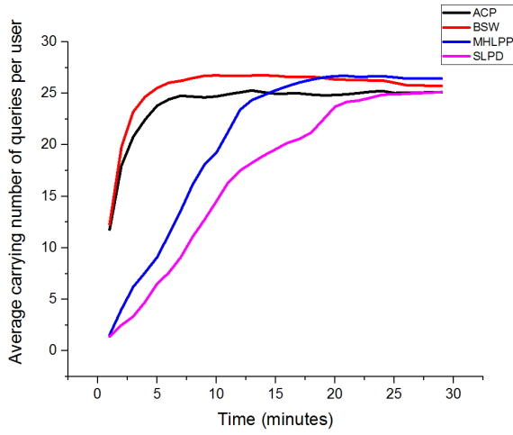
(c) communication range is equal to 90 meters
