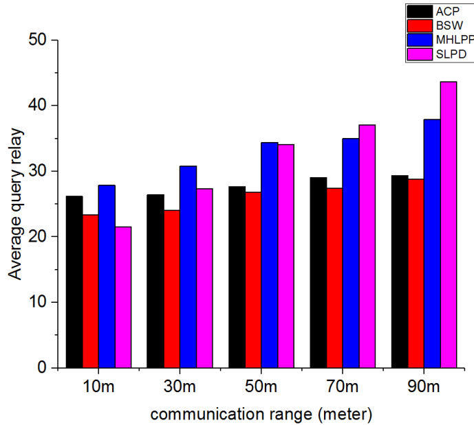
Figure 4.18: Average Number of Forwarding Queries At 20 Minutes Mark
