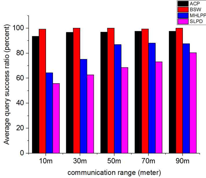
Figure 4.15: Average Query Success Ratio (at 20 minutes mark)
