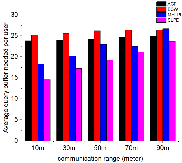
Figure 4.19: Average Number of Query Buffer Needed at 20 Minutes Mark
