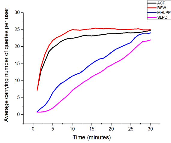
(a) communication range is equal to 10 meters
