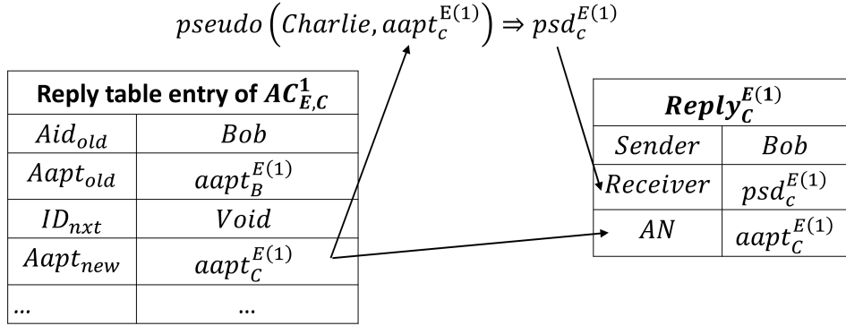
Figure 4.13: Charlie Forwards A Reply
