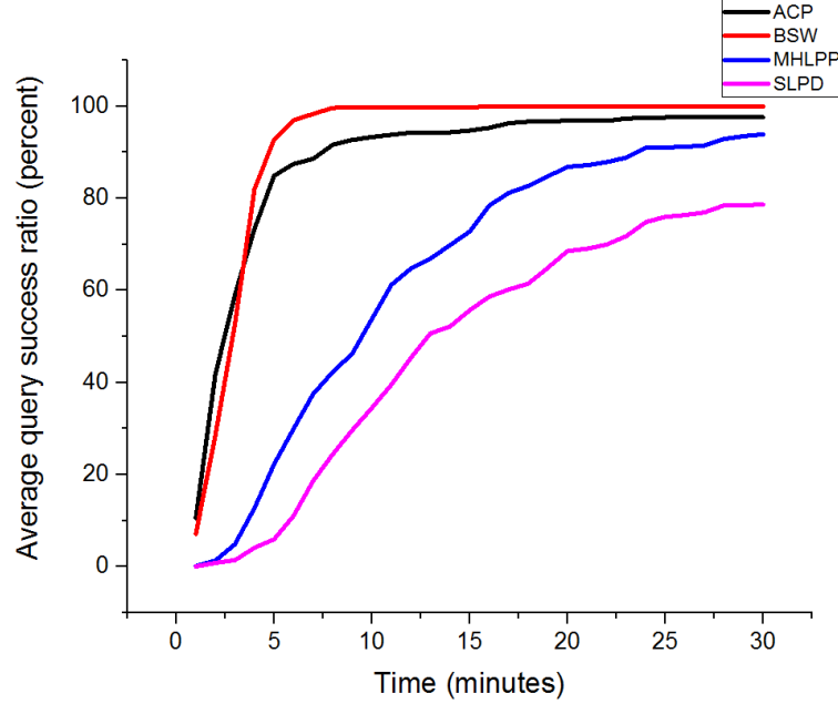
Figure 4.16: Average Query Success Ratio for 50-Meters Communication Range
