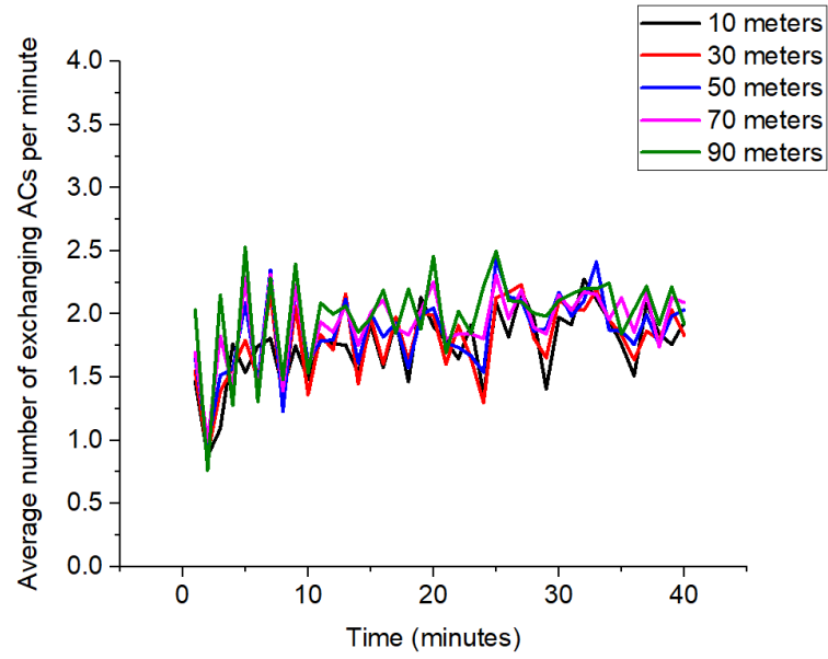
Figure 4.21: Average Number of Exchanging ACs Per Minute Under Different Communication Ranges
