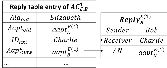
Figure 4.12: Bob Forwards A Reply
