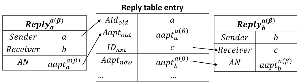
Figure 4.8: The Reply of The Second Agent
