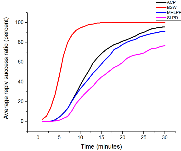
Figure 4.17: Average Reply Success Ratio for 50-Meters Communication Range
