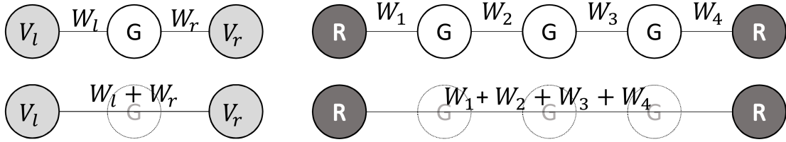
Figure 5.3: Remove Ignorable Vertices
