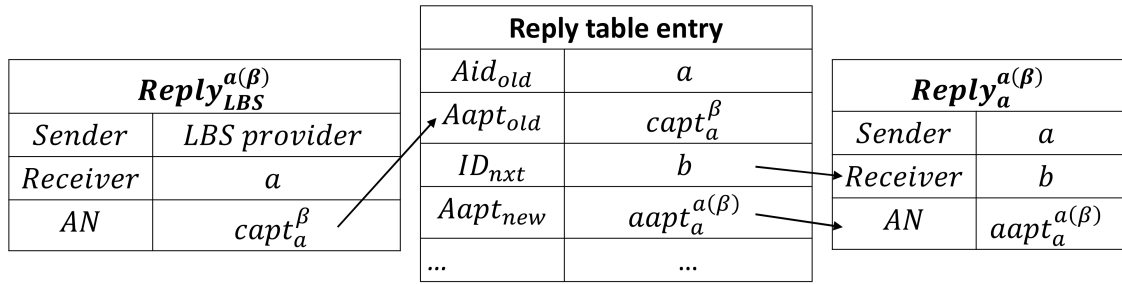
Figure 4.7: The Reply of The First Agent
