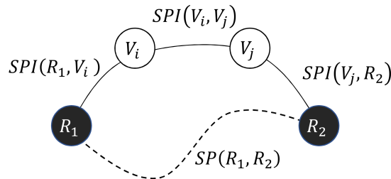
Figure 5.2: Shortest Path On A Single Segment-Line
