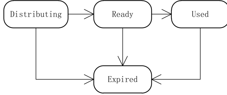
Figure 4.2: AC's Life Cycle
