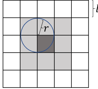
Figure 5.5: Grid Size For Still Nodes
