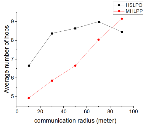
(b) Number Of Hops With Various Communication Radii
