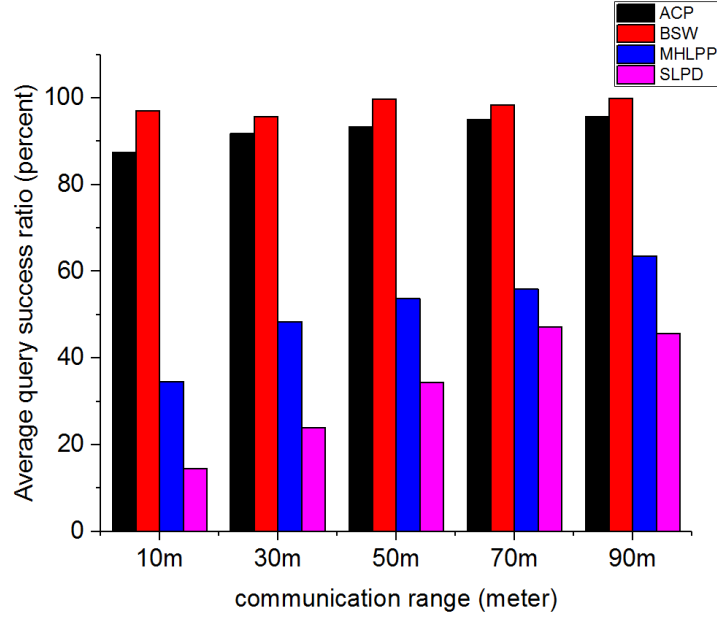
Figure 4.14: Average Query Success Ratio (at 10 minutes mark)
