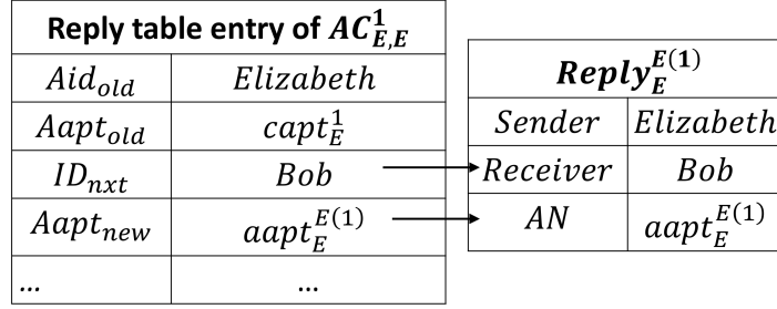
Figure 4.11: Elizabeth Forwards A Reply
