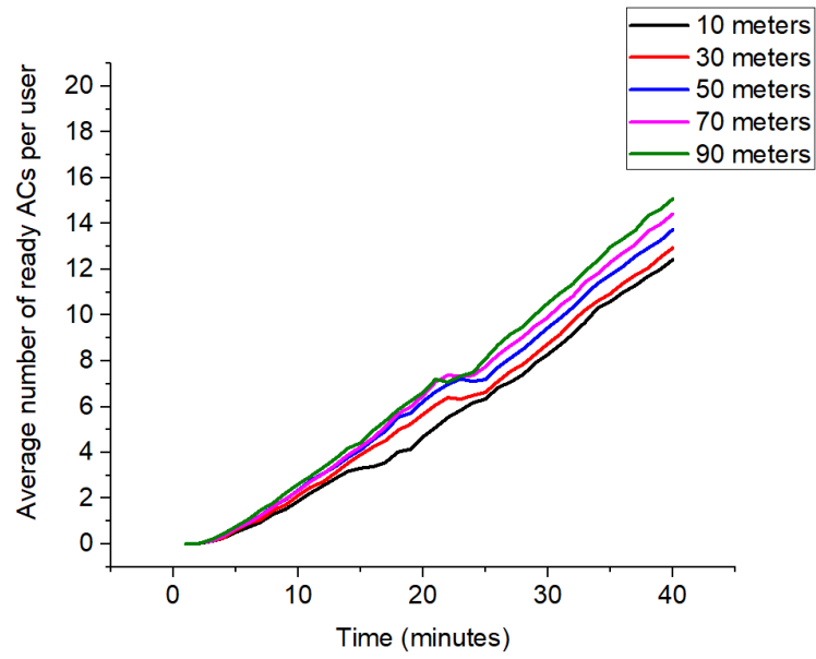
Figure 4.22: Average Number of Ready ACs Per User
