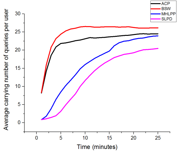
(b) communication range is equal to 50 meters
