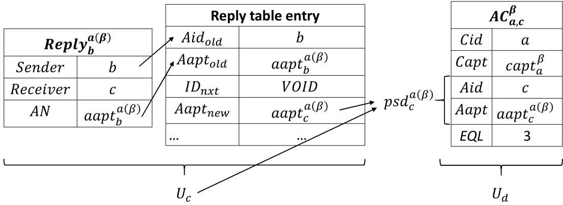
Figure 4.9: The Reply of the Last Agent
