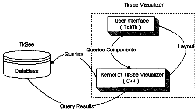
Figure 5-1: TkSee Visualizer
