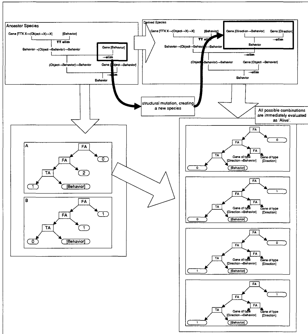
Figure 6.11: In this crossover scenario, a new species is created from the species to which both parent belong. The gene slots that match in the offspring species and in the parent species are filled as in the first case. The gene slots that do not match are filled from random choices in the gene pool
