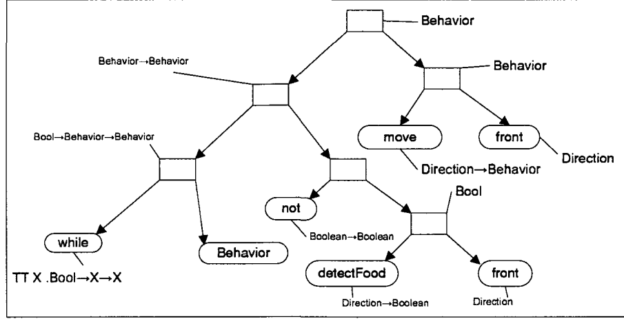
Figure 4.10: Polymorphically-typed looping construct
