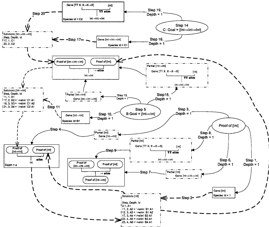
Figure 6.5: A trace of the modifyProof (code 6.5.4) function when initial argument is [Int]
