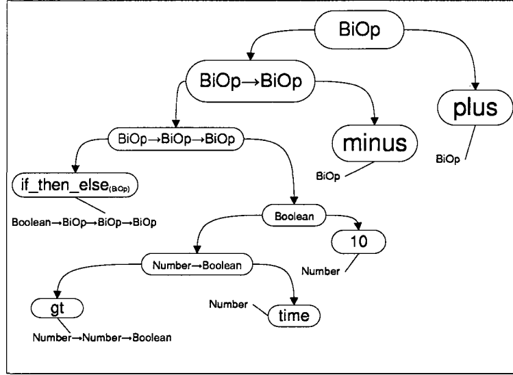
Figure 4.2: The illegal genotype of figure 4.1 can now be legally expressed using types. Note that [BiOp] is a name for the type [Number \rightarrow Number \rightarrow Number]
