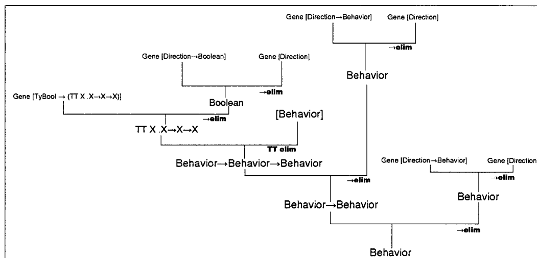
Figure 6.2: A species constructed on a gene pool generated from the primitives defined in table 6.2.2 with GoalType [ Behavior ]
