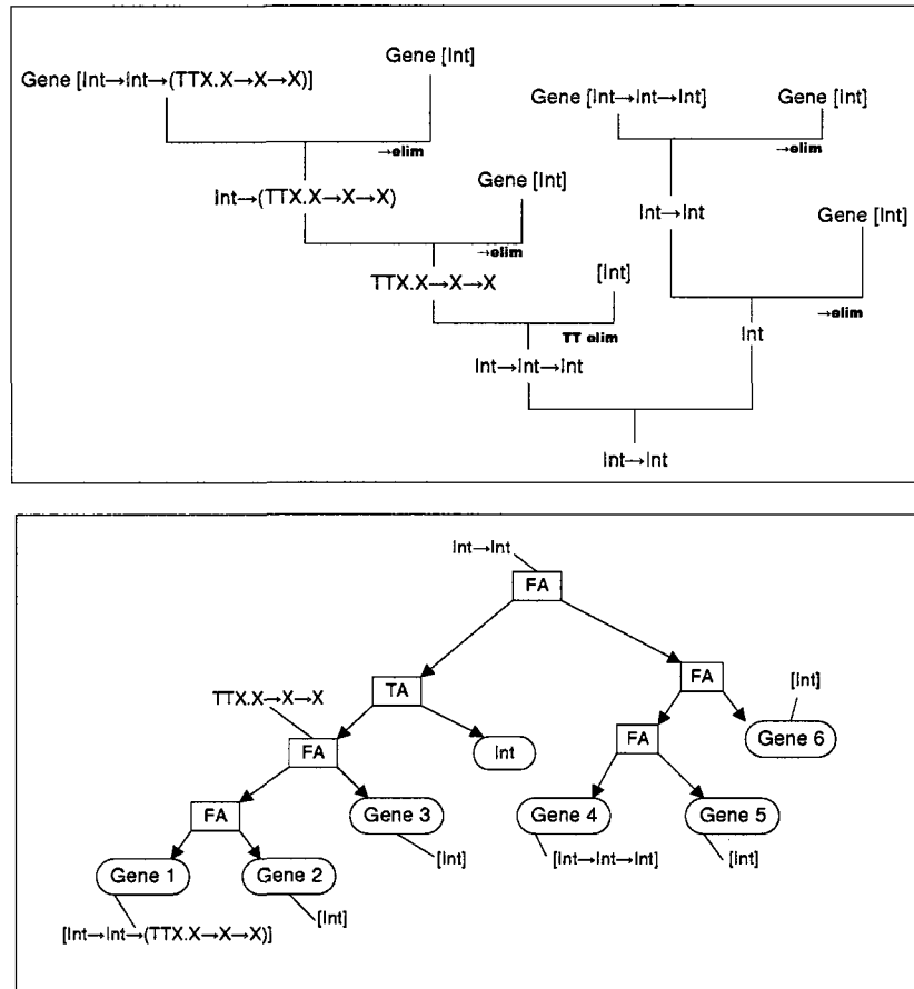
Figure 6.3: A species (above) and the genotype pattern that it produces (below)
