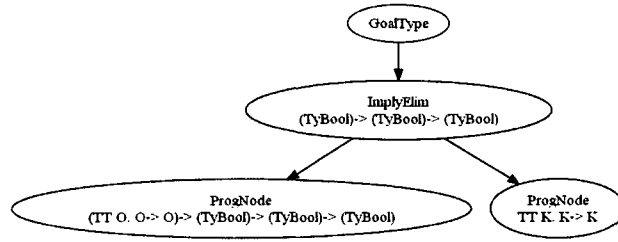
Figure 7.3: Species to which the example program ( or function) that normalizes to 7.3 belongs
