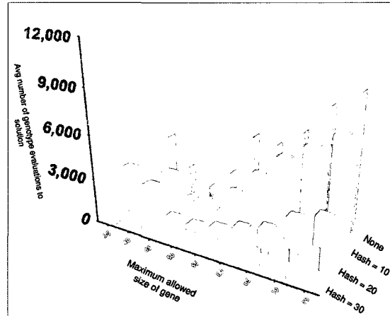
Figure 7.19: Relationship between average number of evaluation to either a maximum of 20 generations (equivalent to 20000 genotype evaluations) or to solution discovery, compared to the maximum size of genes in gene pool and to the hash differentiation factor for the evolution of the xor boolean function. Each data point was obtained as the average of 50 runs. The settings for the system that do not vary are: maxComp =1500 units, ecosystemDefaultSize =1000
