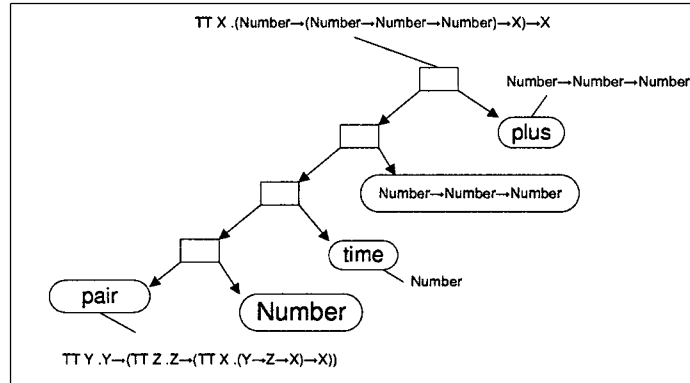
Figure 4.6: Rewrite of the genotype of figure 4.4 in the STN style
