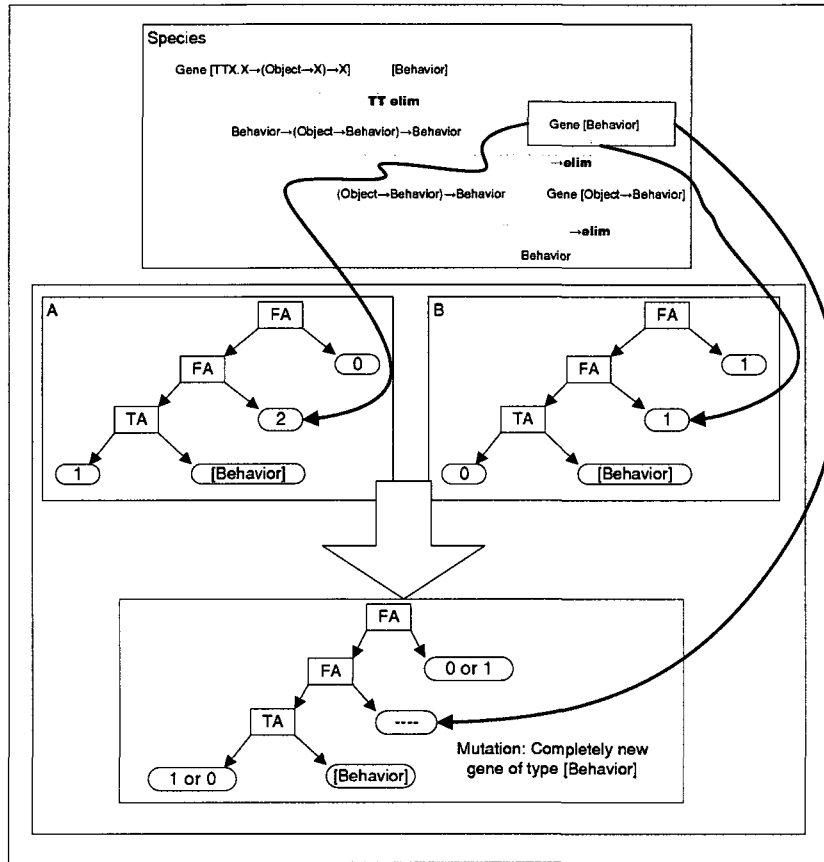
Figure 6.10: Crossover with mutation generated by the introduction of a new gene in the gene pool.
