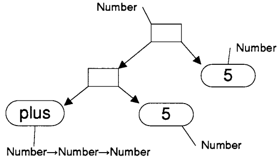
Figure 5.1: Parse tree for term (plus\ 5\ 5)
