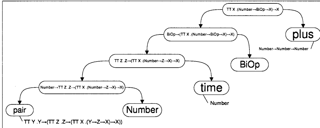
Figure 4.4: Representing a pair data structure with parametric polymorphism. This structure of the tree becomes the data structure that associates an object of type [Number] with an operation of type [Number \rightarrow Number \rightarrow Number]
