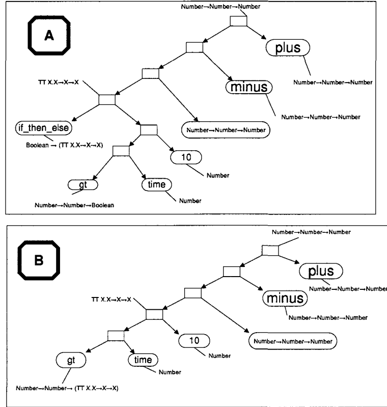
Figure 4.7: Two polymorphically-typed versions of the computational block represented in figure 4.2. Because the gt operator of the terminal set of the genotype labeled B evaluates directly to an appropriate projection function, the genotype is able to express branching without a branching operator.
