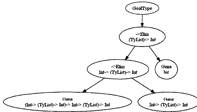
Figure 7.9: Species to which the example program that normalizes to 7.10 belongs
