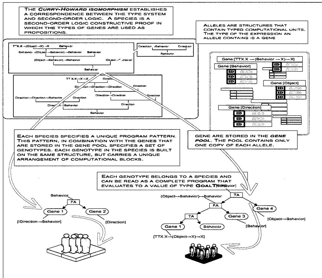
Figure 6.1: Overview of the relationship between species, alleles and genotypes
