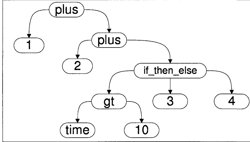
Figure 2.1: Genotype formed using the classical GP representation scheme and built from primitives defined in table 2.1
