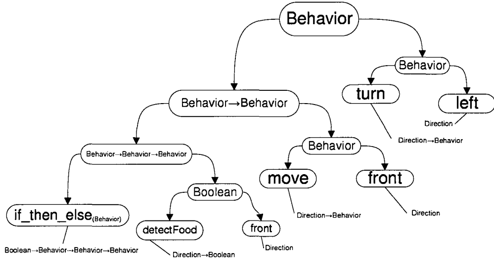
Figure 3.1: Strongly-typed genotype for a side-effect GP system based on the primitives defined in table 3.2
