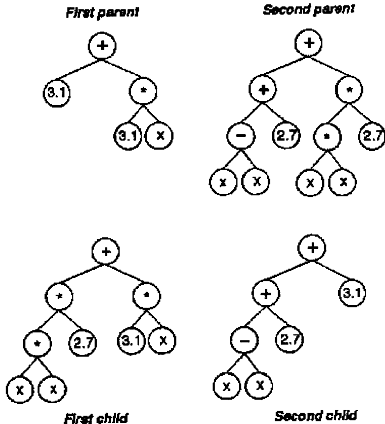
Figure 2.5: An example of crossover. A branch is selected for crossover in each of the parent trees. In this example, the first left branch from the first parent is exchanged with the first right branch of the second parent. This creates two new trees. Diagram from [19]
