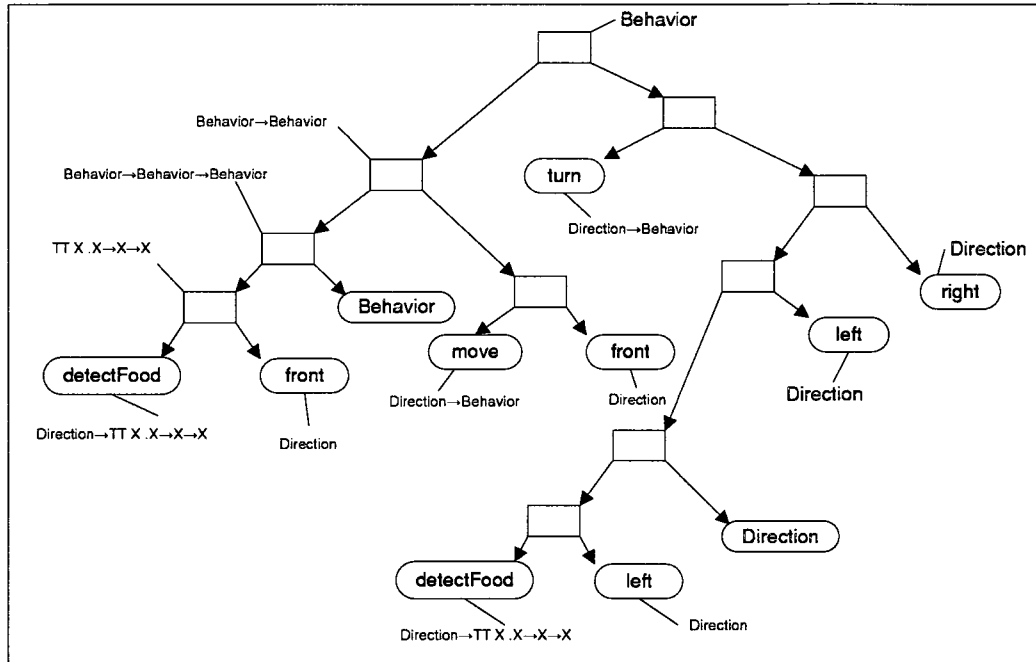
Figure 5.2: The STN parse tree corresponding to term 5.4
