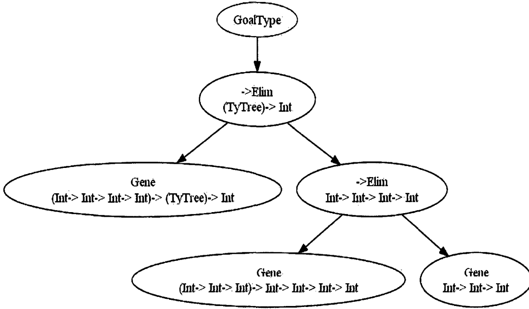
Figure 7.12: The species of the solution program corresponding to the term of 7.15
