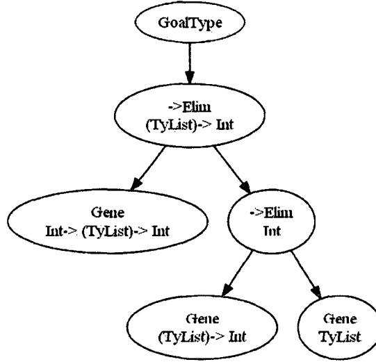
Figure 7.7: Species to which the example program that normalizes to 7.8 belongs
