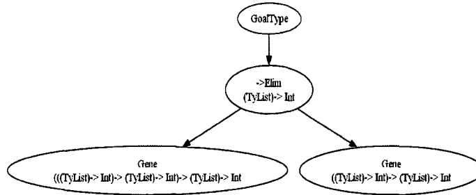
Figure 7.8: Species to which the solution listed for the parity of a list problem belongs
