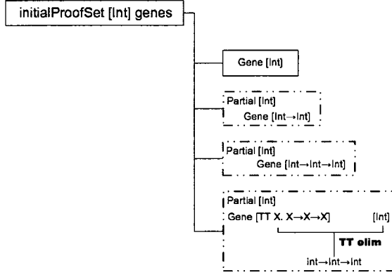
Figure 6.4: A call to the initialProofSet function with goal type [Int]
