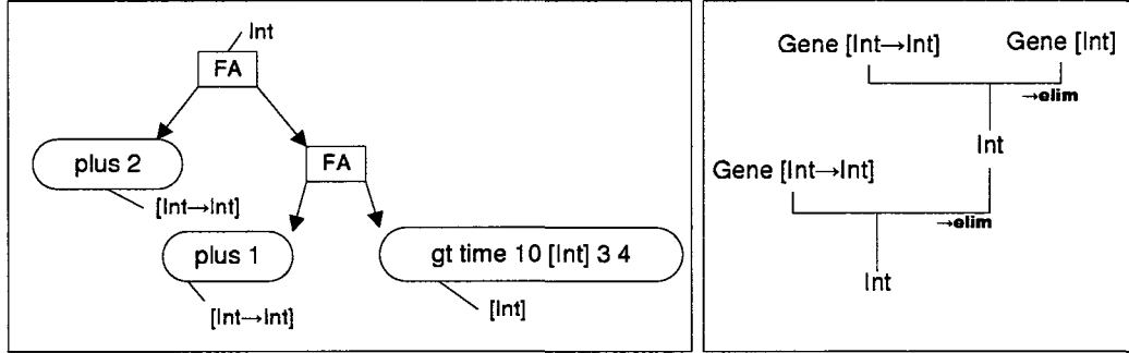
Figure 6.7: A non-evaluated phenotype assembled from alleles contained in a gene pool built using the context defined in table 6.2.3 and the species it belongs to (right)
