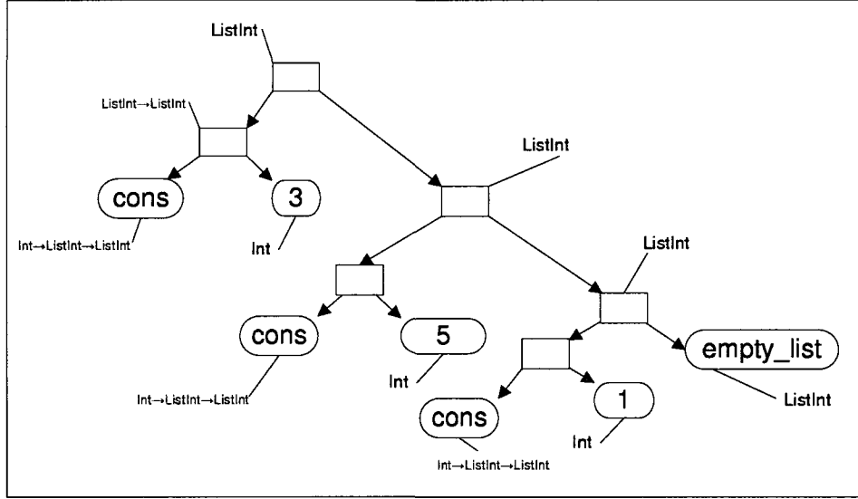
Figure 5.4: Parse tree for list of three objects of type [Int]
