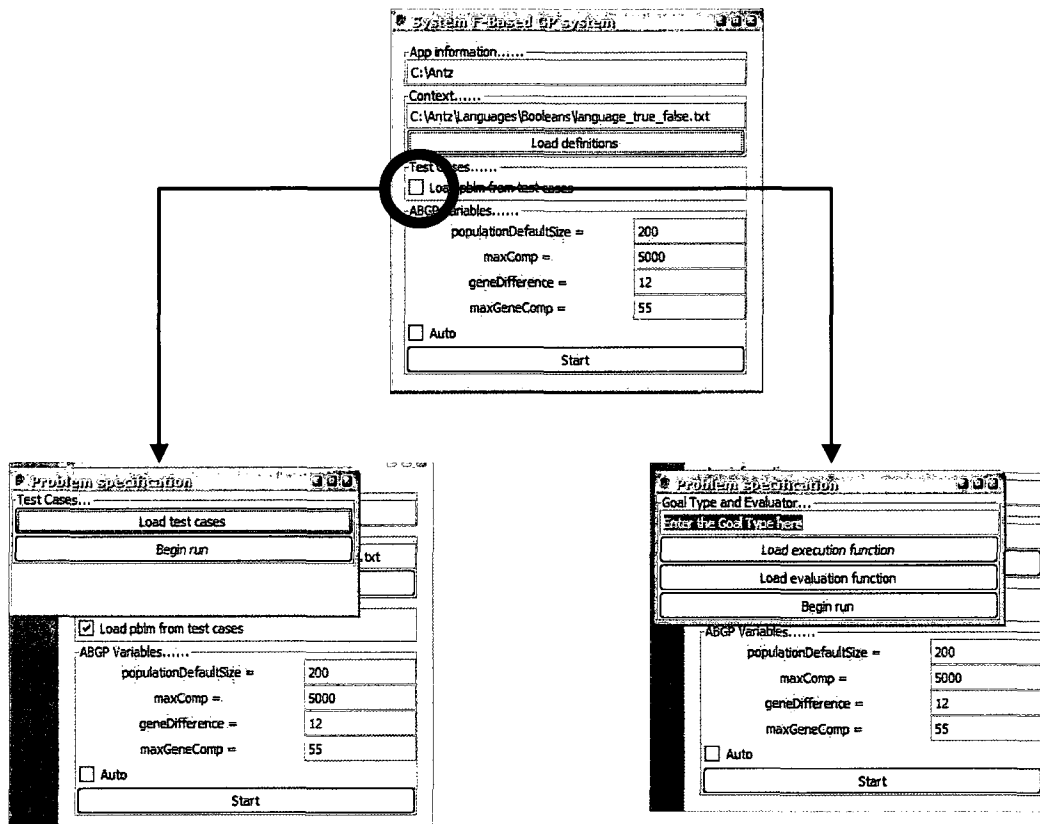
Figure A.3: A problem may be specified either by test cases or by a custom method, such as for the ant application
