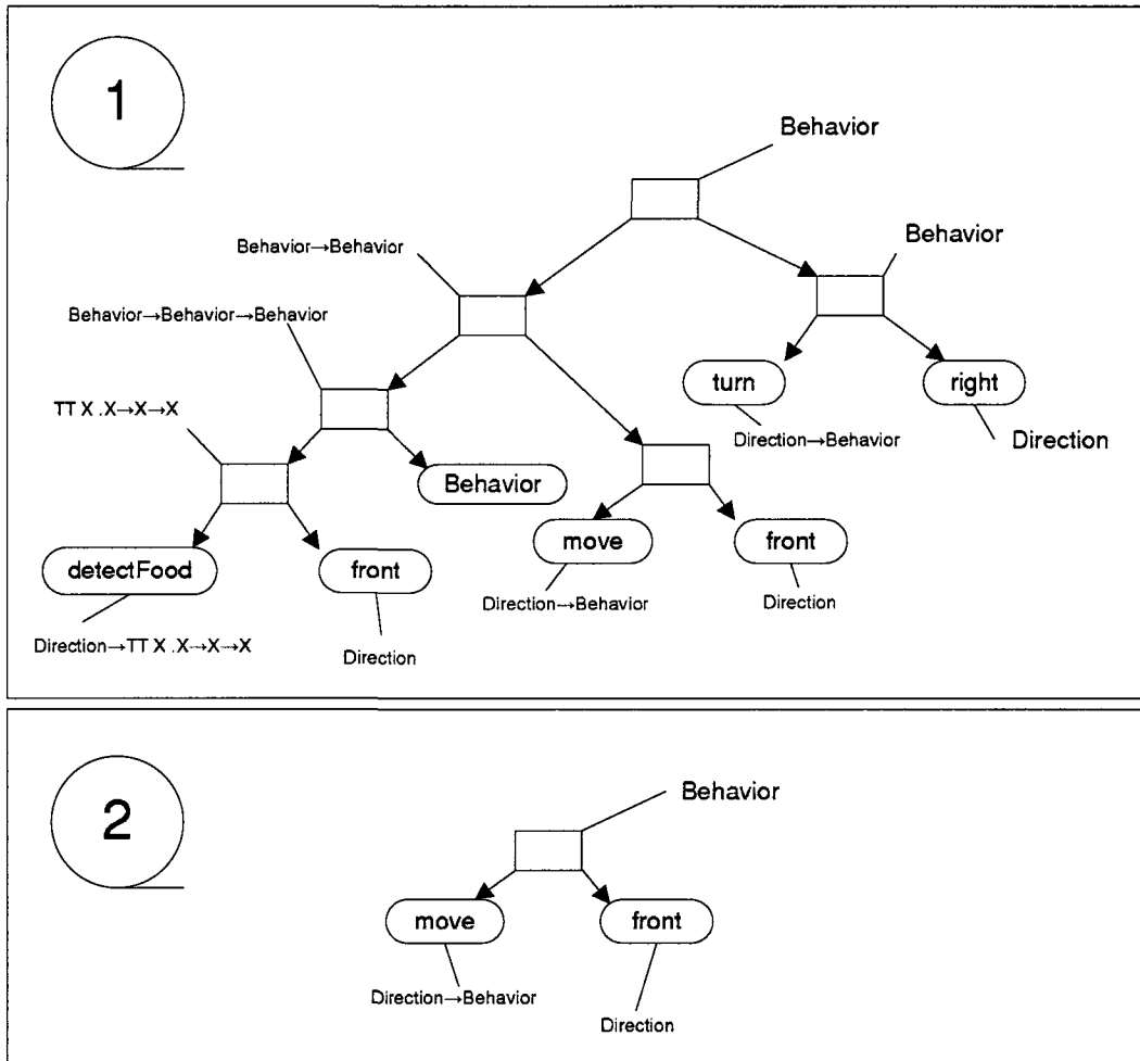
Figure 4.12: Execution sequence of the genotype of figure 4.2
