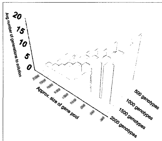
Figure 7.20: Relationship between average number of generations to convergence to solution and size of genotype population and maximum size of gene pool. Gene Pool Maximum Size of Individual Genes = 55 units, problem is xor, hash differentiator is set at 10
