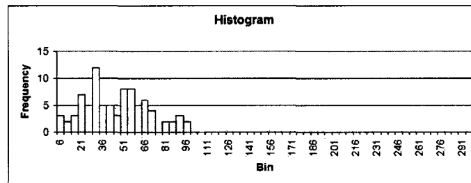
Figure 7.18: Distribution of allele size in gene pool after one generation when maxGeneComp is set at 300 units of complexity. Results obtained using system 1. The settings for the system were: maxComp = 7000 units, ecosystemDefaultSize = 4000
