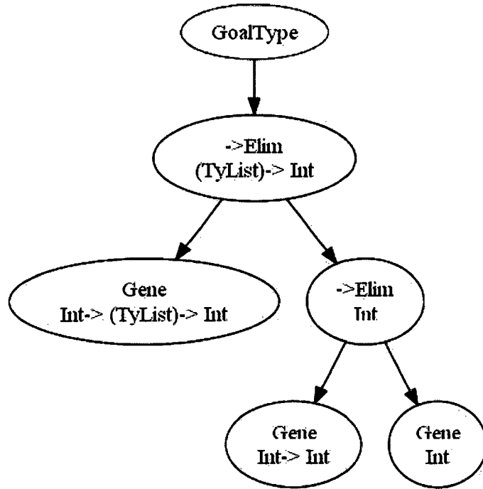
Figure 7.10: Species to which the solution for the list parity problem belongs (term 7.11)
