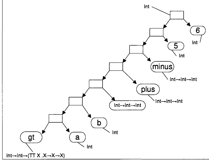
Figure 5.3: A parse tree of the System F term (gt\ a\ b\ [Int \rightarrow Int \rightarrow Int]\ plus\ minus\ 5\ 6)
