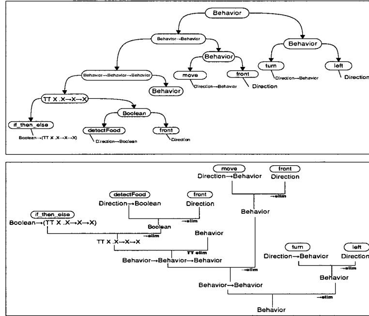
Figure 4.5: The parse tree of a polymorphically typed genotype (above) and its corresponding Curry-Howard proof tree (below)
