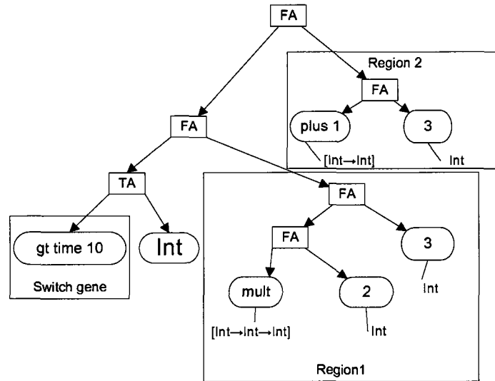
Figure 8.1: The ABGP analogy of an homeotic gene
