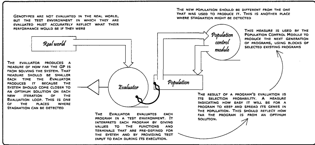
Figure 2.4: GP evaluator feed-back loop
