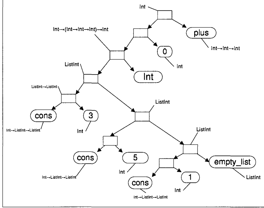
Figure 5.5: Recursive sum on a List
