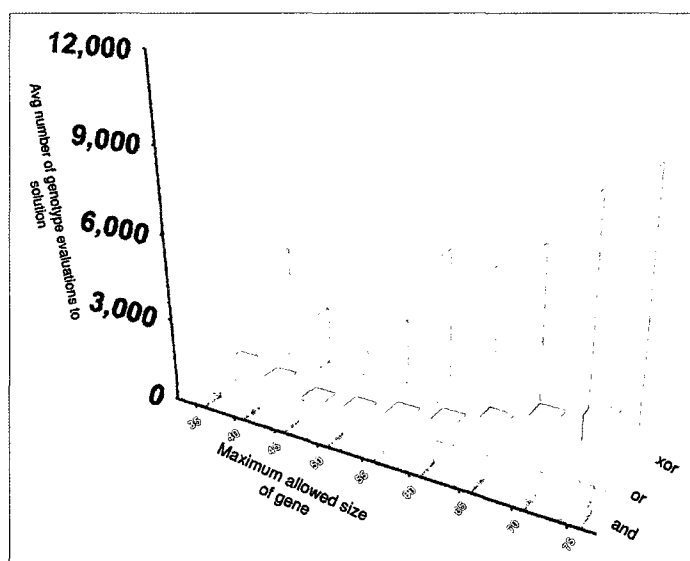
Figure 7.16: Relationship between average number of evaluation to either a maximum of 20 generations (equivalent to 20000 genotype evaluations) or to solution discovery and maximum size of genes in gene pool for each of the three boolean functions evolved. Each data point was obtained as the average of 50 runs. The settings for the system that do not vary are: maxComp = 1500 units, ecosystemDefaultSize = 1000
