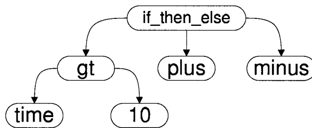
Figure 4.1: A potentially useful computational block that cannot be expressed using the classical representation scheme. The program uses the terminals of table 2.1 in a reasonable way from a computational perspective, but is an illegal formation according to definition 2.2.3
