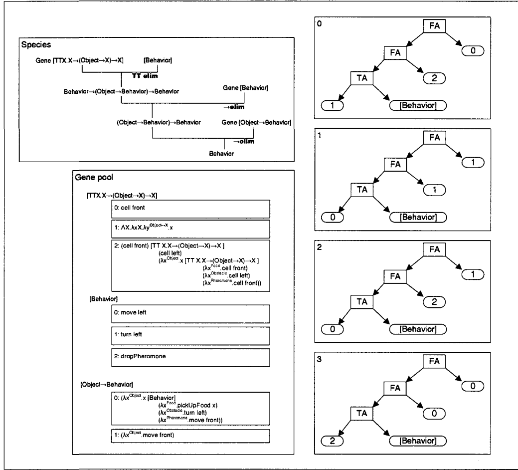
Figure 6.6: Four genotypes that belong to the same species and the subset of the gene pool that contains the alleles that compose them
