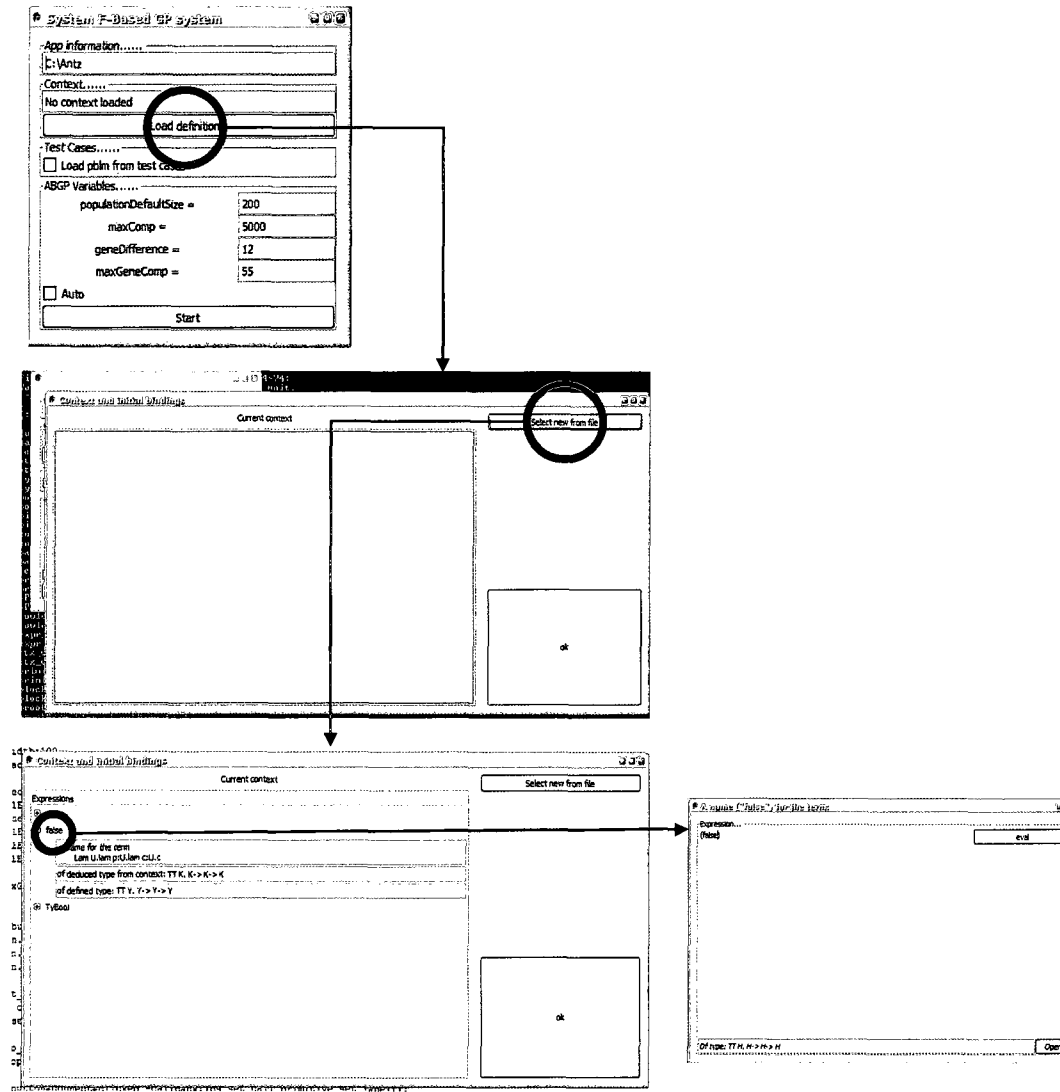
Figure A.2: The application's entry point, and loading a context
