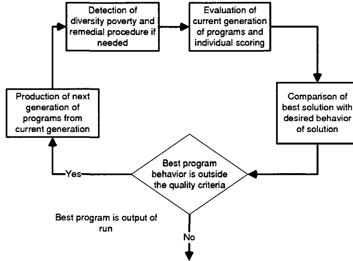
Figure 2.3: GP system cycle
