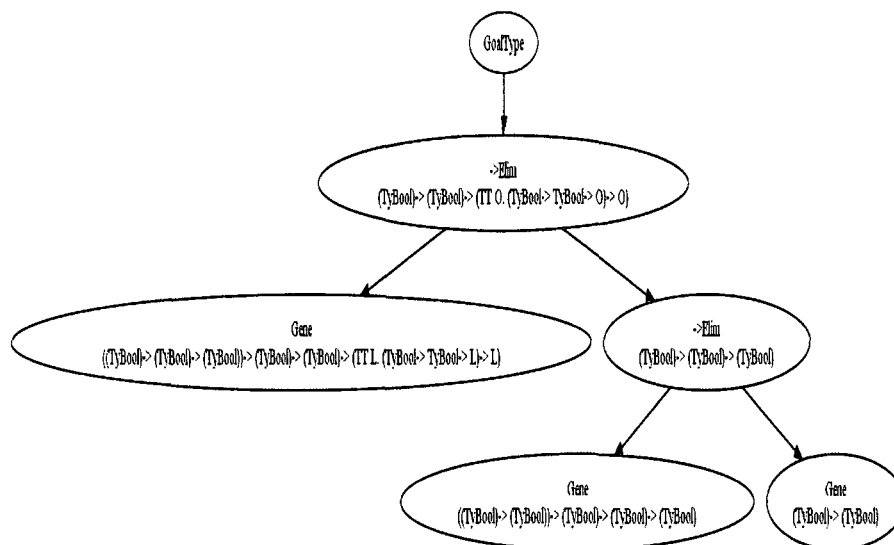
Figure 7.6: Species to which the example program (half-adder) that normalizes to 7.6 belongs
