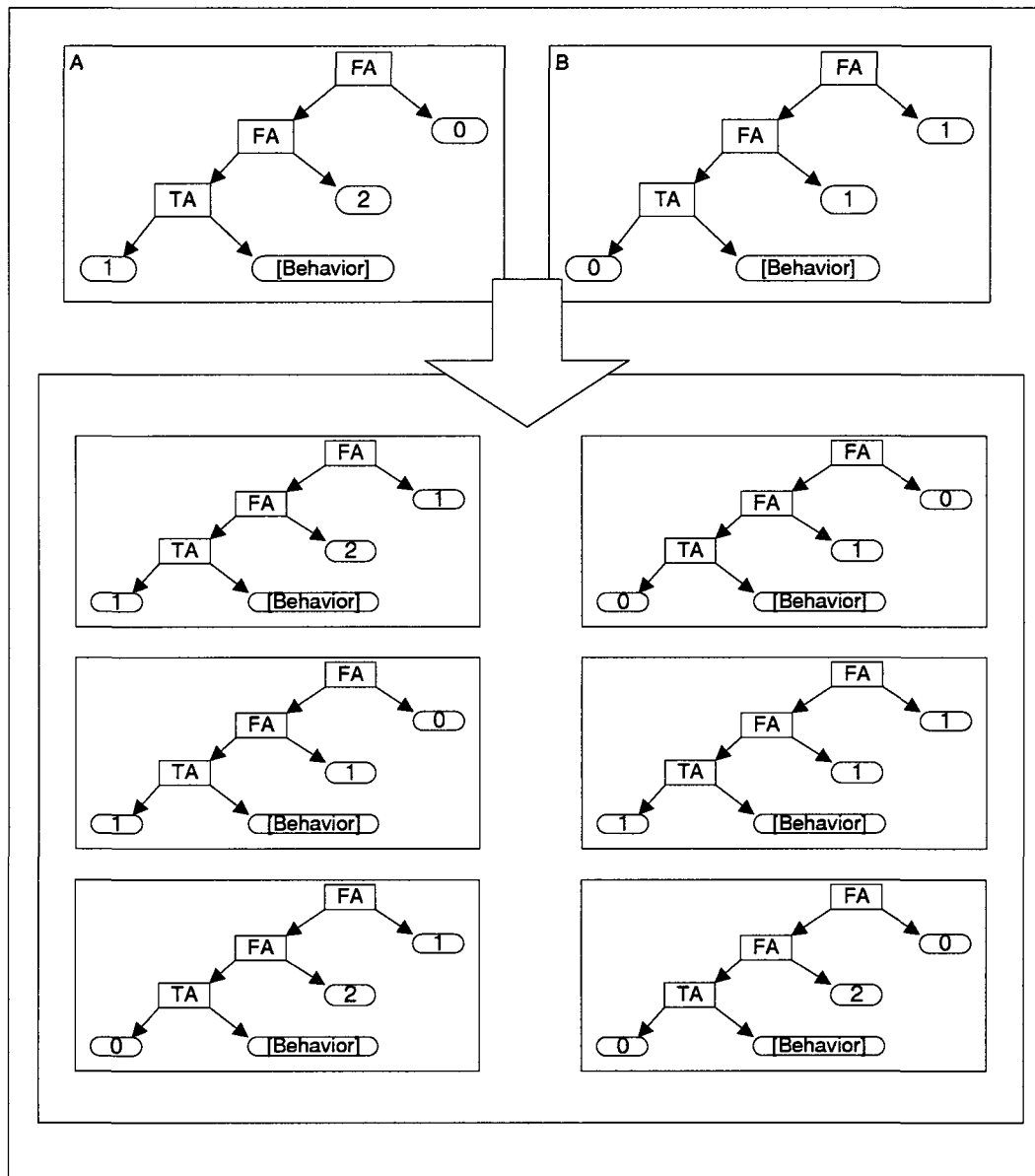
Figure 6.9: The basic crossover case. Any of the 6 possible offspring belongs to the same species that both their parents belong to and each of the offspring genes originates from one or the other parent
