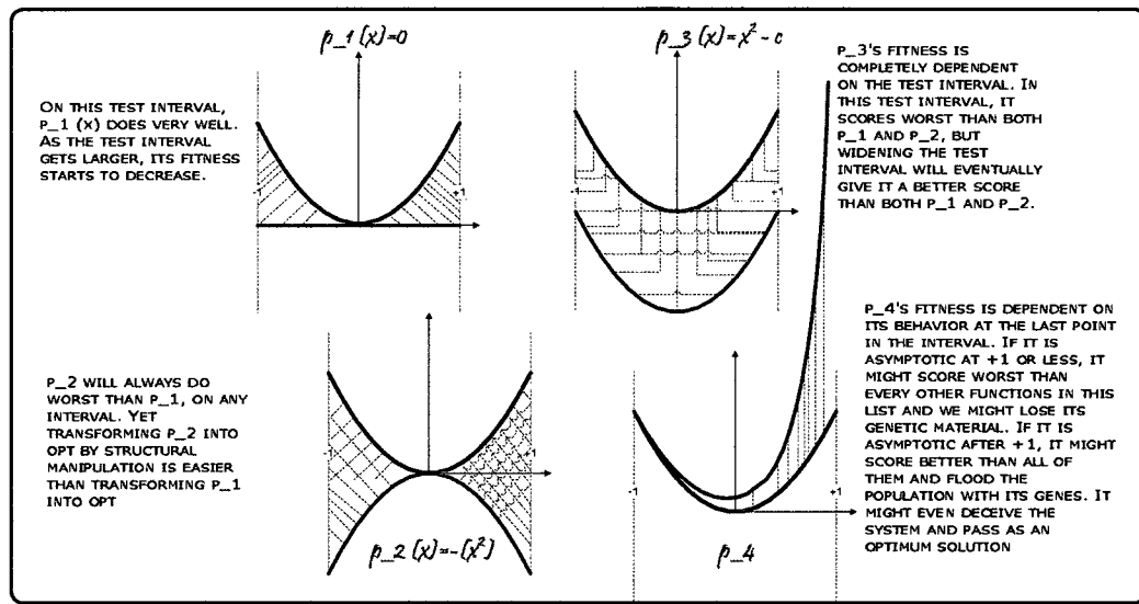
Figure 2.6: Measuring the quality of an approximation
