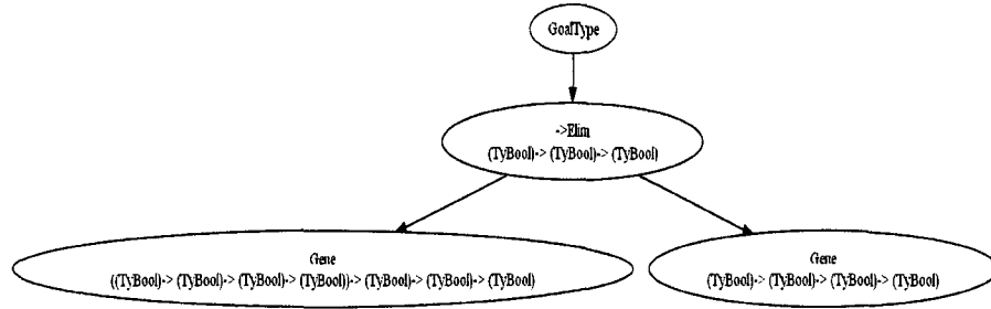
Figure 7.2: Species to which the example program ( and function) that normalizes to 7.2 belongs
