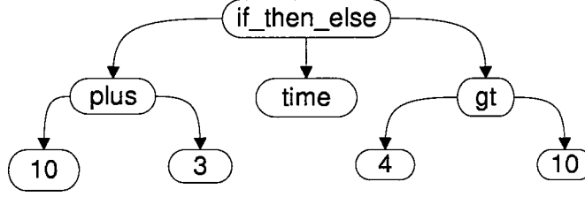
Figure 2.2: This genotype is formed legally using the set of primitives of table 2.1. It is non-sensical when used with the \chi_{(Ph)_1} function defined in table 2.2, but is sensical when the \chi_{(Ph)_2} function is used.
