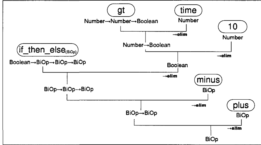
Figure 4.3: The genotype of figure 4.2 corresponds to a proof when the types of the leaves are considered to be propositions. When only simple types are considered, there is only one deduction rule, corresponding to the usual \rightarrow -Elim rule
