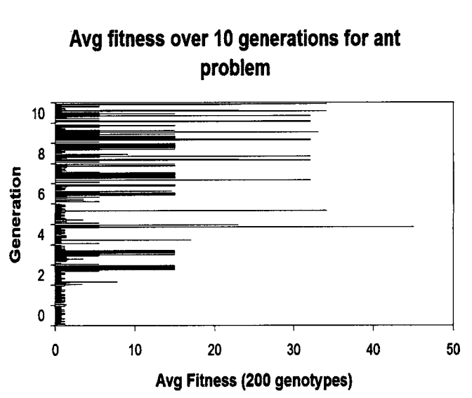
Figure 7.15: Species of genotype example for ant problem
