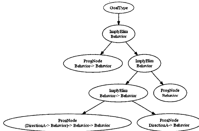
Figure 7.14: Species of genotype example for ant problem
