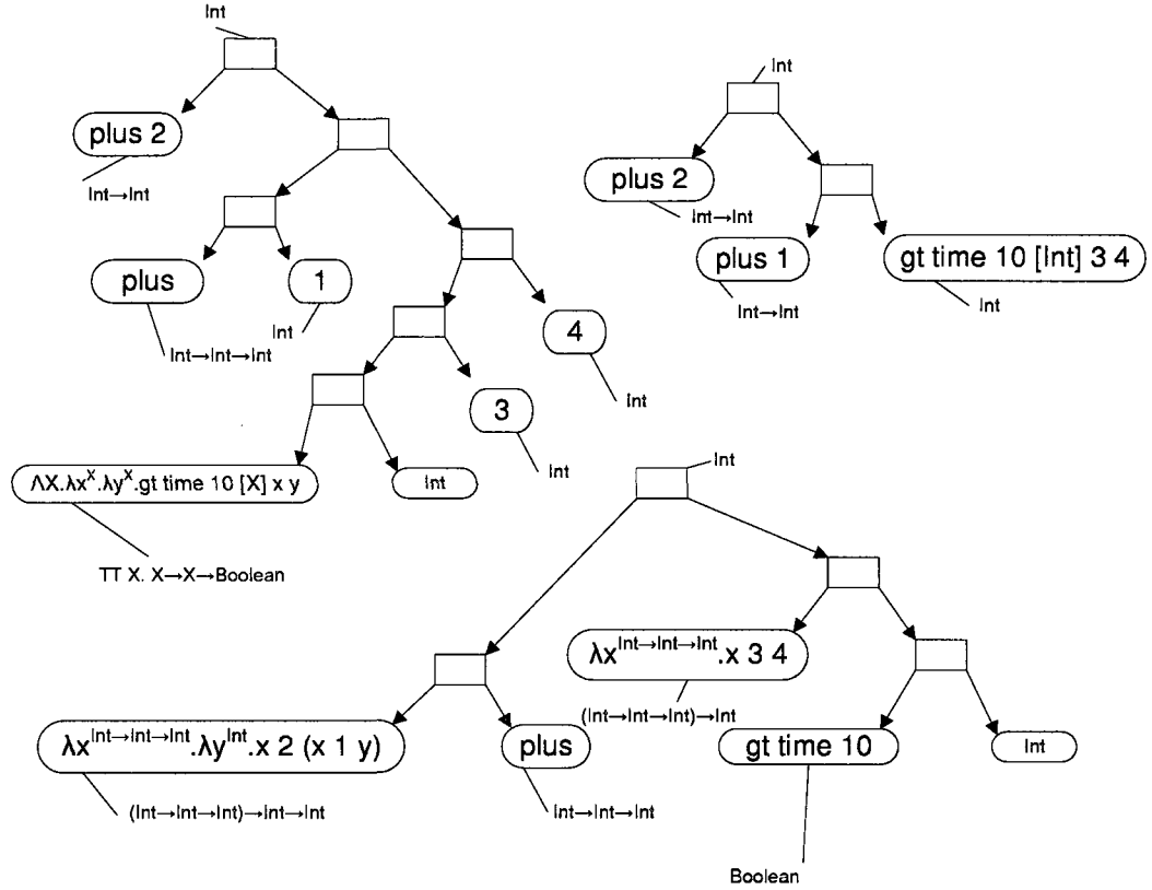
Figure 6.8: The same phenotype results from these three different genotypes as they normalize to the same term
