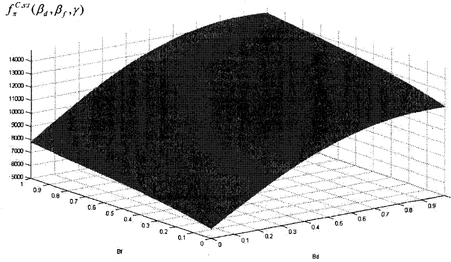
Figure 32 - The graph of f_{\pi}^{C, st}(\beta_d, \beta_f, \gamma) at \gamma = 2
