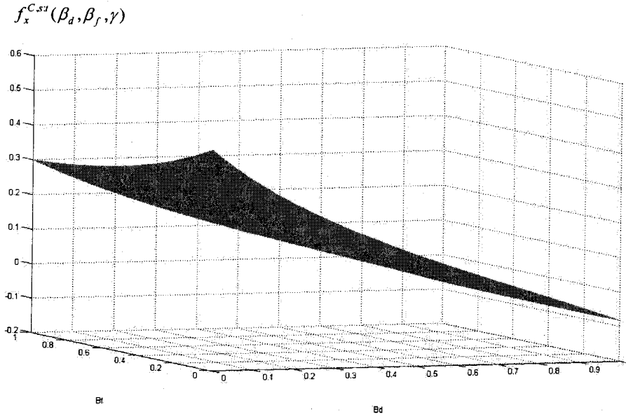
Figure 30 - The graph of f_x^{C,sl}(\beta_d, \beta_f, \gamma) at \gamma = 2
