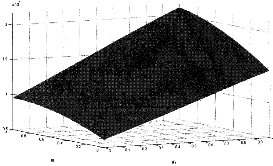
Figure 28 - The graph of f_{CS}^{NC,sz}(\beta_d, \beta_f, \gamma) at \gamma=2
