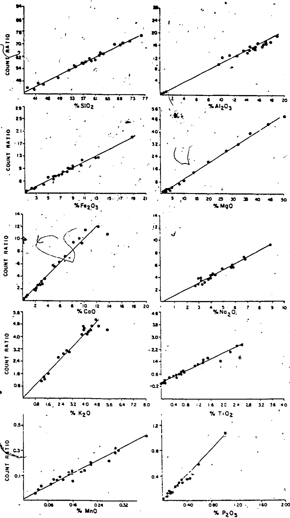
Figure B.1: Calibration Curves Used in This Study
