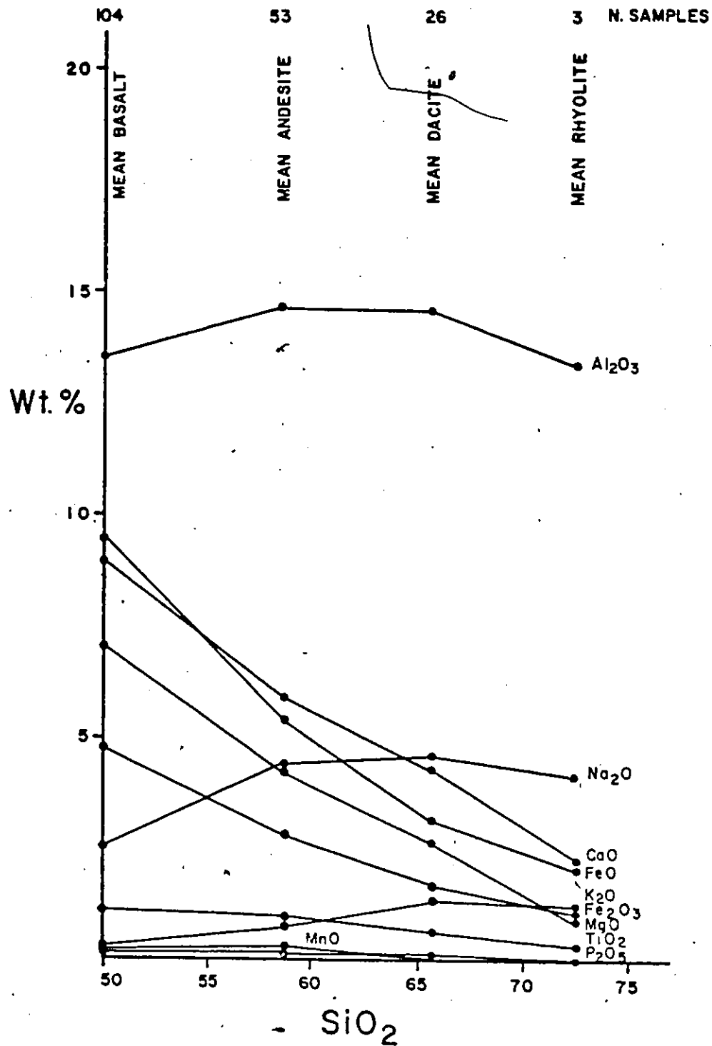
Figure 6.6: Whole Bachelor Lake Region - Harker Variation Diagram
