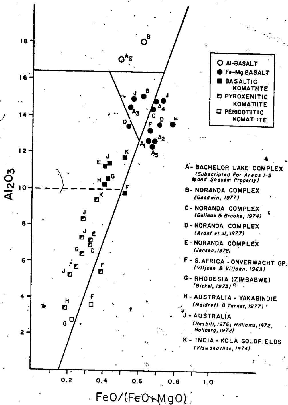
Figure 3.6: World Archean Mafic-Ultramafic Rock Suites on the Al 2 O 3 vs FeO/FeO+MgO Diagram
