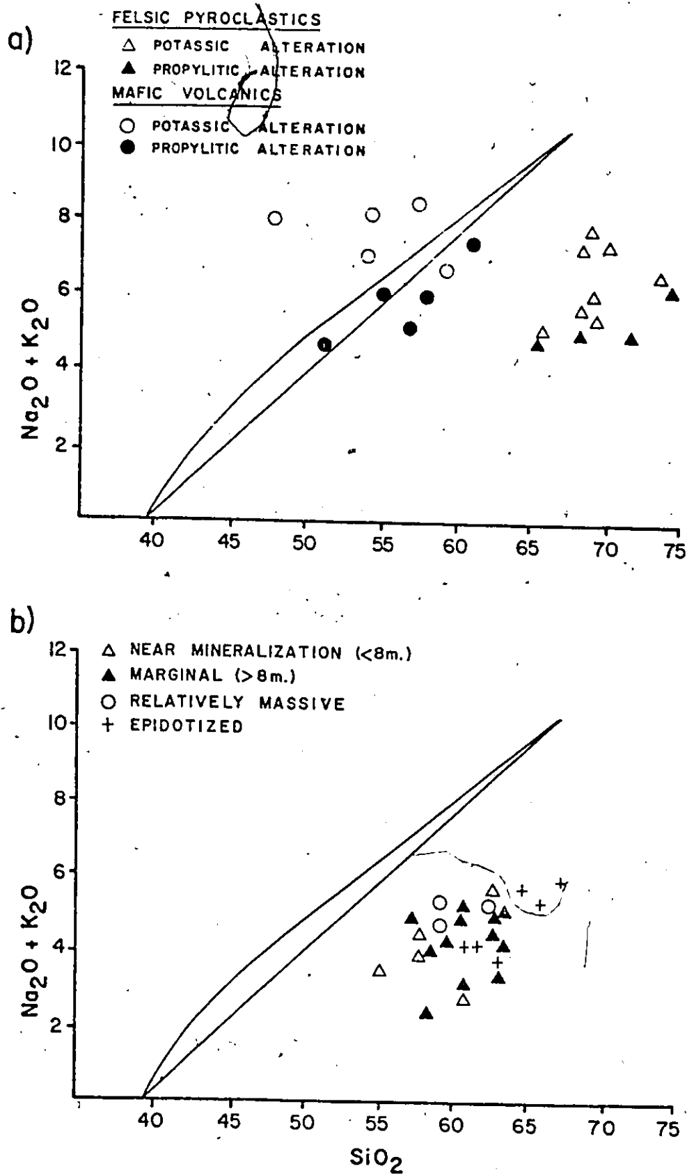
Figure 7.5: Alkali-Silica Diagrams a) QSRML b) Soquem Properties
