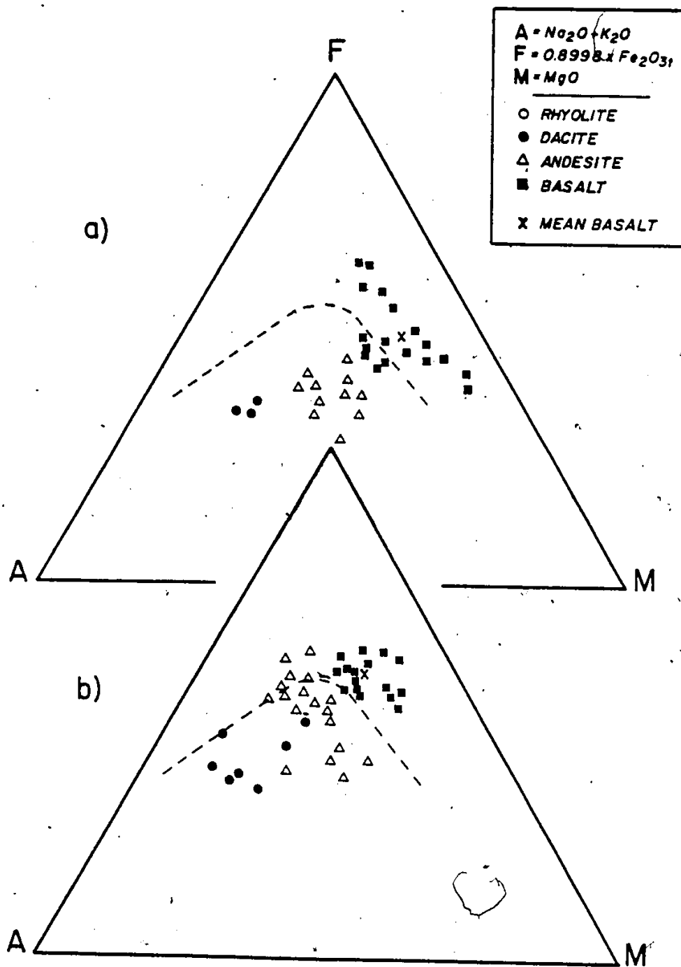
Figure 6.18: AFM Diagram a) Area 3 b) Area 4
