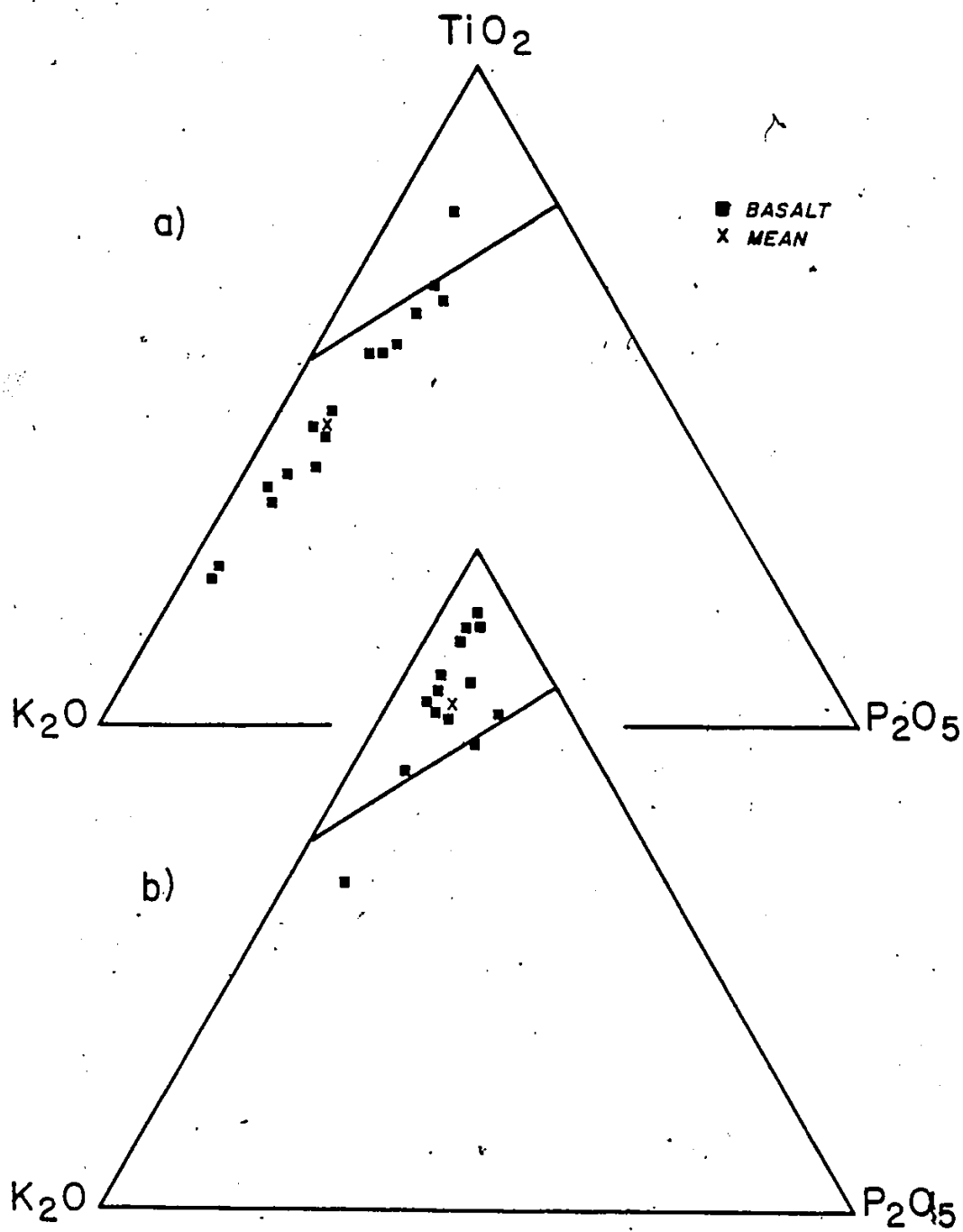
Figure 6.22: Pearce Diagram a) Area 4 b) Area 5
