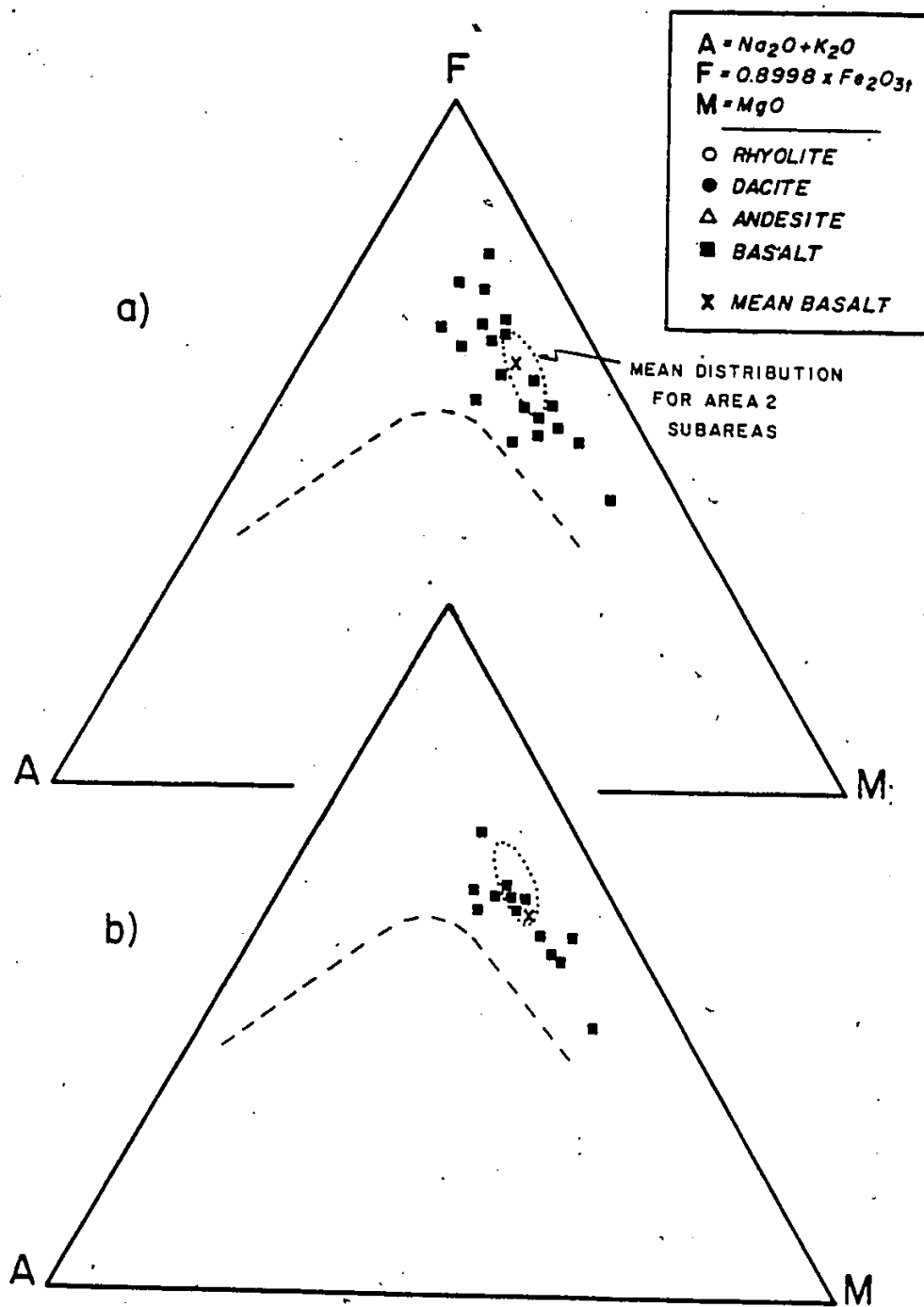
Figure 6.12: AFM Diagram - Subareas a) 2a b) 2b
