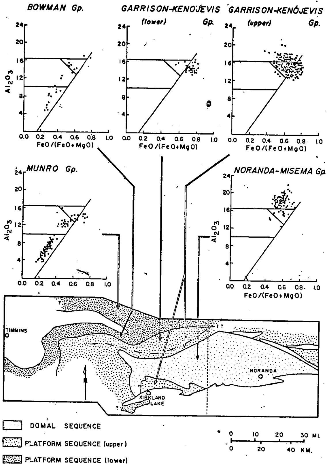
Figure 8.2: Major Chemical Trends in the Noranda Complex
