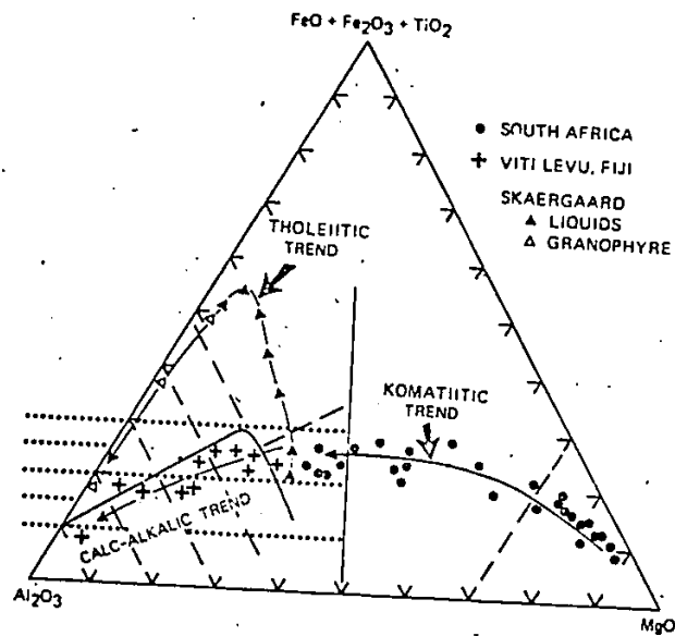
Figure 3.10: Jensen (1976) Volcanic Rock Classification Diagram
