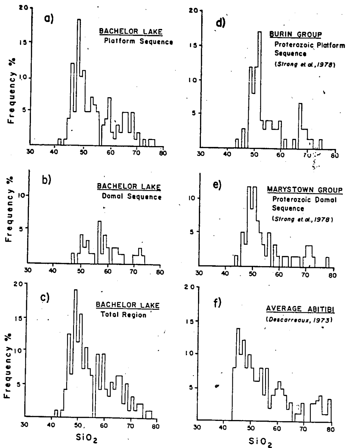
Figure 8.3: SiO 2 Frequency Distribution for Selected Volcanic Sequences
