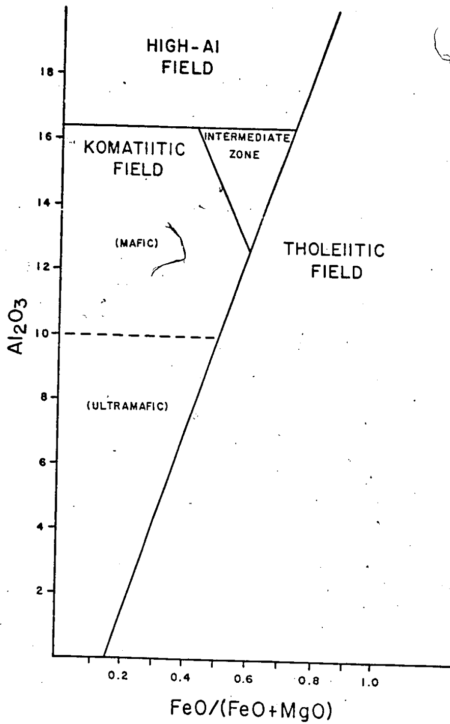
Figure 3.5: Al_2O_3 vs FeO/(FeO+MgO) Diagram
