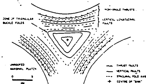
2. Plan view of level "X" in 1 after basement remobilization showing the trigonal symmetry of the greenstone belt due to "close-packed" plutons, which are partially unroofed. Due to faulting, synclines predominate in the greenstone, giving way to a zone of triangular buckle folds above the "sink".
