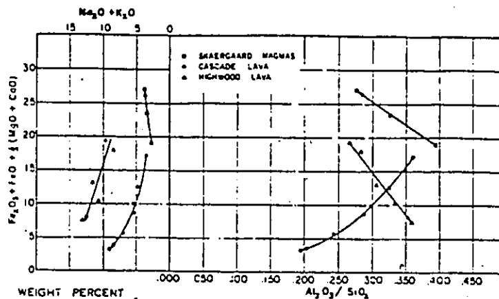
Figure 3.9: Church (1975) Volcanic Rock Classification Diagram
