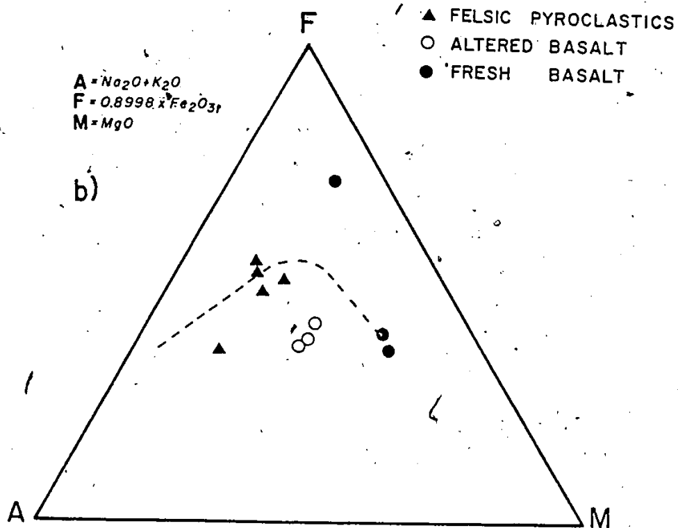
Figure 7.3: Coniagas Minesite Geochemistry a) Alkali-Silica b) AFM Variation
