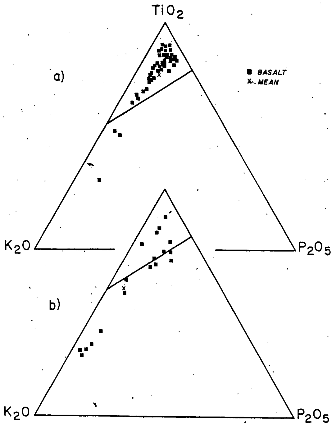
Figure 6.15: Pearce Diagram a) Area 2 b) Area 3
