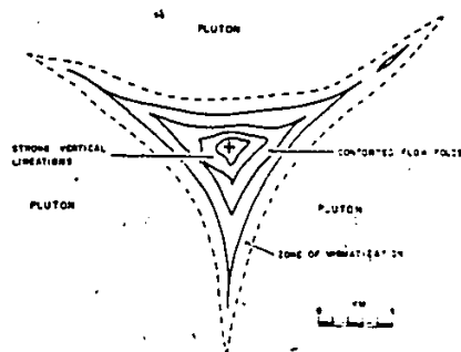
3. Plan view of level "Y" in 1 after basement remobilization. At this level (near the catasone) the rocks are metamorphosed to amphibolite-facies with contorted flow-folding and prominent vertical lineations. The margins of the greenstones have reacted with the surrounding plutonic material to form a zone of migmatites.
