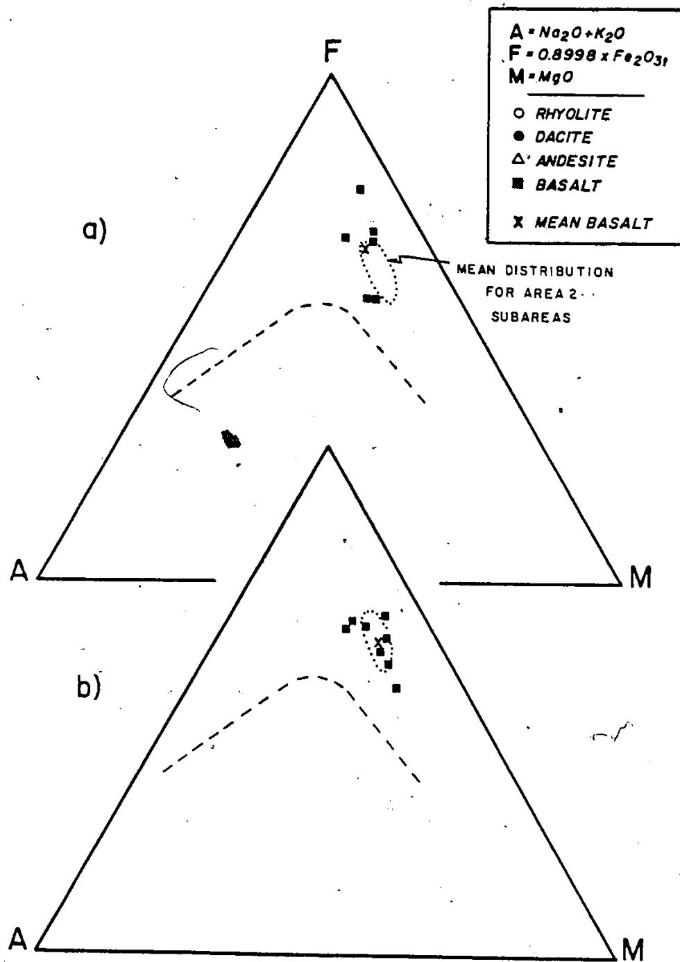
Figure 6.13: AFM Diagram - Subareas a) 2c b) 2d
