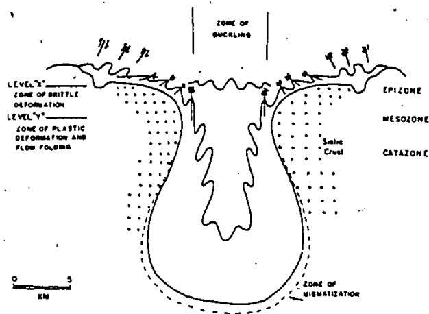
1. Structures expected near the centre of the subsiding greenstone belt. The attitude of faulting changes from high-angle reverse to subvertical and longitudinal nearing the central "sink". Buckling may be present in the upper sequences of the greenstones. At depth, plastic deformation predominates.
