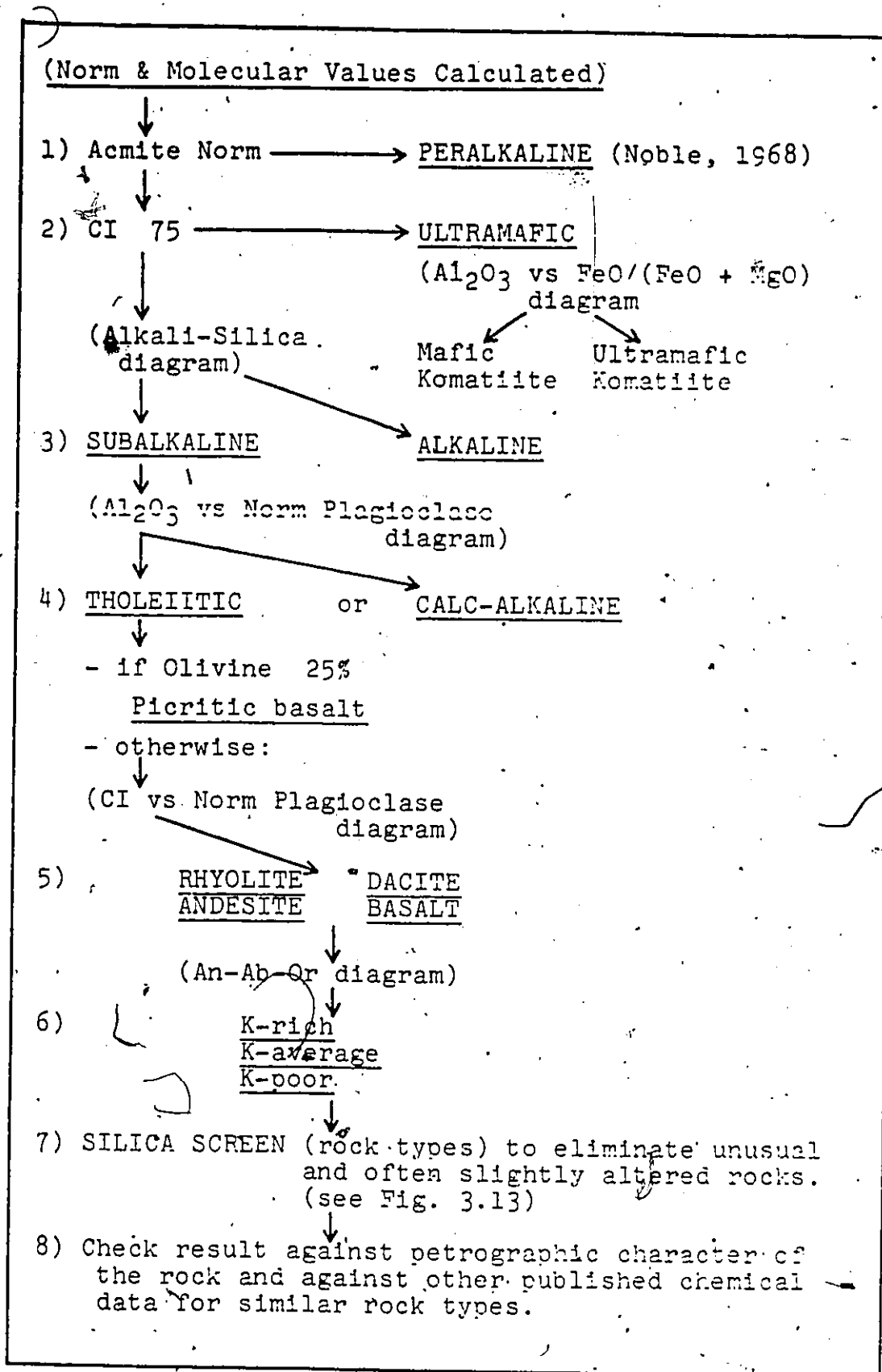
Figure 3.12: Modified Irvine-Bağar (1971) Classification Flow-Chart for the Bachelor Lake Suite
