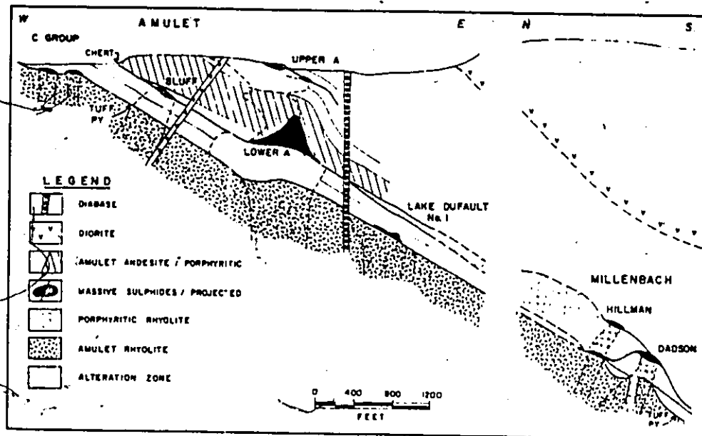
Composite sections, E-W through Amulet C and A deposits (Price, 1953) and N-S through adjacent Millenbach deposits (Simmons et al., 1973) modified by removal of most intrusions.
