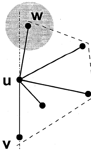
(c) Inconsistent
