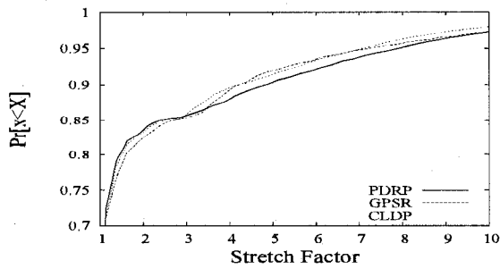
(e) 1700, d=8
