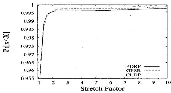
(a) 1300, d=5.1
