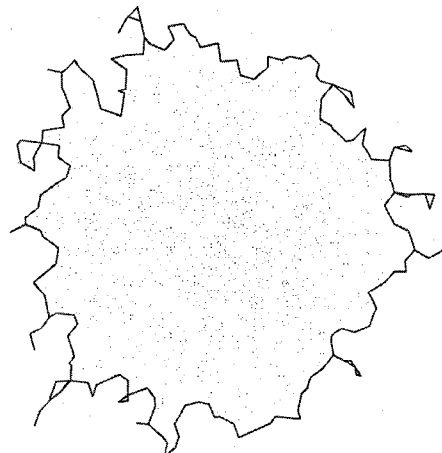
(c) 1500 nodes.
