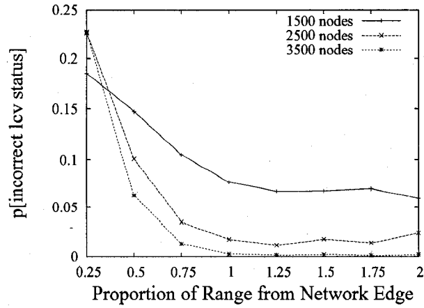
(a) Uniform
