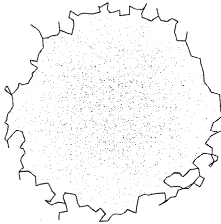
(a) 3500 nodes.
