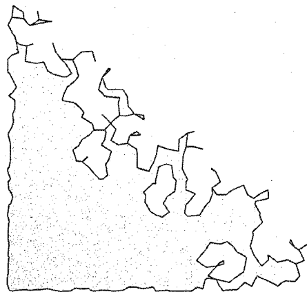
(c) 1500 nodes.
