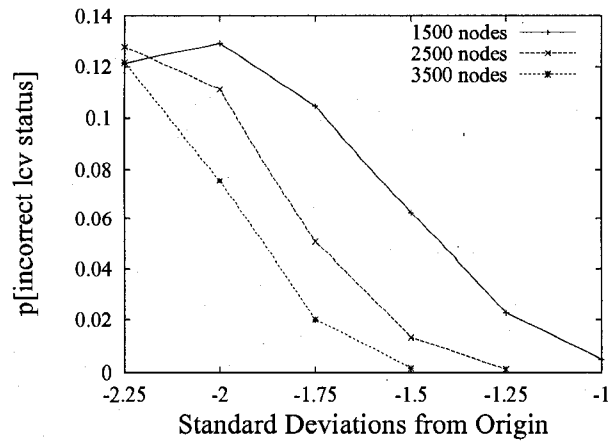
(b) Normal
