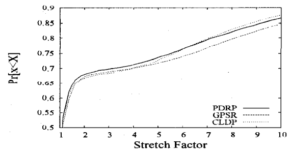
(h) 2000, d=12
