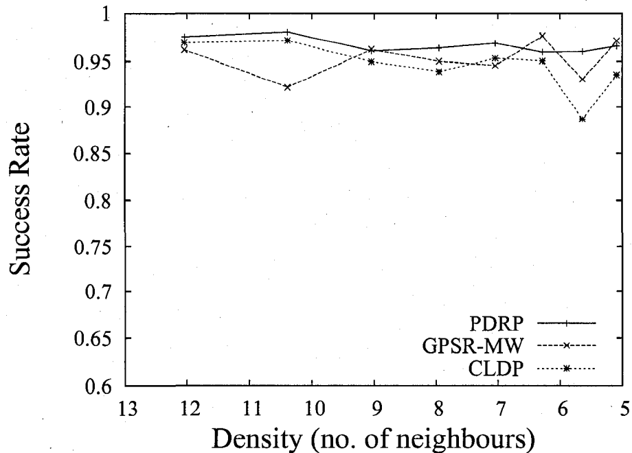
Figure 5.7: Routing Success.
