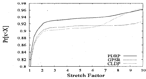
(c) 1500, d=6.3
