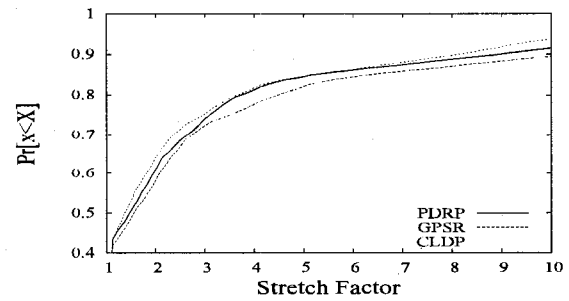
(f) 1800, d=9
