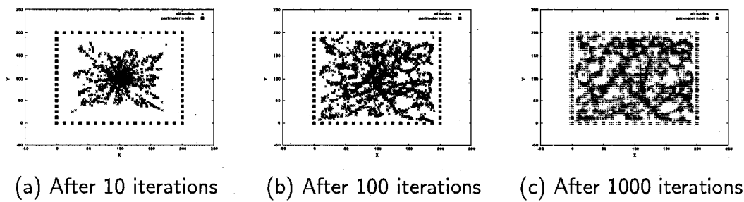
Figure 2.13: Intermittent virtual coordinates of 3200 nodes in a 200x200 space where nodes are known in advance to lie on the network's perimeter.
