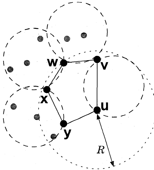
Figure 4.5: Node u may insert in \alpha_l(S) only directed incident edges uv and uy .
