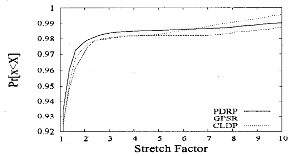
(b) 1400, d=5.6
