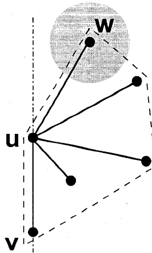
(a) Consistent
