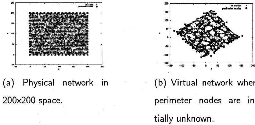
Figure 2.12: The (a) real and (b) virtual coordinates of a 3200 node network.
