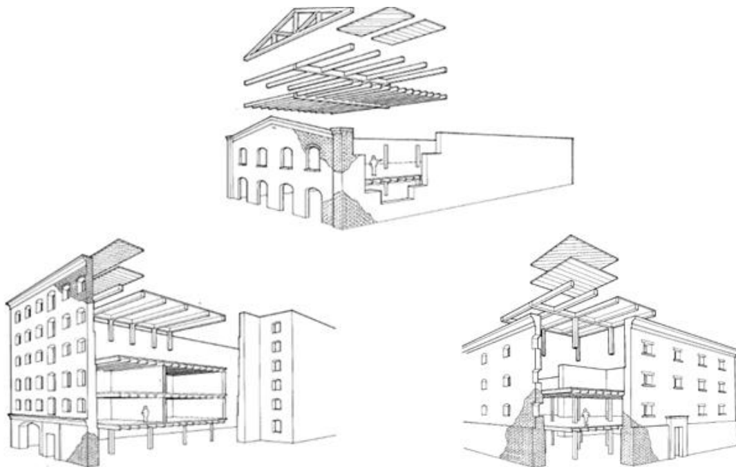
Figure 2-4: Typical construction of URM bearing-wall buildings in North America (ATC, 2002)
