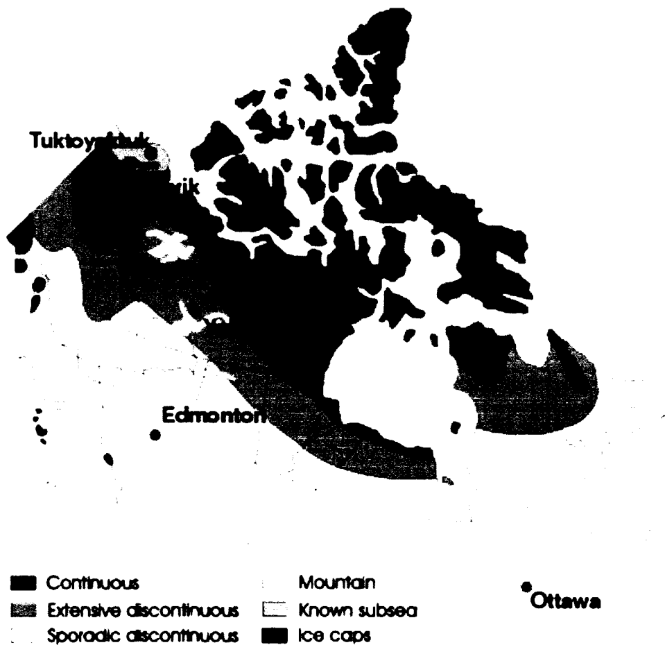
Figure 2.1: Canada Permafrost Distribution (From Geological Survey of Canada 2007).
