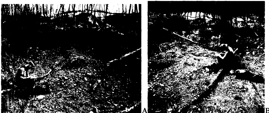
Figure 5.4: SC13A Photographs A: View upslope of the headscarp. Note the coarse material on the failure surface. B: Scar and debris pile. July 22, 2005.
