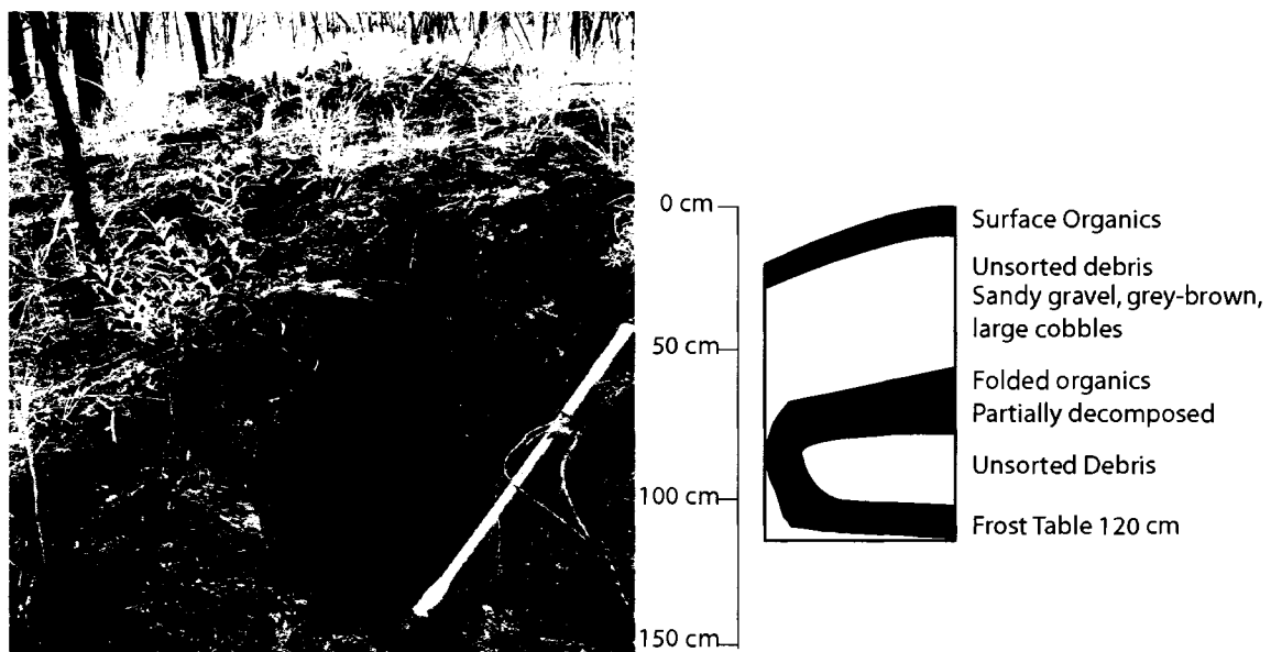
Figure 5.31. Excavation of Fossil Failure in Steele Creek. Mattock handle 1.2 m long. Dark organic material visible approximately 50 cm from the surface. June 20, 2006.
