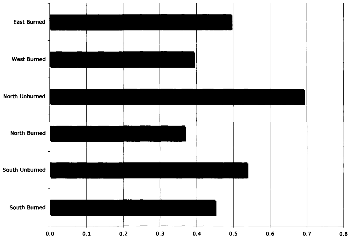
Figure 6.13: N-Freezing Factor. July 1, 2005- June 30, 2006.
