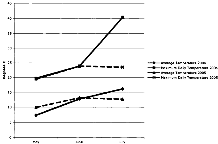
Figure 3.3: Henderson Dome Temperatures 2004-2005.
