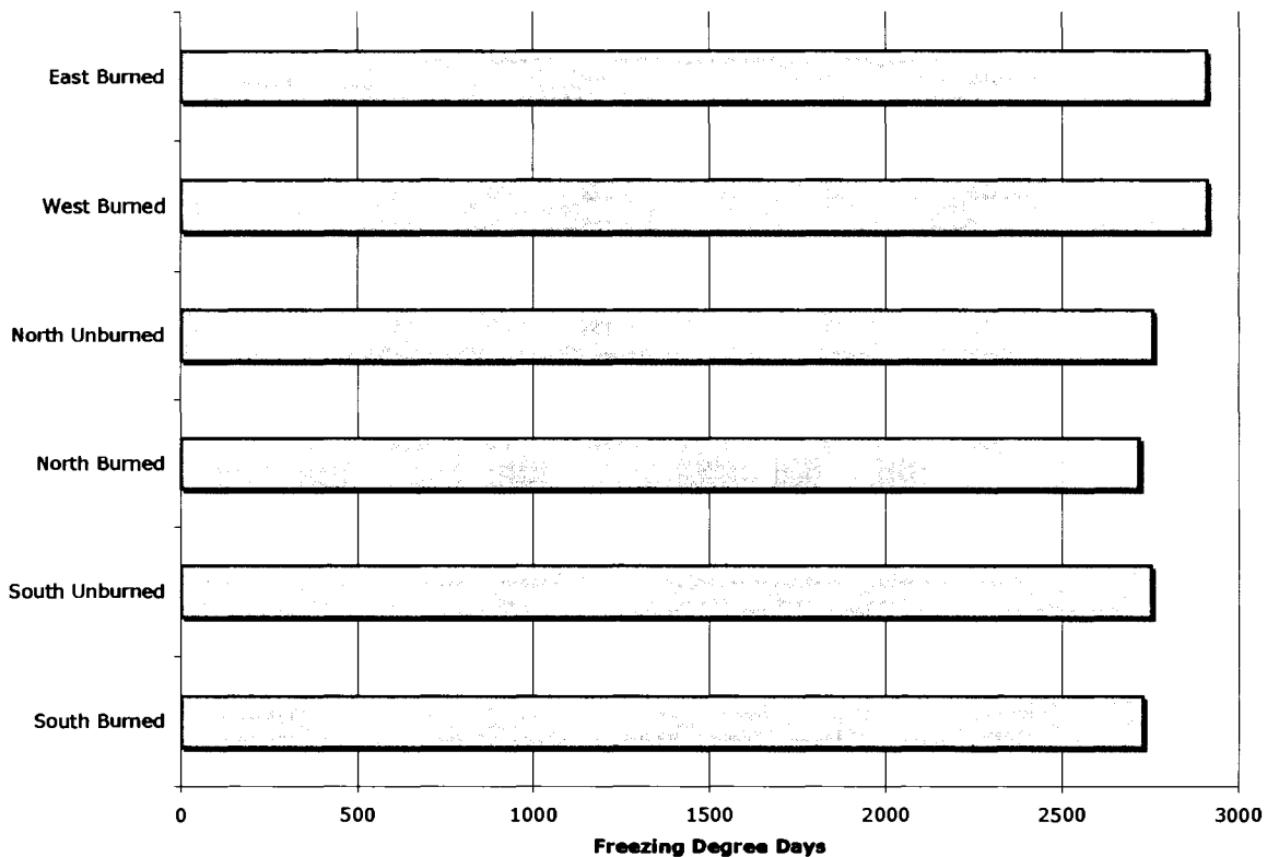
Figure 6.10: Air Freezing Degree Days. July 1, 2005- June 30, 2006.
