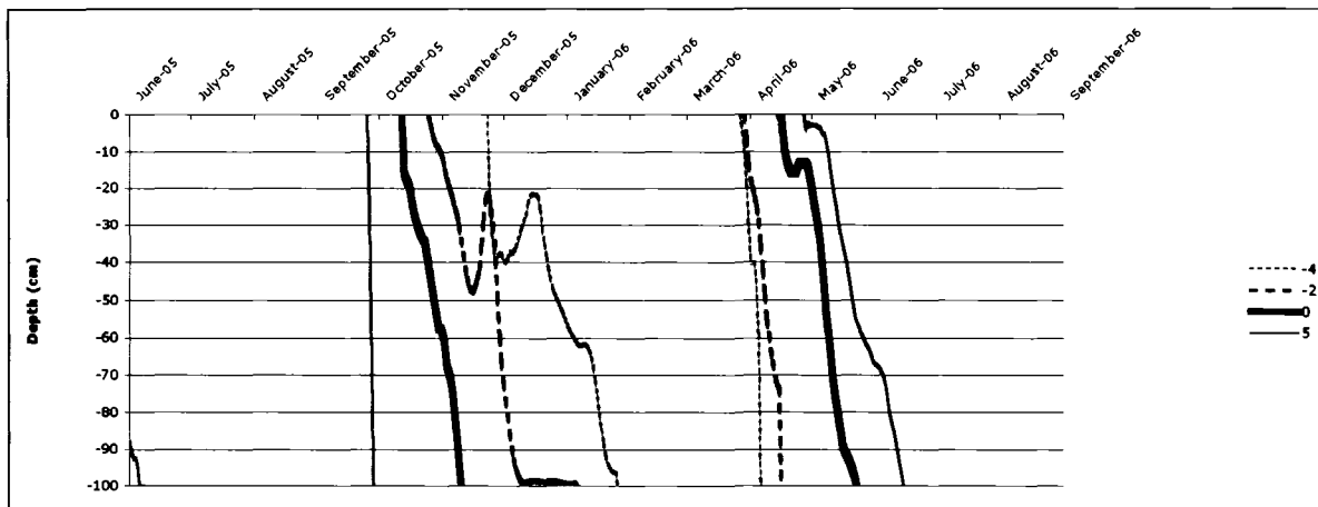
Figure 6.16: South-Facing Burned Site Isotherms. Isotherms were interpolated between measurement depths of 2 cm, 25 cm, 50 cm, 75 cm, 100 cm.
