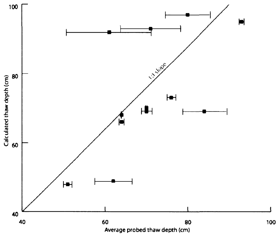
Figure 4.1: Relationship between average probed and thaw depths calculated from thermistor measurements. Average standard deviation over all points was 6.6 cm. Each point represents one site on one day.
