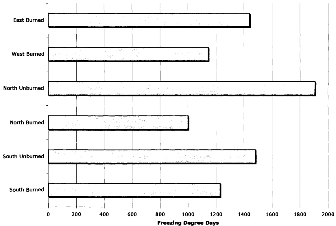
Figure 6.11: Ground Freezing Degree Days. July 1, 2005- June 30, 2006.
