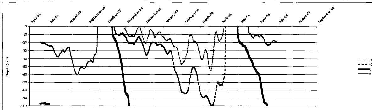
Figure 6.17: South-Facing Unburned Site Isotherms. Data not available after July 1, 2006. Isotherms were interpolated between measurement depths of 2 cm, 25 cm, 50 cm, 75 cm, 100 cm.
