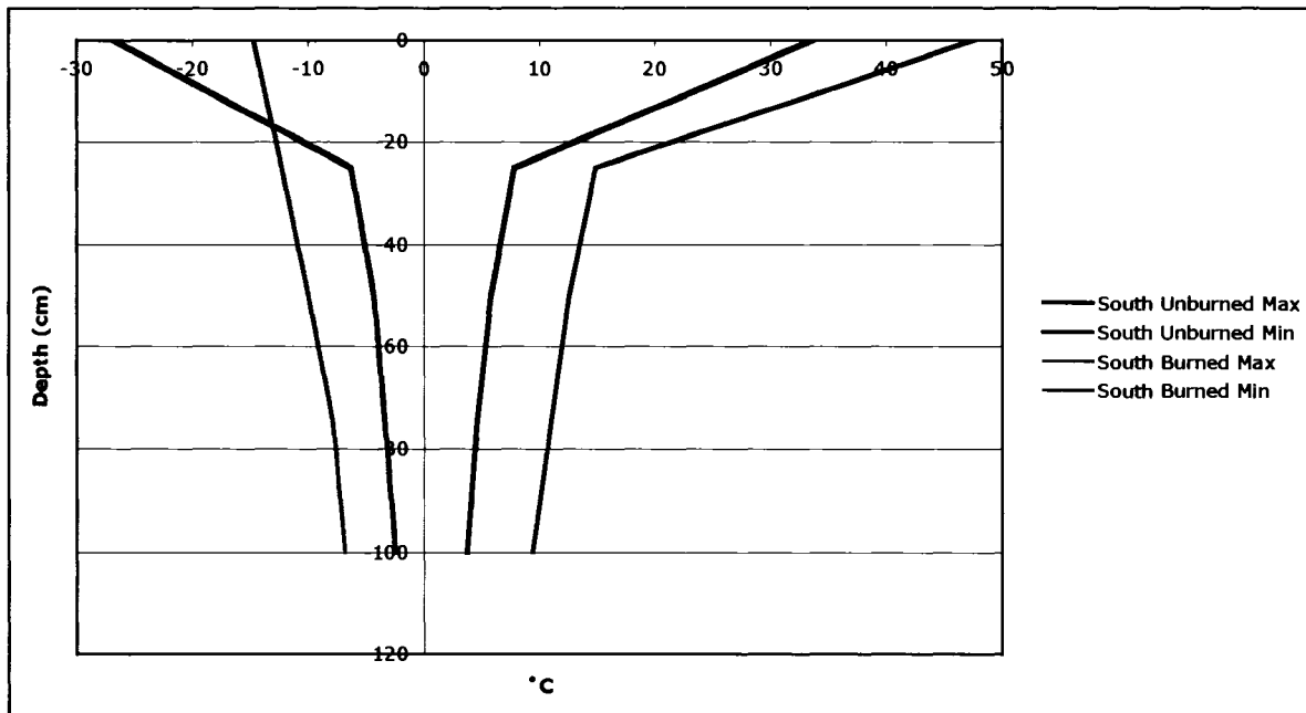
Figure 6.2: South ground temperature envelopes. June 29, 2005- July 1, 2006
