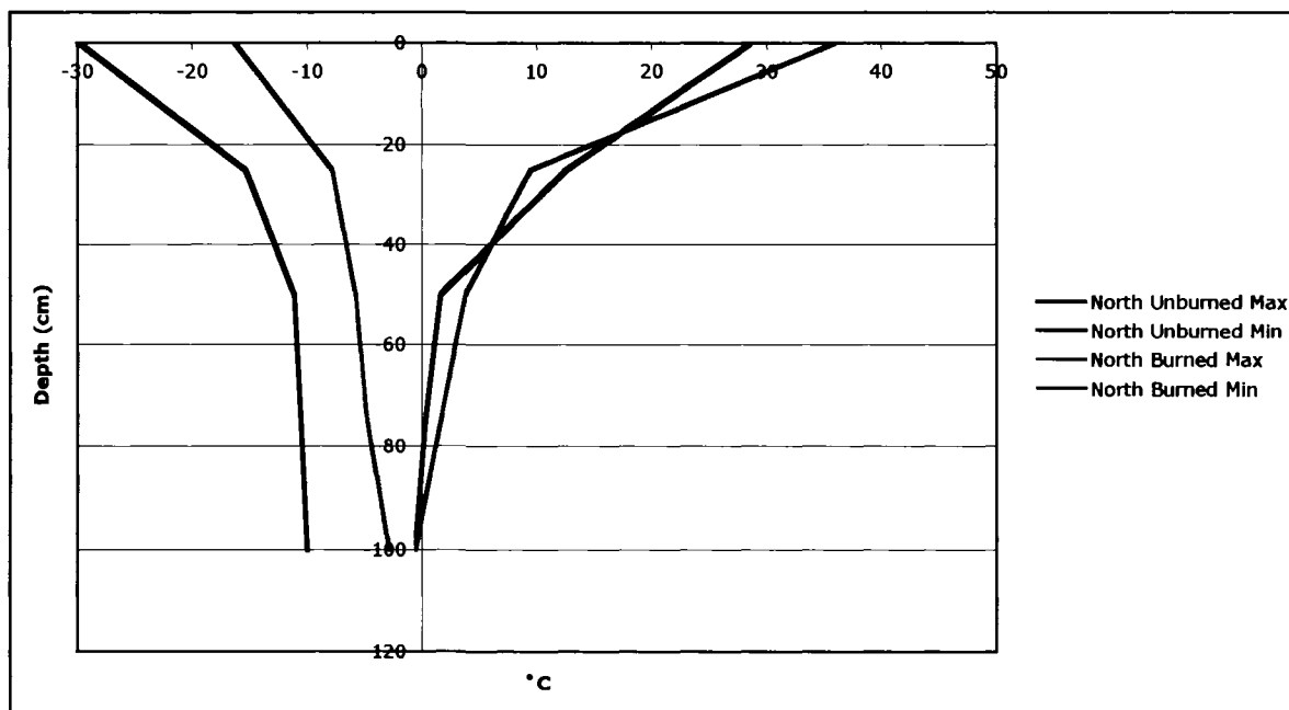
Figure 6.1: North ground temperature envelopes. June 29, 2005- July 1, 2006
