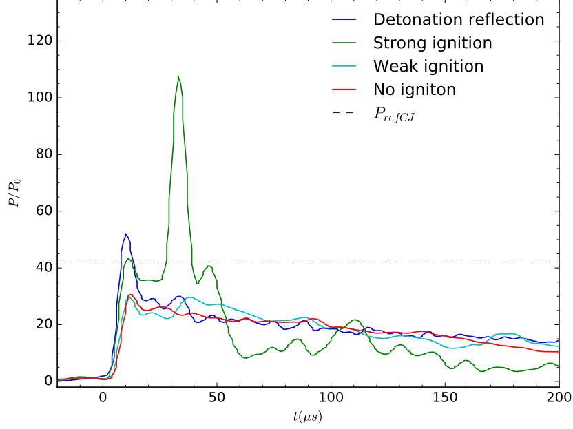
Fig. 2: Pressure profiles at the end wall recorded for the reflection of detonation and high-speed deflagration with strong ignition, weak ignition and no ignition.
