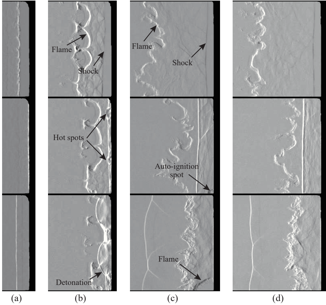
Fig. 1: Schlieren image sequence of (a) detonation reflection, and high-speed deflagration reflection with (b) strong ignition, (c) weak ignition and (d) no ignition at the end wall.
