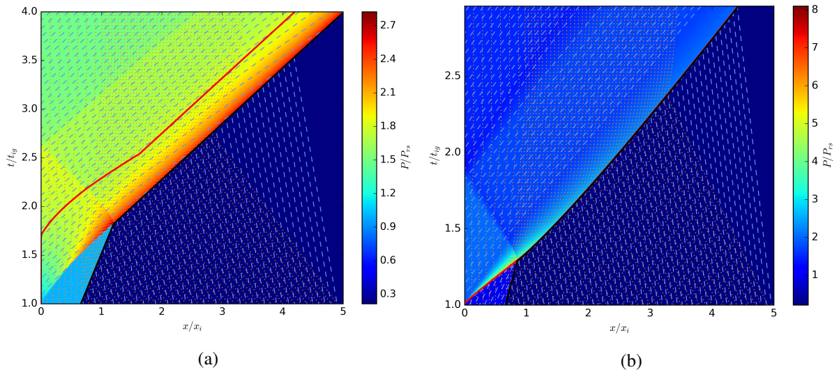
Fig. 9: Comparison of (a) t_{ig}/t_r = 3.87 and (b) t_{ig}/t_r = 387 on the flow field illustrated by the space-time diagram on top of the pressure profile, same legend as for Fig. 5.
