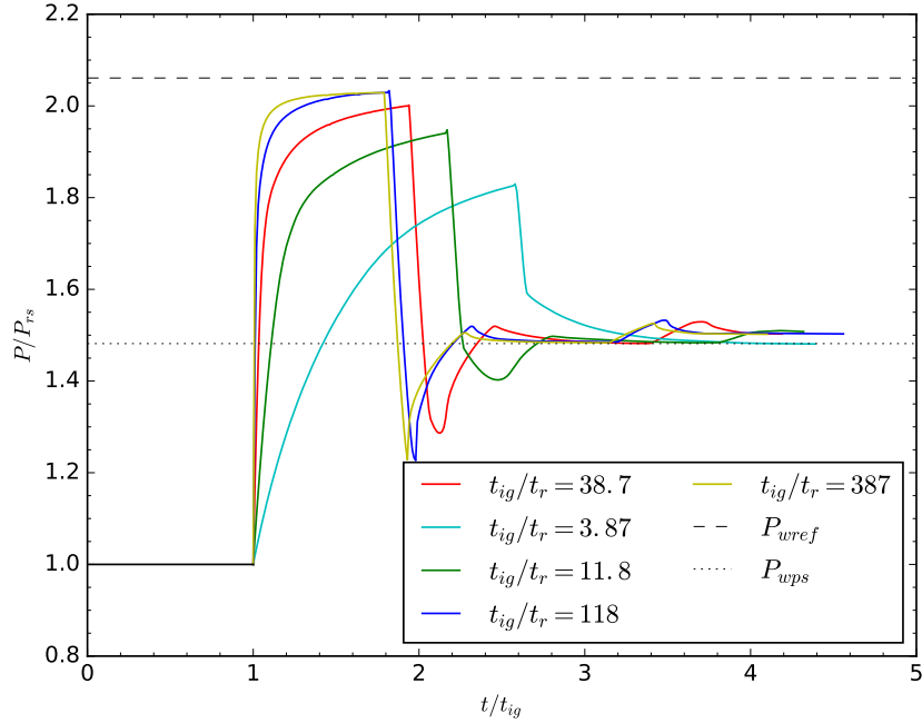
Fig. 8: Comparison for the influence of t_{ig}/t_r on pressure at the end wall as a function of time.
