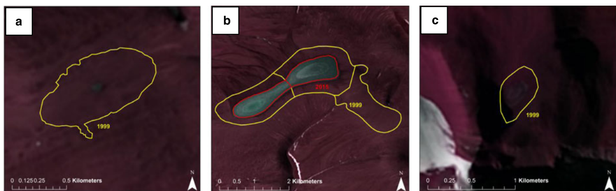
Fig. 7. Outlines from 1999 of small ice caps that lost 100% of their area: (a) G74438W81359N overlaid on Landsat 8 image from 12 July 2015 (#7 on Fig. 2a); (b) G76500W81203N (eastern-most basin) overlaid on Landsat 8 image from 14 July 2015 (#13 on Fig. 2a); and (c) G76132W82570N overlaid on Landsat 8 image from 12 July 2015 (#12 on Fig. 2a).
