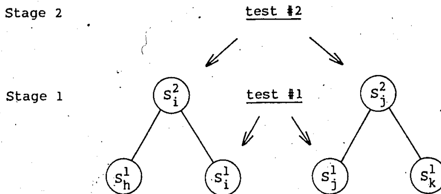
Figure 8.1 : Sequence of segment testings in a hierarchy.
