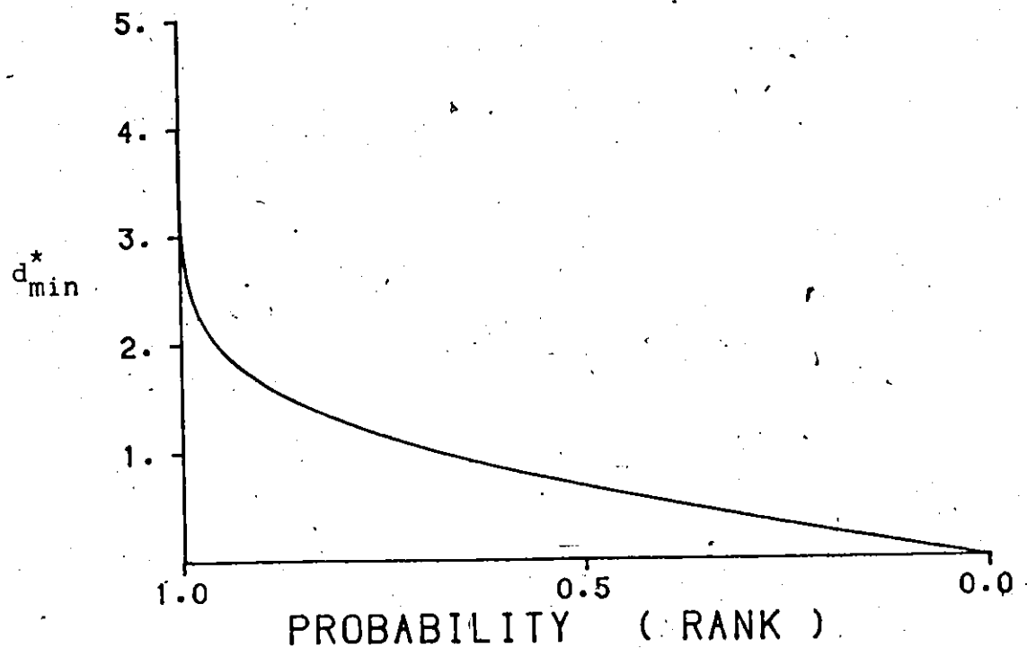
Figure 8.7 : The inverse function of P_{H0}(d_{\min}^*) .
