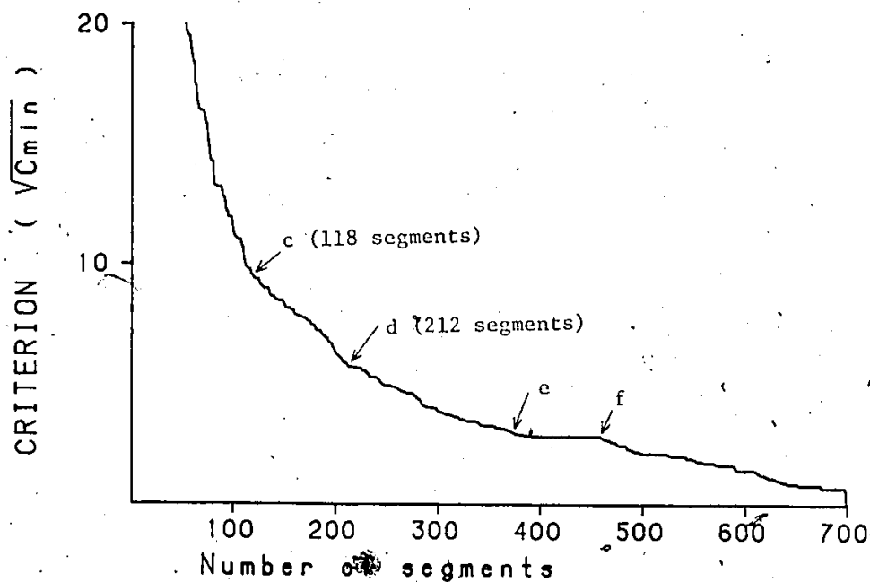
Figure 9.4 : Upper bound curve of the minimum step-wise criterion for different axis scales.
