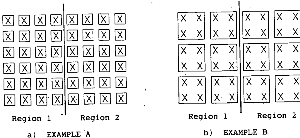
Figure 8.4 : Division of a two region picture into segments a) segments of one pixel, b) segments of four pixels.
