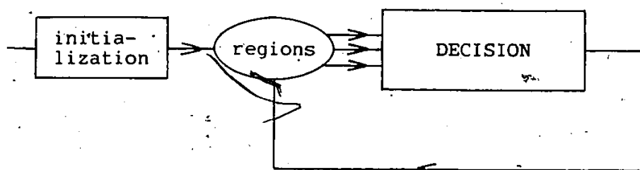
Figure 6.1 : Block diagram of a hierarchical step-wise optimization process. The region descriptions are first calculated by an initialization step, then they are updated after each decision or segment merger. The decision examines all region pairs and selects one for the merger.
