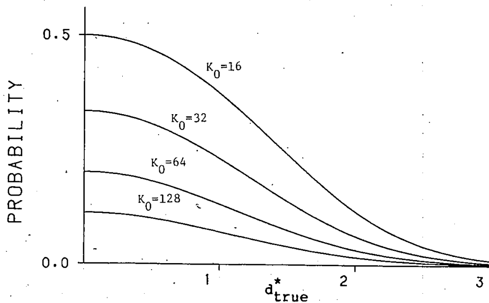
Figure 8.3 : Step-wise probability of error in function of d_{\text{true}}^* and for different values of K_0 and K_1 .
