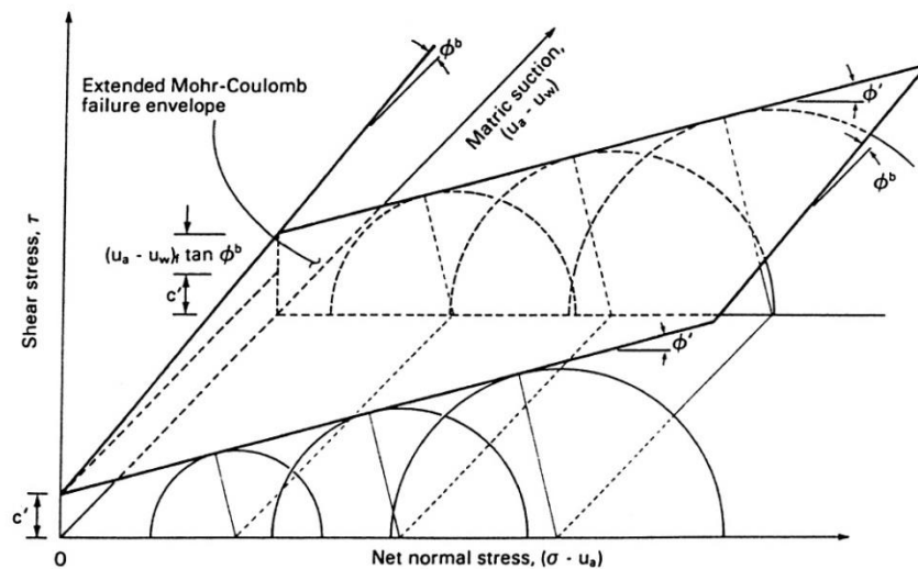
Figure 2.6 Extended Mohr-Coulomb failure envelope (Gasmo et al., 1999)
