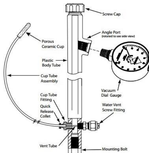
Figure 4.17 A schematic of commercial Tensiometer (Soilmoisture Equipment Corp. 2009)
