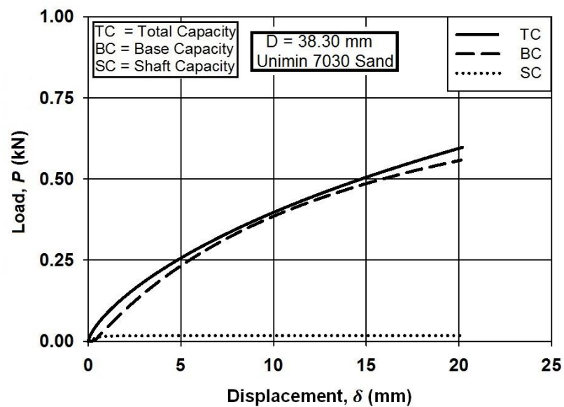
Figure 5.6 Measured load-displacement of single model pile D38.30 mm in Unimin 7030 sand under saturated condition.
