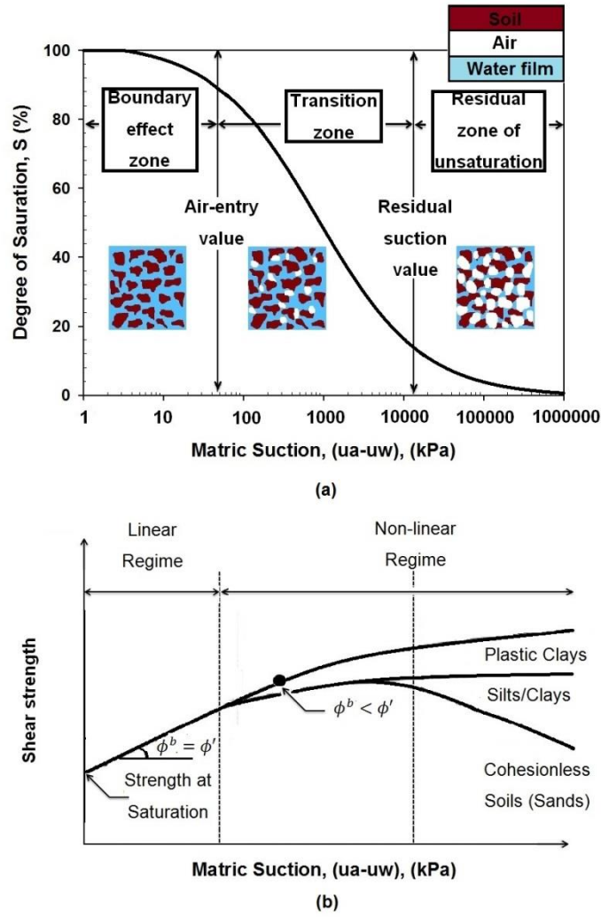
Figure 2.10 The relationship between the SWCC and shear strength of unsaturated soils (modified after Vanapalli, 2009)
