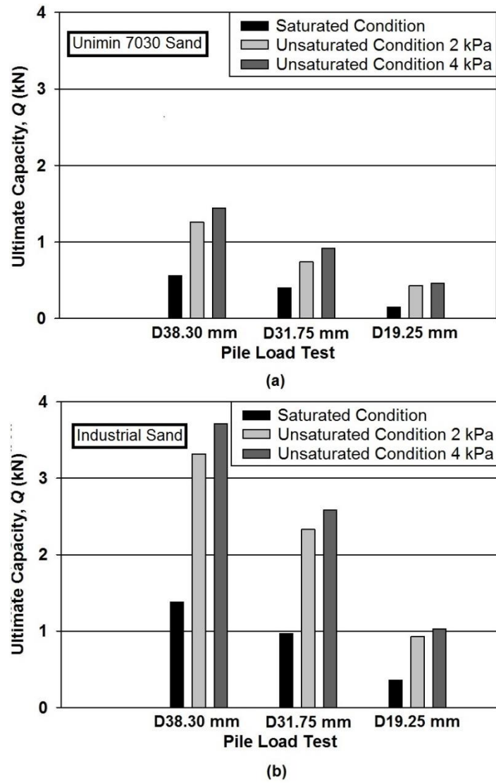
Figure 5.26 Comparison between the results of saturated and unsaturated (i.e., 2 and 4 kPa) pile load test for (a) Soil #1 and for (b) Soil #2.
