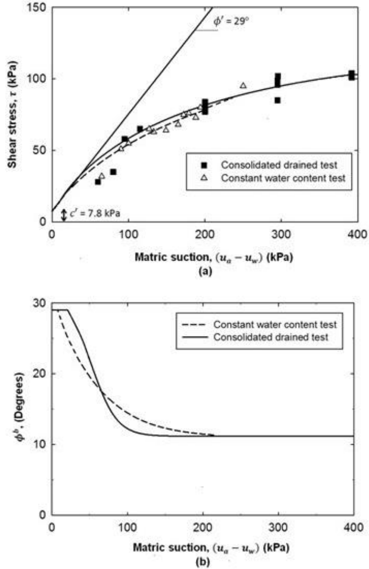
Figure 2.8 Non linearity in the failure envelope with respect to the matric suction, (u_a - u_w) : (a) curved failure envelopes for compacted Dhanauri clay at low density (data from Satija 1978), (b) corresponding \phi^b values (Fredlund et al., 1987)
