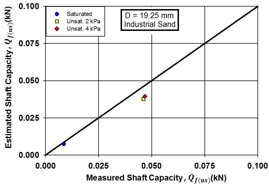
Figure 6.19 Comparison between the measured and predicted model pile shaft capacity for Pile D19.25 mm in Industrial sand
