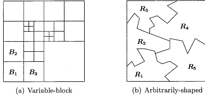
Fig. 5.4: Examples of region-based disparity-compensation
