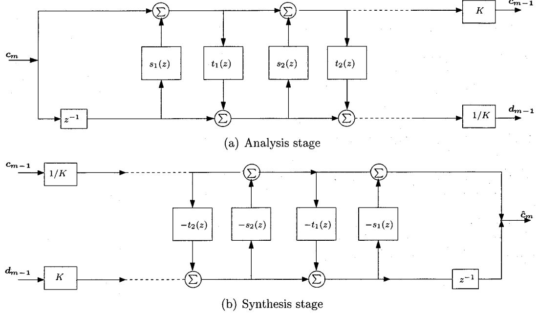
Fig. 2.5: Lifting-based implementation of a 1-scale DWT, previously shown in Fig. 2.2
