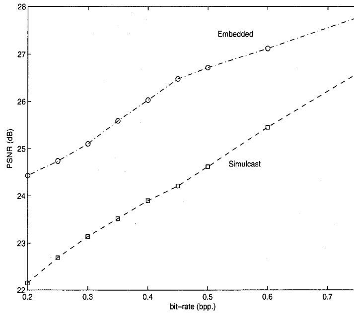
(a) PSNR values of reconstructed target images from the “ outdoors ” stereo-image pair, in independent (simulcast) ( \square ) and embedded ( \circ ) modes. “CDF-9/7” filters are used for transforming images.
