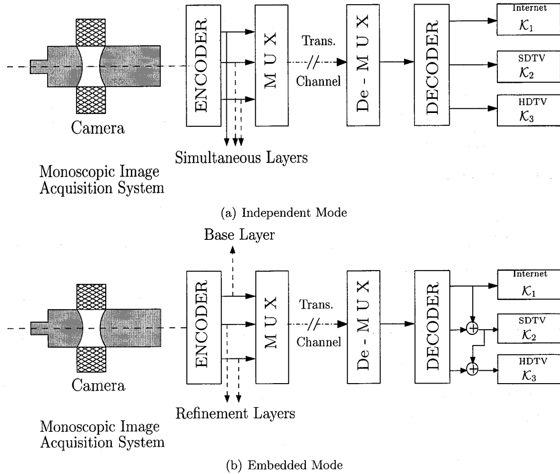
Fig. 1.1: QoS frameworks for transmission of monoscopic video content in (a) independent and (b) embedded simulcast modes. \mathcal{K}_1 , \mathcal{K}_2 and \mathcal{K}_3 represent bit-rates.
