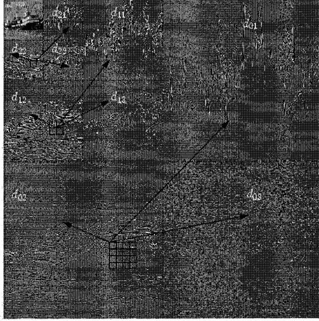
Fig. 3.3: Intra-scale relationship between wavelet coefficients in any given subband. Coefficients have been scaled for display purpose. The direction of arrows indicate that all coefficients at a particular scale are examined before a coefficient can be deemed significant.
