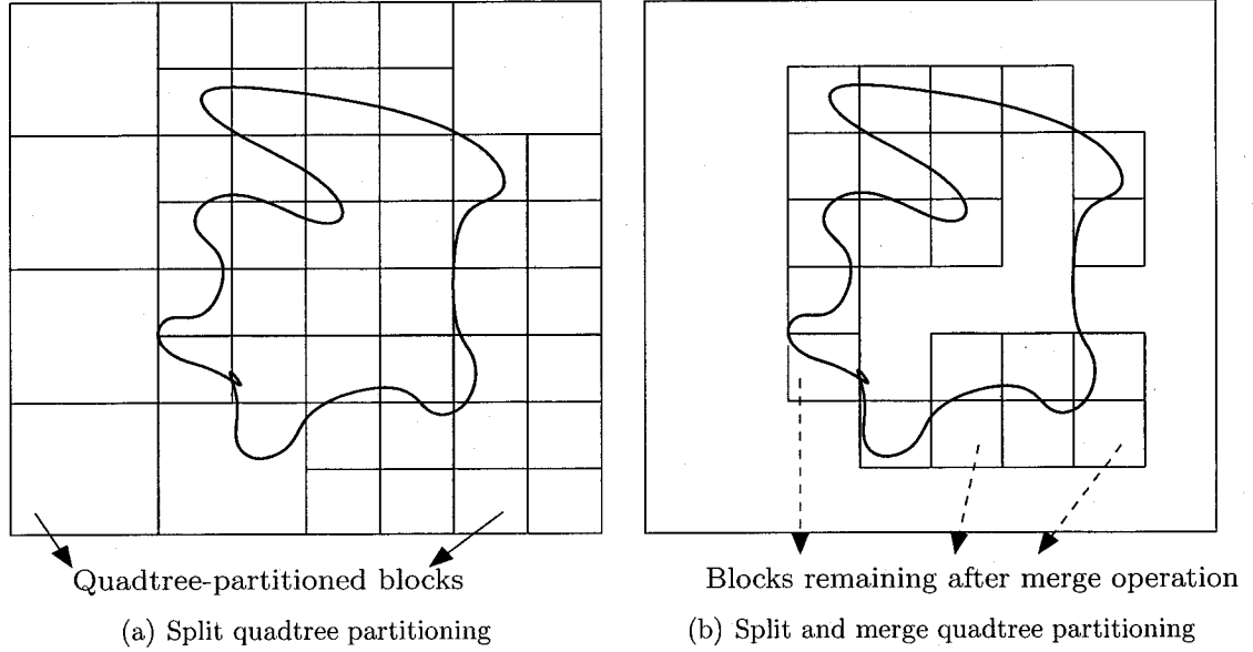
Fig. 5.5: Representative examples of quadtree-partitioning schemes
