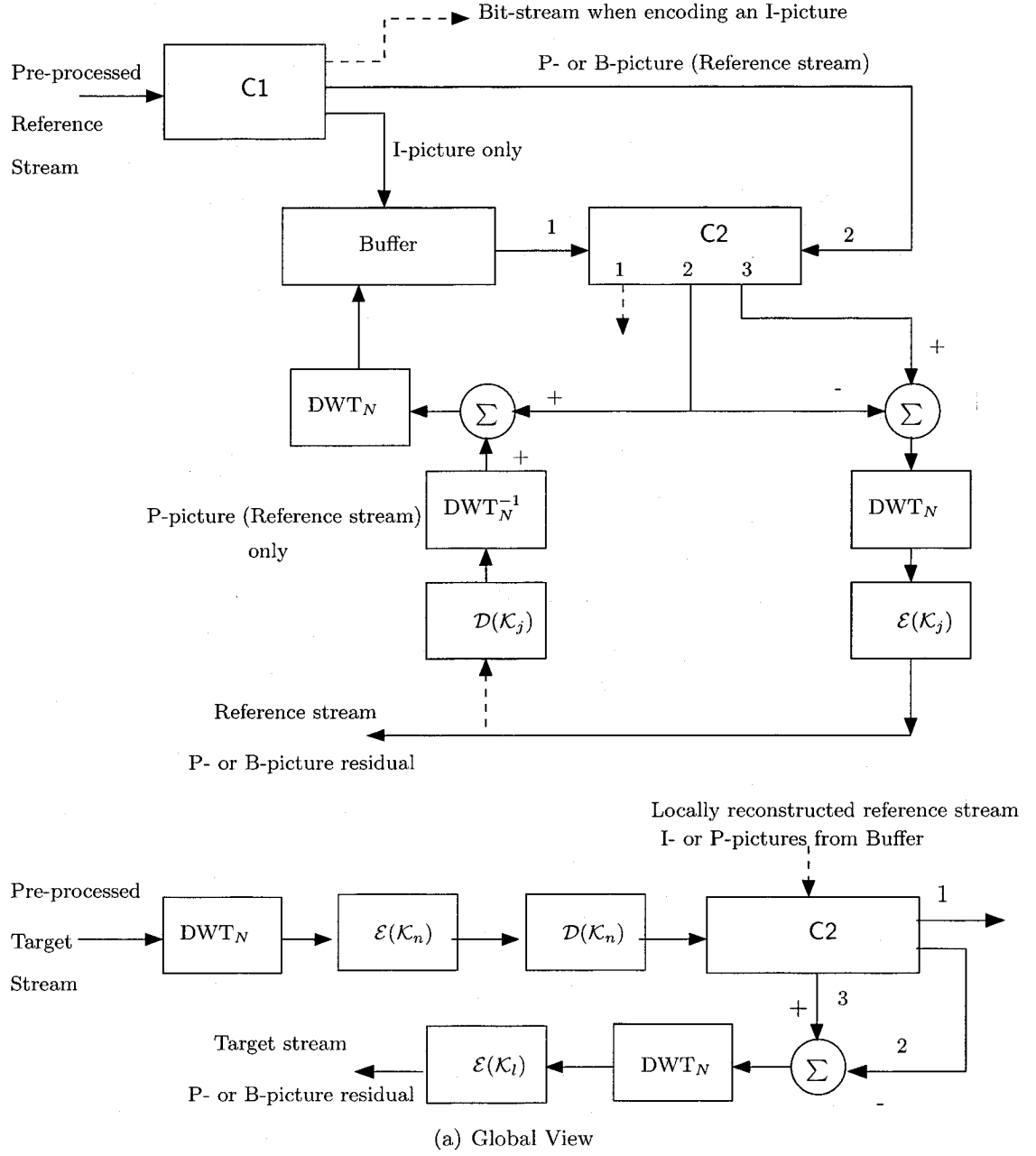
Fig. 7.3: Fundamental Structure employed when encoding different pictures of a stereoscopic moving-image sequence at the highest spatial resolution.
