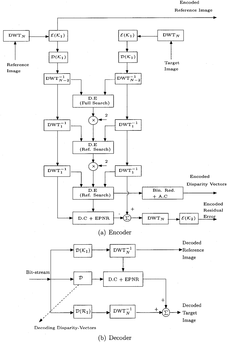
Fig. 5.1: Block diagram of proposed codec, with SNR-scalability, at a specified spatial-resolution.
