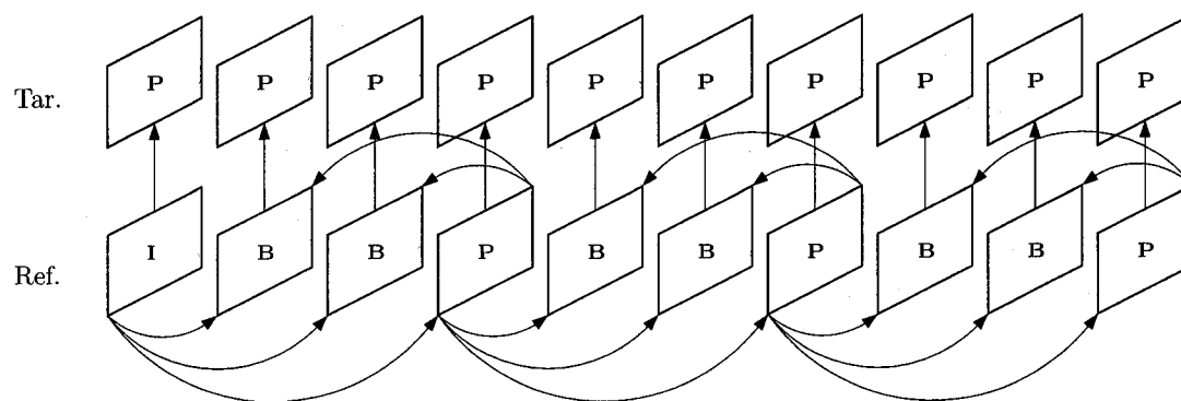
Fig. 6.3: Disparity-compensated multiview picture hierarchy for encoding stereoscopic imagery.
