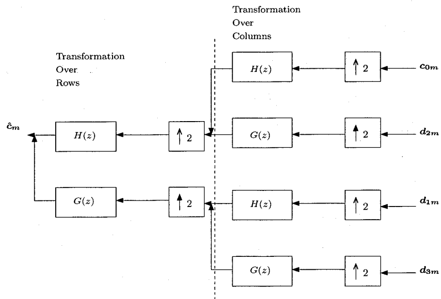
(b) Synthesis-stage
