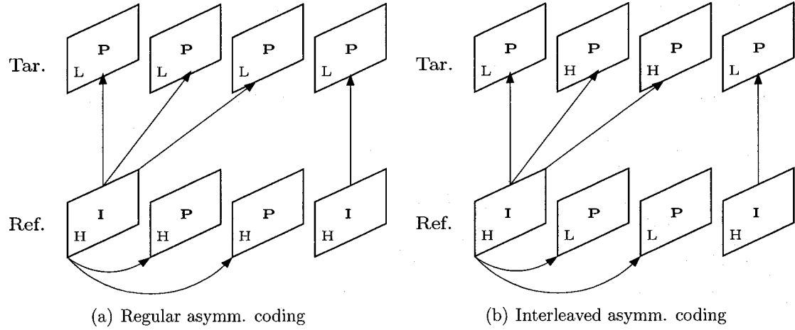
Fig. 7.9: Modified asymmetrical coding frameworks for stereoscopic moving-images. “H” and “L” indicates overall high and low bit-rates when encoding reference and target pictures.
