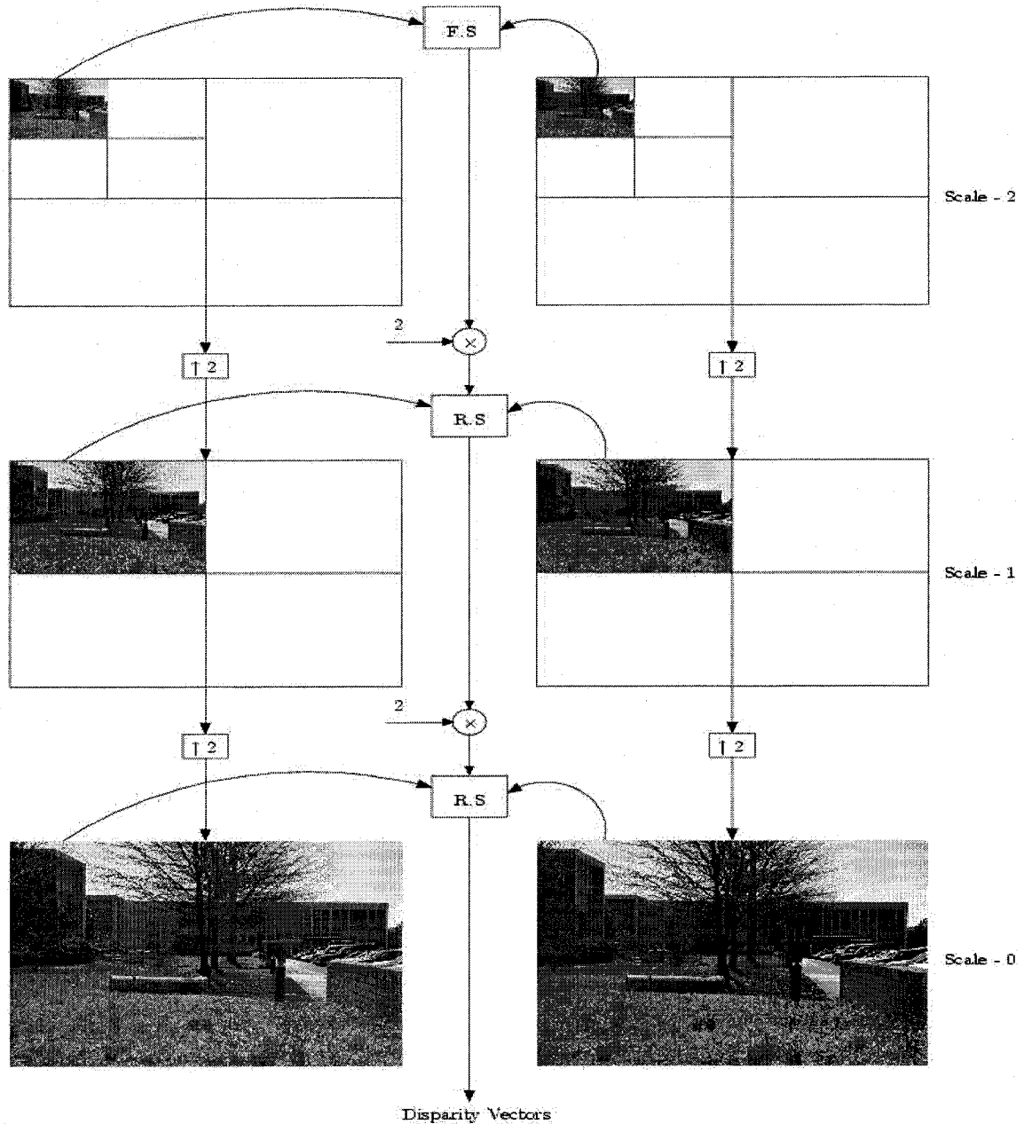
Fig. 2.7: Hierarchical disparity-vector estimation, in a DWT framework. \uparrow 2 indicates a dyadic upsampling performed in a 2-D separable DWT. Disparity-estimation is performed between the all low-pass subband at each scale. Disparity-vectors from coarse-scales are scaled by a factor of two, when moving to a finer scale. A similar strategy can be used when estimating motion-vectors.
