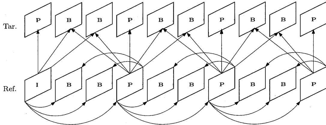
Fig. 7.1: Proposed contiguous picture hierarchy, used in stereoscopic moving-image encoding (GOP = 10)
