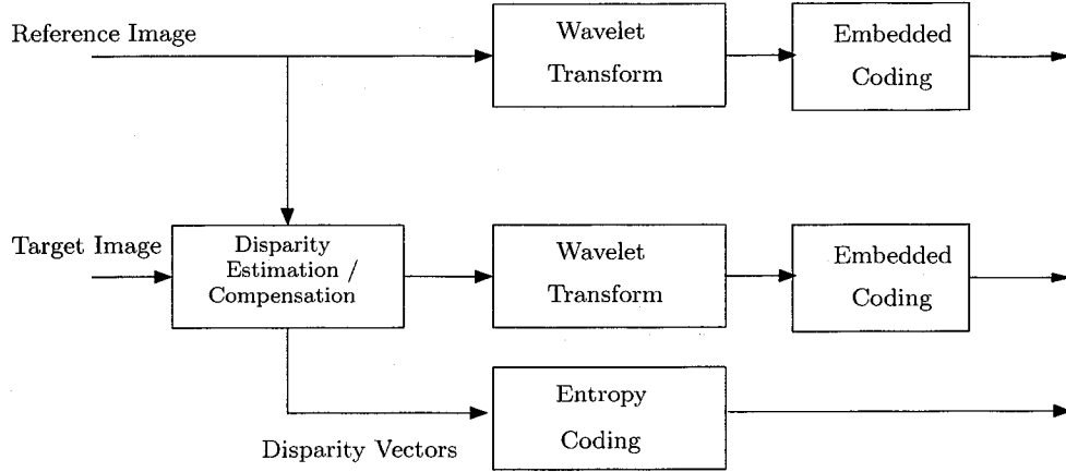
(a) Open-loop (CONCOD) disparity encoder structure
