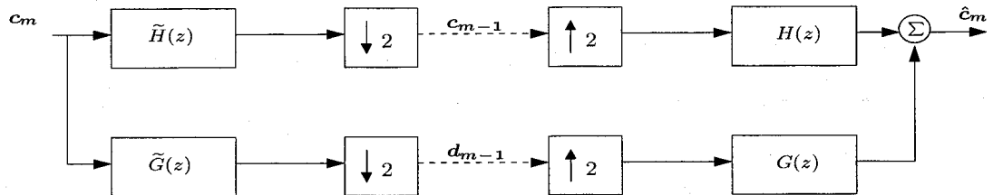
Fig. 2.2: 2-channel filter-bank.
