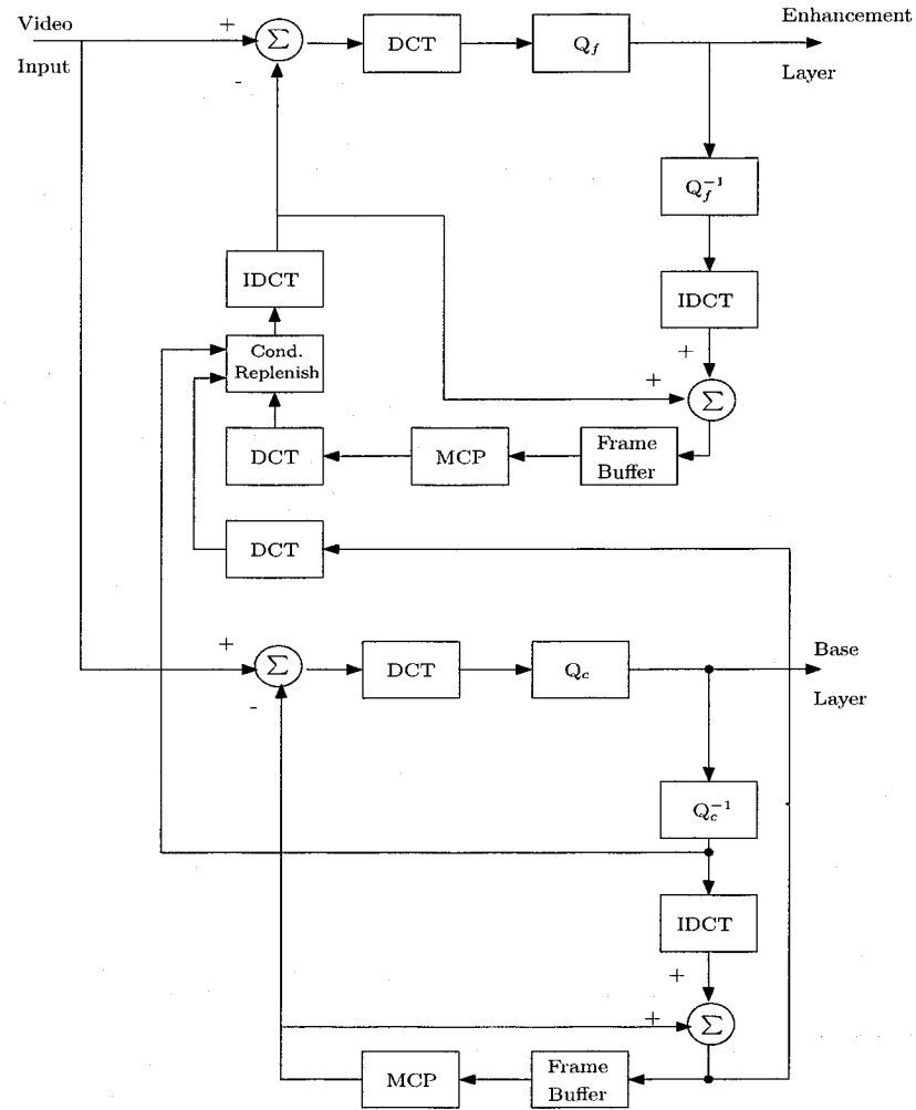
Fig. 6.6: Two-loop, DCT-based SNR-scalable encoder, proposed by Arnold, Frater and Wang.
