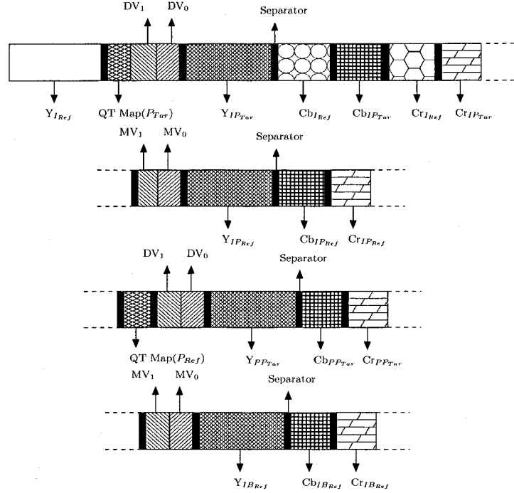
Fig. 7.4: Bit-streams of various components when encoding a stereoscopic moving-image sequence at a specific spatial resolution. e.g., Y_{IP_{Tar}} indicates the Y-component of the disparity compensated residual image between a reference I-picture and a target P-picture. QT Map(.) indicates the quadtree map for the picture that is being estimated. DV_X , MV_X indicates disparity- and motion-vectors as per notations previously introduced in Chapter 2.
