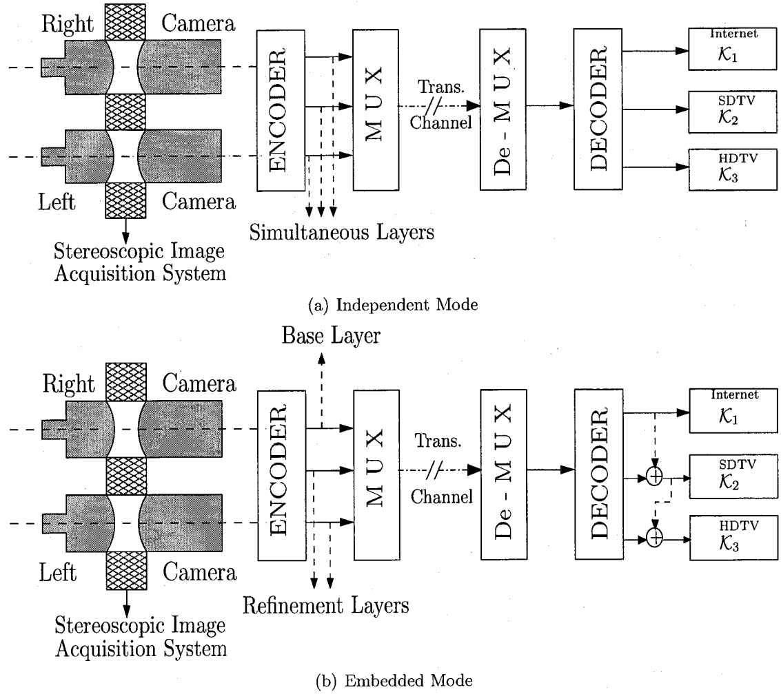
Fig. 1.2: QoS frameworks for transmission of stereoscopic video content in (a) independent and (b) embedded simulcast modes. \mathcal{K}_1 , \mathcal{K}_2 and \mathcal{K}_3 represent bit-rates.
