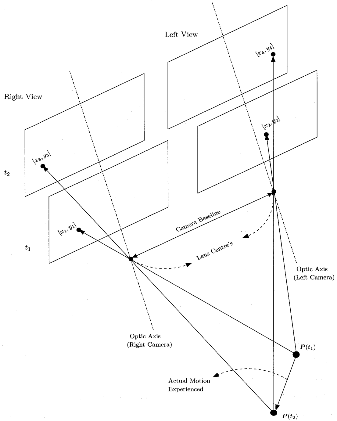
Fig. 2.1: Schematic of a Binocular Stereoscopic Imaging System. Proper optical arrangements are incorporated so as to prevent inversion of images. Both camera's are assumed to be stationary.
