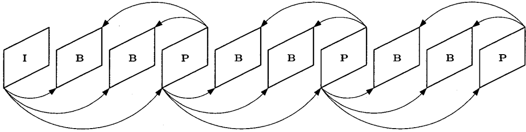
Fig. 6.1: Encoding and display hierarchy of contiguous pictures in a, MPEG-2 compliant, monoscopic moving-image sequence (GOP = 10).
