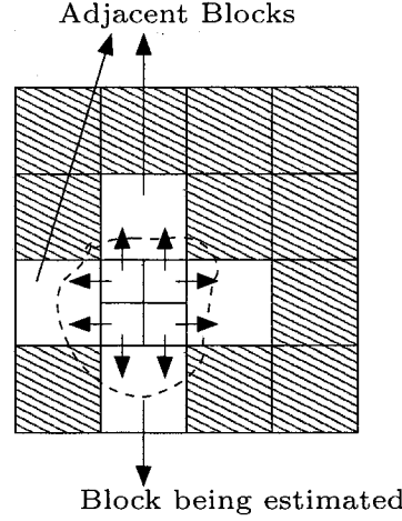
Fig. 5.3: Overlapped-block disparity compensation (OBDC). All blocks must have same dimensions. Different regions of the block (enclosed within the dashed line) are estimated from different neighbours.
