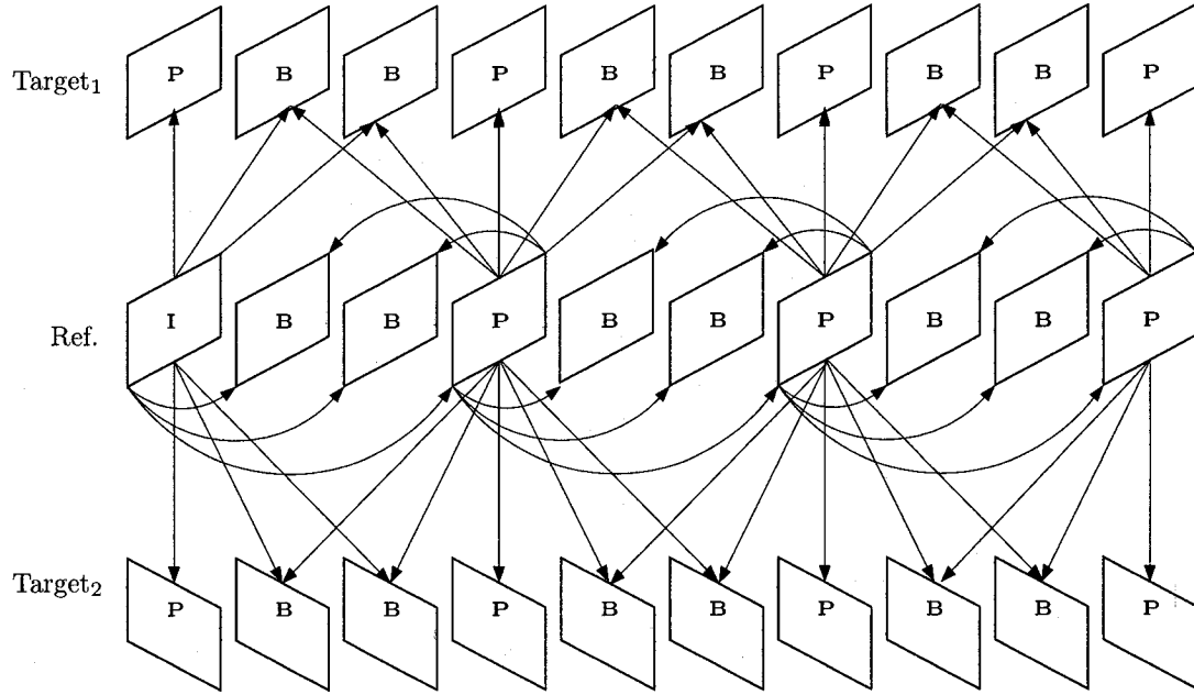
Fig. 7.2: Proposed contiguous picture hierarchy, when used in multi-view (i.e., more than 2 views) moving-image encoding (GOP = 10)
