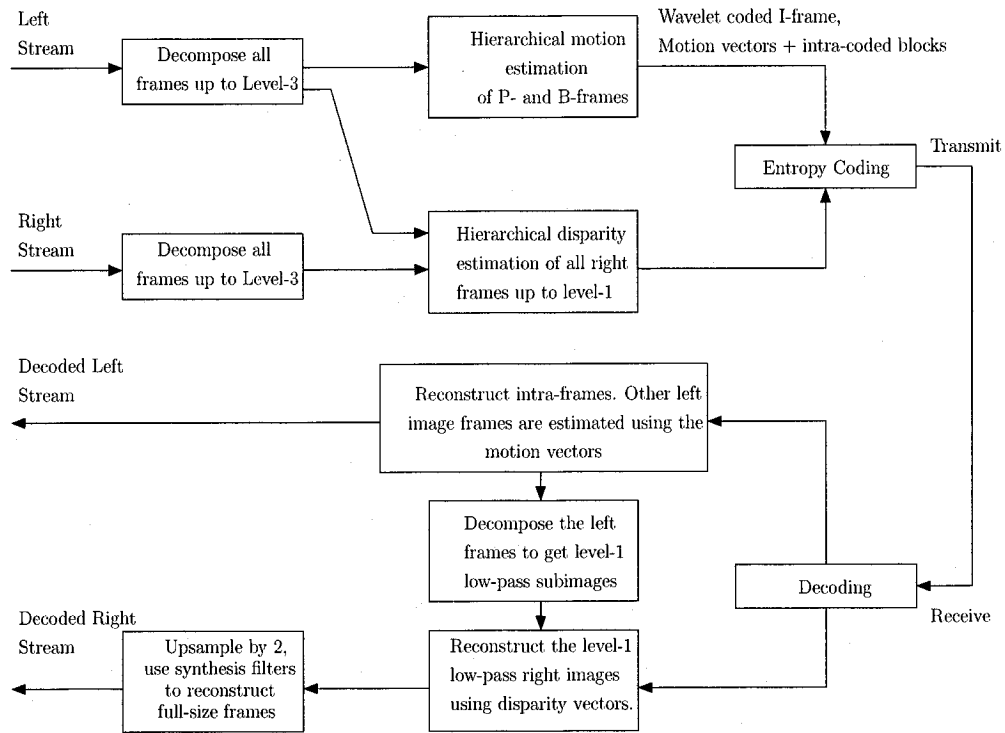
Fig. 6.4: Stereoscopic moving-image codec structure proposed by Sethuraman, Siegel and Jordan
