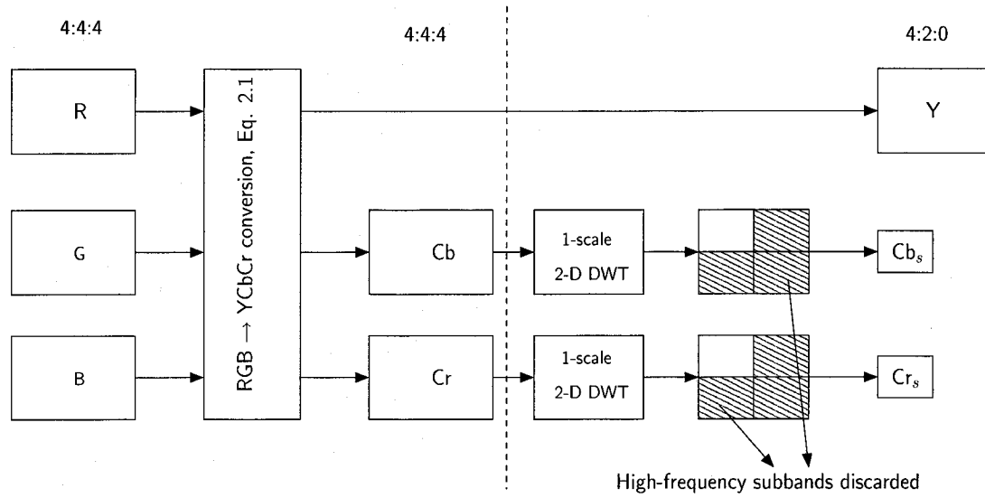
Fig. 5.14: 4:4:4 RGB to 4:2:0 YCbCr conversion. Cb_s and Cr_s represent downsampled versions of Cb- and Cr-components.
