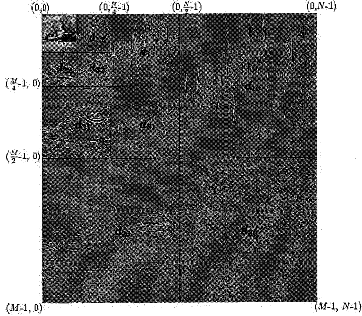
Fig. 2.4: 3-scale wavelet decomposition of a 2-D image (having dyadic dimensions), using Mallat's algorithm. Image dimensions are (M, N) .
