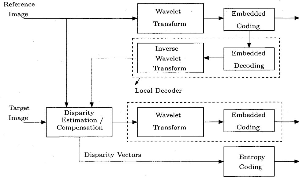
(b) Closed-loop disparity encoder (CLDC) structure
