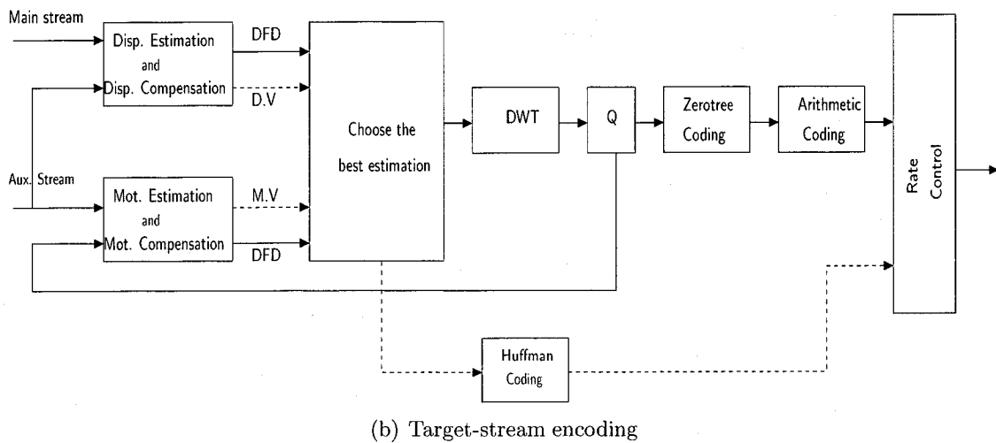
Fig. 6.5: Stereoscopic moving-image encoding structure proposed by Thanapirom, Fernando and Edirisinghe
