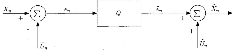
Fig. 4.2: Residual error quantization
