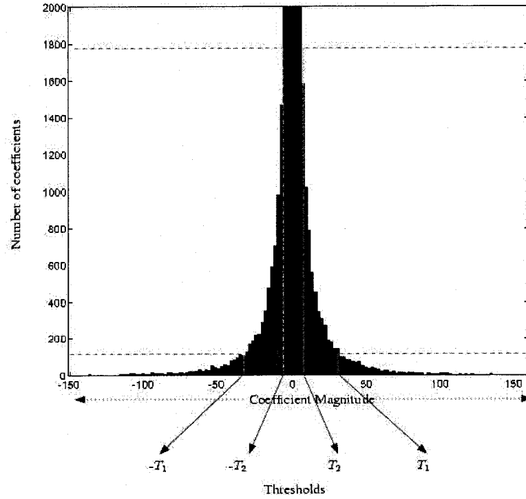
Fig. 3.1: Progressive image coding of wavelet-transformed coefficients. The x-axis indicates magnitudes of coefficients. |T_1| > |T_2| . The y-axis indicates the number of coefficients satisfying a “greater than threshold” criterion.
