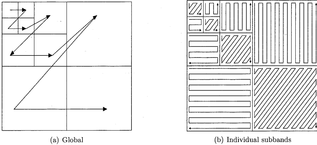
Fig. 3.6: Scan order employed in accumulating coefficients.
