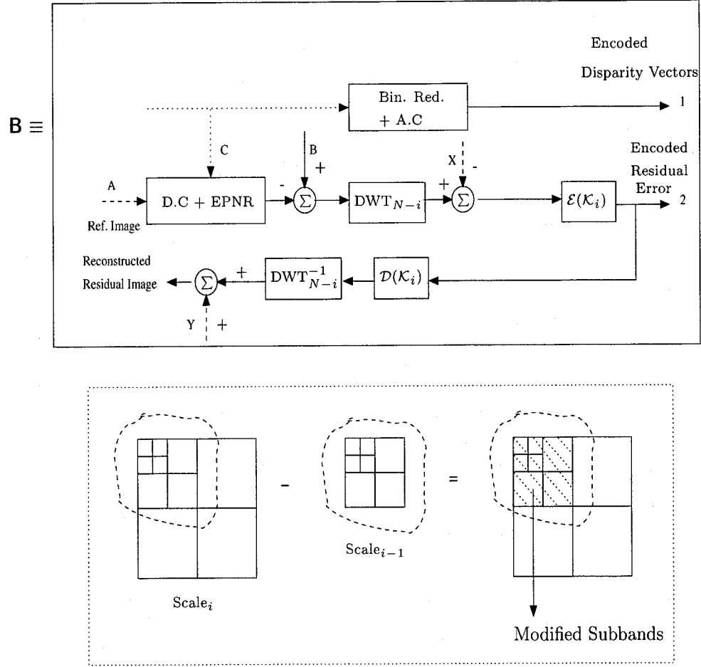
(b) Expansion of B and reduced energy residual generation
