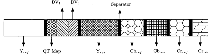
Fig. 5.15: File structure of an encoded color stereo-image pair (independent simulcast mode).
