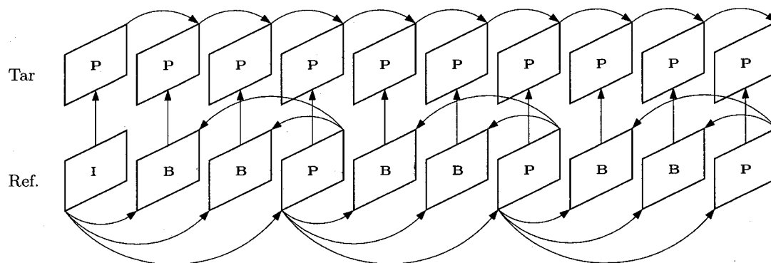
Fig. 6.2: MPEG-2 compliant multiview picture hierarchy for encoding stereoscopic imagery.
