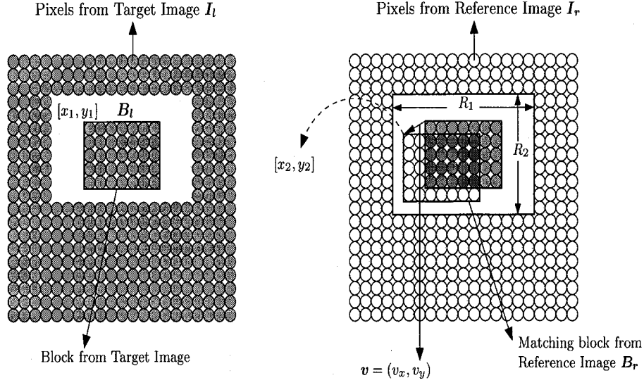
Fig. 2.6: Block disparity- or motion-vector estimation
