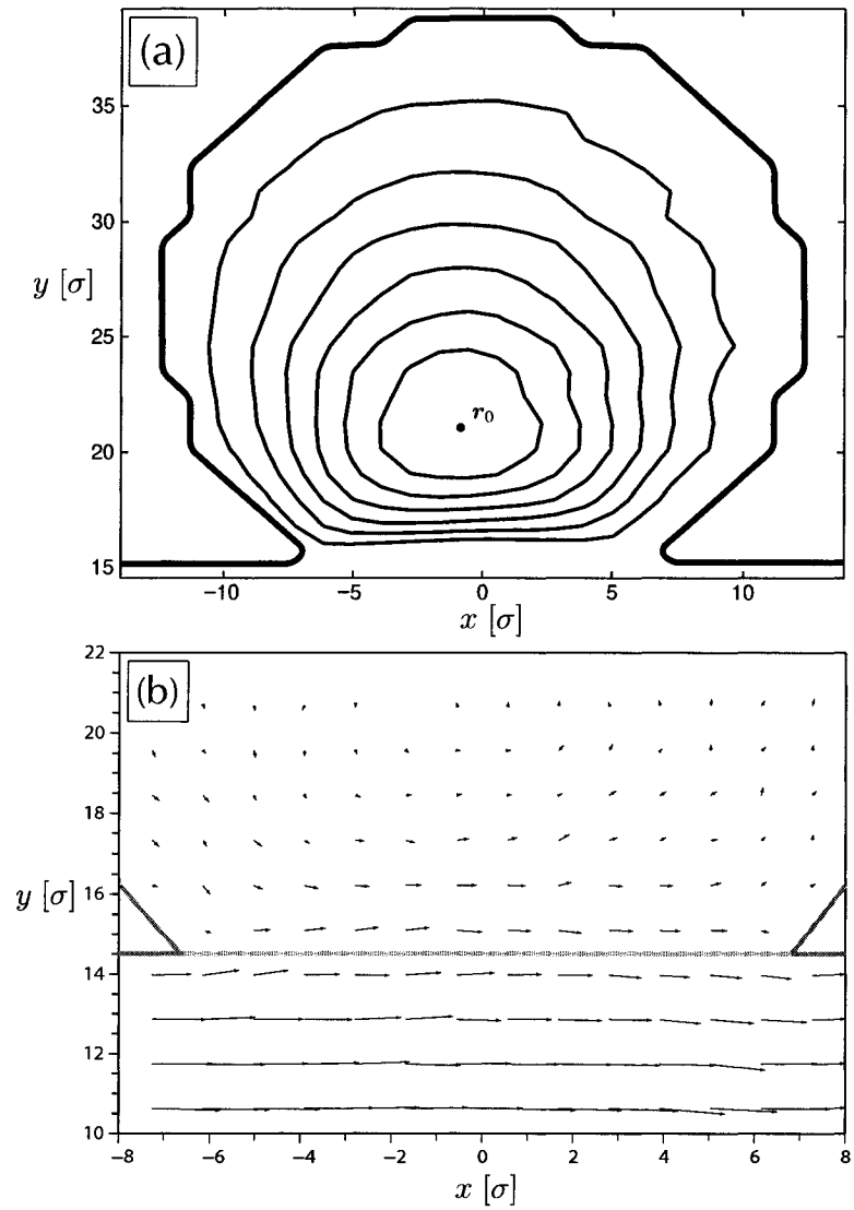
Fig. 6 Time-averaged velocity field and streamlines computed from the velocity field for c_{fw} = 0.5 and g = 0.025 \sigma/\tau^2 using scheme B. (a) shows the rotation of the fluid in the cavity. Closed streamlines, of course, represent circulation of fluid particles. The thick black line represents the approximate location of boundary between the fluid and the cavity walls. (b) shows the continuity of velocity across the coupling region. The solid gray lines denote the approximate location of the fixed wall and the dotted gray line shows the coupling region between the cavity and the channel.
