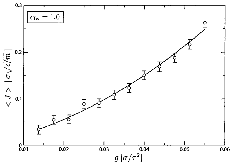
Fig. 7 Average angular momentum per particle in the cavity for various accelerations with no modification of wall-fluid interactions (i.e., c_{fw} = 1 ). As expected, the average angular momentum of the fluid inside the cavity increases as a function of g . The empirical fit \langle \bar{J} \rangle = ag(1 + g/g_0) is shown with parameters a = 1.77 \pm 0.13\sigma \sqrt{\epsilon/m} and g_0 = 0.0353 \pm 0.0026 \sigma/\tau^2 . The latter value is thus an estimate of the critical acceleration which indicates the onset of nonlinearity.
