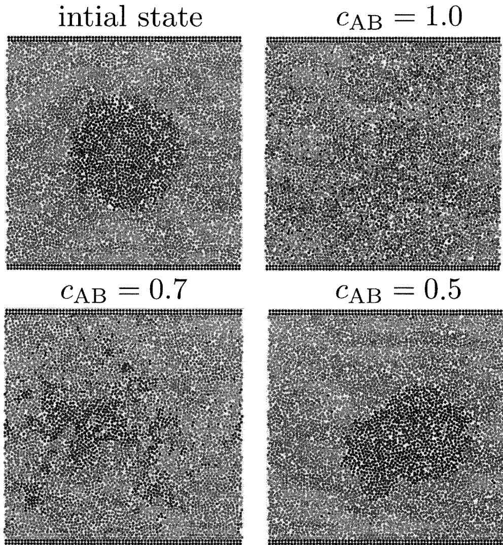
FIGURE 1.8 Molecular Dynamics simulations of two fluid species ( A and B , dark and light gray respectively) and fixed wall particles (shown in black) in a 75 by 75 particle channel. There are periodic boundary conditions along the x direction, all particles interact with the LJ potential, the densities are all \rho = 0.8/\sigma^2 and the temperature is kept constant at k_B T = 1 \epsilon . All interactions except between unlike fluid species has the constant c = 1 and we set c_{AB} \leq 1 . The first frame shows the initial state for all simulations and the other frames are the final state for various simulations. We see that as c_{AB} is decreased from a value of one, the two fluid species become less miscible until there is nearly no mixing between them at all.
