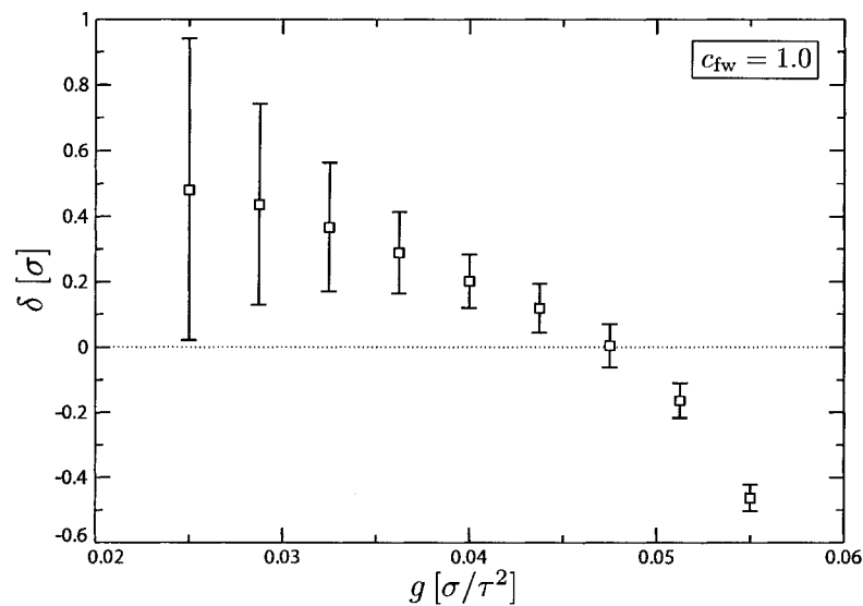
Fig. 5 Slip length \delta as a function of applied acceleration g using the linear extrapolation method. The parameter c_{fw} is always constant at a value of 1.0. The quadratic method yields nearly identical values so we have left them off this figure for simplicity. As expected, the slip length becomes more negative as g increases. When g \rightarrow 0 the slip length corresponds to the position of the first layer of fluid near the wall.
