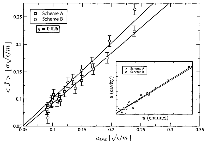
Fig. 10 The dependence of average angular momentum \langle \bar{J} \rangle from the MD simulations on average forcing velocity ( u_{\text{avg}} = (u_{\text{chan}} + u_{\text{cav}})/2 ). The acceleration is constant at g = 0.025 \sigma/\tau^2 and the wall fluid interaction ranges from c_{fw} = 0.5 to c_{fw} = 1.0 . The fit is linear with zero intercept: \langle \bar{J} \rangle = \alpha u_{\text{avg}} with proportionality constants \alpha_A = 0.92 \pm 0.01 and \alpha_B = 1.02 \pm 0.01 . The inset shows the linear relationship between u_{\text{cav}} and u_{\text{chan}} . The slopes are 0.63 \pm 0.01 for scheme A and 0.62 \pm 0.01 for scheme B.
