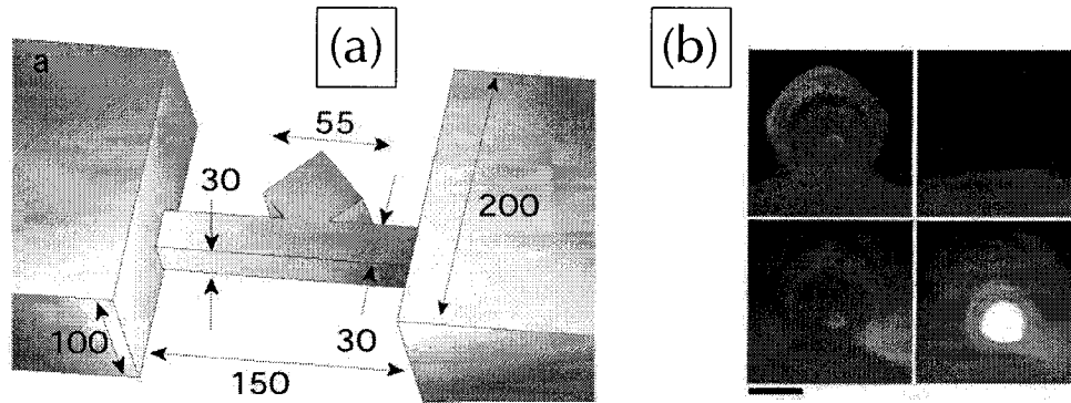
FIGURE 1.1 (a) System used by the Chiu group to explore fluid rotation in a microcavity. A pressure difference is created between the two large reservoirs which generates a Poiseuille flow in a narrow channel (all dimensions are in \mu\text{m} ). A small cavity is coupled to the channel to allow transfer of momentum (via viscous coupling at the channel-cavity interface) between it and the channel. (b) Streamlines in the rotating cavity fluid (visualized using fluorescent beads). The scale bar is 25 \mu\text{m} . Reprinted by permission from MacMillan Publishers Ltd: Nature [4], copyright 2003.
