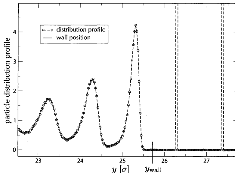
Fig. 2 Particle distribution profile across the channel. Note the presence of the two fixed layers of wall particles at y = 26.27 \sigma and y = 27.39 \sigma as well as the layering of the fluid induced by the rigid wall (layers shown peak at y = 23.24 \sigma , y = 24.30 \sigma and y = 25.31 \sigma ). The distribution profile is normalized such that it goes to 1 in the central region of the channel (about y = 0 , see Fig. 3). The geometric position of the wall, denoted by y_{\text{wall}} , is shown in the figure at y = 25.71 \sigma .
