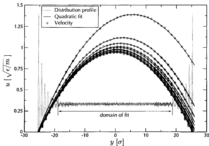
Fig. 3 Equilibrium velocity profiles for various levels of interaction between the fluid and the wall particles (with g = 0.025 \sigma/\tau^2 ). Included in the figure is the particle distribution profile (arbitrary units) for the c_{fw} = 1.0 case. The domain of the fit is limited to where this density profile is approximately constant and the fluid should resemble bulk conditions. For these simulations the system size is L = 111.8 \sigma and W = 55.9 \sigma and there is no cavity (just plain walls at \pm y_{\text{wall}} .)
