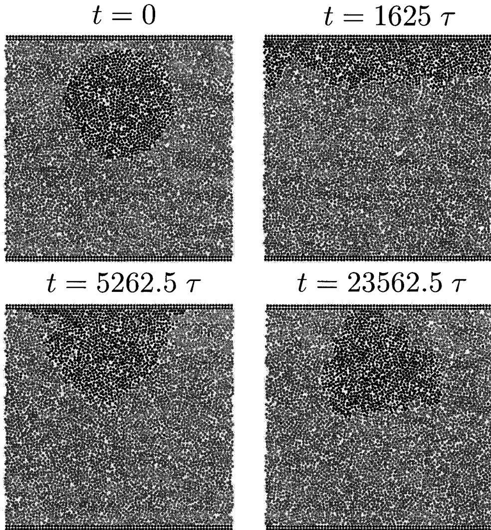
FIGURE 1.9 Molecular Dynamics simulations of two fluid species ( A and B , dark and light gray respectively) and fixed wall particles in a 75 by 75 particle channel. There are periodic boundary conditions along the x direction, all particles interact with the LJ potential, the densities are all \rho = 0.8/\sigma^2 and the temperature is kept constant at k_B T = 1 \epsilon . The fluids are immiscible with c_{AA} = c_{BB} = 1 and c_{AB} = 0.5 . The wall has a preferential attraction to fluid A with the parameters: c_{wA} = 1.2 and c_{wB} = 0.8 . The frames show different points in time during the simulation. We see that the droplet of fluid type A finds the wall through random motion and proceeds to wet it. The final state is fluid A completely adsorbed to the wall and wrapping around the periodic boundary conditions.
