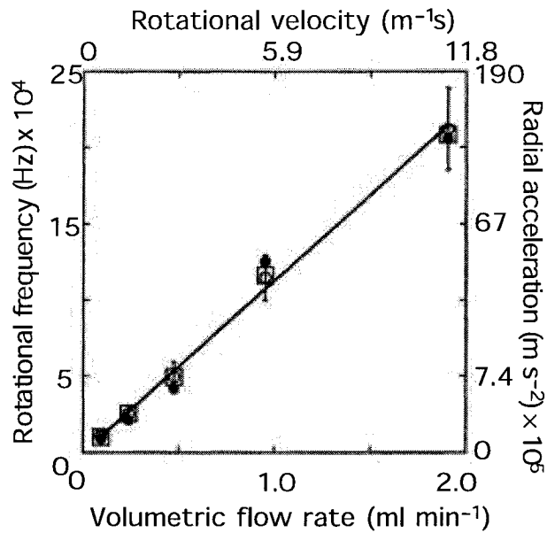
FIGURE 1.2 Results demonstrating a linear dependence of radial acceleration in the microcavity with flow rate in the channel. Reprinted by permission from MacMillan Publishers Ltd: Nature [4], copyright 2003.
