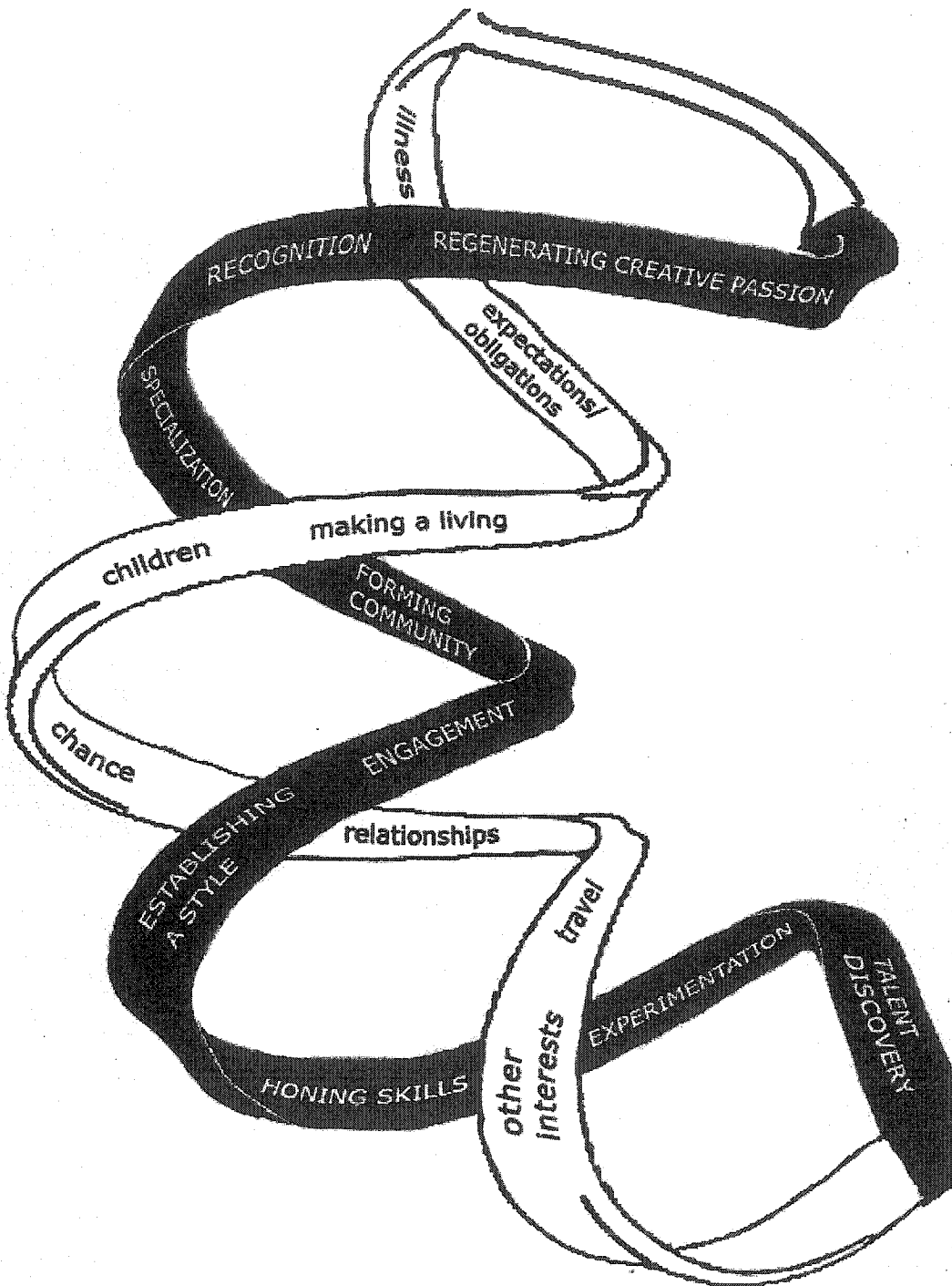
Figure 2 A model of women's creative talent development
