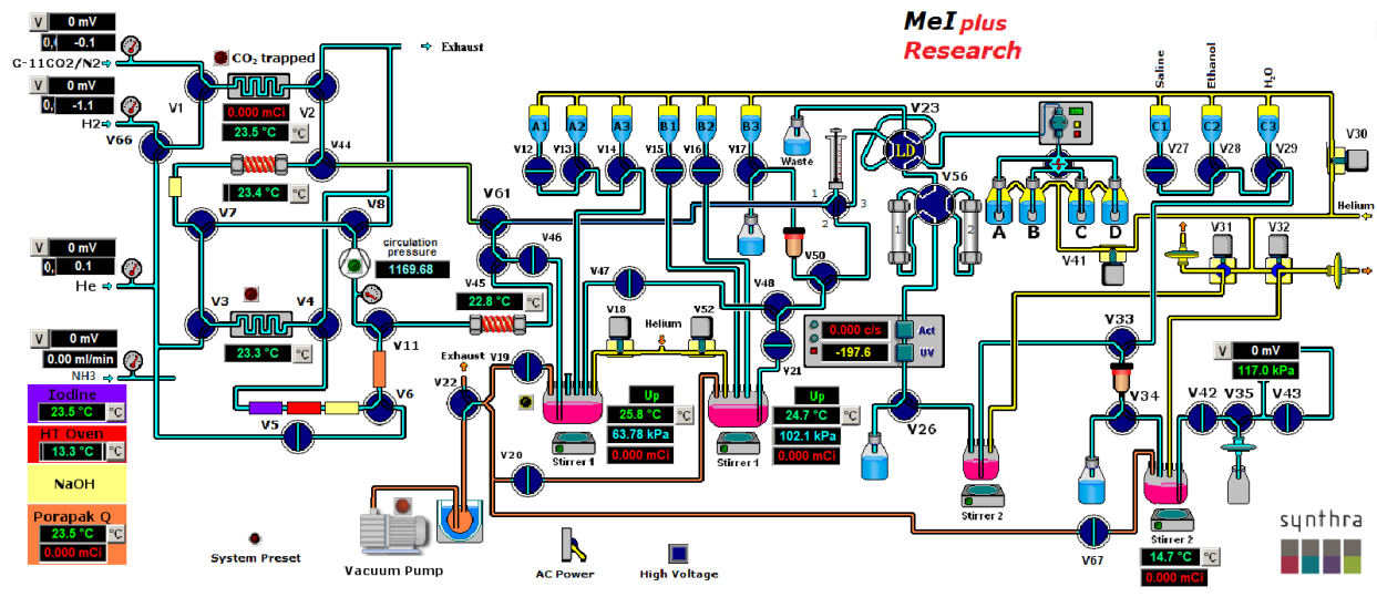
Figure S1. Synthra MeI plus Research apparatus scheme.
