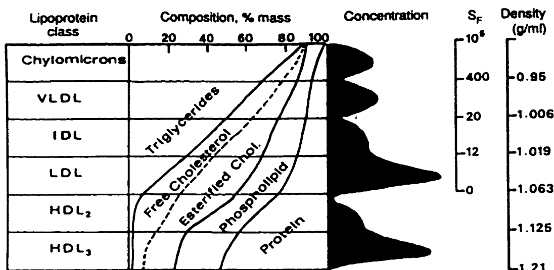
Figure I-2 Classification and chemical composition of lipoproteins using equilibrium ultracentrifugation.
