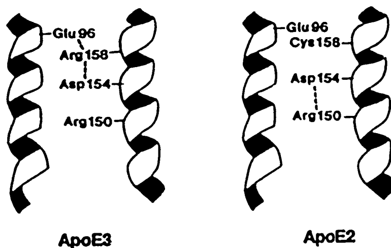
Figure I -17 Comparison between the apoE2 and E3 structures.
