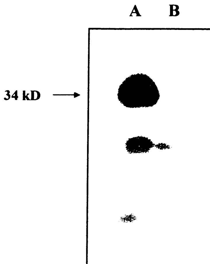
Figure V-7 Immunodepletion of apoE-containing LDL lipoproteins from crude isolates.- This autoradiogram represents an SDS PAGE western blot of 20 ug of crude LDL in lane A, run along side of 20 ug of an apoE-depleted LDL preparation shown in lane B. The blot was detected with the radiolabeled mAb 6C5. A unique major band was consistently observed at 34 kDa for the crude LDL preparations, indicating a substantial amount of apoE associated to the isolated LDLs. In contrast, no band of equivalent size was observed in the apoE immunodepleted preparation, indicating an efficient removal of the apolipoprotein from the preparation. The smaller, less abundant protein, which appears in both lanes A and B, presumably represents small quantities of the 22 kDa degradation product of apoE.
