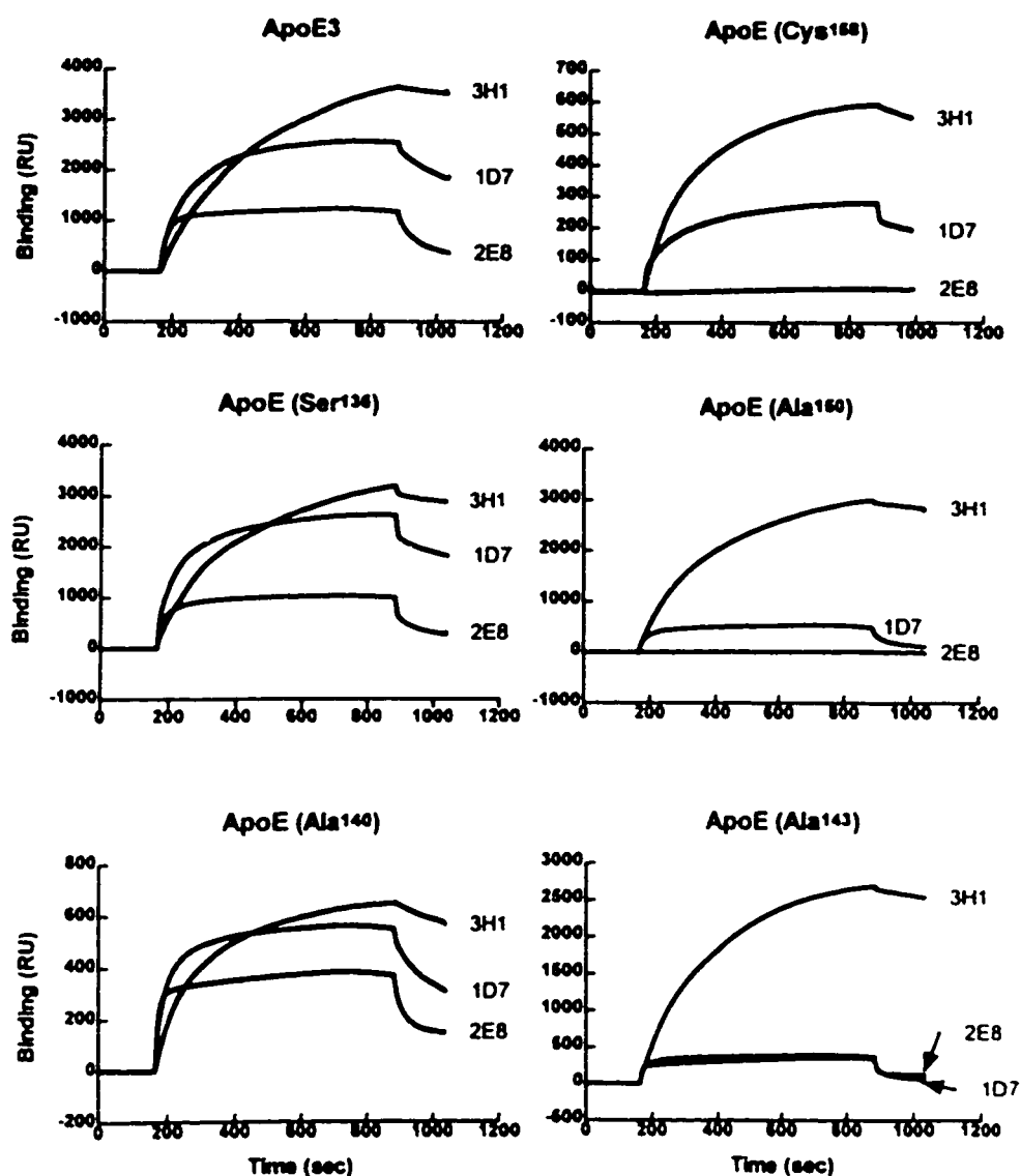
Figure II-6. Sensorgrams of ApoE variants with 1D7, 2E8 and 3H1 using SPR.
