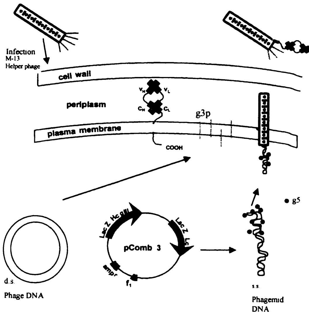
Figure IV-2b Assembly of recombinant antibodies displayed on the surface of filamentous phage.- Recombinant Fab fused to the g3p protein remain associated with the plasma membrane. Upon infection with M13 helper phage, single stranded phagemid DNA is synthesized by a viral DNA polymerase, which is promptly packaged as progeny phage, through the help of several phage encoded proteins, in particular g5. As the progeny phage mature and extrude across the plasma membrane, the recombinant Fab-g3p fusion protein become associated with, and cap the trailing extremity of the particles. As only five to six g3p proteins associate with the progeny phage extremity, there is a competition between the M-13 helper phage-encoded g3p and the Fab-g3p fusion protein for the phage. It has been estimated, than on average there is one to three Fab-g3p fusion proteins per phage particle.
