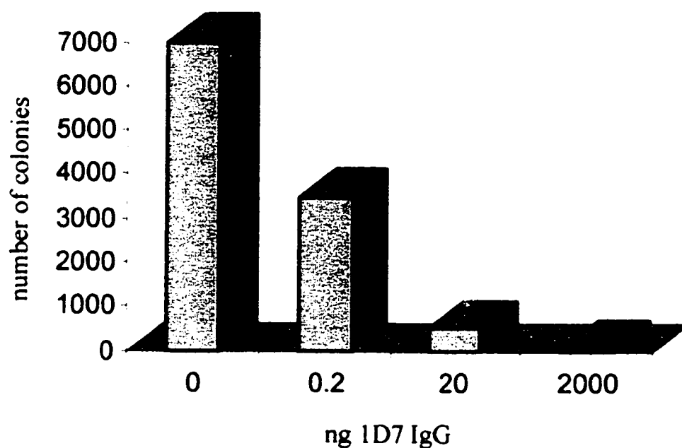
Figure IV-7 Assessment of the antigen-binding specificity of 2E8 phab preparations.- This histogram depicts the antigen-binding specificity of 2E8 phab preparations, as determined using the phage rescue procedure. ApoE coated wells were filled with equal amounts of freshly isolated 2E8 phab, diluted once in 4 % BSA-PBS, and increasing amounts of the cross-reacting, apo-E specific mAb 1D7 were added as a competitor. As shown by the first bar in the diagram, when no competitor mAb was added, many colonies were observed. However, as increasing amounts of the 1D7 mAb were added, correspondingly fewer bacteria were rescued, demonstrating the specificity of the 2E8 phab interaction. This type of competition was not observed when an irrelevant mAb, such as mAb 3H1 was added as a competitor.
