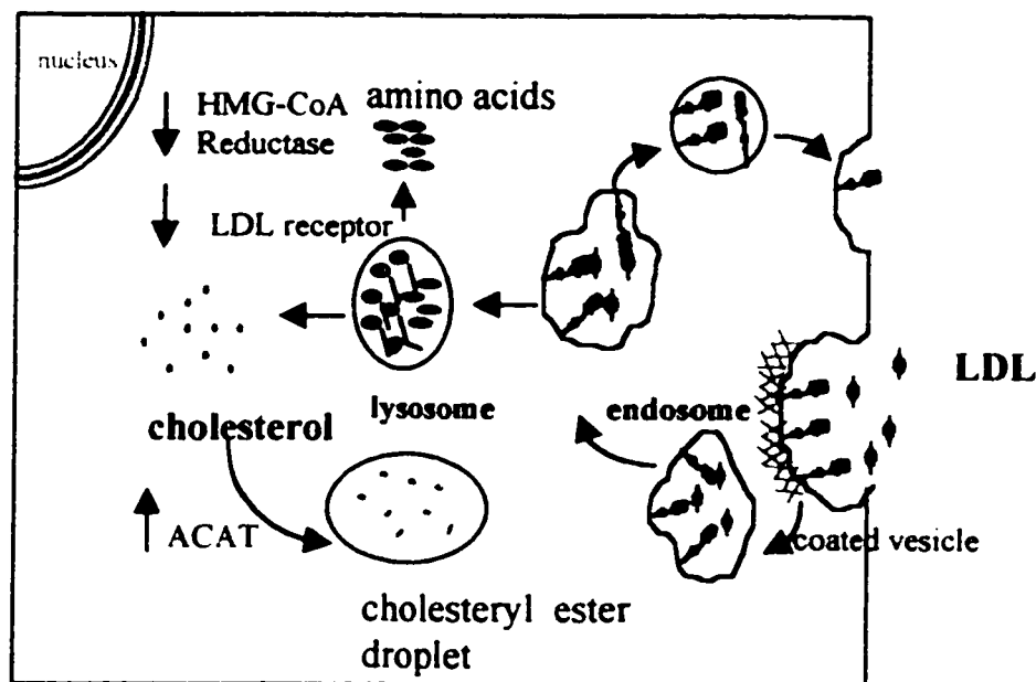
Figure I-11 The LDL-Receptor Pathway
