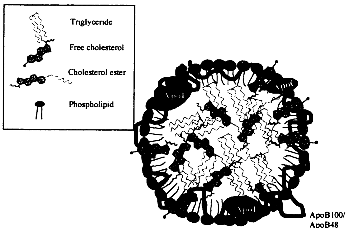
Figure I-1 Schematic diagram of a metabolic lipoprotein particle.
