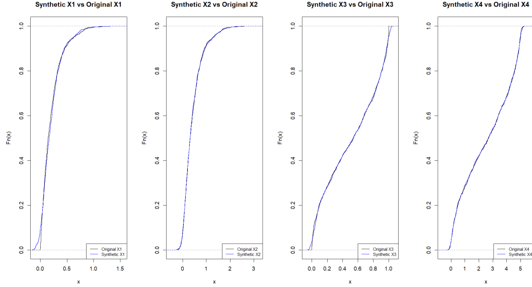
Figure 4.5: Comparison of original and empirical ECDF when there is no sequential relationship proposed algorithm
