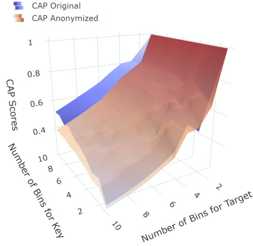
Figure 2.7: 3D plot of equal length method, CAP vs. number of bins for target and key
