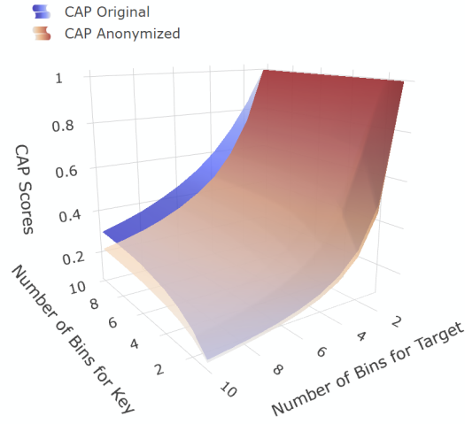
3D Surface Plot of CAP Scores for Equal Frequency
