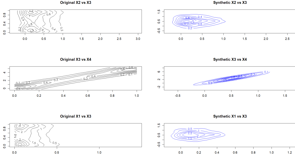
Figure 4.4: Comparison of contour plot when there is no sequential relationship
