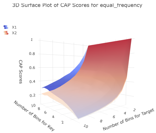
Figure 2.13: Comparison of CAP anonymized score between 2 randomization algorithm
