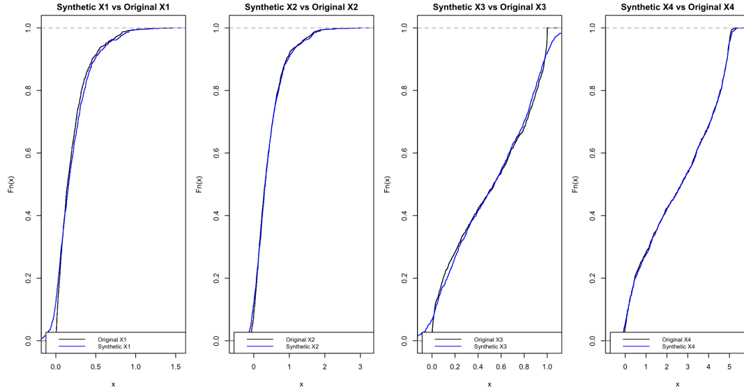
Figure 4.7: Comparison of original and empirical ECDF with proposed DP method
