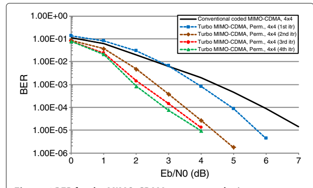
Figure 6 BER for the MIMO-CDMA system employing permutation spreading with N_t = 4 and N_r = 4 .
