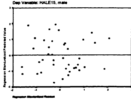
Figure 5.3b Plot of standardized residuals against HALE, male model.
