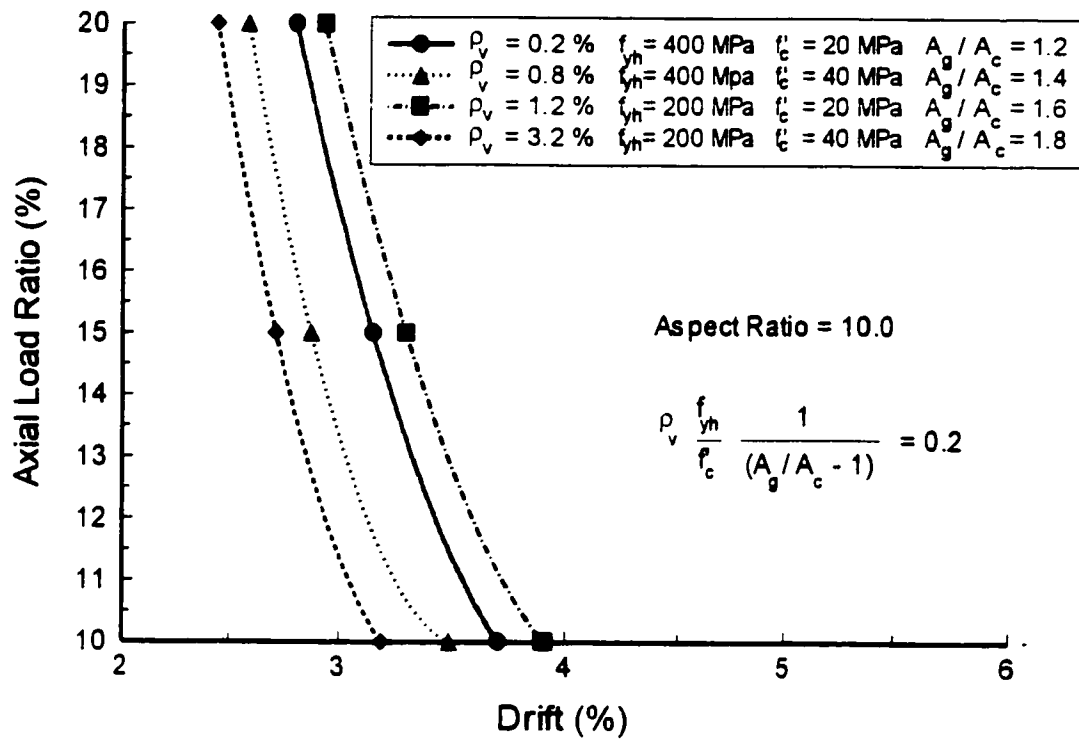
Figure 3.22 Effect of different concrete covers and different levels of confinement on drift capacity of columns.
