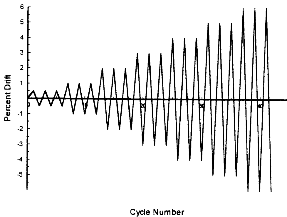
Figure 5.12 Loading program.
