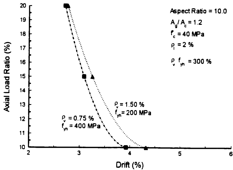
Figure 3.20 Effect of the product of volumetric transverse reinforcement ratio and hoop steel yield stress on drift capacity of columns.
