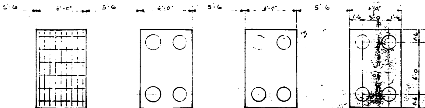
FOOTING PLAN
