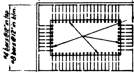
PLAN OF FOOTING
