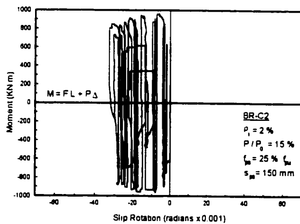
Figure 5.27 Moment-Rotation relationships for column BR-C2.
