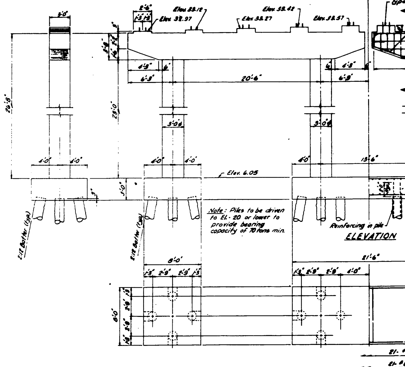
PLAN-FOOTINGS
