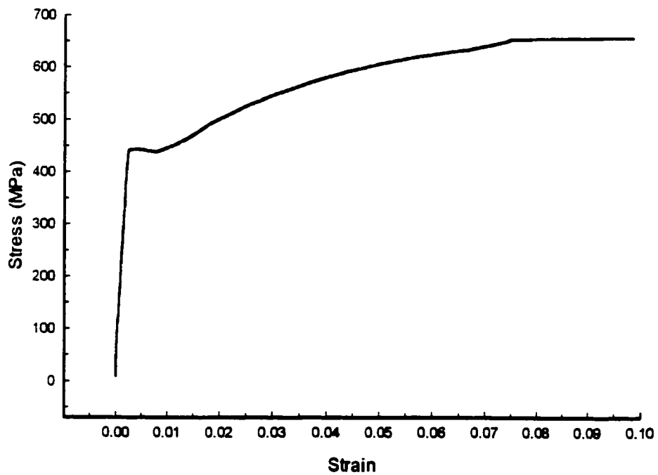
Figure 5.5 Stress-strain relationship of Grade 400, No. 25 deformed reinforcing steel.
