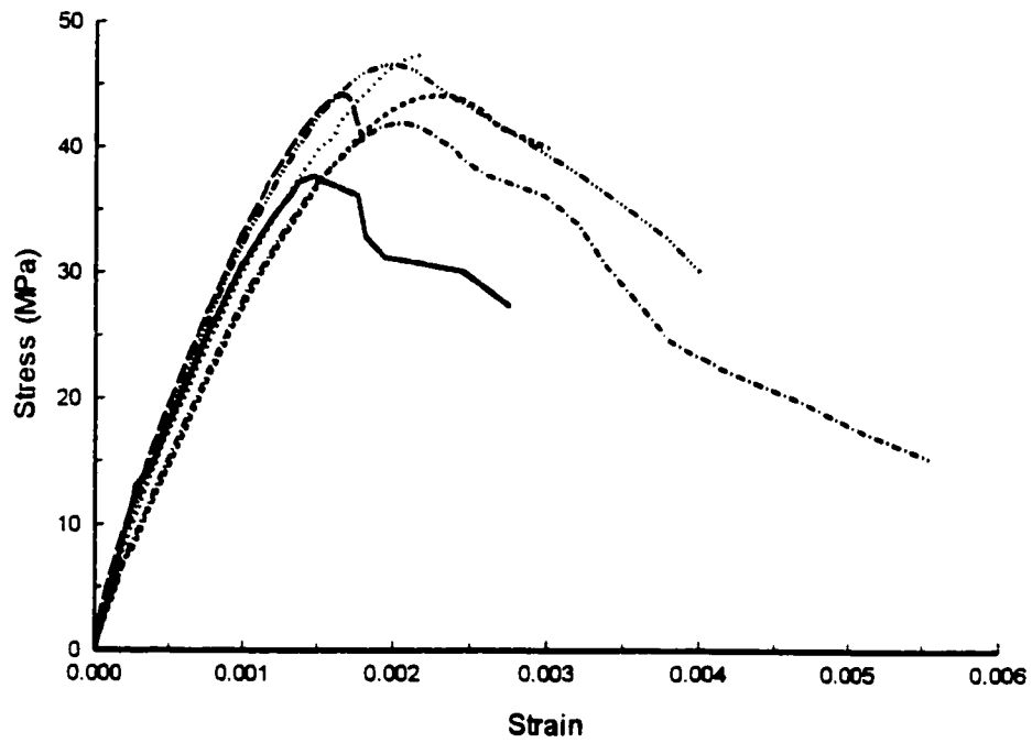
Figure 5.4 Stress-strain relationship of concrete cylinders.
