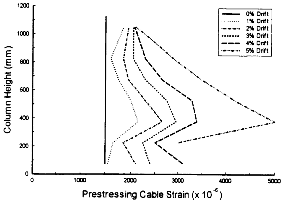
Figure 5.50 Prestressing wire strain profile for column BR-C2.
