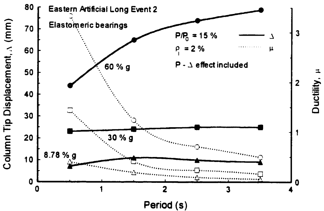
Figure 4.10 Eastern earthquake response of bridges with elastomeric bearings with P- \Delta effect.
