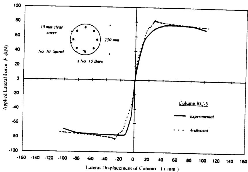
Comparison of Force - Displacement Relationships for Columns RC-5 (Experimental and Analytical - Without P-\Delta effect)
