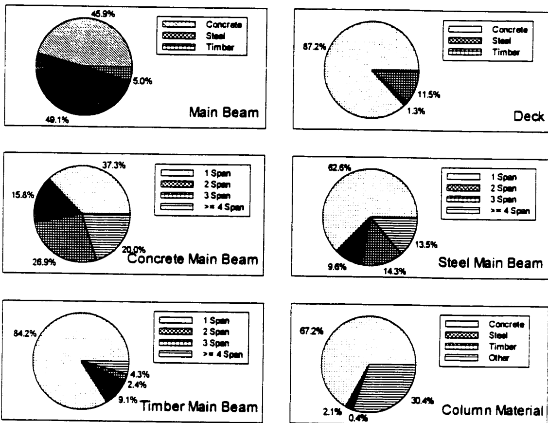
Figure 2.1 Classification of Ontario Bridges.
