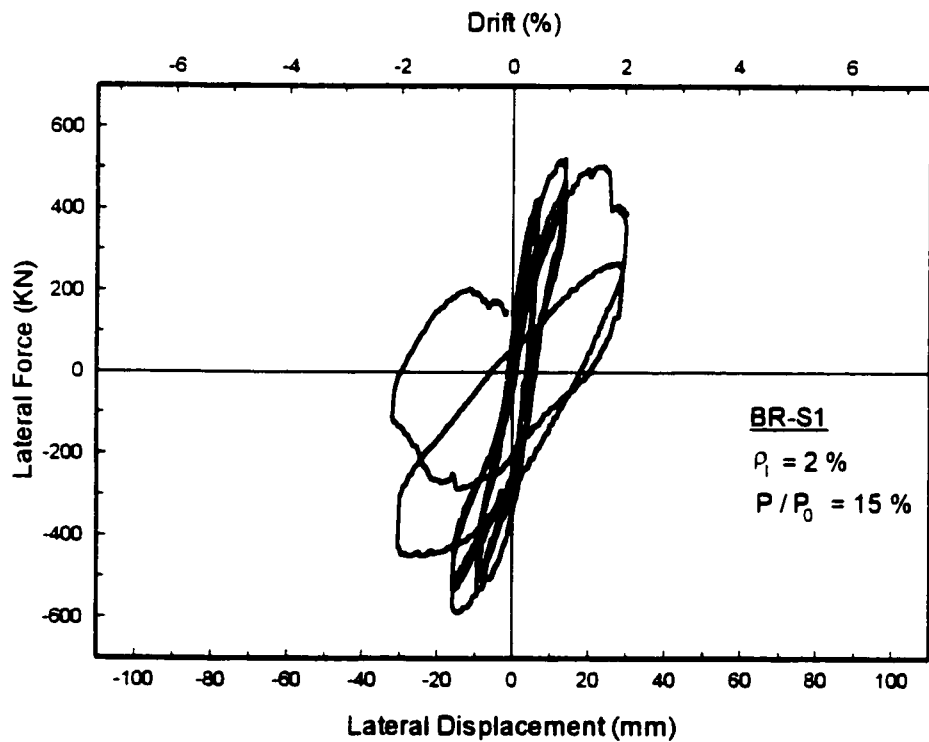
Figure 5.18 Moment-Displacement and Force-Displacement relationships for column BR-S1.
