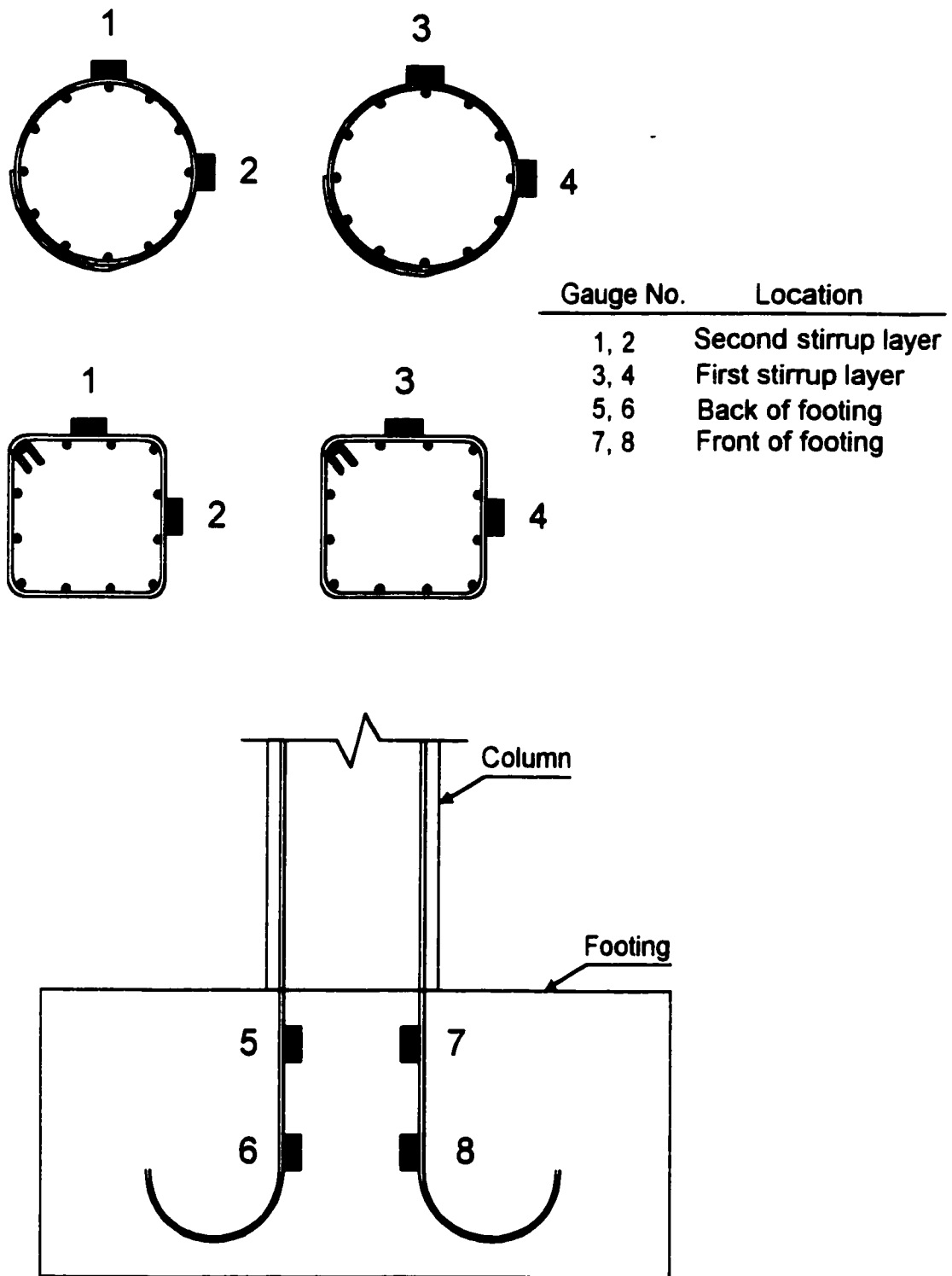
Figure 5.9 Strain gauge location on reinforcing steel.
