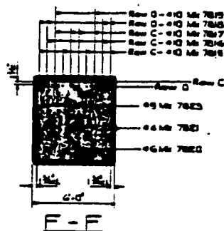
PLAN OF PIER TOP
