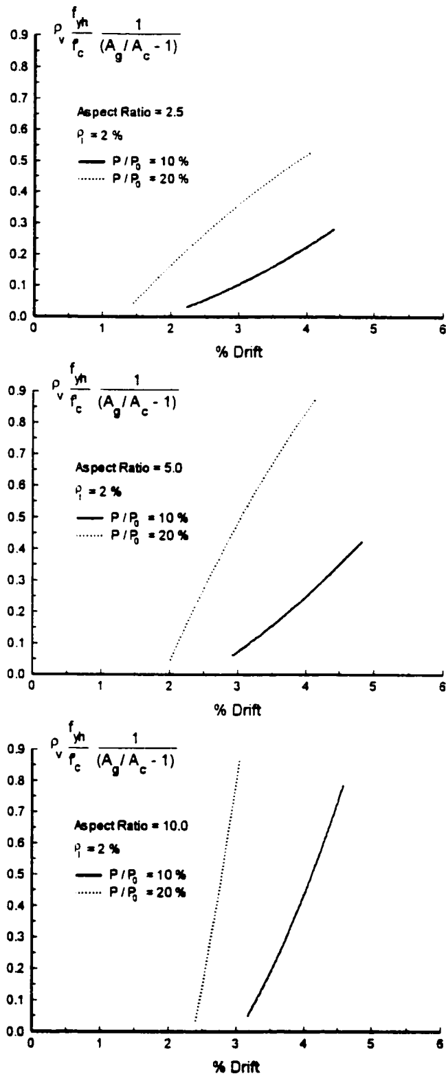
Figure 3.24 Design charts for circular columns ( \rho_l = 2\% ).
