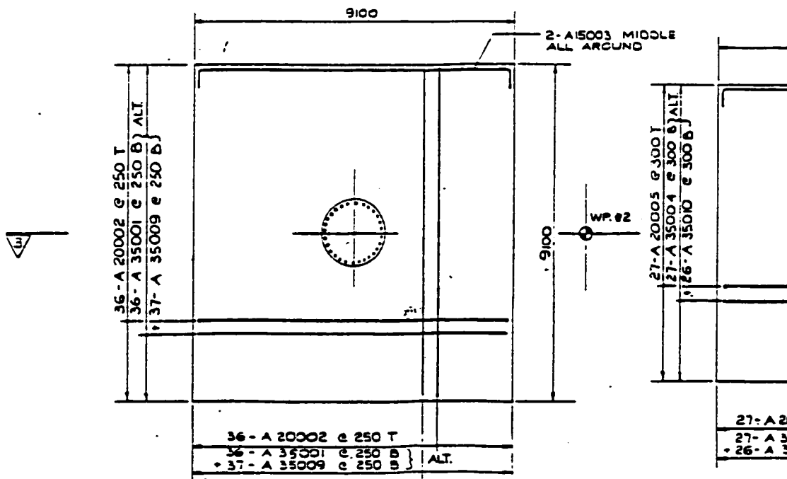
FOOTING REINFORCING
