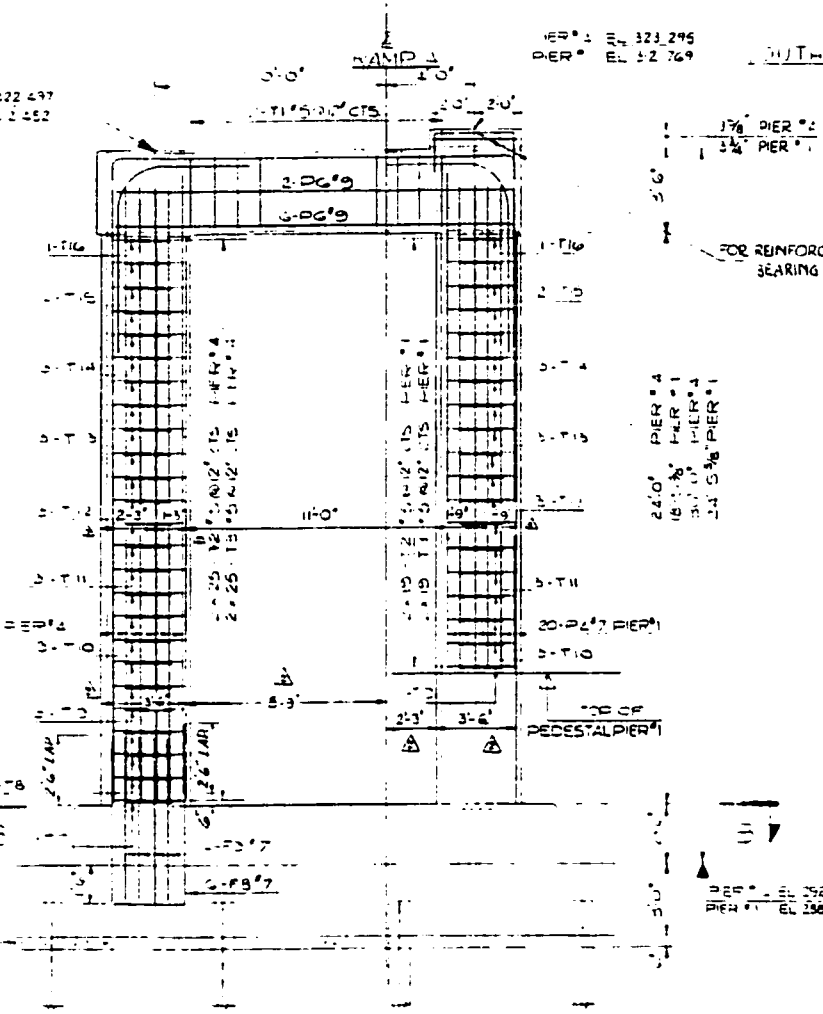
ELEVATION OF PIER #4
