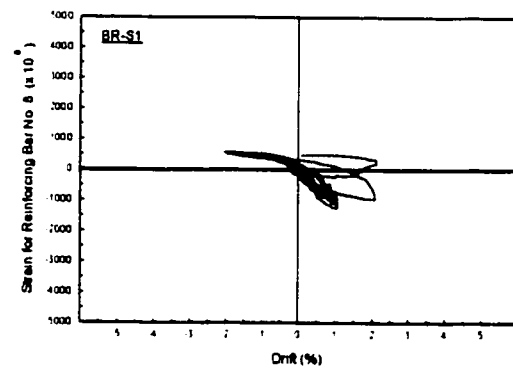
Figure 5.20 Reinforcing steel strains for column BR-S1.
