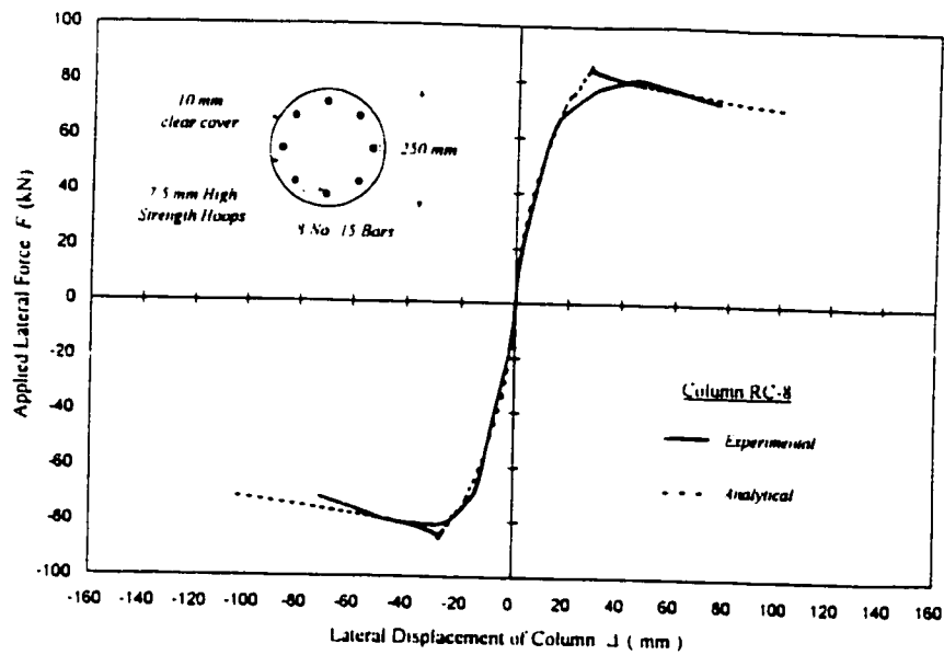
Comparison of Force - Displacement Relationships for Columns RC-8 (Experimental and Analytical - Without P-\Delta effect)
