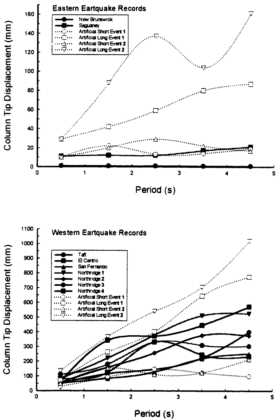
Figure 4.6 SDOF analysis of Eastern and Western Earthquake records normalized to 30% of g .
