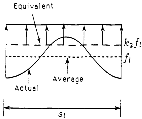
(c) Actual, average and equivalent lateral pressures
