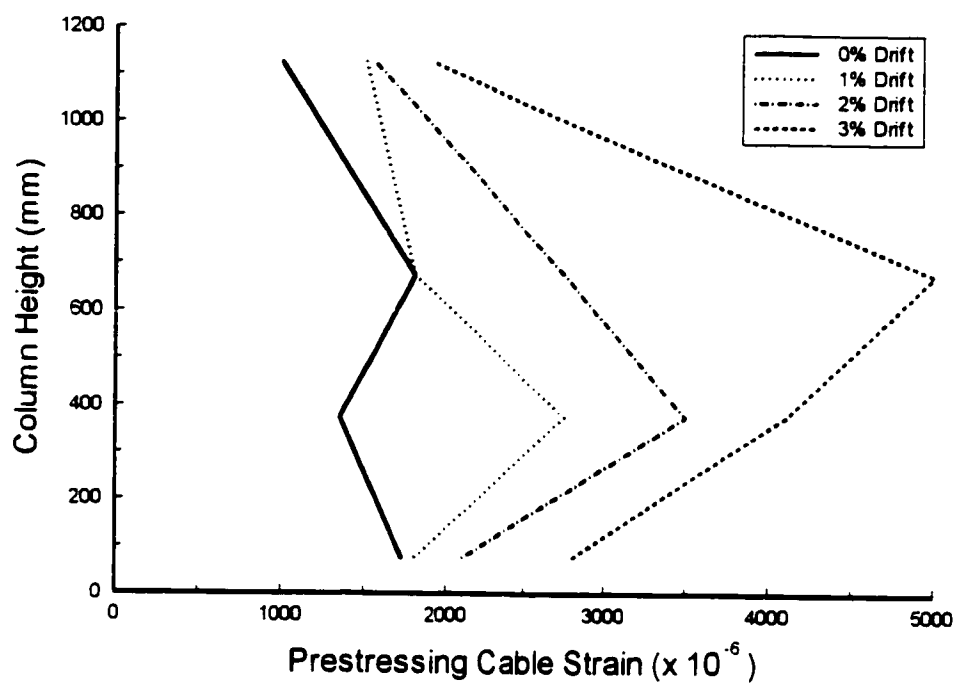
Figure 5.52 Prestressing wire strain profile for column BR-C4.
