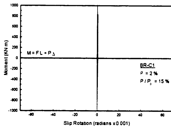
Figure 5.23 Moment-Rotation relationships for column BR-C1.
