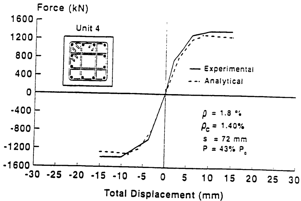
Figure 3.12 Comparisons of analytical and experimental lateral force-displacement relationships for columns tested by Sheikh and Khourey; Park, Priestley and Gill.
