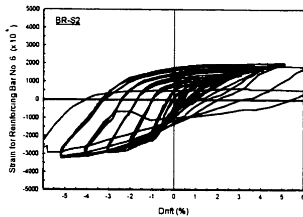
Figure 5.48 Reinforcing steel strains for column BR-S2.
