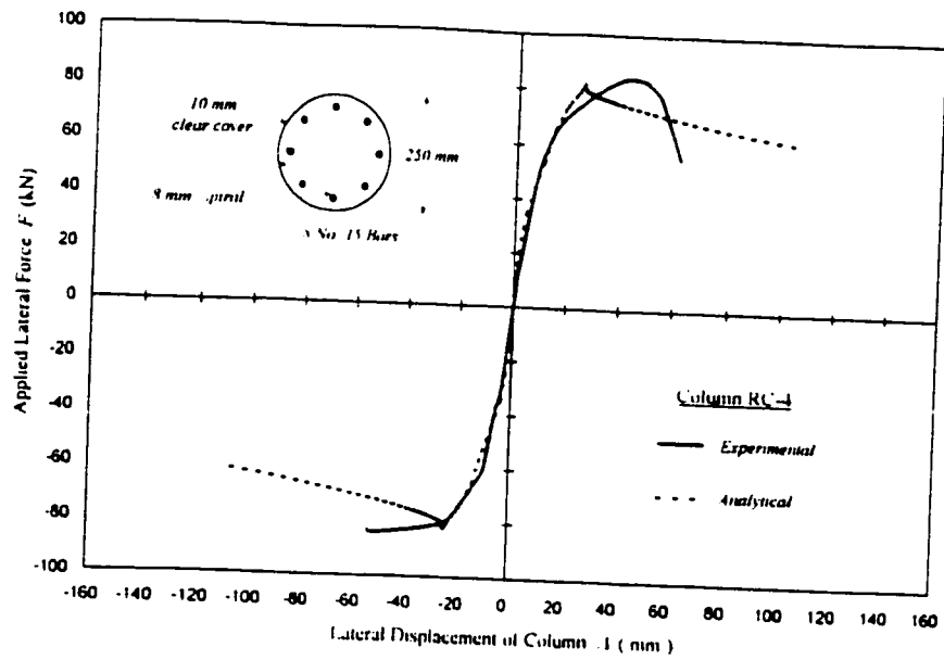
Comparison of Force - Displacement Relationships for Columns RC-4 (Experimental and Analytical - Without P-\Delta effect)
