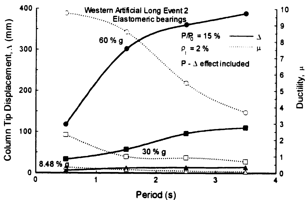
Figure 4.12 Western earthquake response of bridges with elastomeric bearings with P- \Delta effect.
