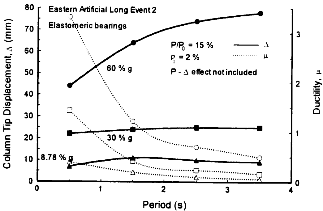
Figure 4.9 Eastern earthquake response of bridges with elastomeric bearings without P- \Delta effect.
