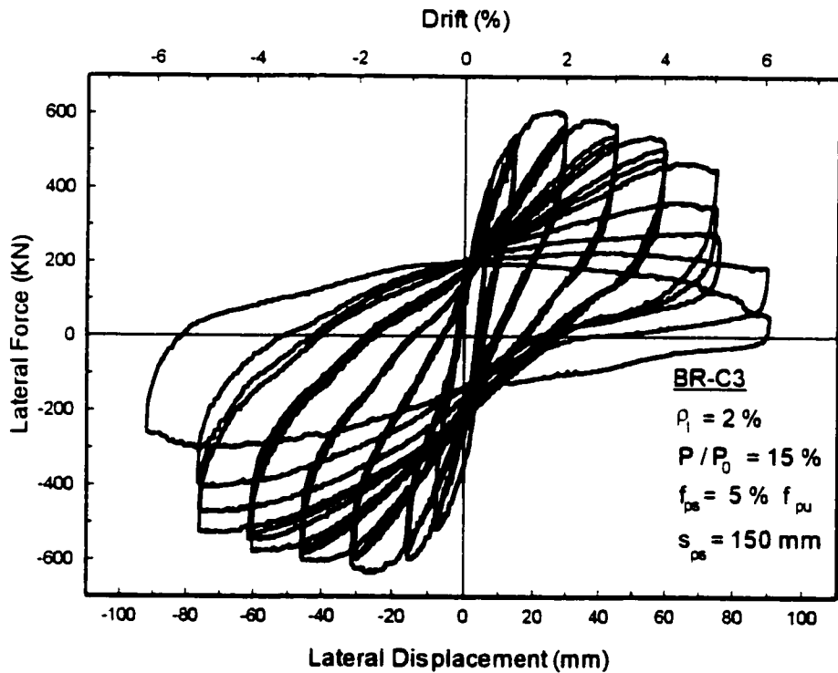
Figure 5.31 Moment-Displacement and Force-Displacement relationships for column BR-C3.
