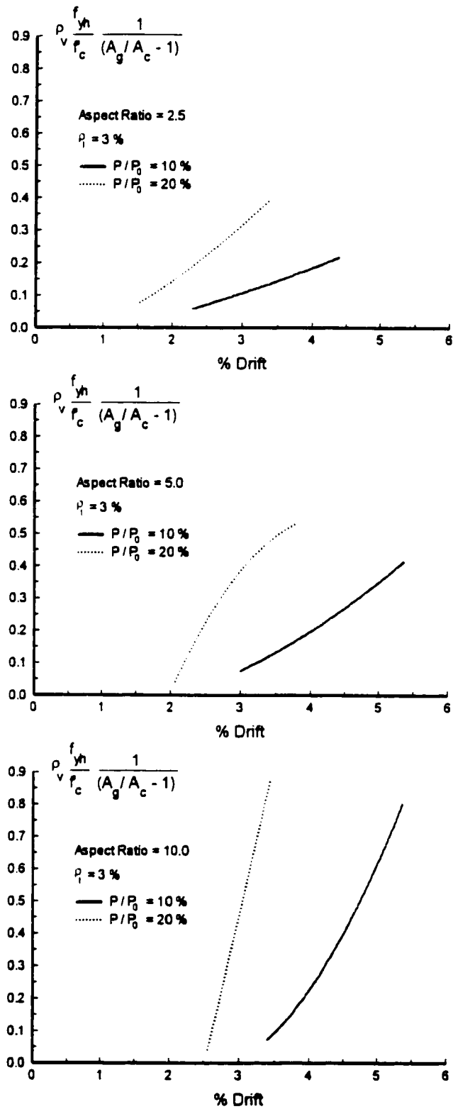
Figure 3.25 Design charts for circular columns ( \rho_l = 3\% ).
