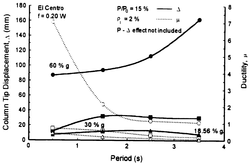
Figure 4.17 El Centro Earthquake response of bridges with roller or rocker bearings without P- \Delta effect.
