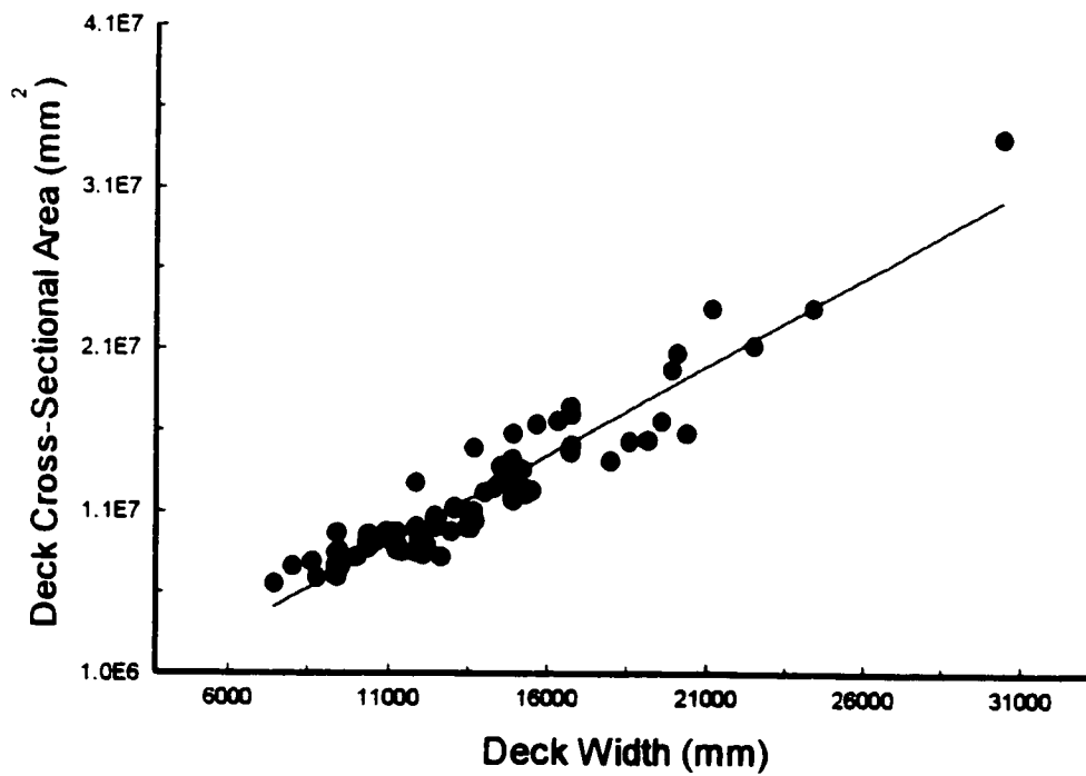
Figure 2.5 Statistical analysis of round-voided post-tensioned decks.
