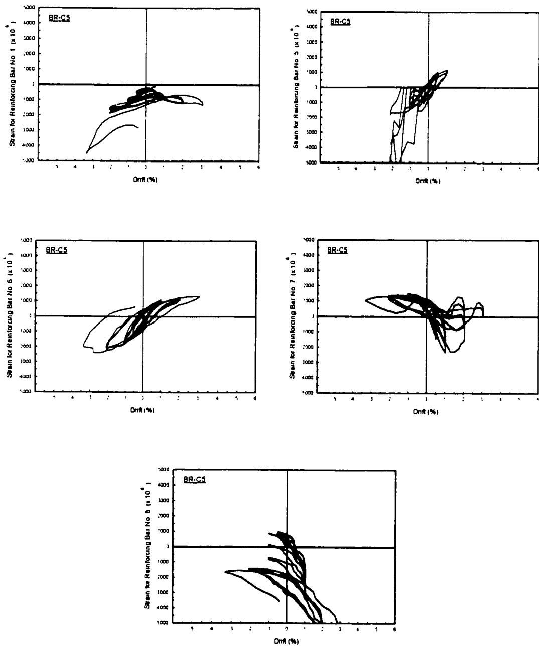
Figure 5.43 Reinforcing steel strains for column BR-C5.
