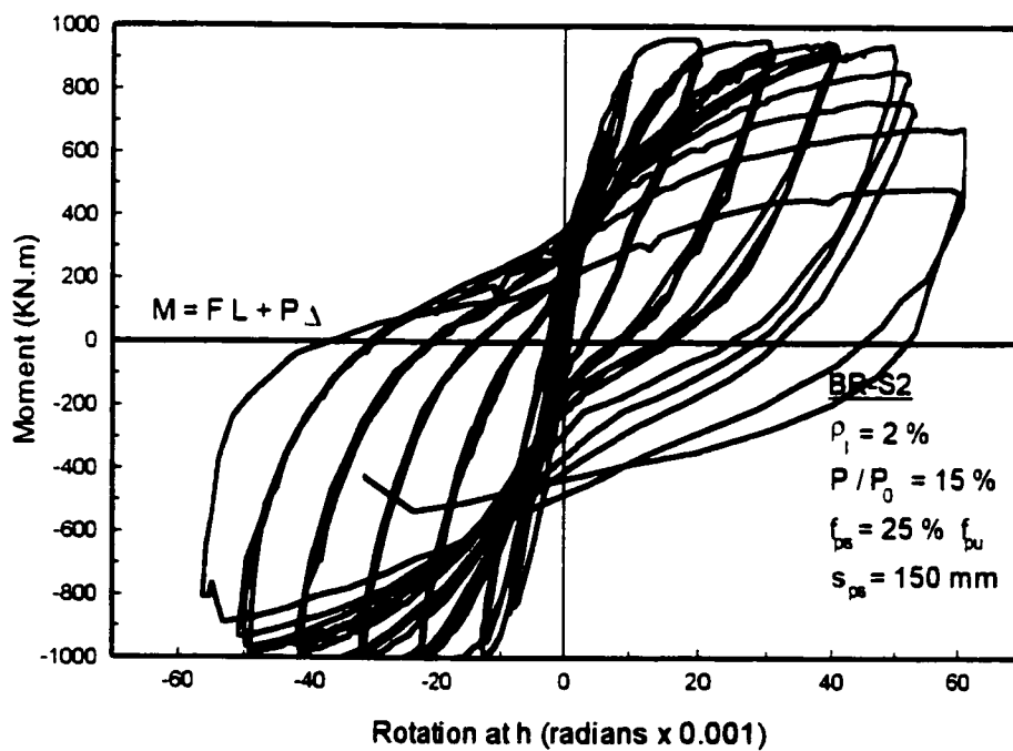
Figure 5.47 Moment-Rotation relationships for column BR-S2.
