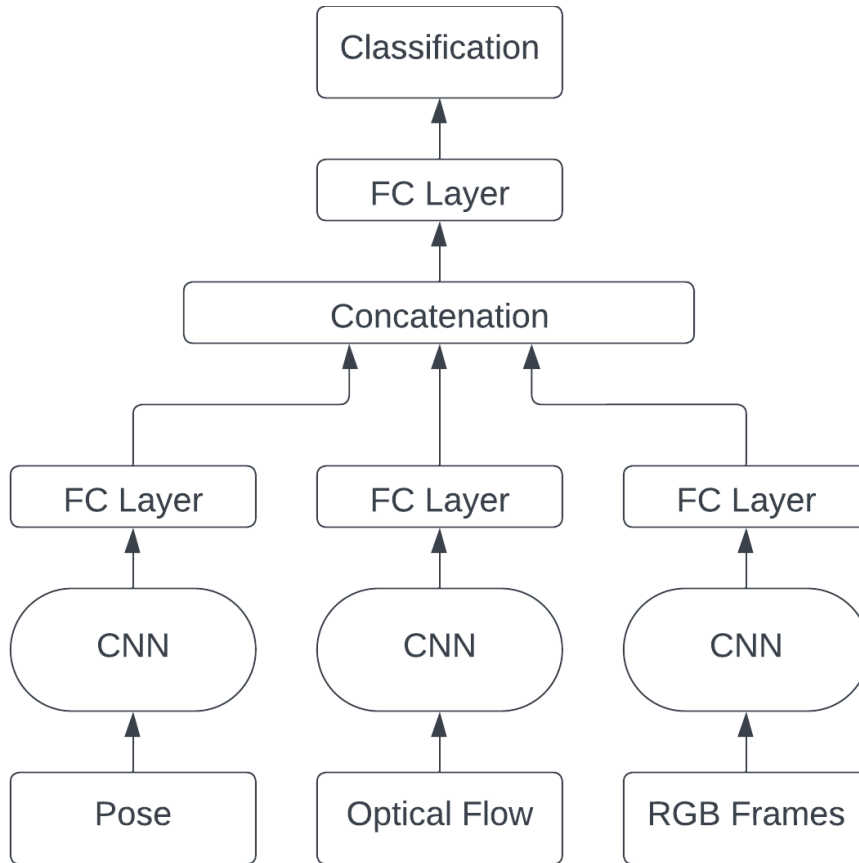
FIGURE 2.20: A typical fused architecture. Each of the Pose, Optical Flow, and RGB Frames are passed through individual 3D-CNN's, the outputs are then concatenated to achieve a final output.
