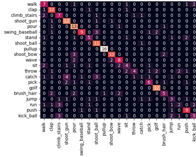
(b) Split 2
