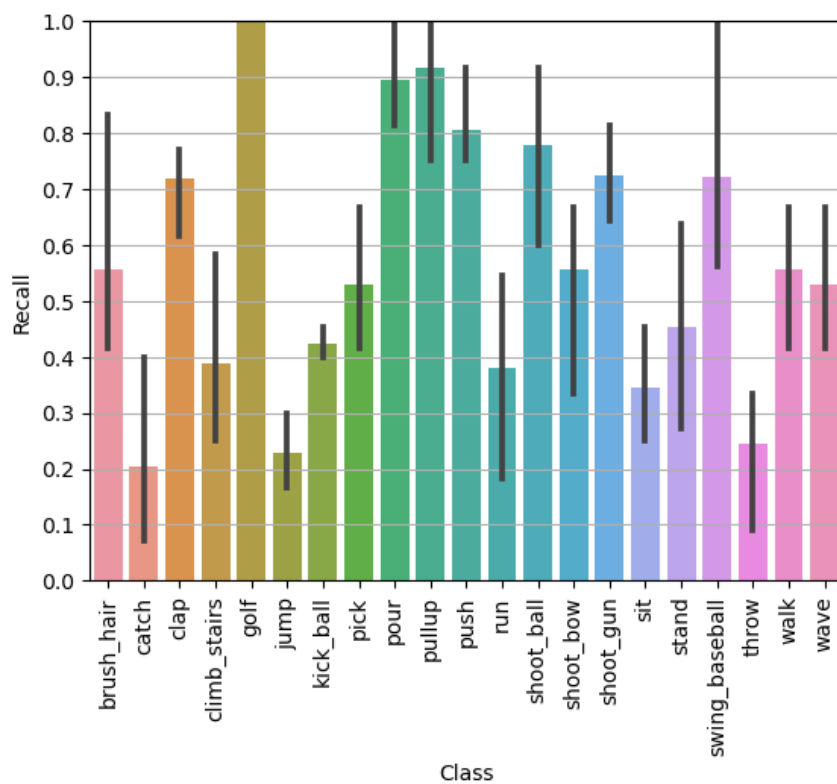
(b) Recall
