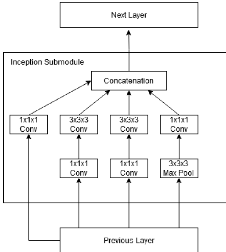
FIGURE 2.13: The detailed inception submodule used in the I3D model [6].
