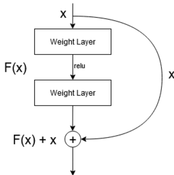
FIGURE 2.5: The Residual Block utilized by the ResNet [12] model. The input is added to the output of the convolutional block, resulting in an output that has both the output of the convolutions as well as the original input, which can then be fed into further blocks.
