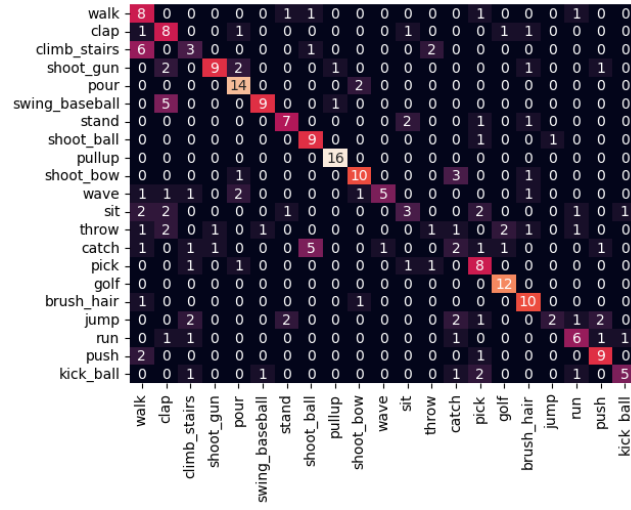
(a) Split 1
