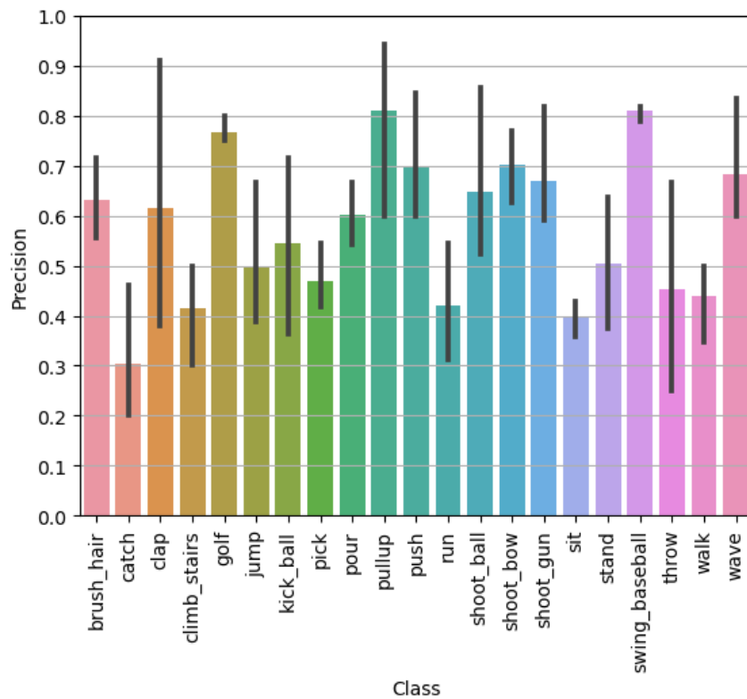
(a) Precision
