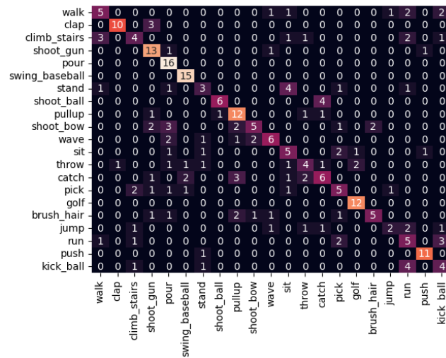
(c) Split 3
