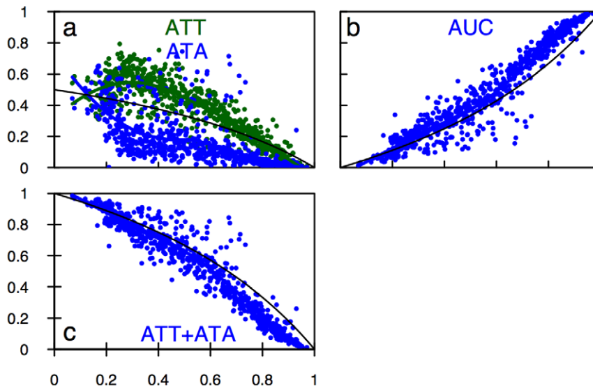
Figure 5. Codon usage frequency for isoleucine based on prokaryotic data. The x-axis is genomic GC3 as an estimate of GC bias, The y-axis is usage frequency. The colored points and lines correspond to the observed codon usage frequencies for a given GC3 and the corresponding loess fit respectively. The black line is the model prediction. (A) ATT and ATA codons. (B) ATC codon. (C) The sum of the ATA+ATT codon usages. doi:10.1371/journal.pone.0013431.g005
