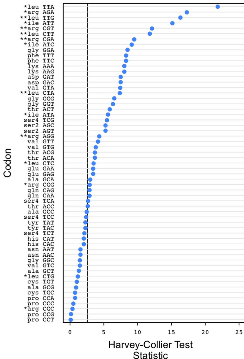
Figure 2. Graph of Harvey-Collier test statistic for codon bias as a function of GC3 for prokaryotes, ordered by decreasing magnitude. Low values indicate linearity, high values indicate nonlinearity. * and ** indicate codons that our model predicts to be nonlinear and nonlinear, non-monotone respectively. doi:10.1371/journal.pone.0013431.g002
