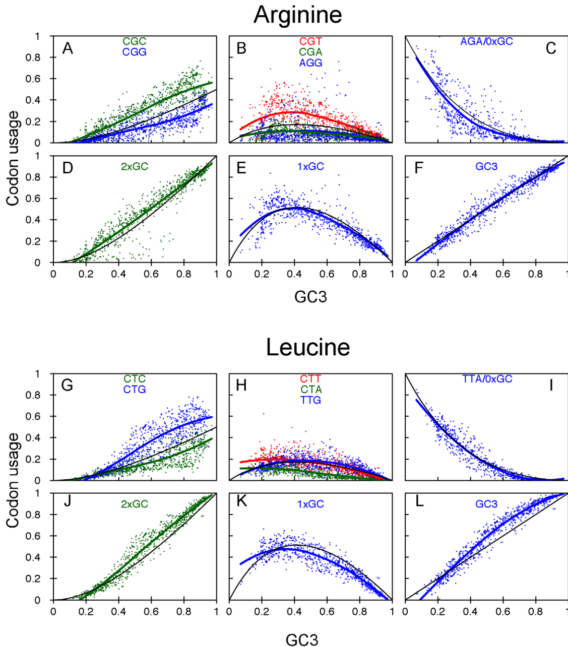
Figure 6. Codon usage frequency for arginine and leucine based on prokaryotic data. The x-axis is genomic GC3 as an estimate of GC bias, the y-axis is usage frequency. The colored points and lines correspond to the observed codon usage frequencies for a given GC3 and the corresponding loess fit respectively. The black line is the model prediction. (A) 2×GC arginine codons (those with two G/C in the 1st or 3rd codon position). (B) 1×GC arginine codons (those with one G/C in the 1st or 3rd codon position). (C) The 0×GC arginine codon (with no G/C in the 1st or 3rd codon position). (D) The sum of 2×GC arginine codons. (E) The sum of 1×GC arginine codons. (F) GC3 for arginine codons. (G) 2×GC leucine. (H) 1×GC leucine codons. (I) 0×GC leucine. (J) The sum of 2×GC leucine codons. (K) The sum of 1×GC leucine codons. (L) GC3 for leucine codons. doi:10.1371/journal.pone.0013431.g006
