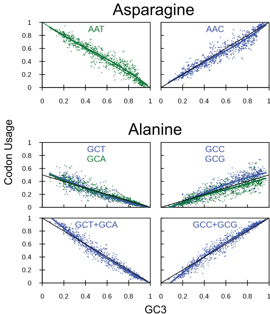
Figure 4. Codon usage frequency for asparagine and alanine based on prokaryotic data. The x-axis is genomic GC3 as an estimate of GC bias, The y-axis is usage frequency. The colored points and lines correspond to the observed codon usage frequencies for a given GC3 and the corresponding loess fit respectively. The black line is the model prediction. (A) Asparagine AAT codon. (B) Asparagine AAC codon. (C) Alanine GCT and GCA codons. (D) Alanine GCC and GCG codons. (E) The sum of the GCT + GCA alanine codons. (F) The sum of the GCC + GCG codons. doi:10.1371/journal.pone.0013431.g004
