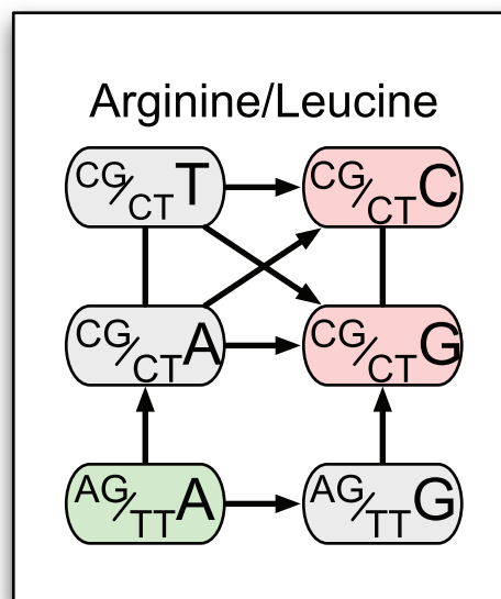
Figure 3. Networks of synonymous single site substitutions for all amino acids. GC increasing substitutions are indicated with an arrow. GC preserving substitutions are represented by a line. For amino acids with 2 and 4 codons as well as serine, G/C-ending codons are pink, and A/T-ending codons green. For arginine and leucine, codons with G/C in both synonymous positions ( 2 \times \text{GC} ) are red, those with only one G/C in a synonymous position ( 1 \times \text{GC} ) are grey, and those with A/T in both synonymous positions ( 0 \times \text{GC} ) are green. (A) Amino acids whose codons are predicted to have a linear response to GC mutational bias. (B) Isoleucine, whose codons are predicted to have a nonlinear but monotone response to GC mutational bias. (C) Arginine and leucine, whose codons are predicted to have nonlinear, and in some cases non-monotone, responses to GC mutational bias.
