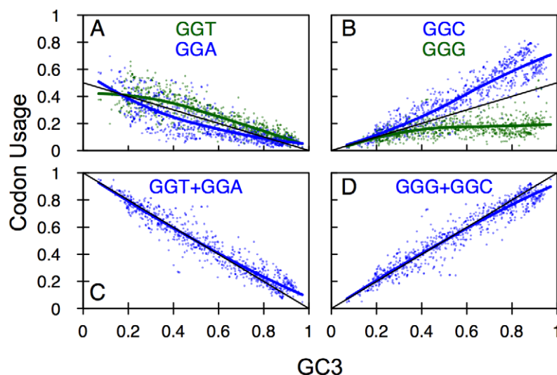
Figure 7. Codon usage frequency for glycine based on prokaryotic data. The x-axis is genomic GC3 as an estimate of GC bias, the y-axis is usage frequency. The colored points and lines correspond to the observed codon usage frequencies for a given GC3 and the corresponding loess fit respectively. The black line is the model prediction. (A) Glycine A/T-ending codon usage. (B) Glycine G/C-ending codon usage. (C) Glycine A/T-ending codon usage summed. (D) Glycine G/C-ending codon usage summed.
