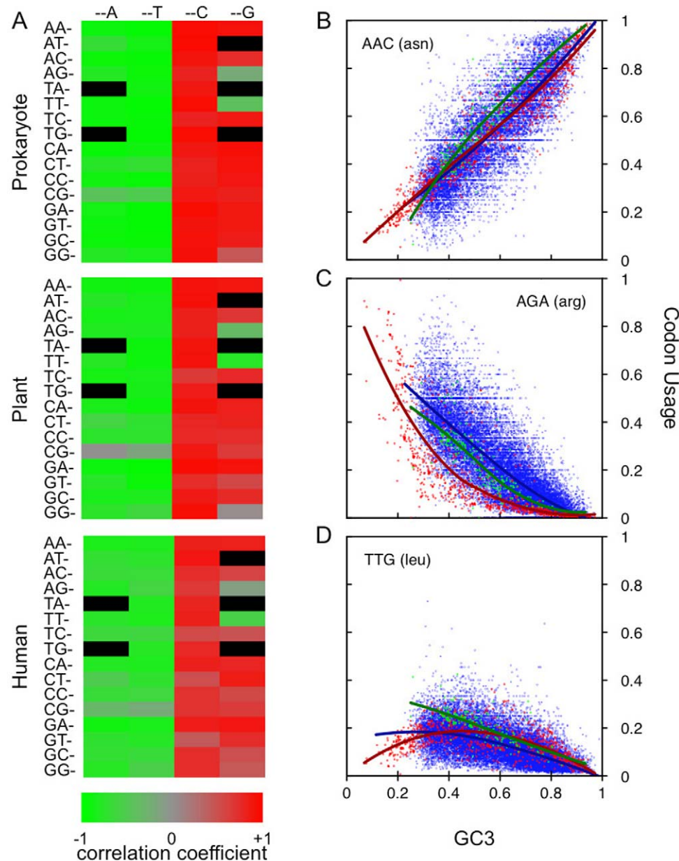
Figure 1. Relationships between codon usage and GC3. (A) Heat maps of correlation values for codon usage vs GC3 for bacteria and plant genomes and human genes. The color and intensity indicates type and degree of correlation: red indicates positive, green negative. Black fields are stop and non-degenerate codons (tryptophane and methionine). AGG and TTG are the only G/C-ending codons having negative correlation with GC3. (B) Codon usage frequency for the asparagine codon AAC (linear). Red, green and blue points and lines are, respectively, bacterial, plant and human scatter plots and LOESS fits of codon usage frequency versus GC3. This is also the case for Figures 1C and 1D. (C) Codon usage frequency for the arginine codon AGA (nonlinear, but monotone). (D) Codon usage frequency for the leucine codon TTG (nonlinear and non-monotone). doi:10.1371/journal.pone.0013431.g001
