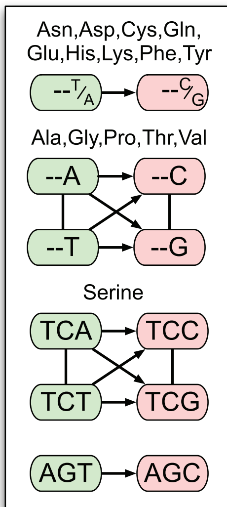
Figure 3. Networks of synonymous single site substitutions for all amino acids. GC increasing substitutions are indicated with an arrow. GC preserving substitutions are represented by a line. For amino acids with 2 and 4 codons as well as serine, G/C-ending codons are pink, and A/T-ending codons green. For arginine and leucine, codons with G/C in both synonymous positions ( 2 \times \text{GC} ) are red, those with only one G/C in a synonymous position ( 1 \times \text{GC} ) are grey, and those with A/T in both synonymous positions ( 0 \times \text{GC} ) are green. (A) Amino acids whose codons are predicted to have a linear response to GC mutational bias. (B) Isoleucine, whose codons are predicted to have a nonlinear but monotone response to GC mutational bias. (C) Arginine and leucine, whose codons are predicted to have nonlinear, and in some cases non-monotone, responses to GC mutational bias.
