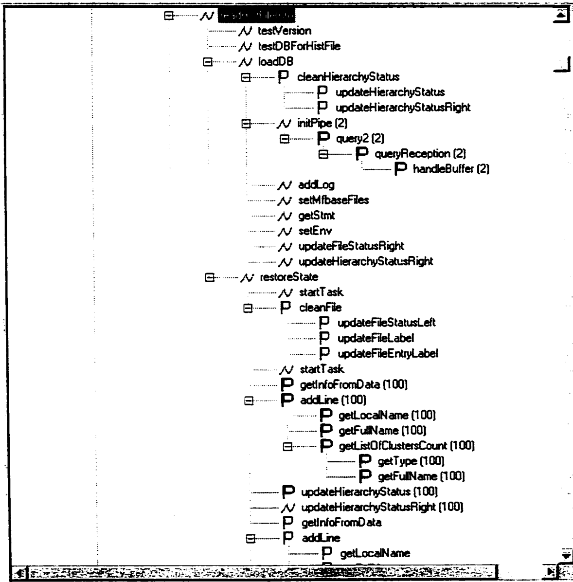
Figure 8: DynaSee call tree, the P nodes belong to patterns while the N nodes do not. Note the numbers in brackets: they represent compressed repetitions
