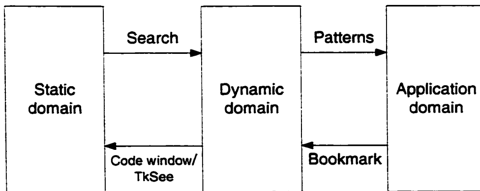
Figure 10: the support for domain mapping in DynaSee.
