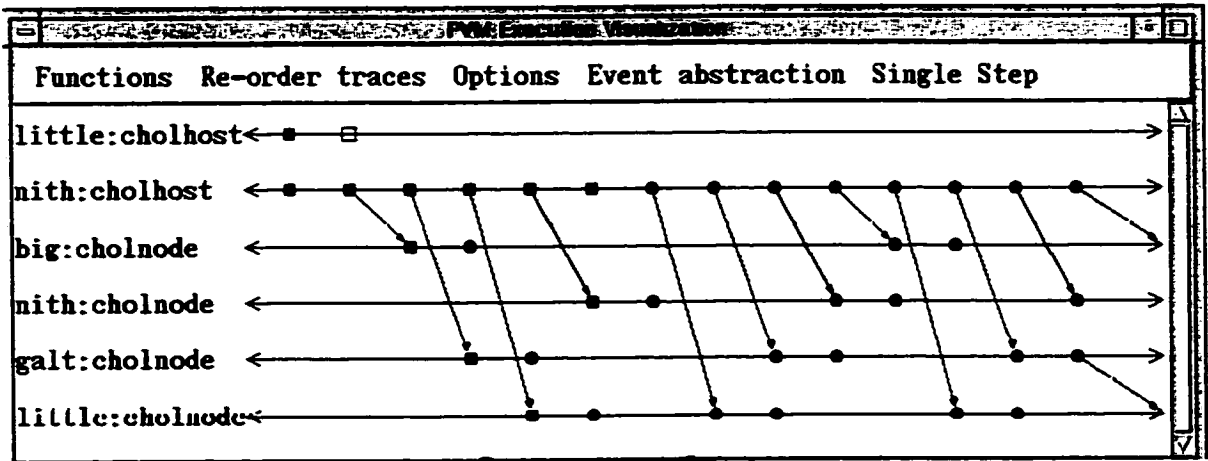
Figure 2: POET screen dump
