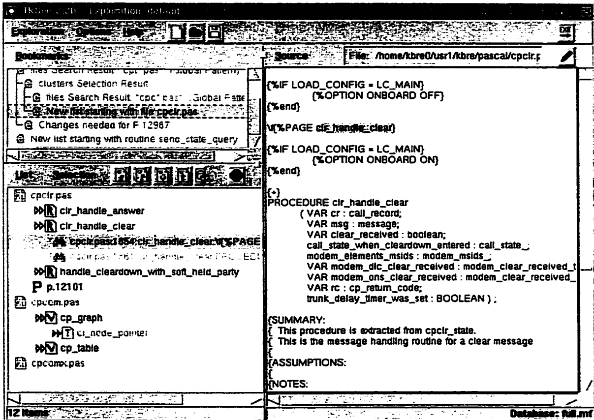
Figure 1: Screen dump of TkSee: the exploration pane (left) shows symbols. The source code for the selected routine is displayed in at the right pane. The top-left history pane shows the current task.
