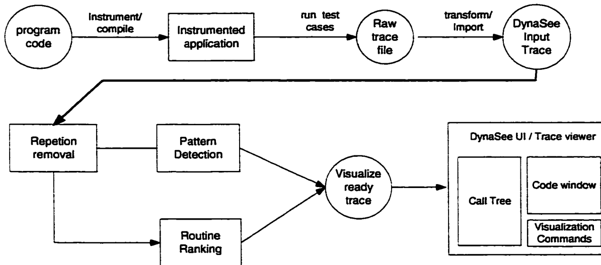
Figure 6: Processing phases in DynaSee where a box corresponds to processing and a circle to a data in a particular format
