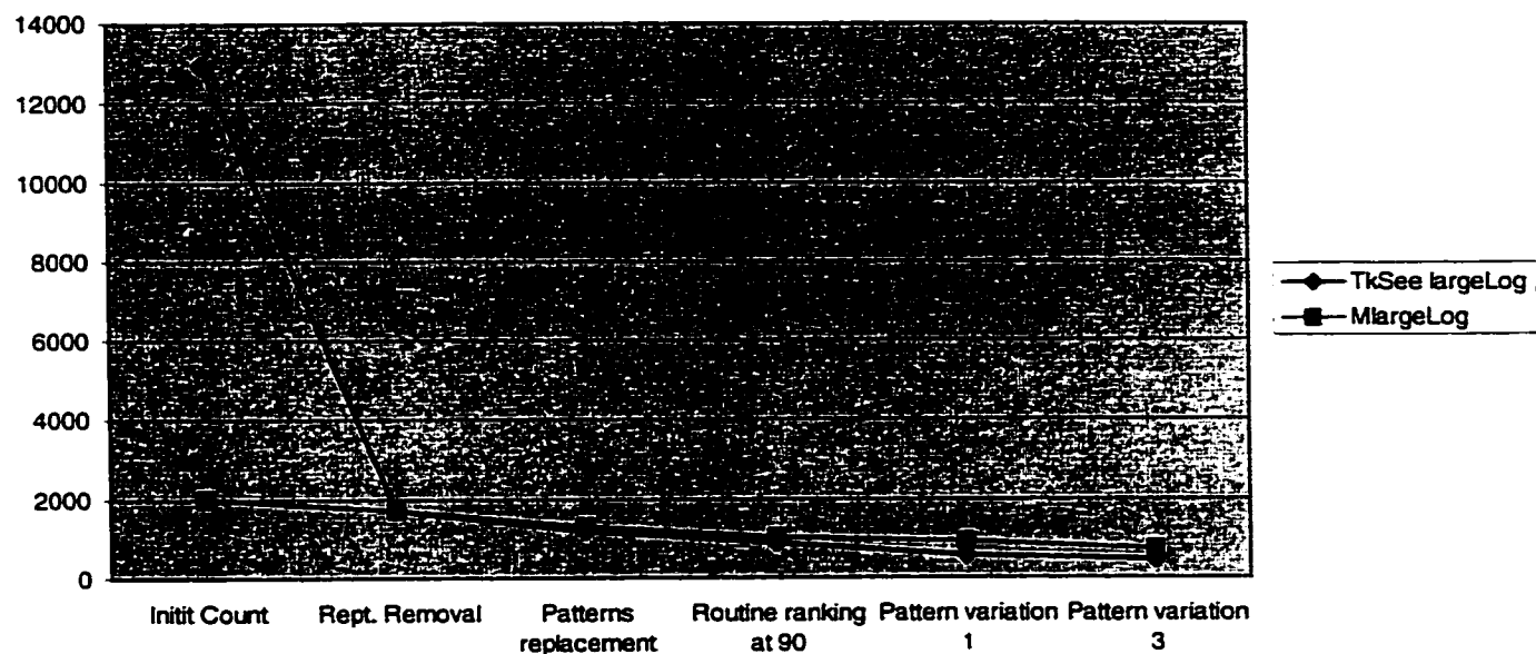
Figure 12: Graph showing the compression rate after applying each feature
