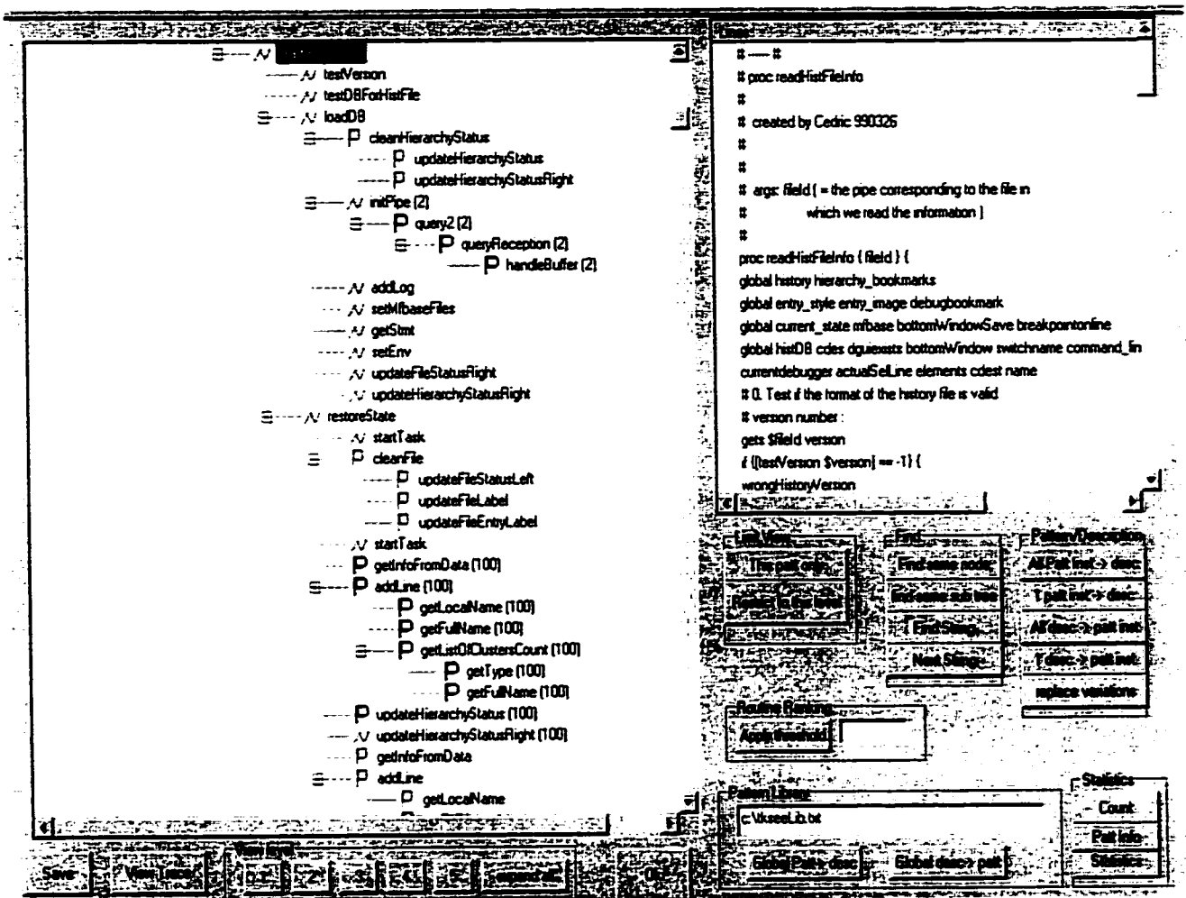
Figure 5: A screen dump of DynaSee where the call tree is on the left and code window on the right
