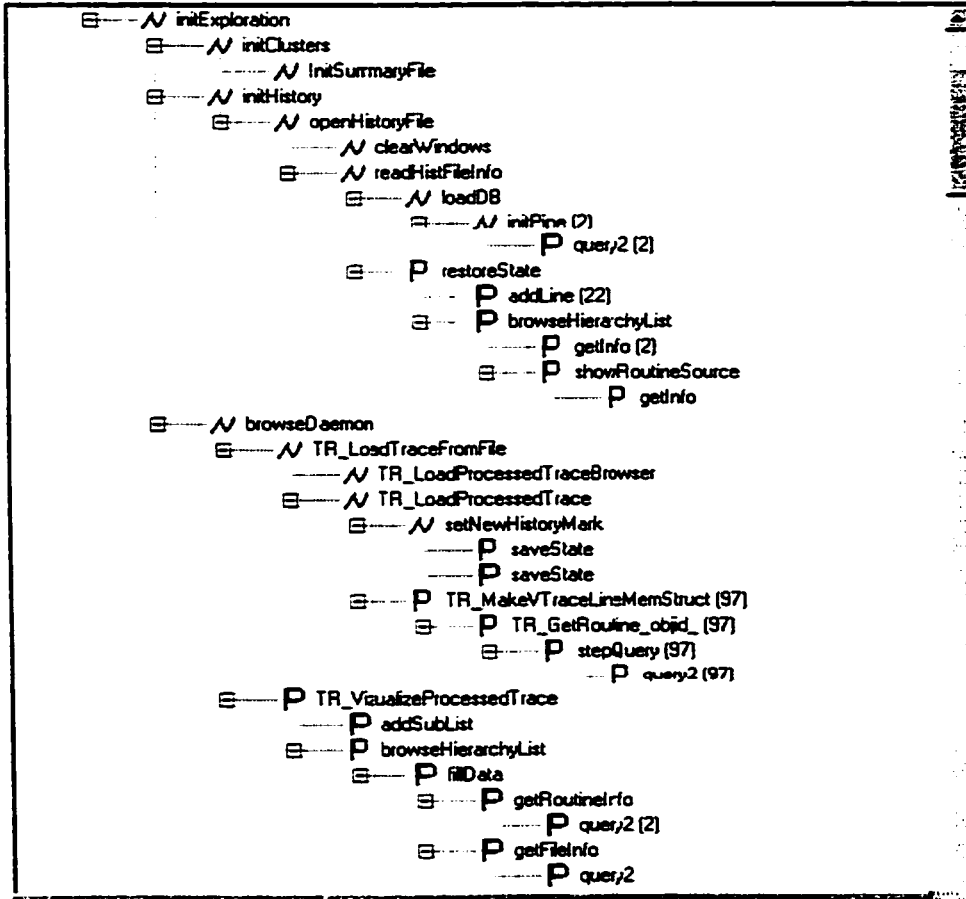
Figure 11: the diagonal shape of the call tree branches after W is set to 71
