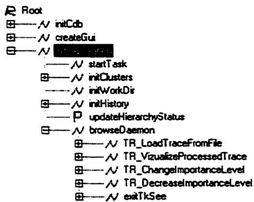
Figure 9: Call tree collapsed to form a visual pattern
