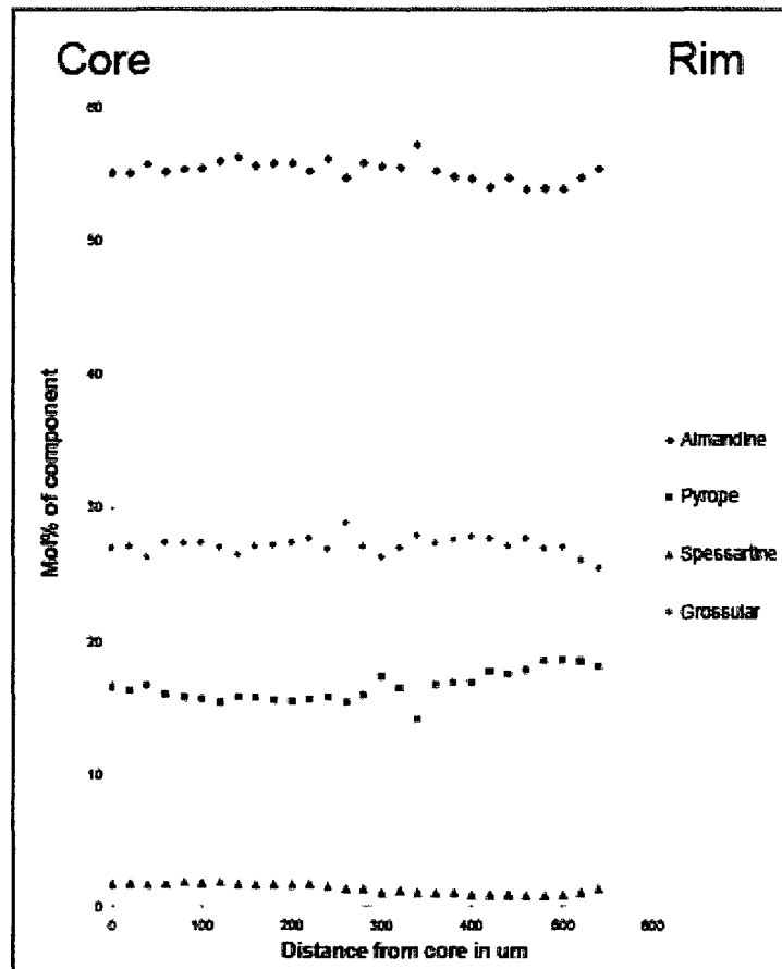
Figure 4.1: Eclogite garnet zoning profile of sample ZT-17-01 presented in mol% compositions of garnet end-members. The original growth zoning is only partially preserved and retrograde zoning is apparent at the rim.
