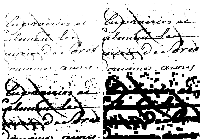
Figure 4.1: Original image (top-left), segmented output with window size set to 1 (top-right), segmented output with window size set to 5 (bottom-left), segmented output with window size set to 15. (bottom-right)
