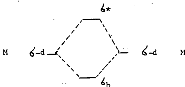
Figure 14: \sigma_b =bonding orbital; \sigma^* =antibonding orbital.
