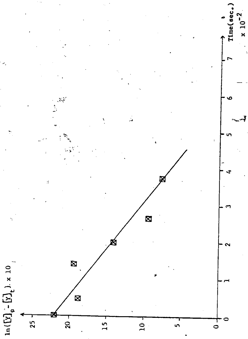
Figure 9: A plot of \ln([Y]_e - [Y]_t) against time for 54d at 274.5K .
