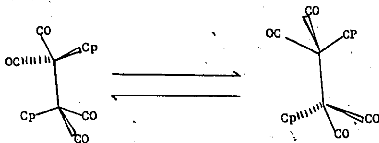
Scheme XVII
