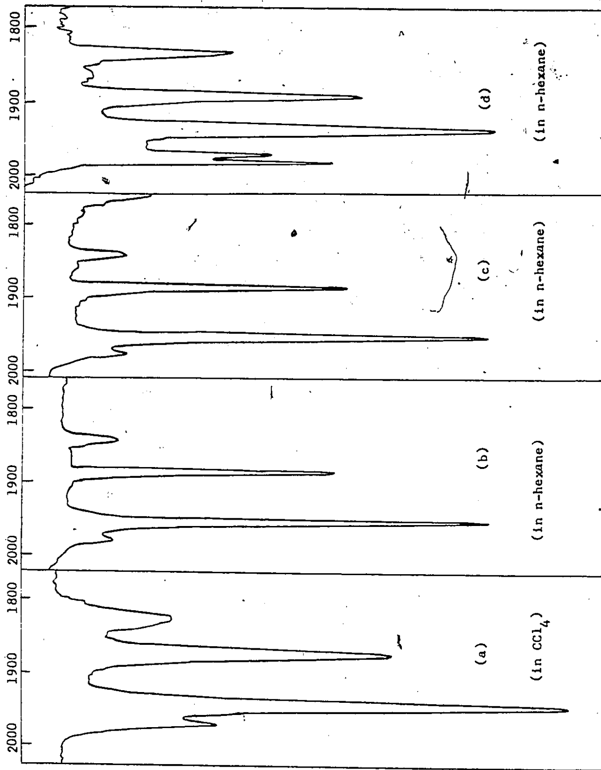
Figure 1: Infrared spectra ( \nu_{C=O} ) of (Cp)_2Mo_2(CO)_4 (L equals (a) (4-H_3COC_6H_4)_2CS , (b) (C_6H_5)_2CS , (c) 4-H_3COC_6H_4C(S)C_6H_5 and (d) adamantanethione).
