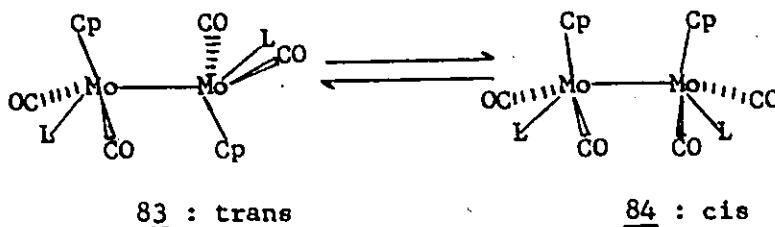
Scheme XIII: (L = \text{P}(\text{OCH}_3)_3 , \text{P}(\text{OC}_2\text{H}_5)_3 )
