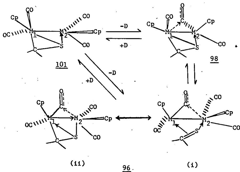
Scheme XVIII ( M_1=M_2=Mo, W ; D =Solvent Molecule).
