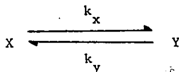
Scheme XXII
