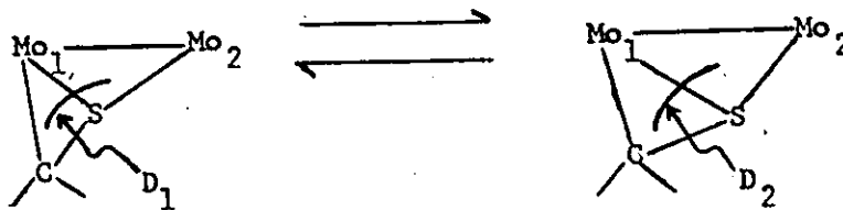
Scheme XIX ( D_1 < D_2 )
