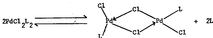
Scheme XXIII
