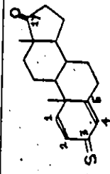
71 (in 64)
