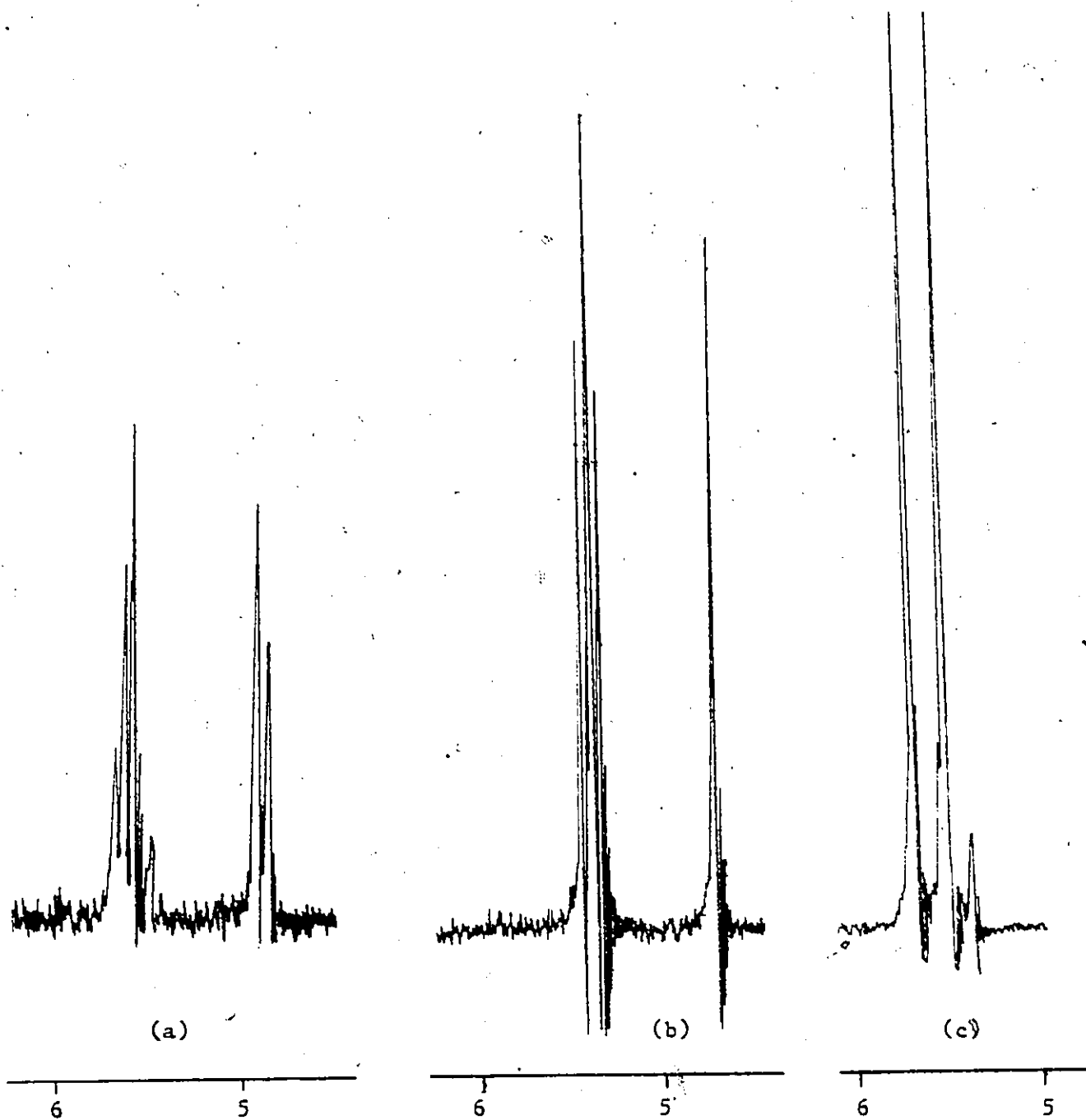
Figure 11: Cyclopentadienyl proton chemical shifts ( \delta ppm) of (Cp_2Mo_2(CO)_4L) in DMSO: (a) L=4-H_3COC_6H_4 \cdot C(S) \cdot C_6H_5 (b) L=(4-FC_6H_4)CS and (c) L=thiocamphor .
