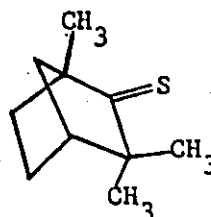
Thiofenchone ( 16 )
