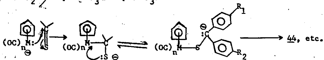
Scheme XI
