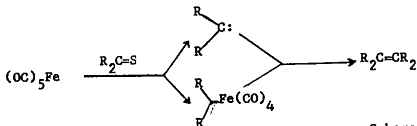
Scheme VIII
