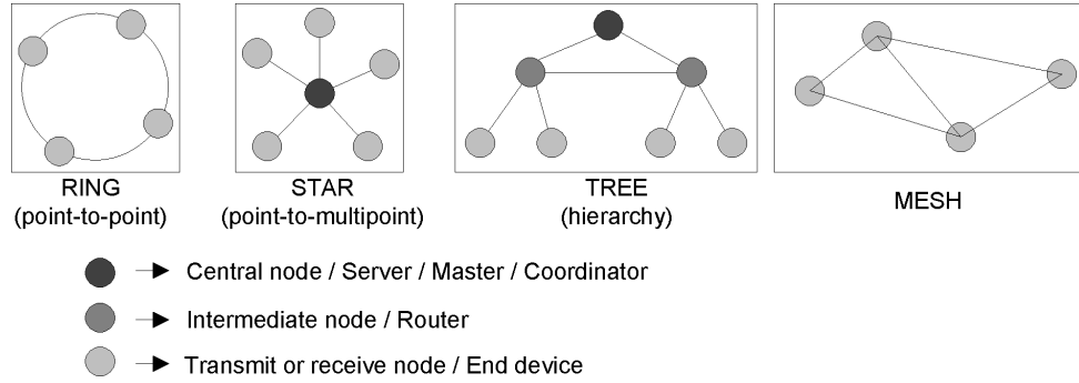
Figure 2.5: Network Topologies
