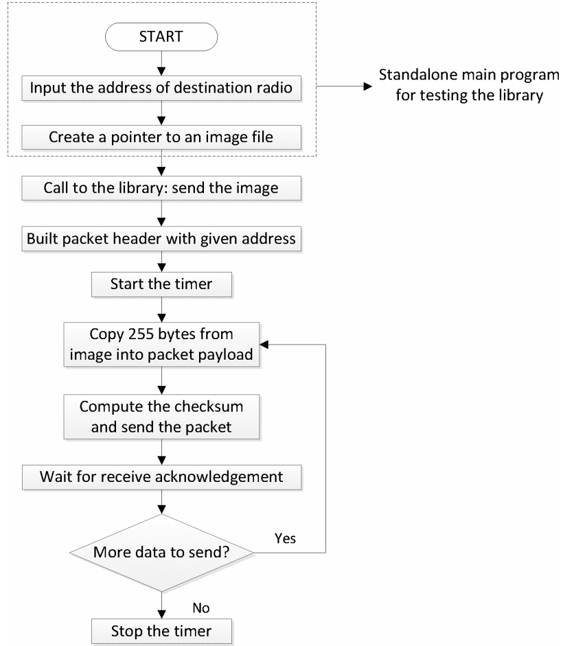
Figure 4.3: Program structure for timing image transmission
